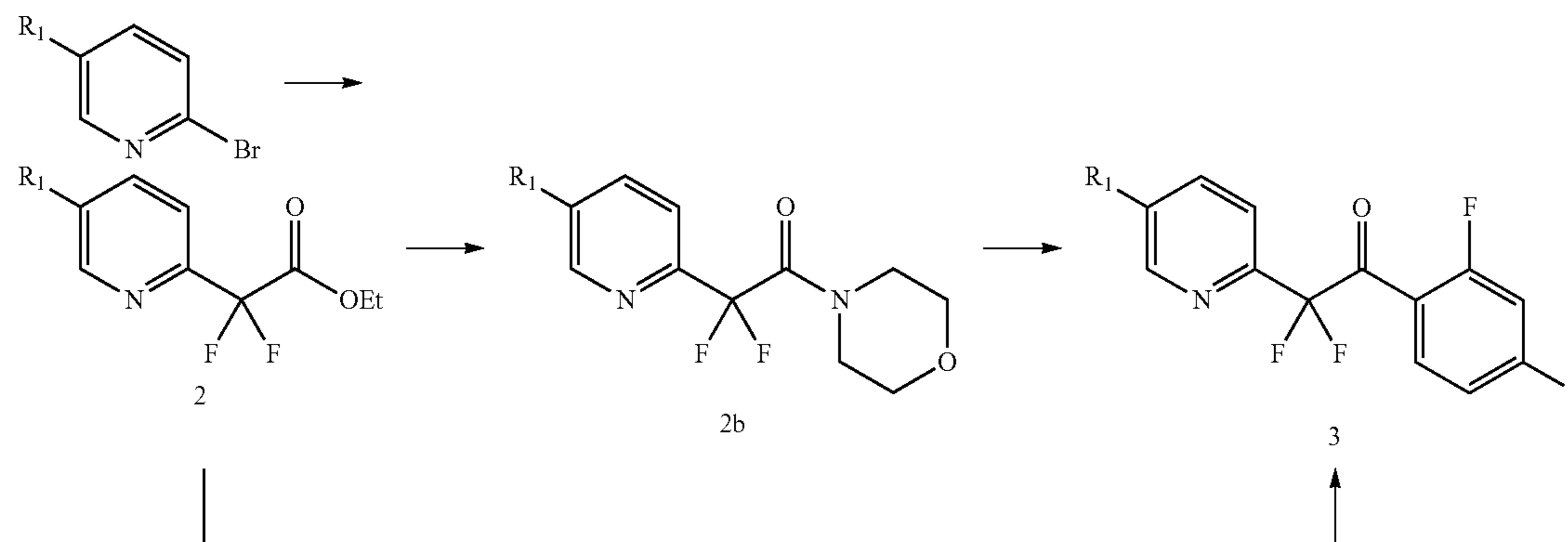
Scheme 2. Synthesis of ketone 3
