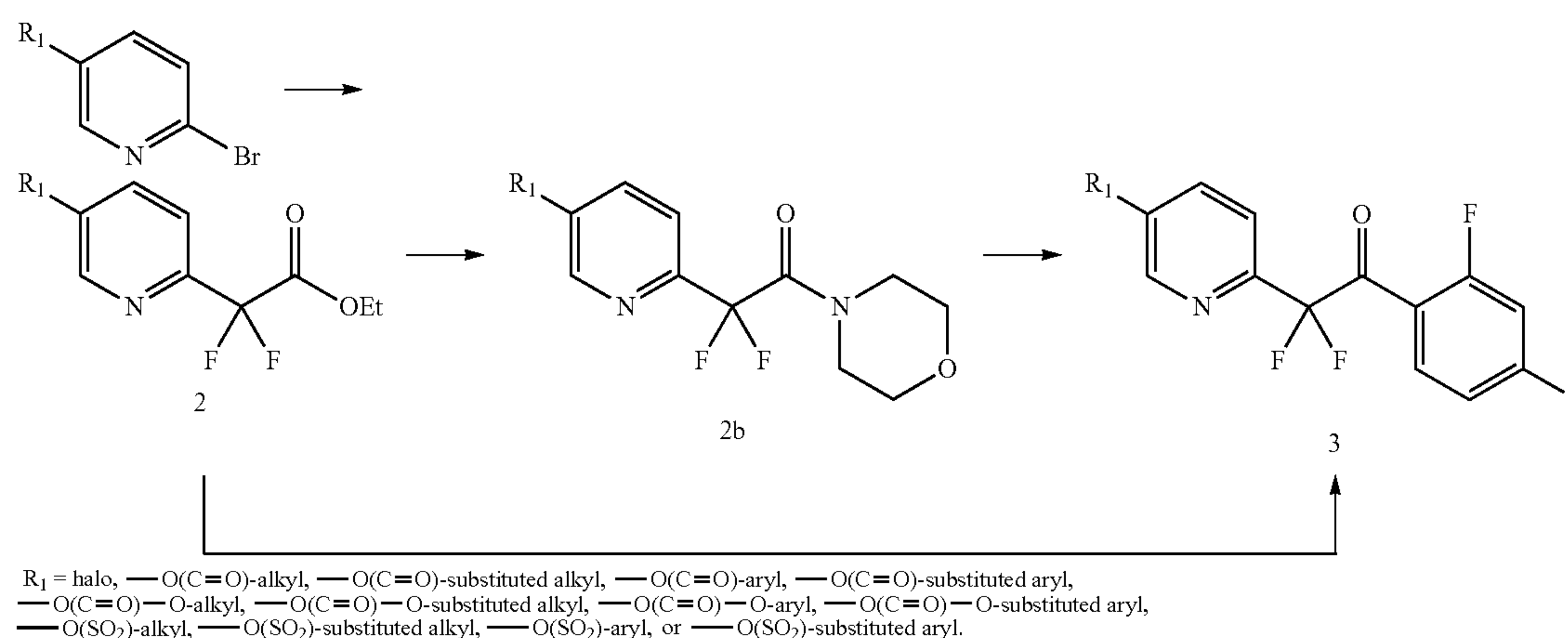
Scheme 2. Synthesis of ketone 3
