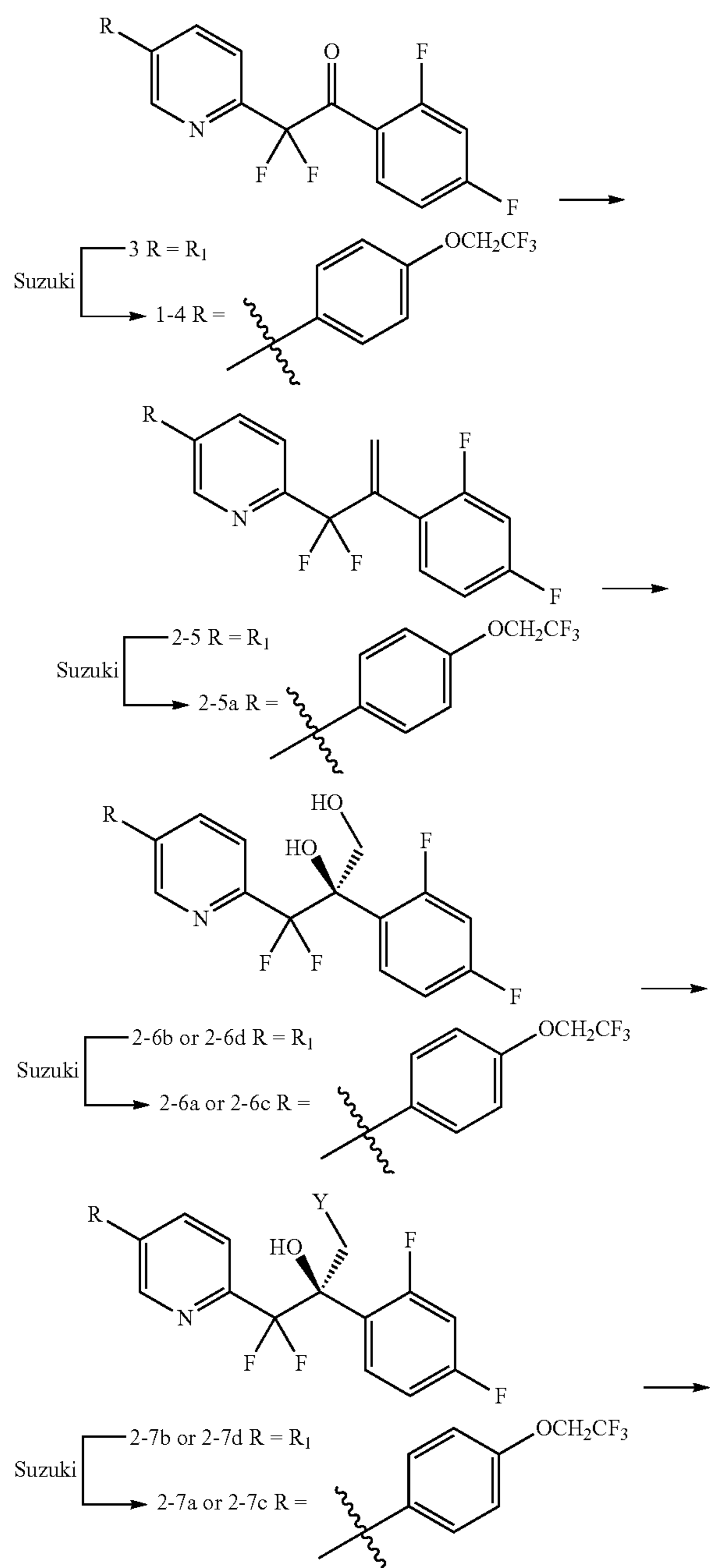
Scheme 3. Synthesis of 1 via Asymmetric Dihydroxylation Method
