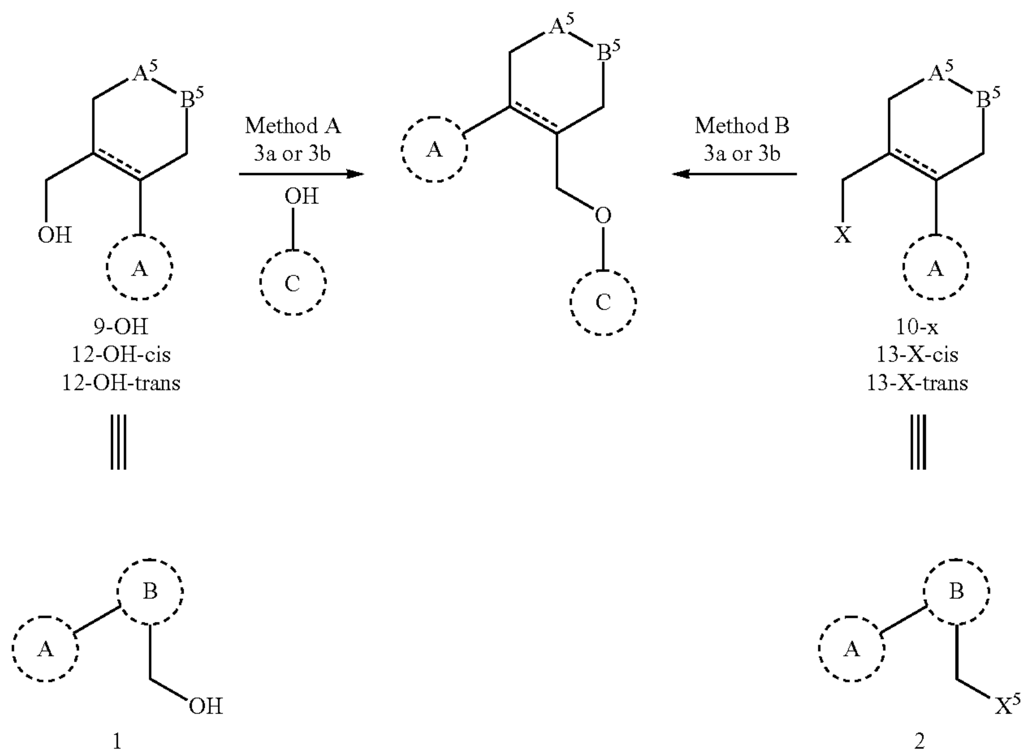
Scheme 3
