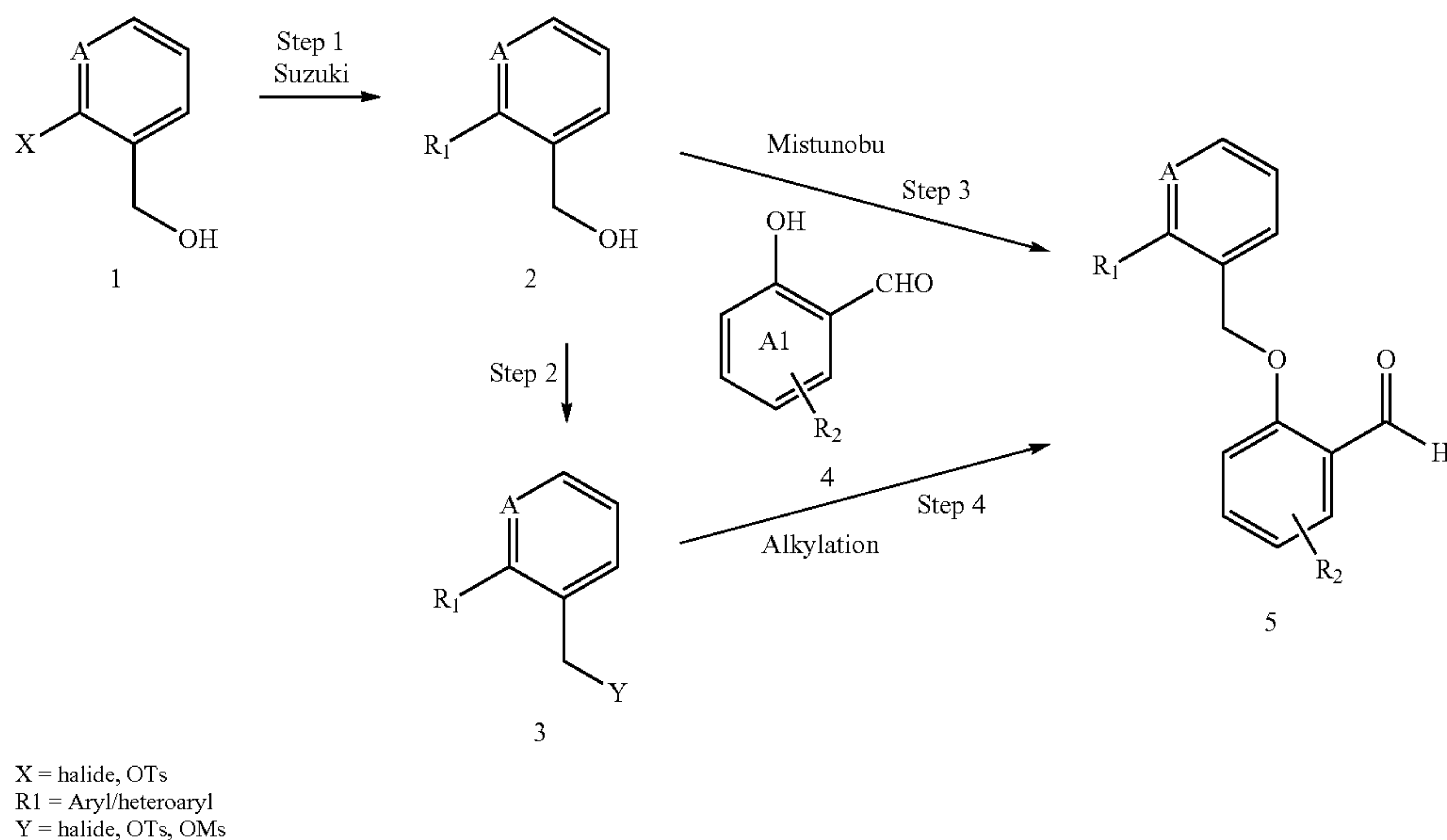
Scheme 9
