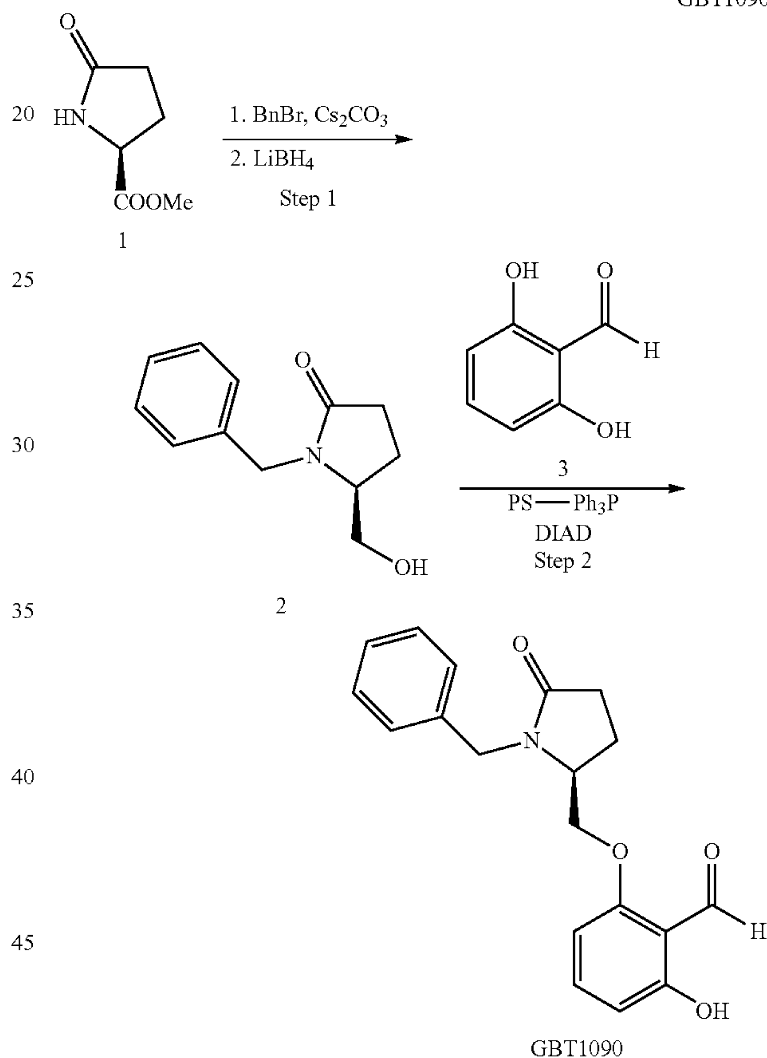
GBT1090—(S)-2-((1-benzyl-5-oxopyrrolidin-2-yl)methoxy)-6-hydroxybenzaldehyde
