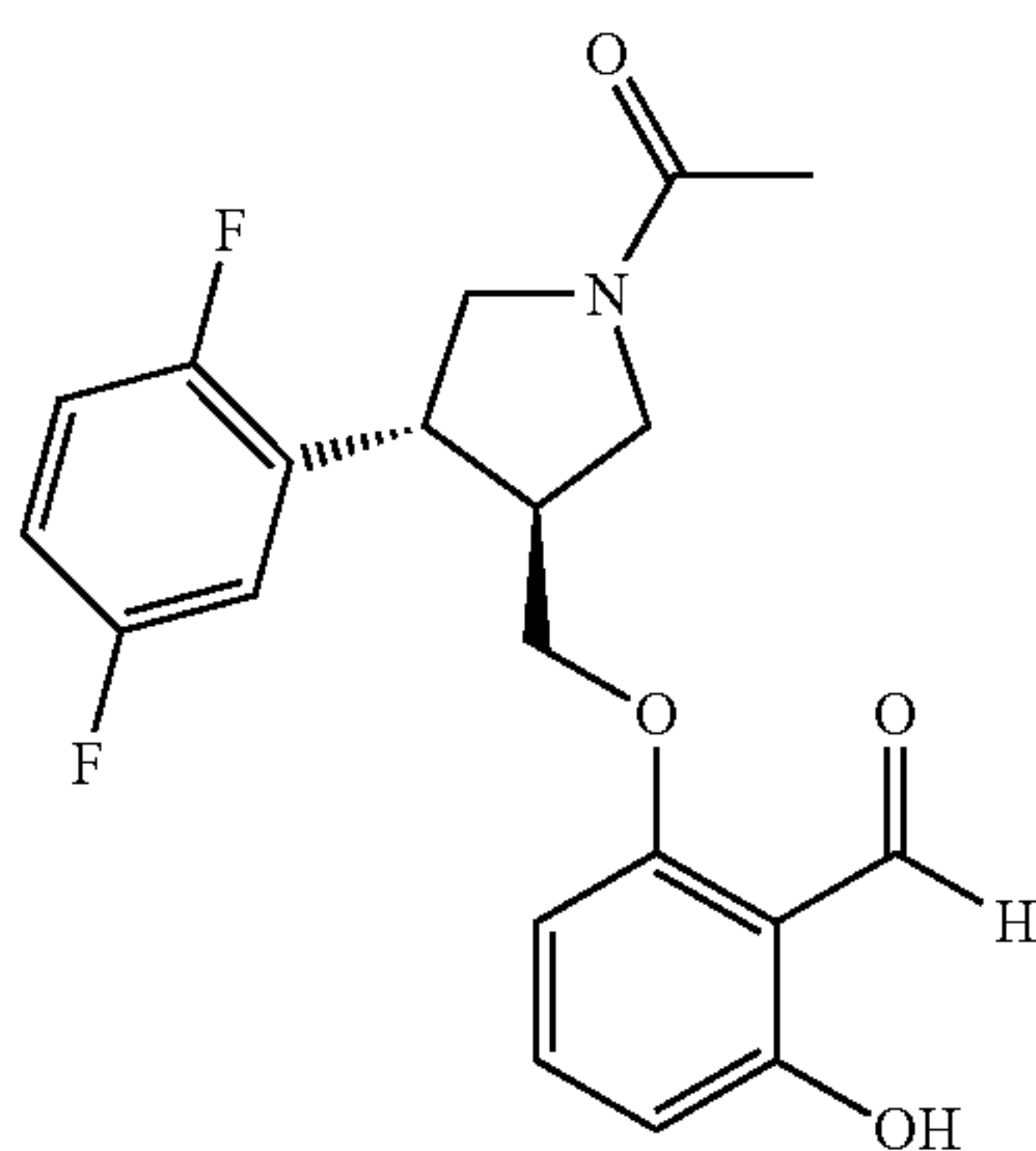
2-(((3S,4R)-1-acetyl-4-(2,5-difluorophenyl)pyrrolidin-3-yl)methoxy)-6-hydroxybenzaldehyde
