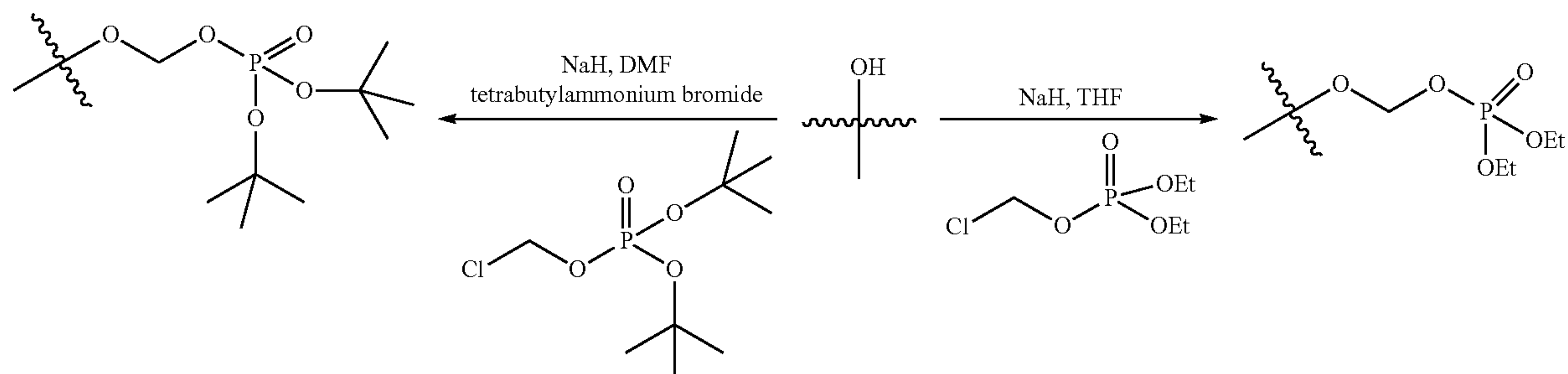
Scheme 6
