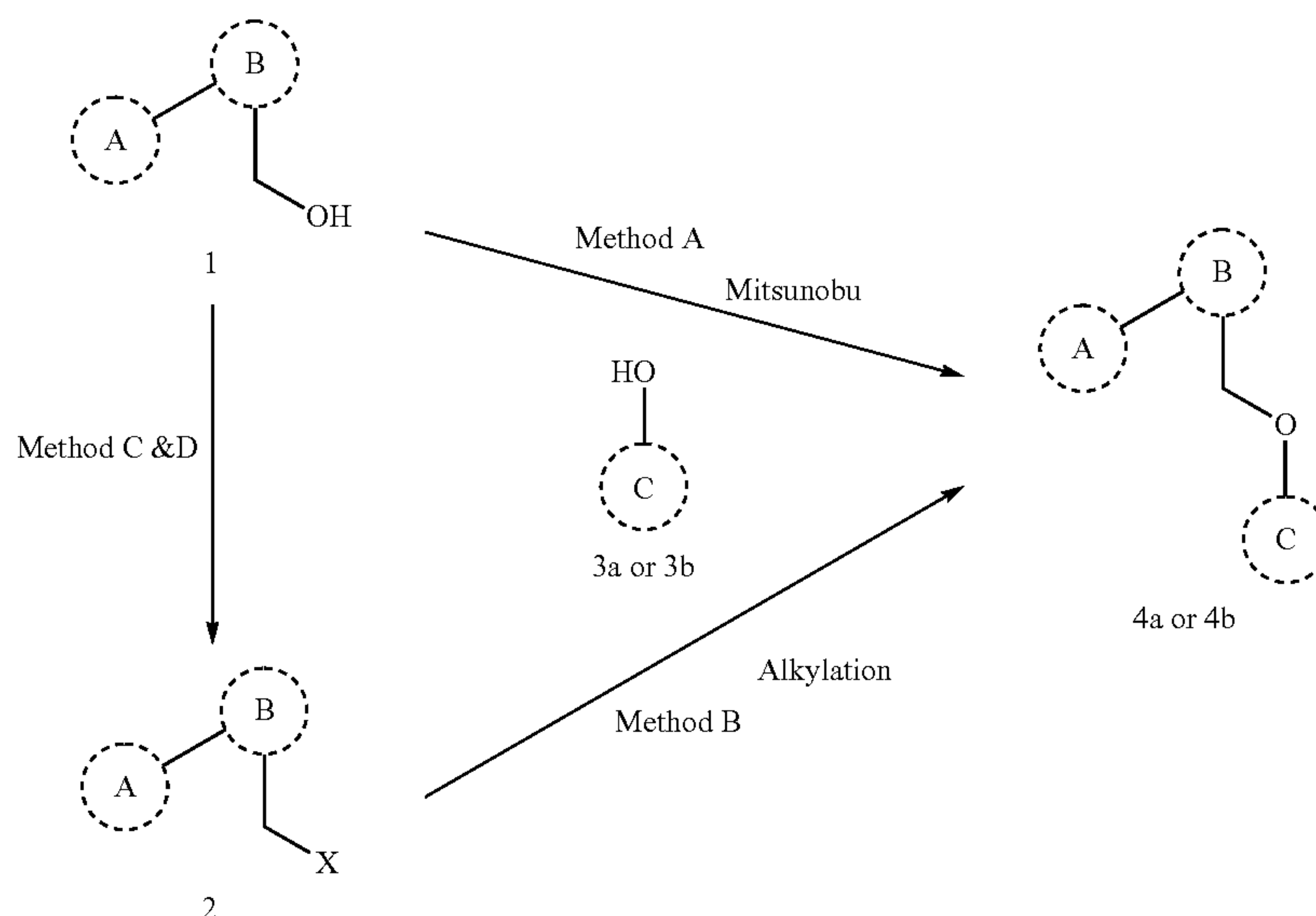
Scheme 1
