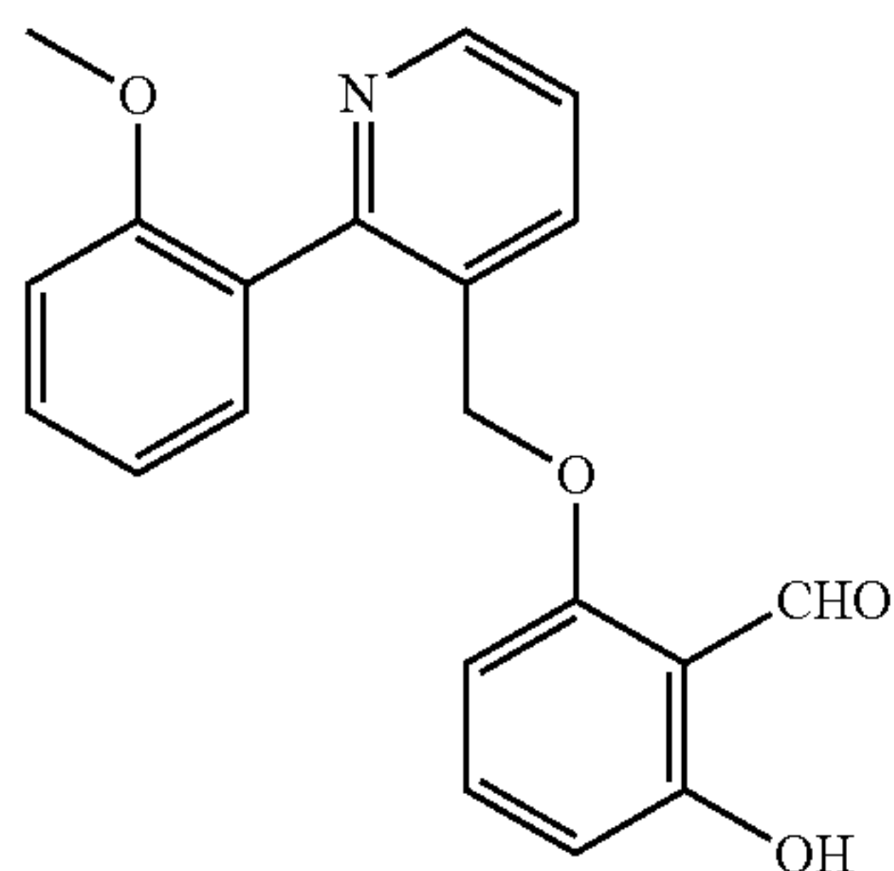
GBT916—2-hydroxy-6-((2-(2-methoxyphenyl)pyridin-3-yl)methoxy)benzaldehyde
