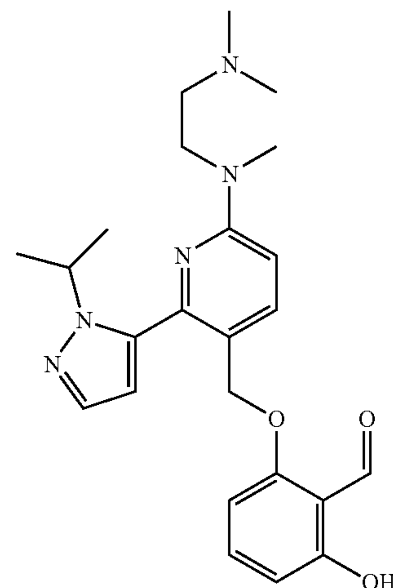
GBT001723—2-((6-((2-(dimethylamino)ethyl)(methyl)amino)-2-(1-isopropyl-1H-pyrazol-5-yl)pyridin-3-yl)methoxy)-6-hydroxybenzaldehyde
