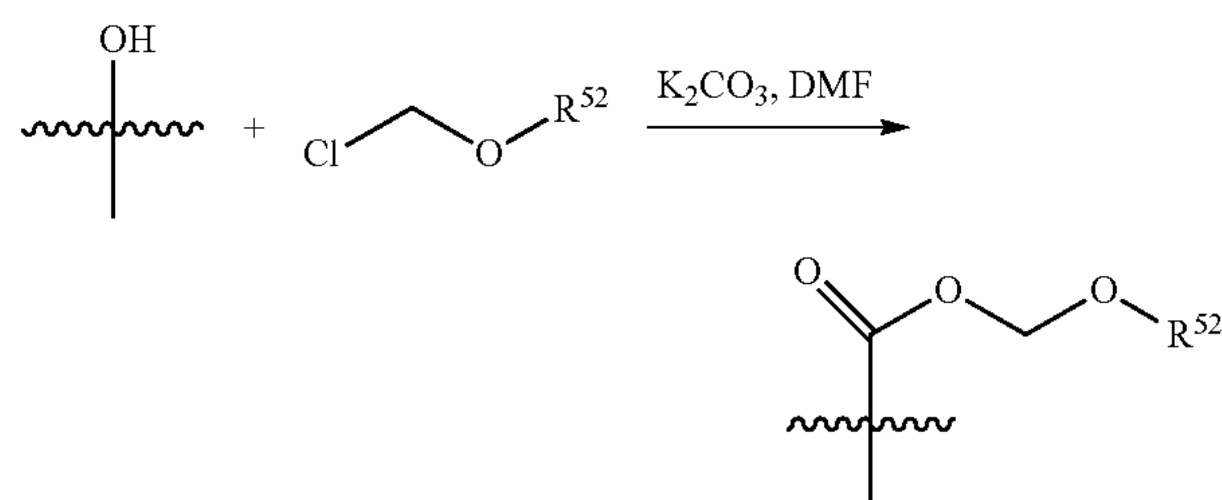
Scheme 7
