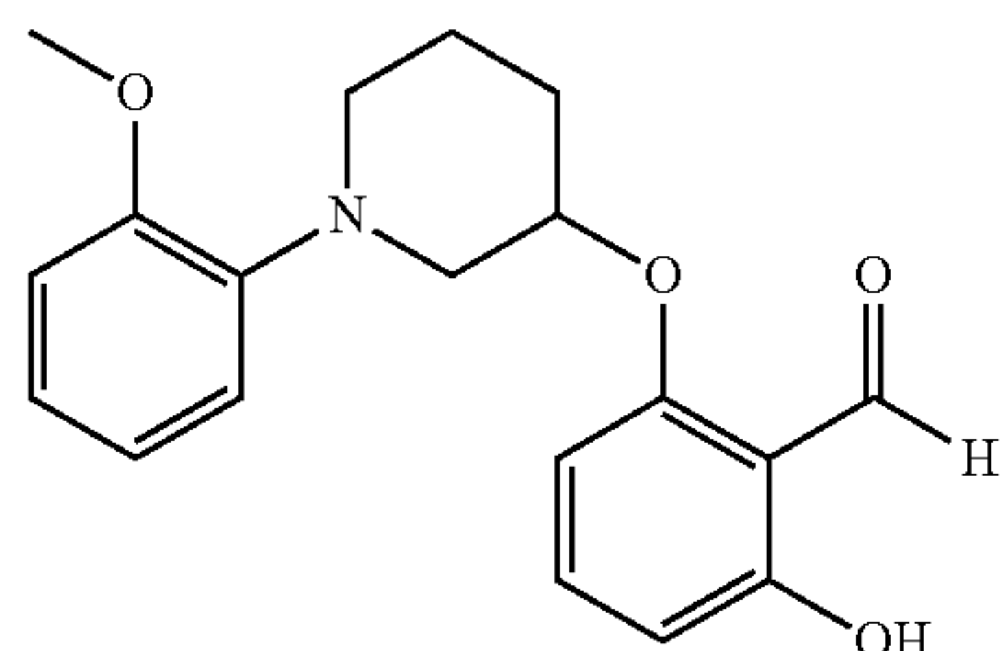
2-hydroxy-6-((1-(2-methoxyphenyl)piperidin-3-yl)oxy)benzaldehyde
