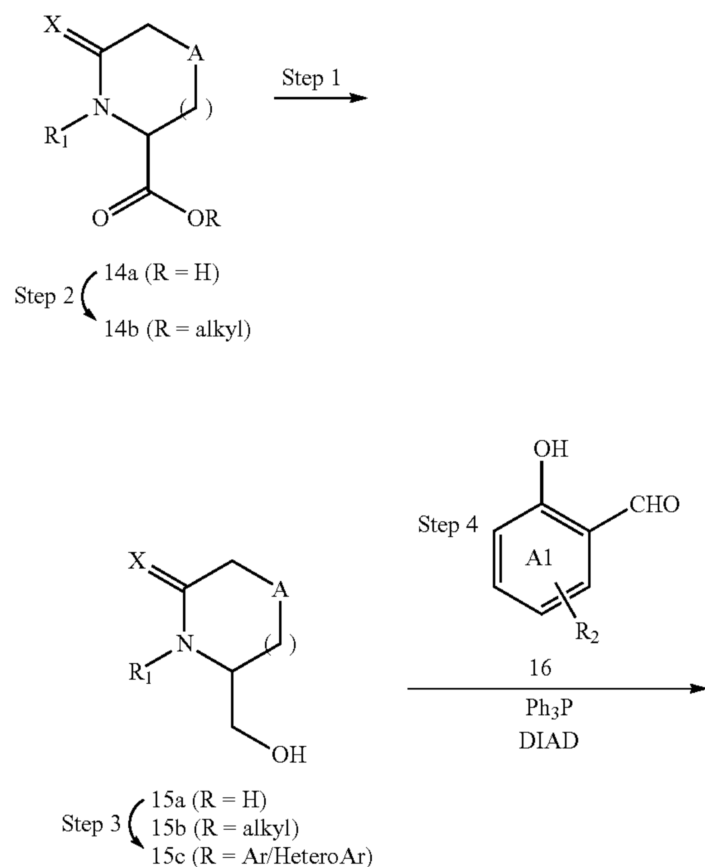
Scheme 8
