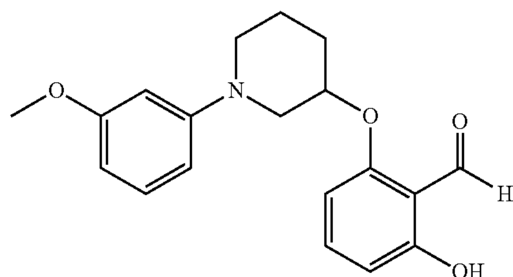
2-hydroxy-6-((1-(3-methoxyphenyl)piperidin-3-yl)oxy)benzaldehyde
