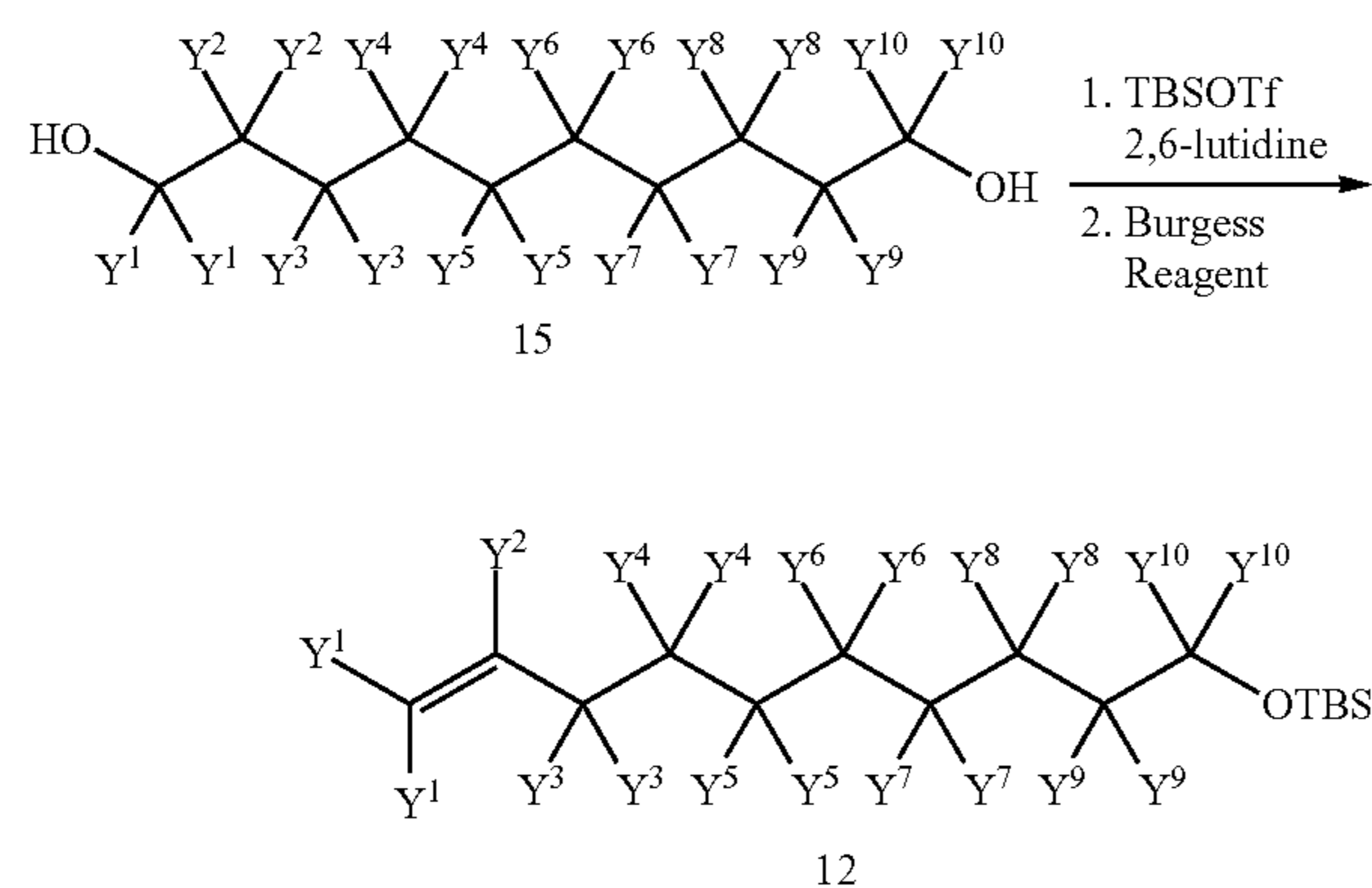
Scheme 2a: A Method for the Preparation of Intermediate 12
