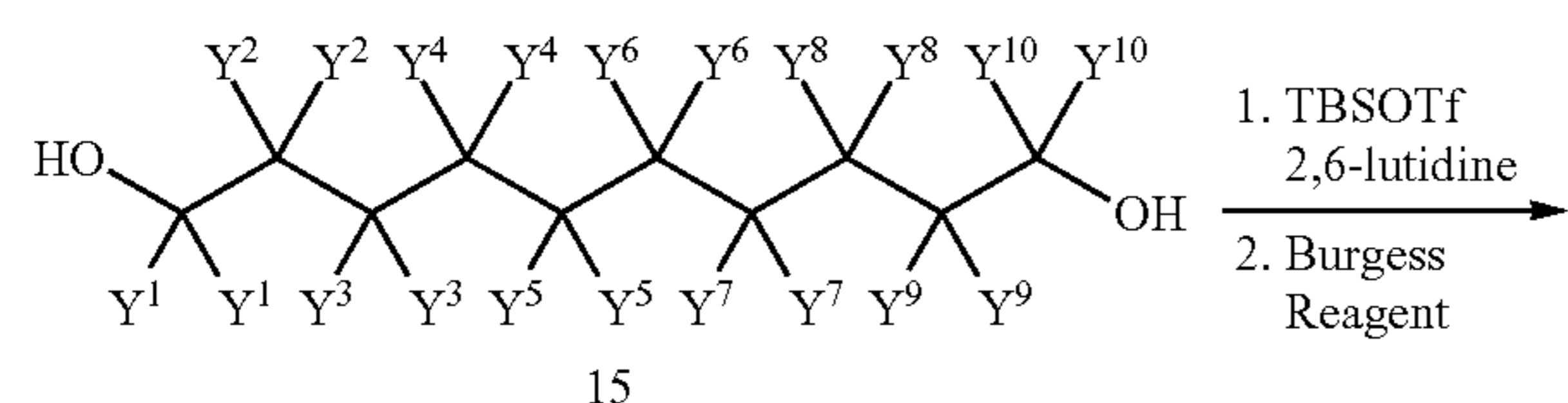
Scheme 2a: A Method for the Preparation of Intermediate 12
