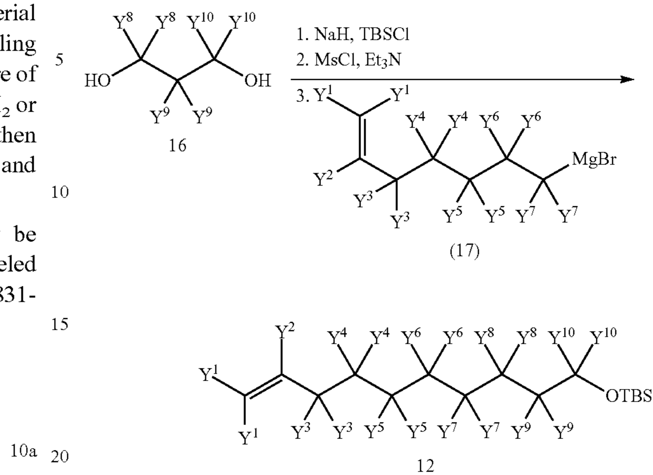
Scheme 2b: Alternate Method for the Preparation of Intermediate 12
