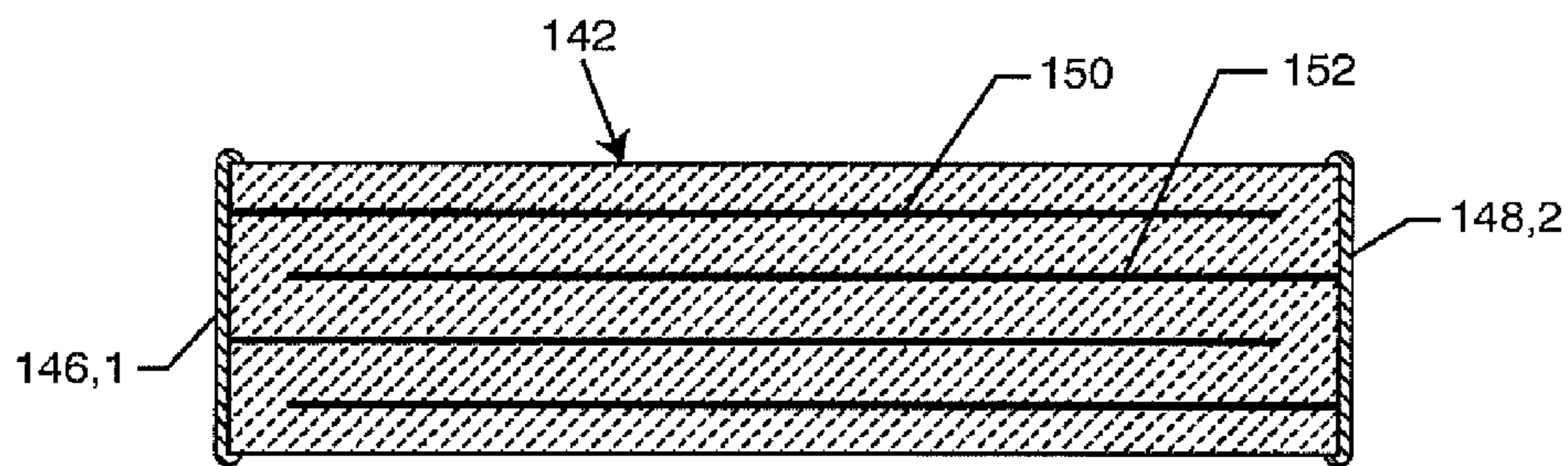
FIG. 14 PRIOR ART
