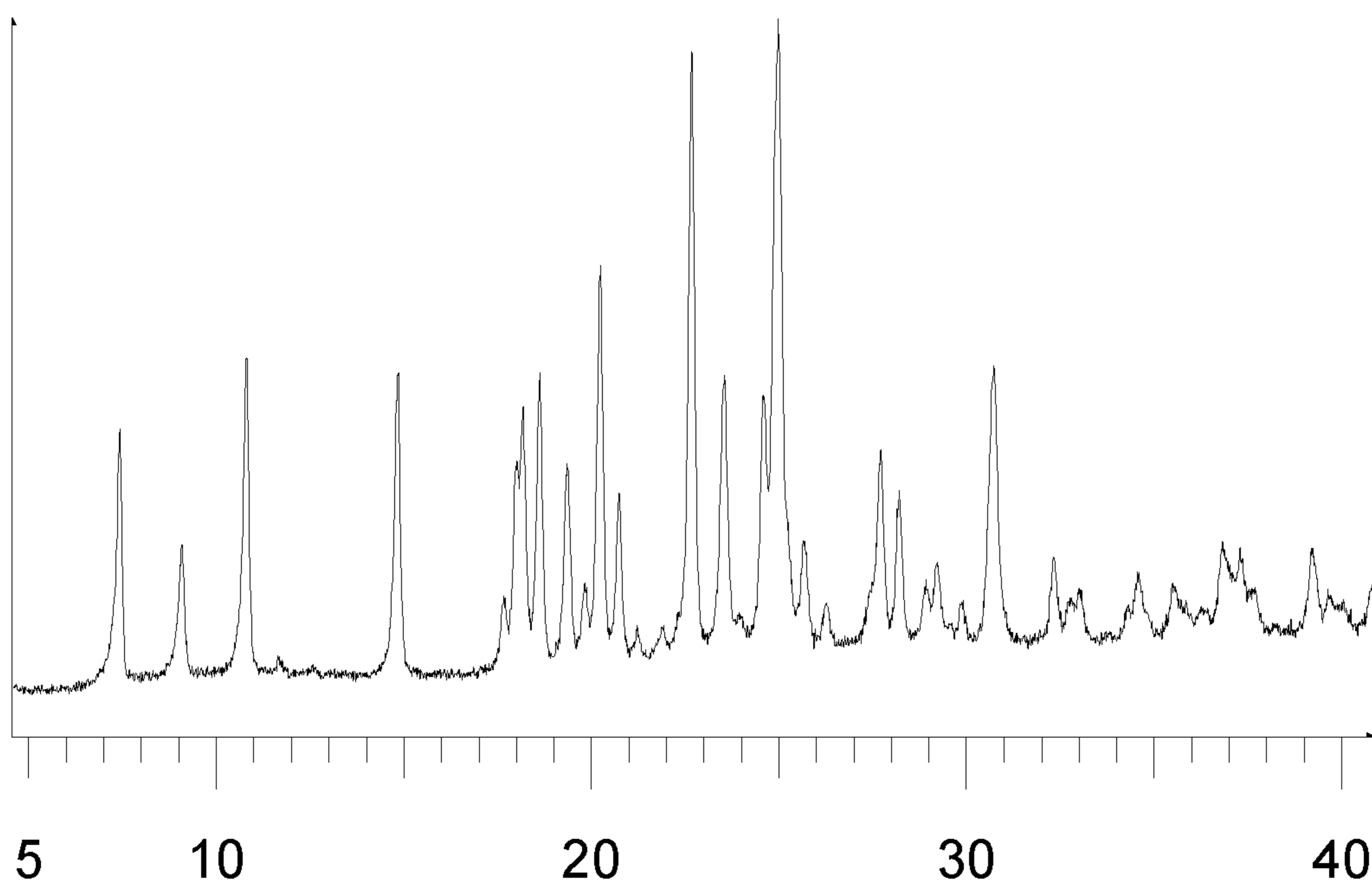
2-Theta - Scale
