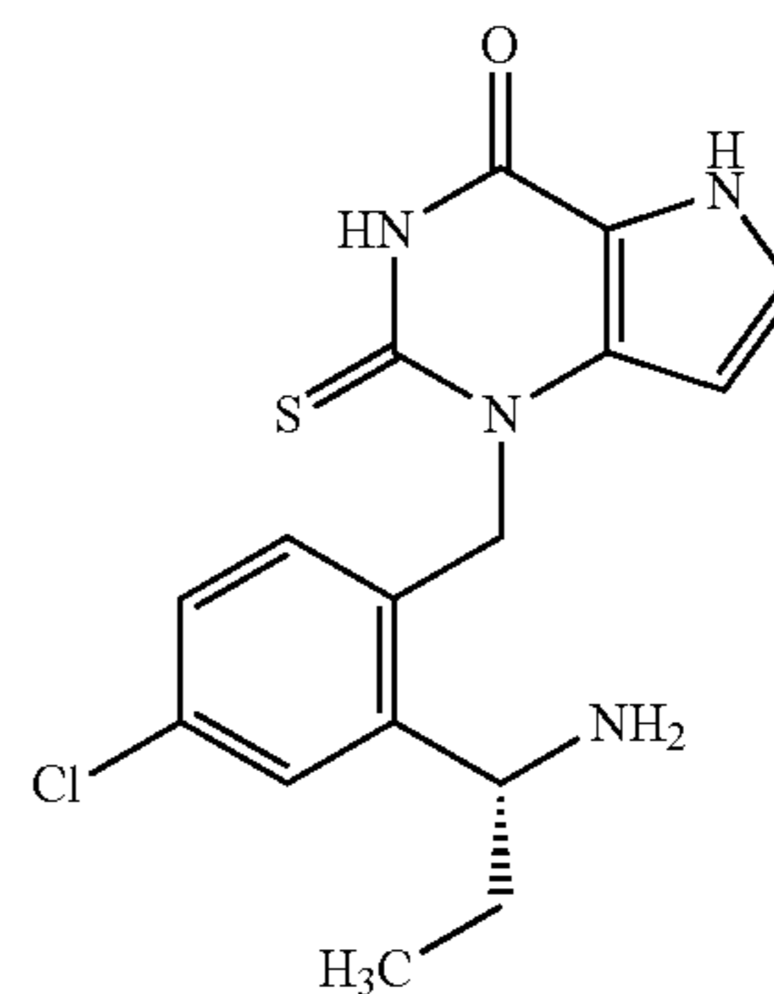
(a) tert-Butyl [(1R)-1-(2-bromo-5-chlorophenyl)propyl]carbamate
