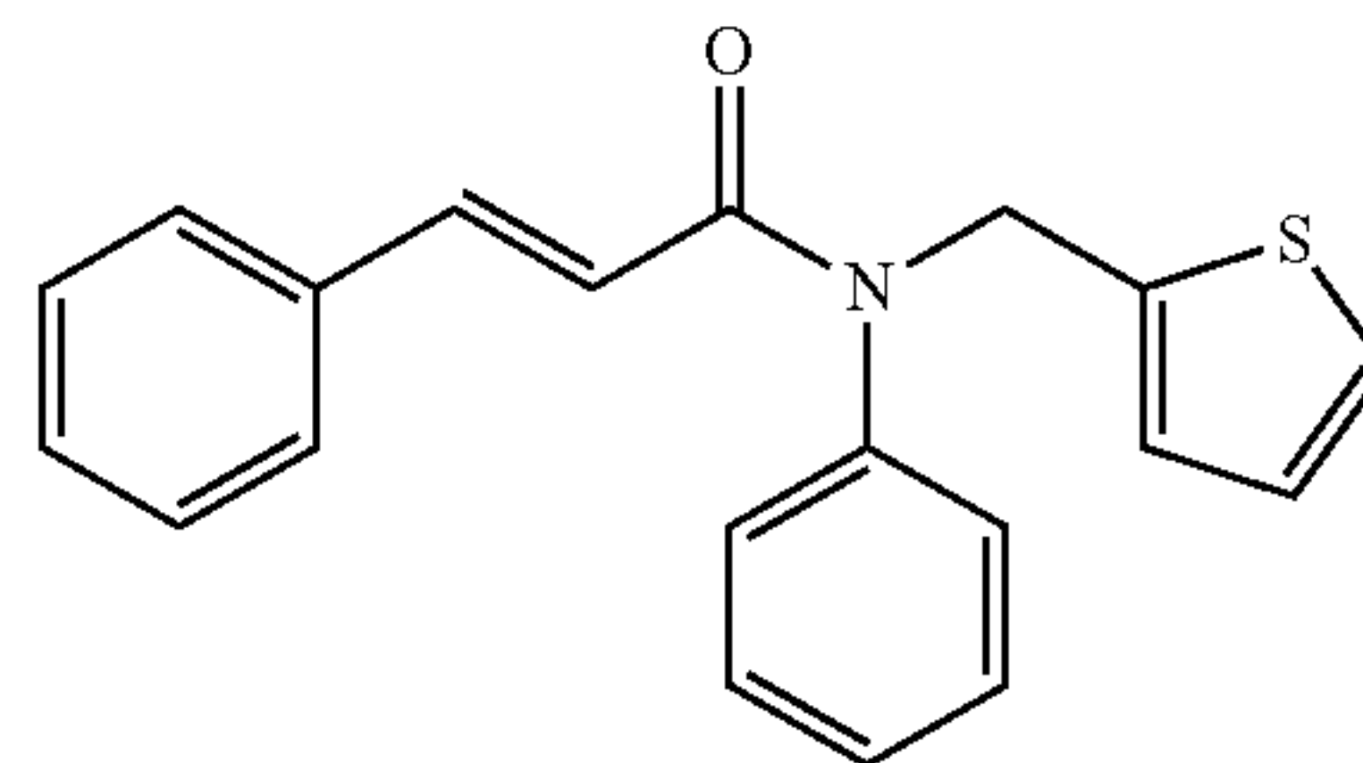
N-phenyl-N-(thiophen-2-ylmethyl)cinnamamide; Example 238
