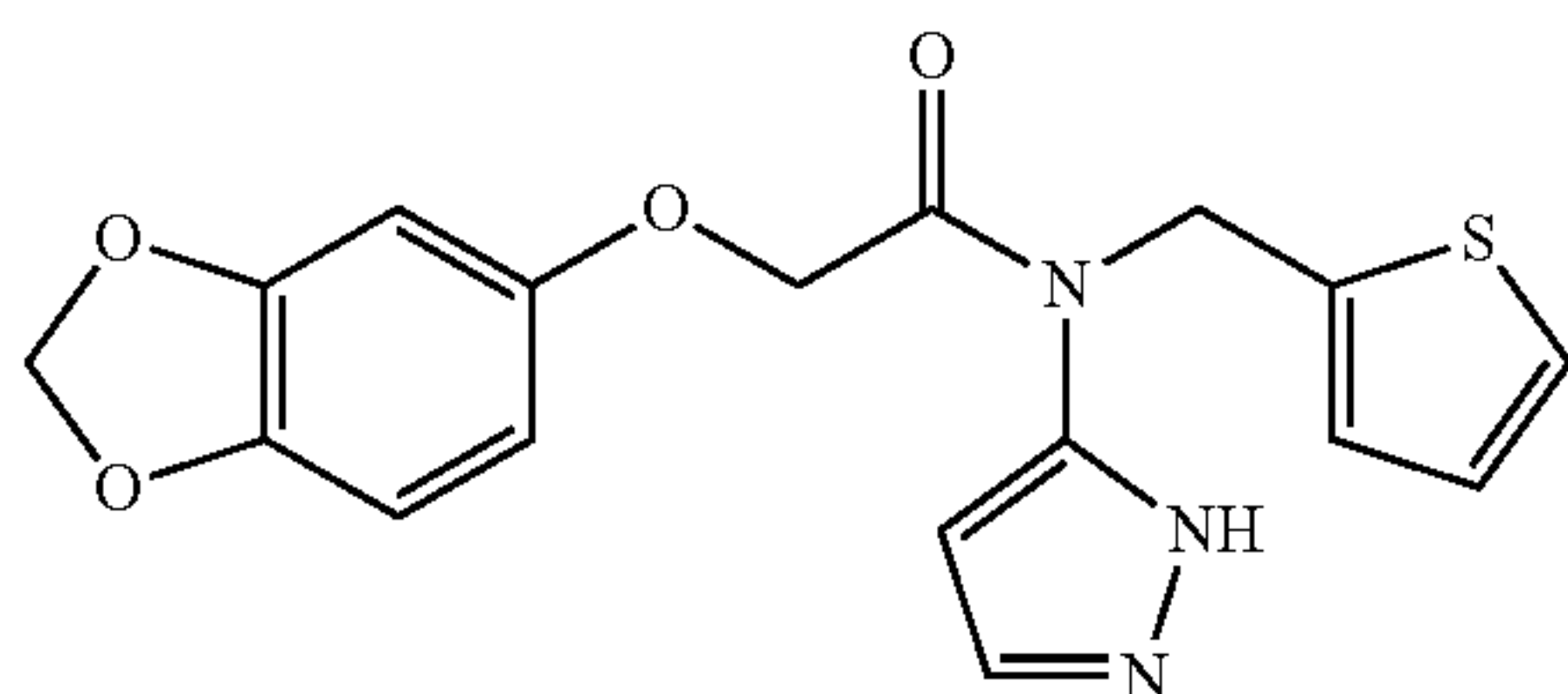
2-(benzo[d][1,3]dioxol-5-yloxy)-N-(1H-pyrazol-5-yl)-N-(thiophen-2-ylmethyl)acetamide; Example 12
