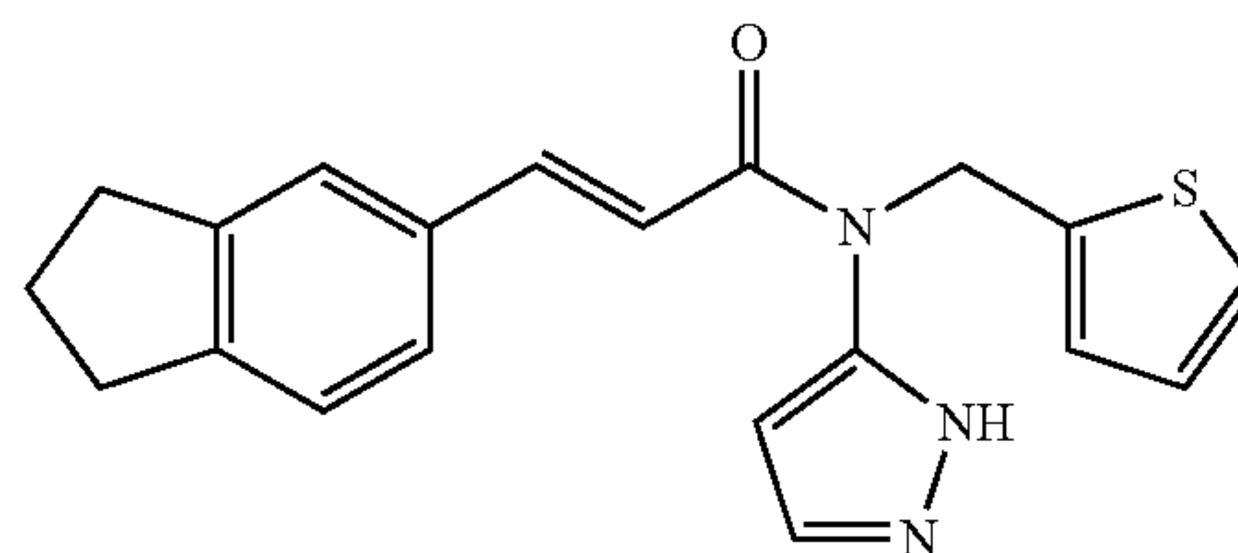
(E)-3-(2,3-dihydro-1H-inden-5-yl)-N-(1H-pyrazol-5-yl)-N-(thiophen-2-ylmethyl)acrylamide; Example 200
