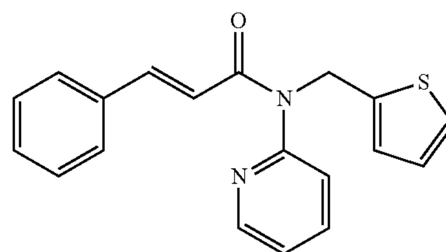
N-(pyridin-2-yl)-N-(thiophen-2-ylmethyl)cinnamamide; Example 239
