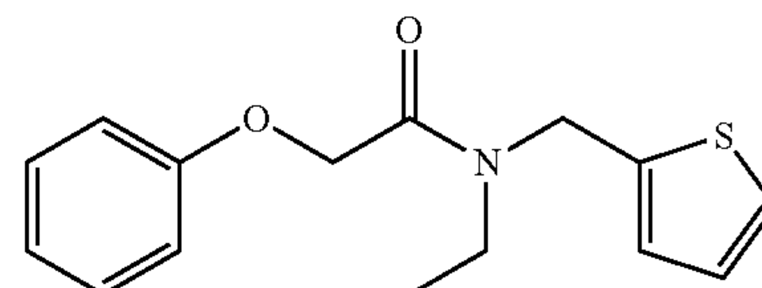
N-ethyl-2-phenoxy-N-(thiophen-2-ylmethyl)acetamide; Example 105
