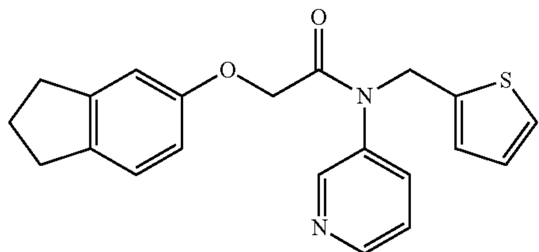
2-(2,3-dihydro-1H-inden-5-yloxy)-N-(pyridin-3-yl)-N-(thiophen-2-ylmethyl)acetamide; Example 34
