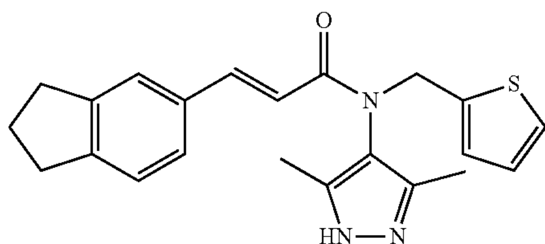
(E)-3-(2,3-dihydro-1H-inden-5-yl)-N-(3,5-dimethyl-1H-pyrazol-4-yl)-N-(thiophen-2-ylmethyl)acrylamide; Example 192
