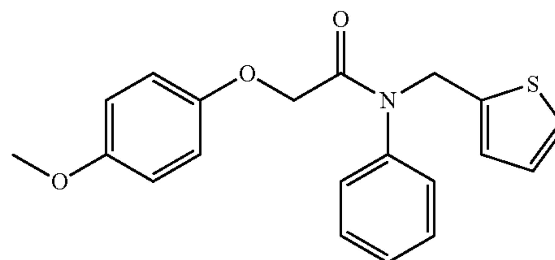
2-(4-methoxyphenoxy)-N-phenyl-N-(thiophen-2-ylmethyl)acetamide; Example 33
