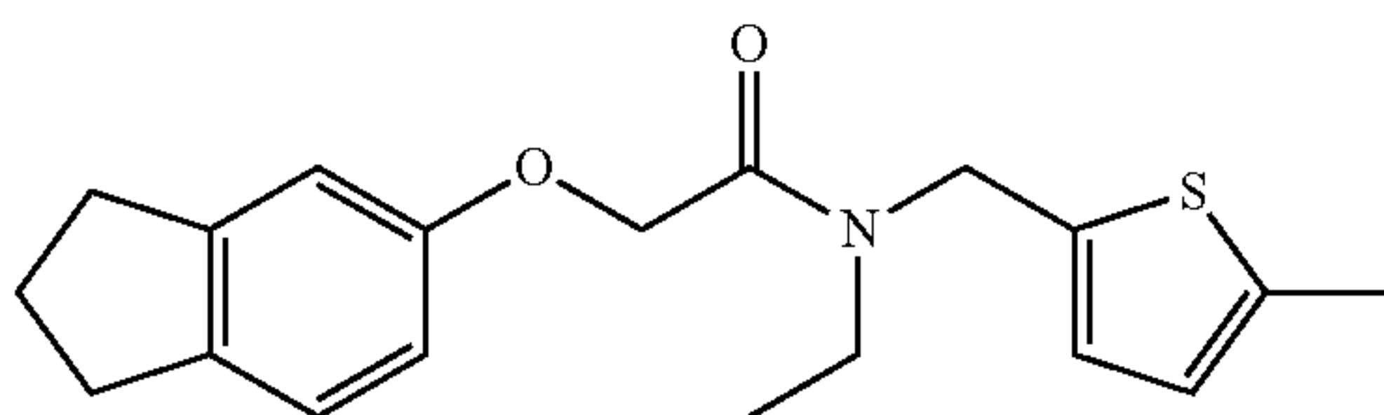
2-(2,3-dihydro-1H-inden-5-yloxy)-N-ethyl-N-((5-methylthiophen-2-yl)methyl)acetamide; Example 236
