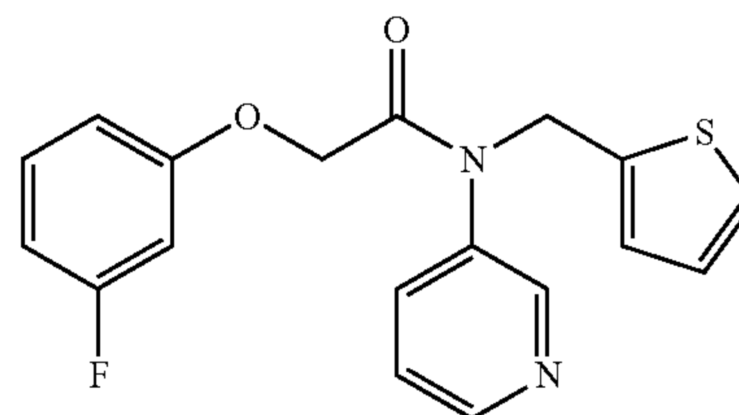
2-(3-fluorophenoxy)-N-(pyridin-3-yl)-N-(thiophen-2-ylmethyl)acetamide; Example 142
