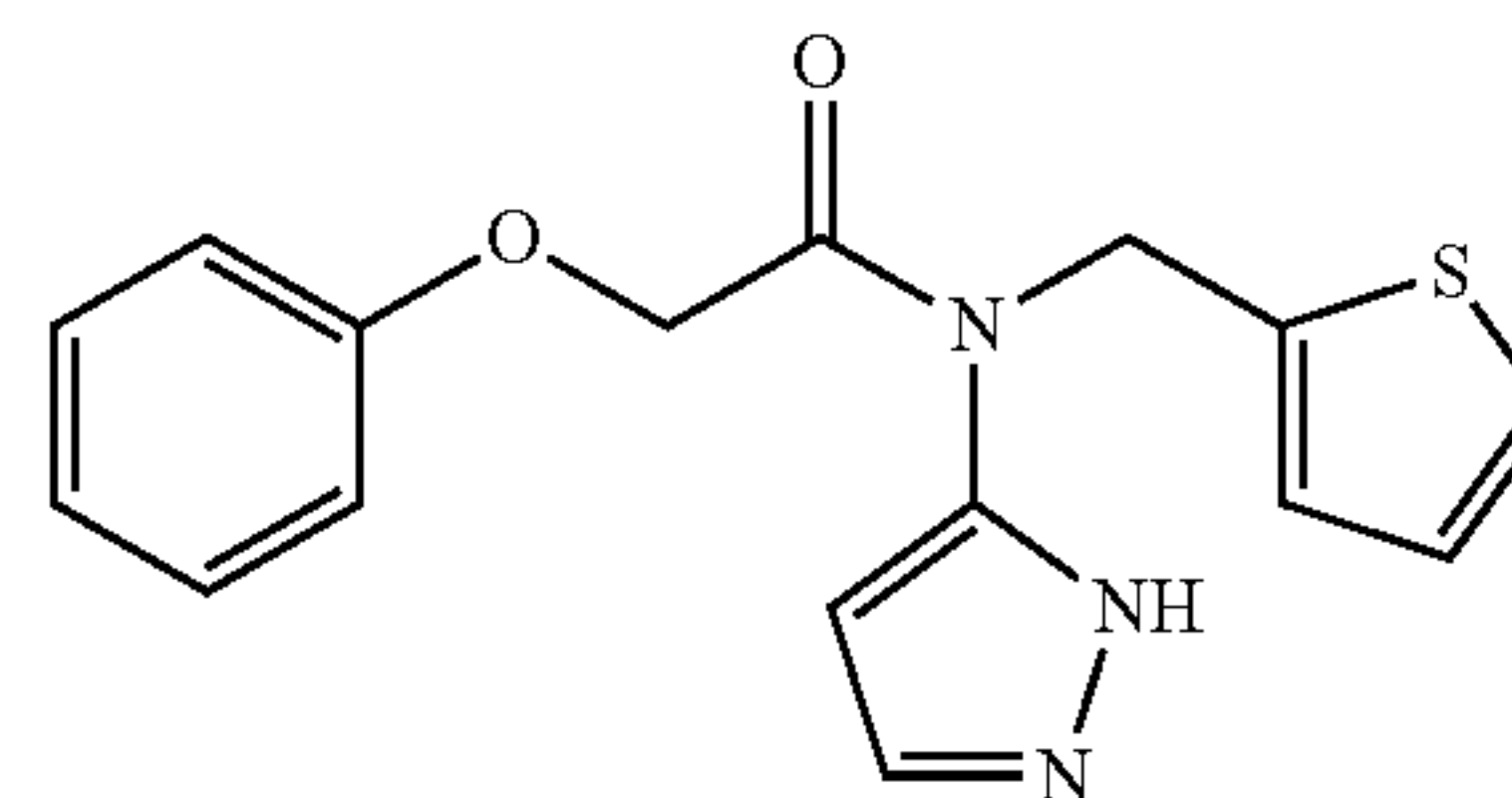
2-phenoxy-N-(1H-pyrazol-5-yl)-N-(thiophen-2-ylmethyl)acetamide; Example 199
