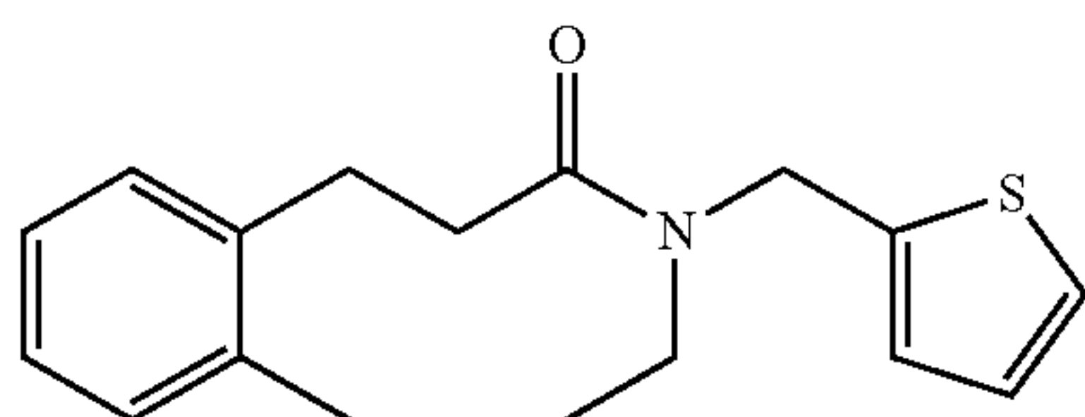
N-ethyl-N-(thiophen-2-ylmethyl)-3-o-tolylpropanamide; Example 77
