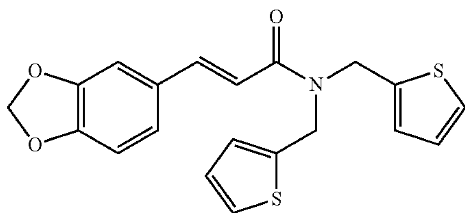
(E)-3-(benzo[d][1,3]dioxol-5-yl)-N,N-bis(thiophen-2-ylmethyl)acrylamide; Example 255
