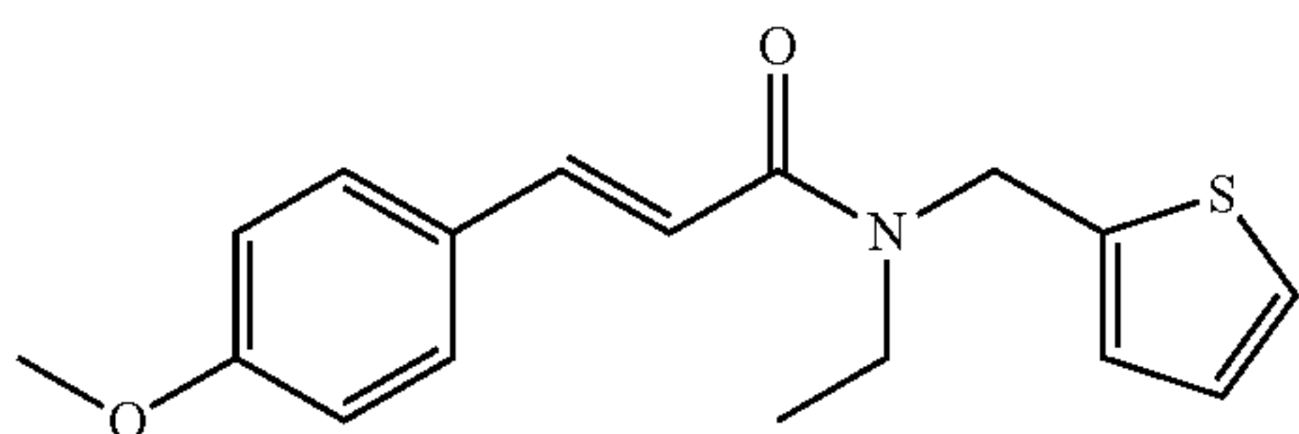
(E)-N-ethyl-3-(4-methoxyphenyl)-N-(thiophen-2-ylmethyl)acrylamide; Example 188
