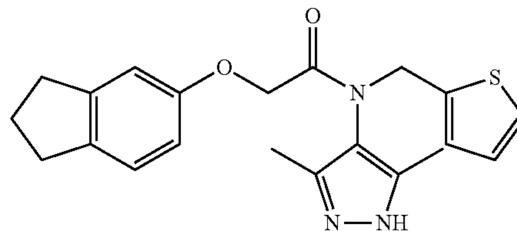
2-(2,3-dihydro-1H-inden-5-yloxy)-N-(3,5-dimethyl-1H-pyrazol-4-yl)-N-(thiophen-2-ylmethyl)acetamide; Example 7
