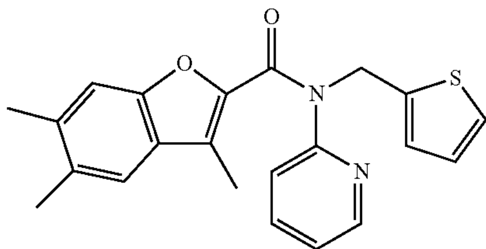
3,5,6-trimethyl-N-(pyridin-2-yl)-N-(thiophen-2-ylmethyl)benzofuran-2-carboxamide; Example 144
