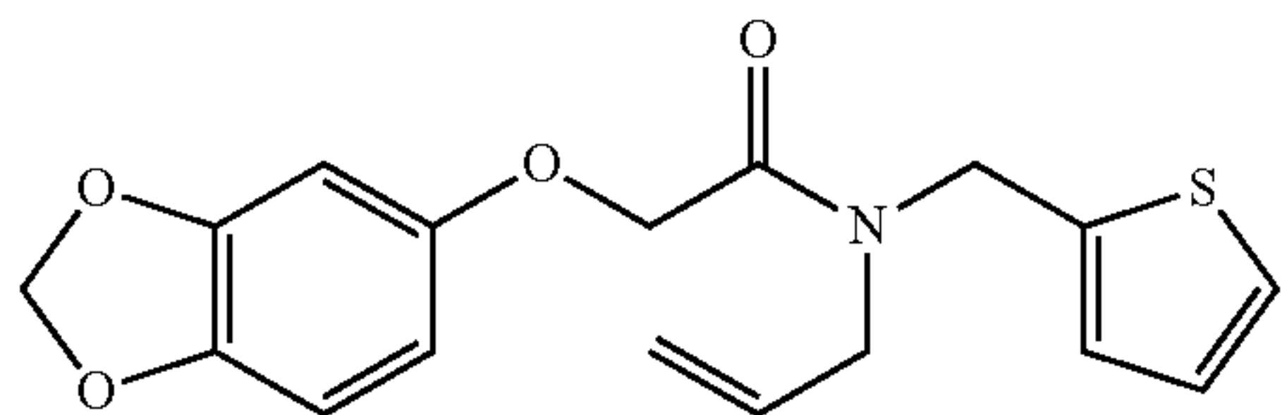
N-allyl-2-(benzo[d][1,3]dioxol-5-yloxy)-N-(thiophen-2-ylmethyl)acetamide; Example 30
