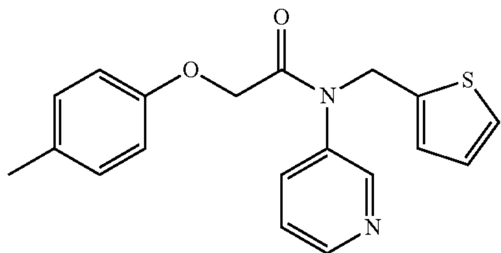
N-(pyridin-3-yl)-N-(thiophen-2-ylmethyl)-2-(p-toloxo)acetamide; Example 51
