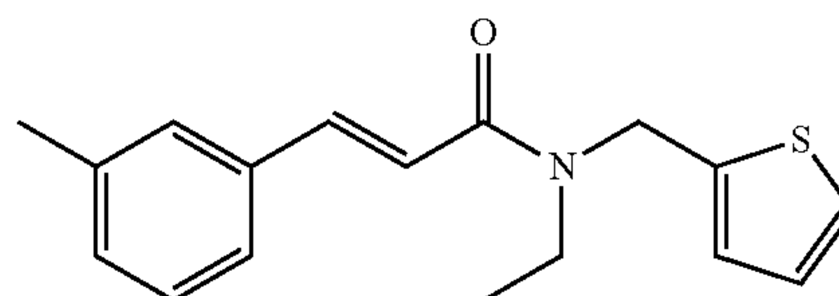
(E)-N-ethyl-N-(thiophen-2-ylmethyl)-3-m-tolylacrylamide; Example 219
