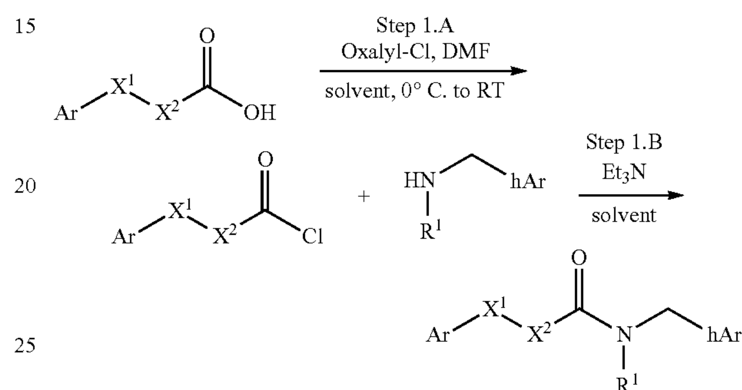
Scheme 1
