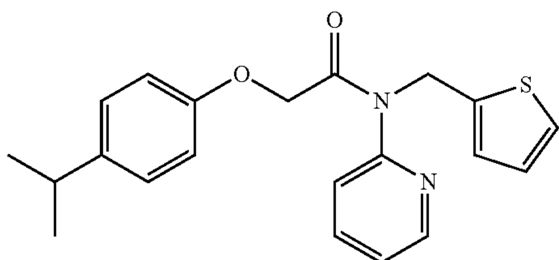
2-(4-isopropylphenoxy)-N-(pyridin-2-yl)-N-(thiophen-2-ylmethyl)acetamide; Example 123
