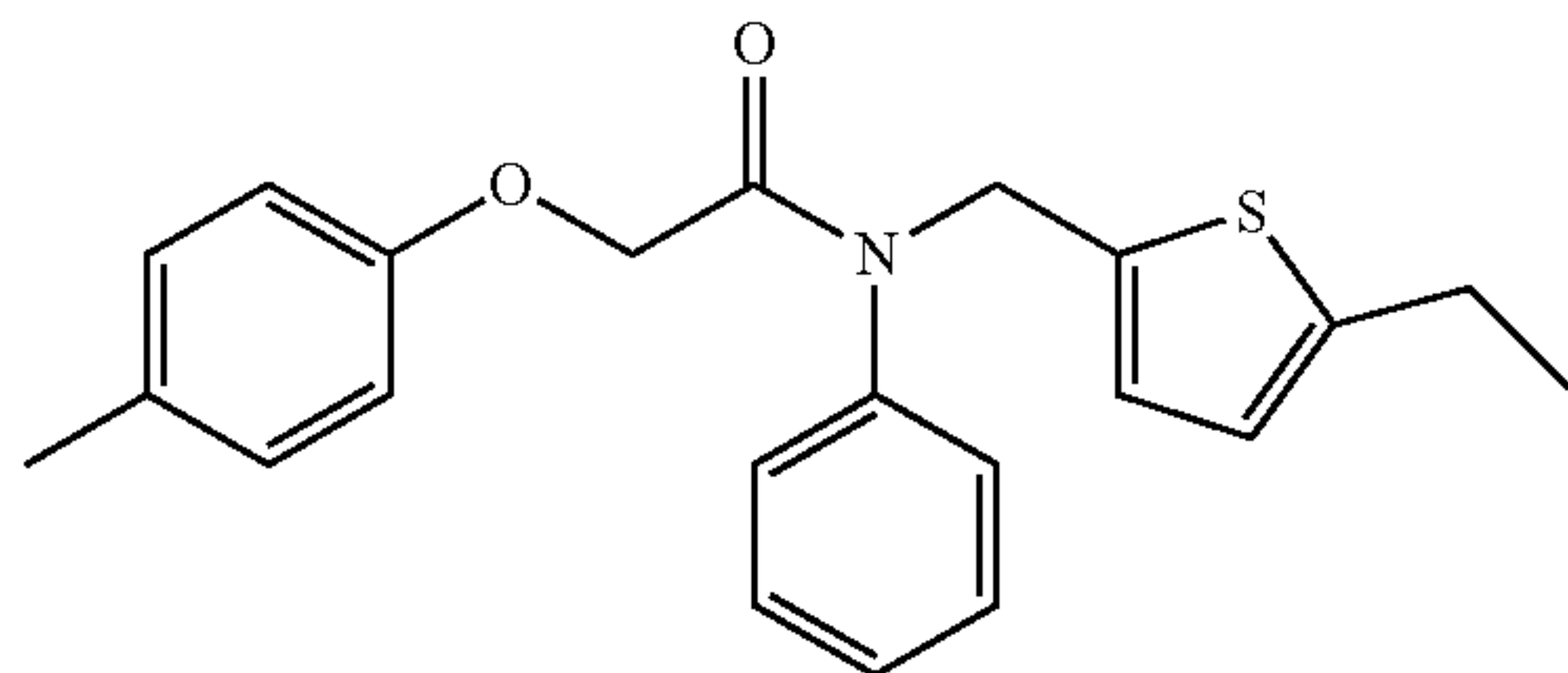
N-((5-ethylthiophen-2-yl)methyl)-N-phenyl-2-(p-tolyloxy)acetamide; Example 151
