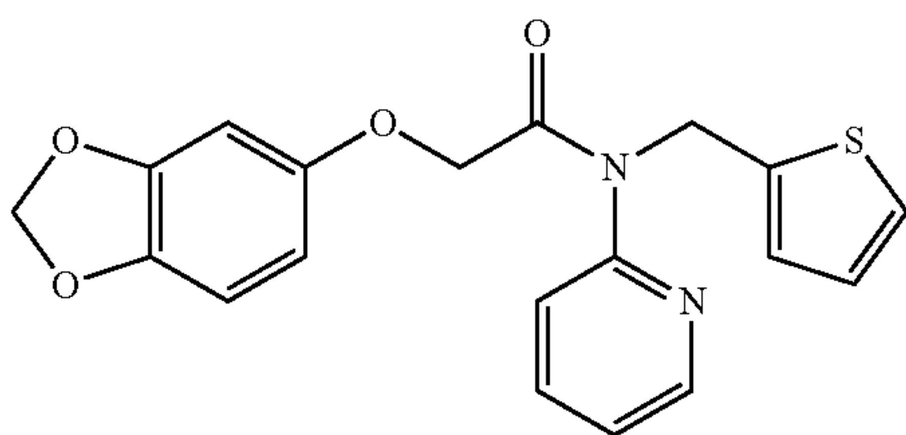
2-(benzo[d][1,3]dioxol-5-yloxy)-N-(pyridin-2-yl)-N-(thiophen-2-ylmethyl)acetamide; Example 67
