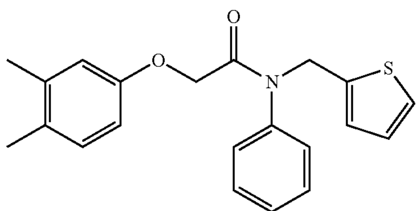
2-(3,4-dimethylphenoxy)-N-phenyl-N-(thiophen-2-ylmethyl)acetamide; Example 65
