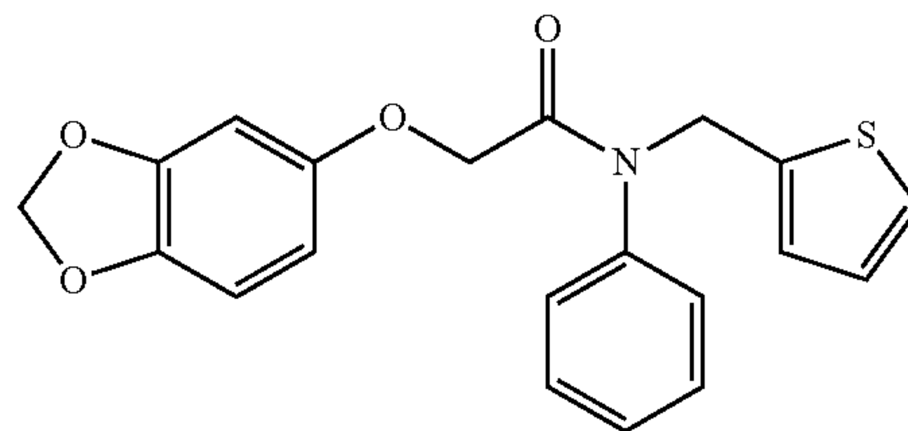
2-(benzo[d][1,3]dioxol-5-yloxy)-N-phenyl-N-(thiophen-2-ylmethyl)acetamide; Example 5
