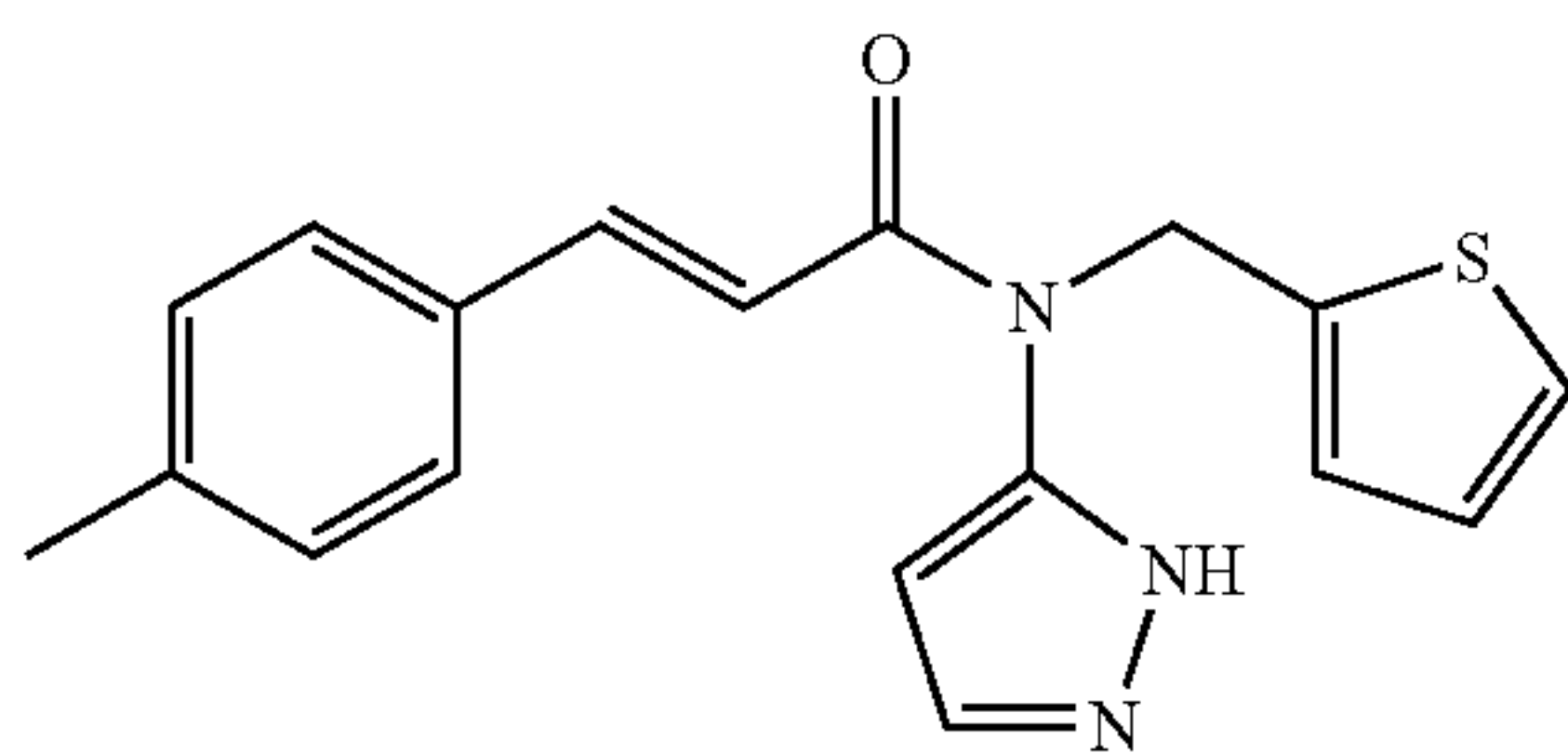
(E)-N-(1H-pyrazol-5-yl)-N-(thiophen-2-ylmethyl)-3-p-tolylacrylamide; Example 173
