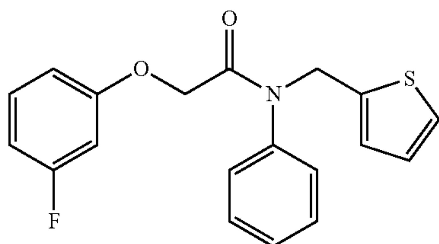
2-(3-fluorophenoxy)-N-phenyl-N-(thiophen-2-ylmethyl)acetamide; Example 53
