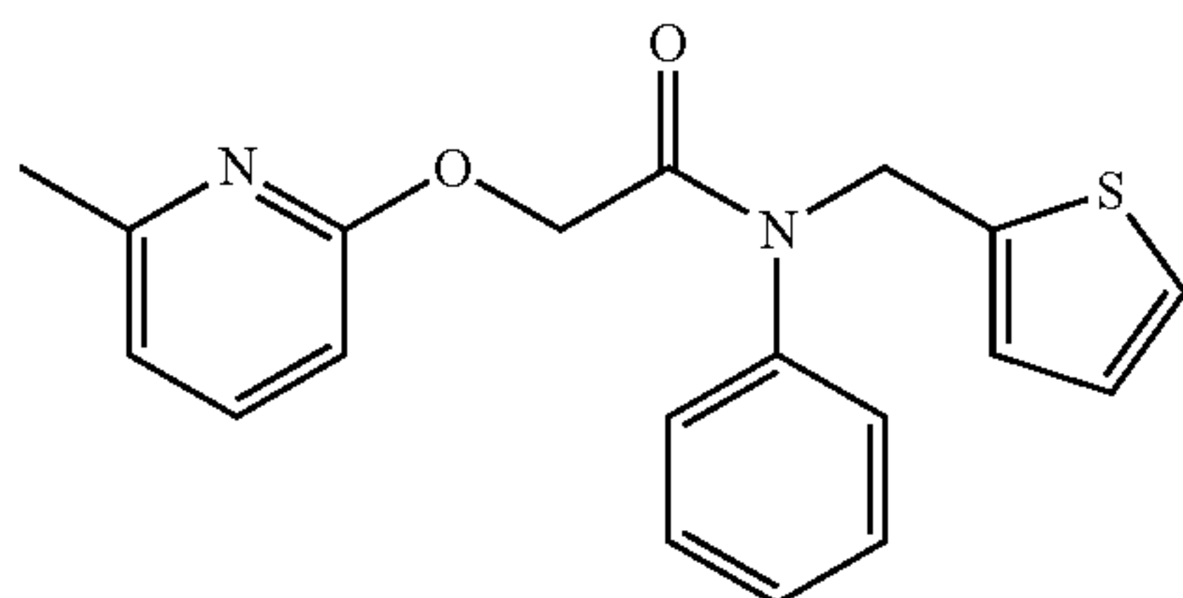
2-(6-methylpyridin-2-yloxy)-N-phenyl-N-(thiophen-2-ylmethyl)acetamide; Example 83
