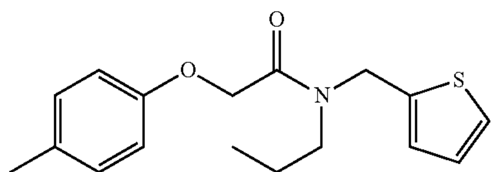
N-propyl-N-(thiophen-2-ylmethyl)-2-(p-tolyloxy)acetamide; Example 28
