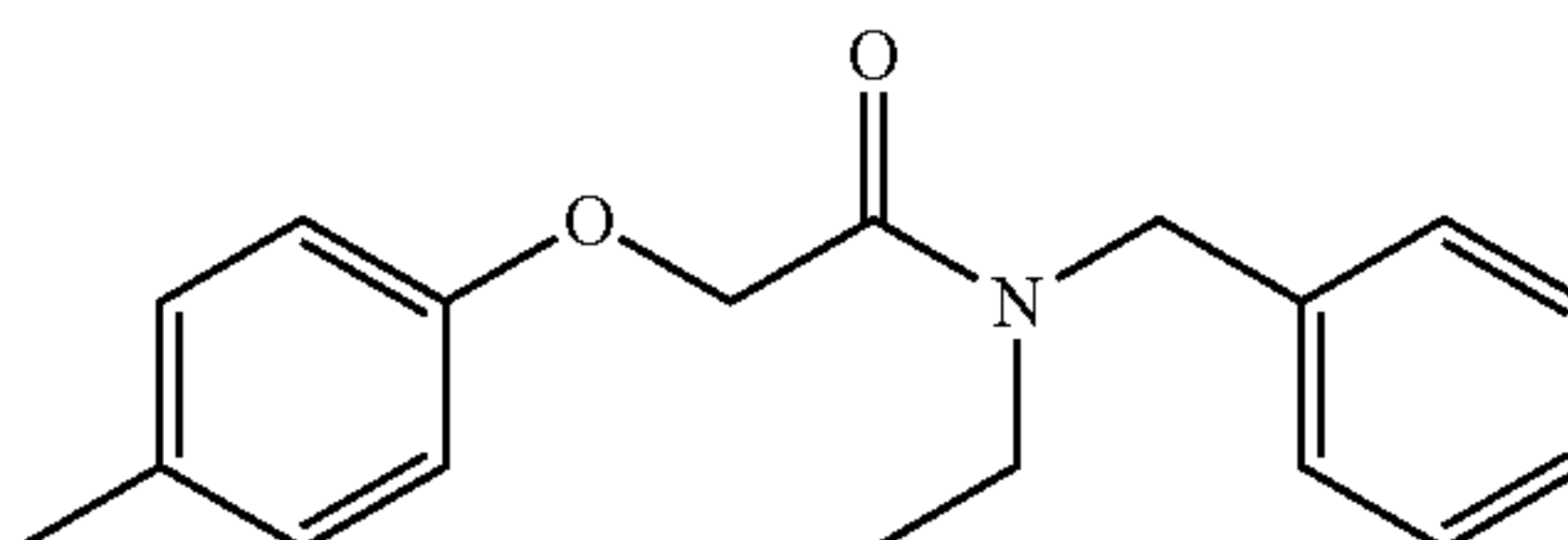
N-benzyl-N-ethyl-2-(p-tolyloxy)acetamide; Example 127
