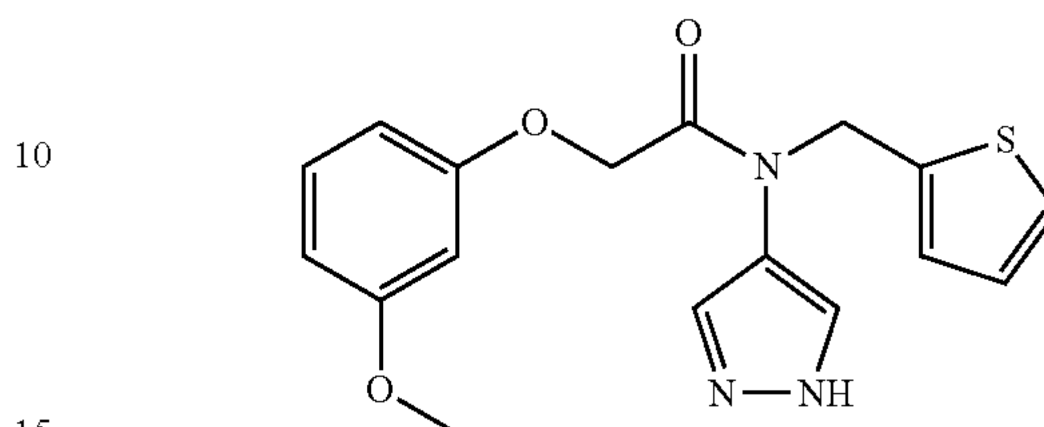
2-(3-methoxyphenoxy)-N-(1H-pyrazol-4-yl)-N-(thiophen-2-ylmethyl)acetamide; Example 35
