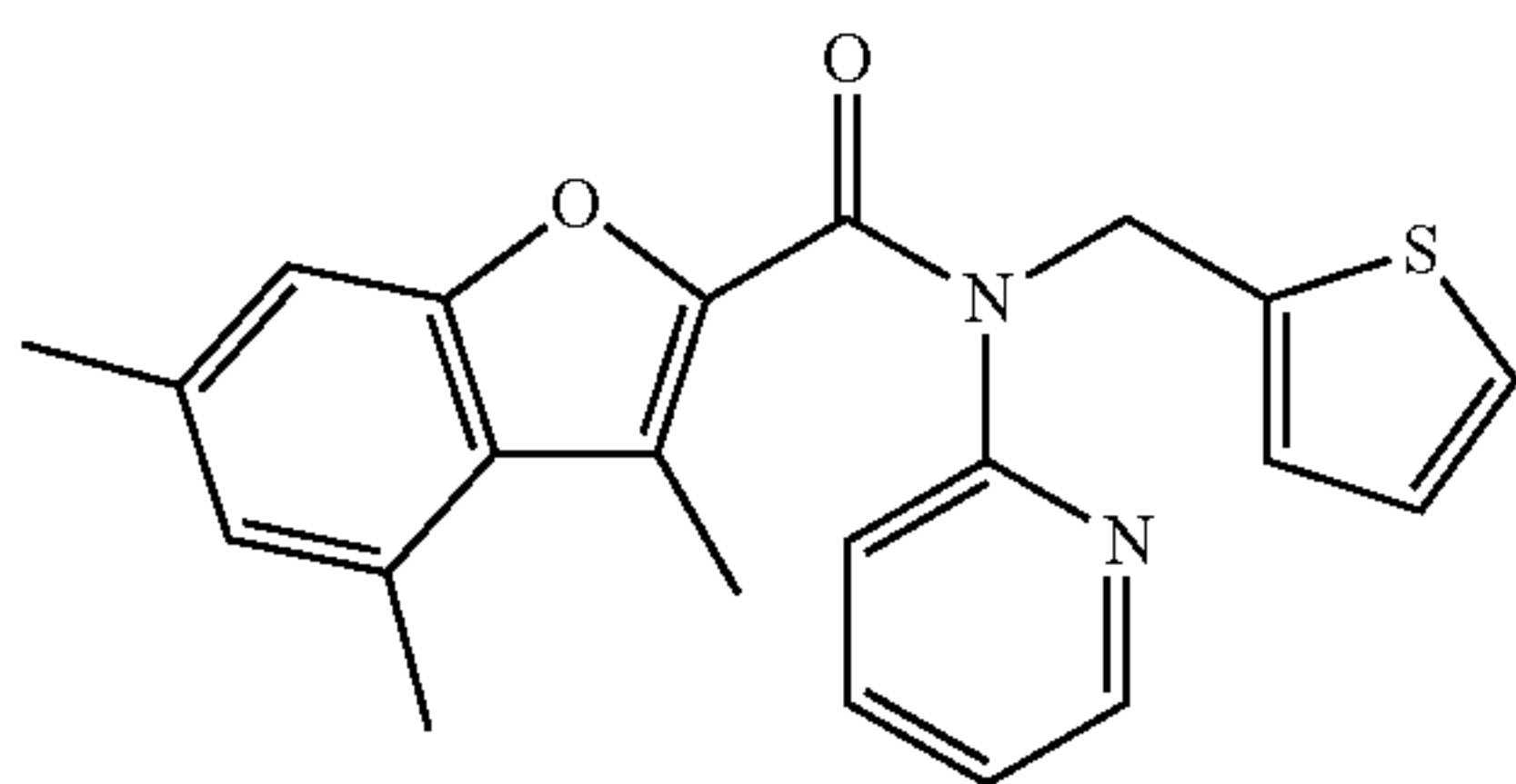
3,4,6-trimethyl-N-(pyridin-2-yl)-N-(thiophen-2-ylmethyl)benzofuran-2-carboxamide; Example 235
