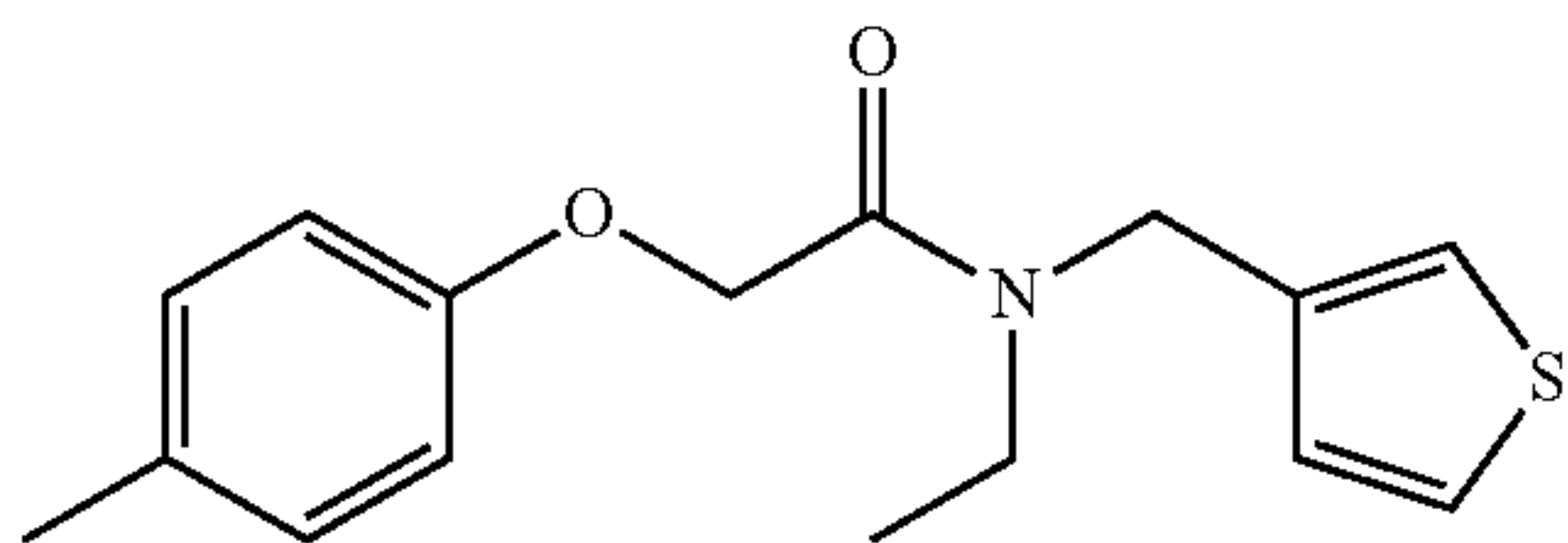
N-ethyl-N-(thiophen-3-ylmethyl)-2-(p-tolyloxy)acetamide; Example 41
