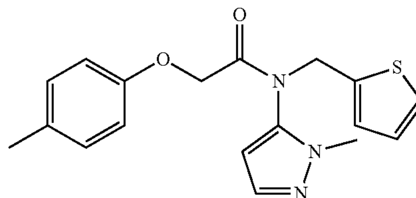
N-(1-methyl-1H-pyrazol-5-yl)-N-(thiophen-2-ylmethyl)-2-(p-toloxo)acetamide; Example 60
