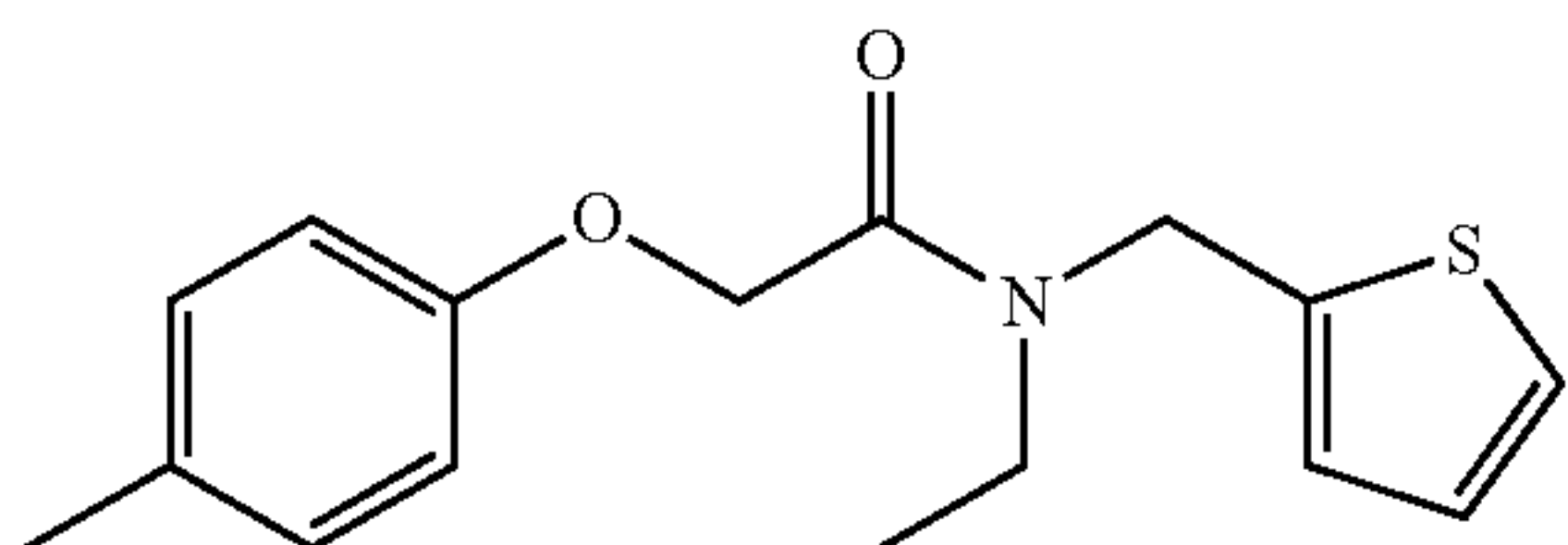
N-ethyl-N-(thiophen-2-ylmethyl)-2-(p-tolyloxy)acetamide; Example 21
