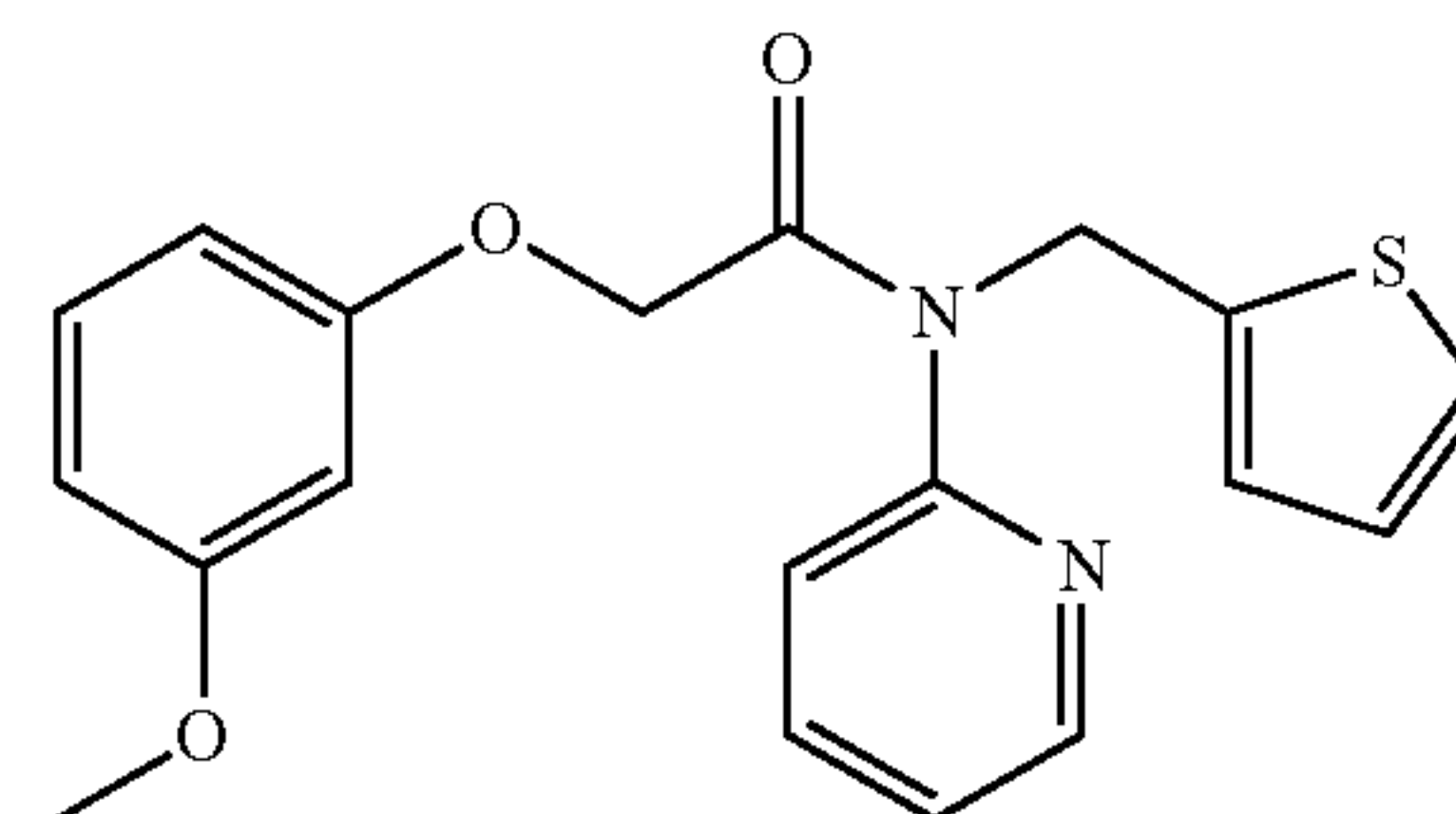
2-(3-methoxyphenoxy)-N-(pyridin-2-yl)-N-(thiophen-2-ylmethyl)acetamide; Example 116
