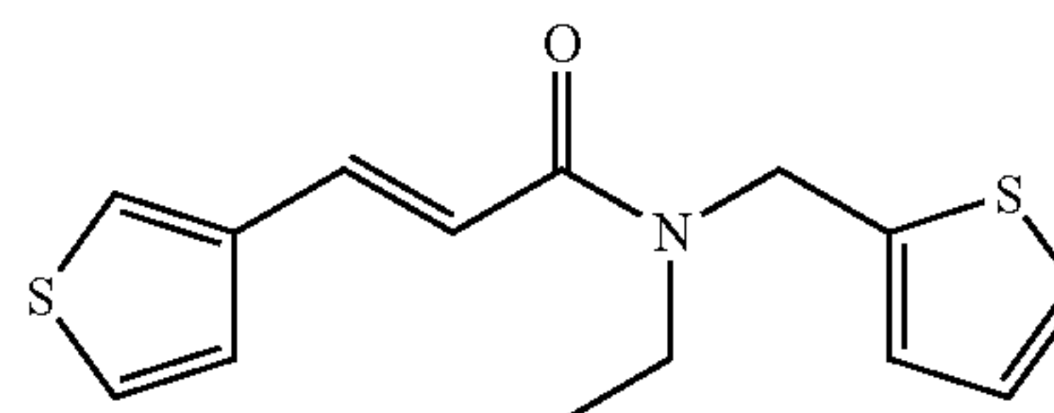
(E)-N-ethyl-N-(thiophen-2-ylmethyl)-3-(thiophen-3-yl)acrylamide; Example 245
