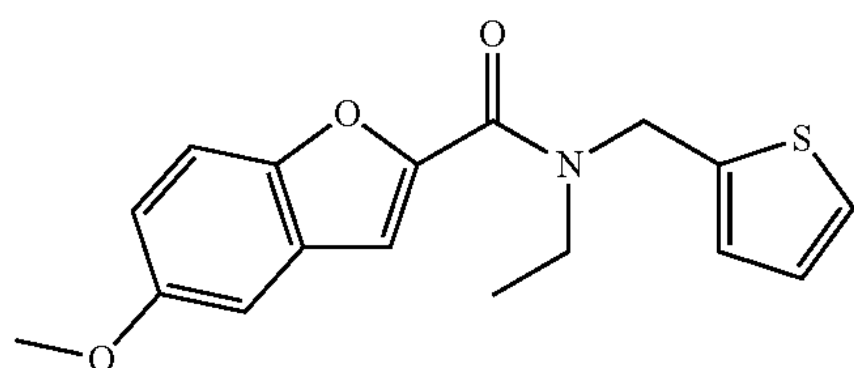
N-ethyl-5-methoxy-N-(thiophen-2-ylmethyl)benzofuran-2-carboxamide; Example 213
