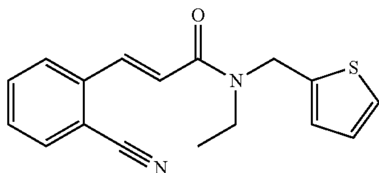
(E)-3-(2-cyanophenyl)-N-ethyl-N-(thiophen-2-ylmethyl)acrylamide; Example 228
