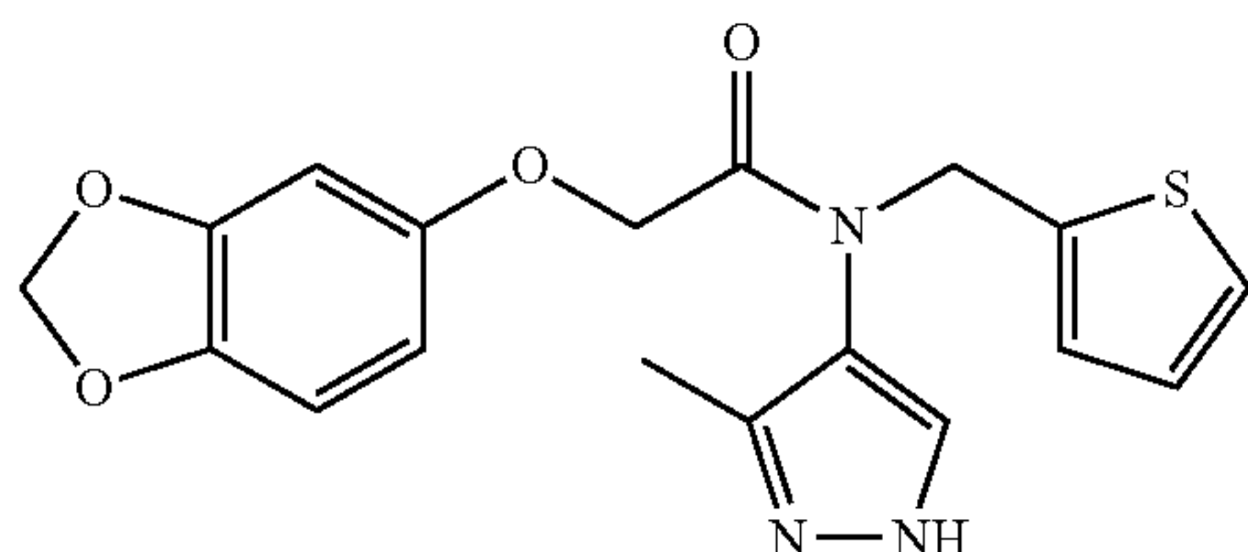
2-(benzo[d][1,3]dioxol-5-yloxy)-N-(3-methyl-1H-pyrazol-4-yl)-N-(thiophen-2-ylmethyl)acetamide; Example 18
