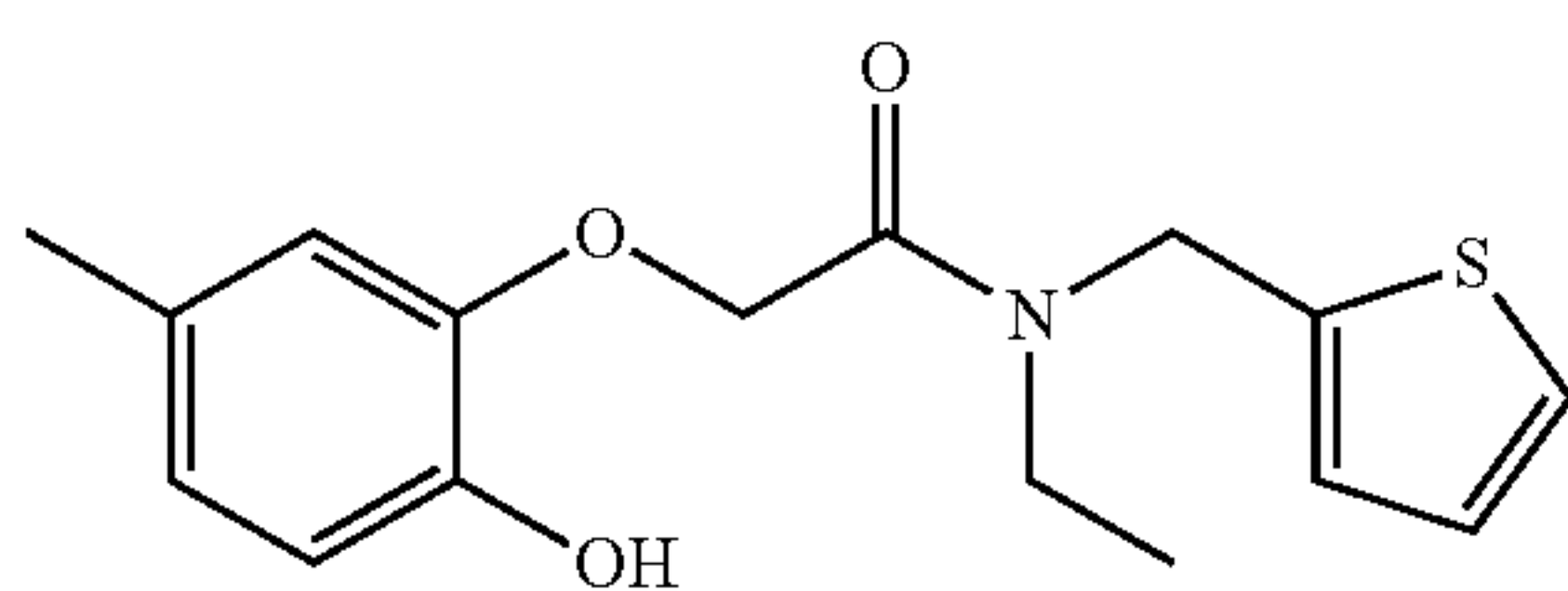
N-ethyl-2-(2-hydroxy-5-methylphenoxy)-N-(thiophen-2-ylmethyl)acetamide; Example 27
