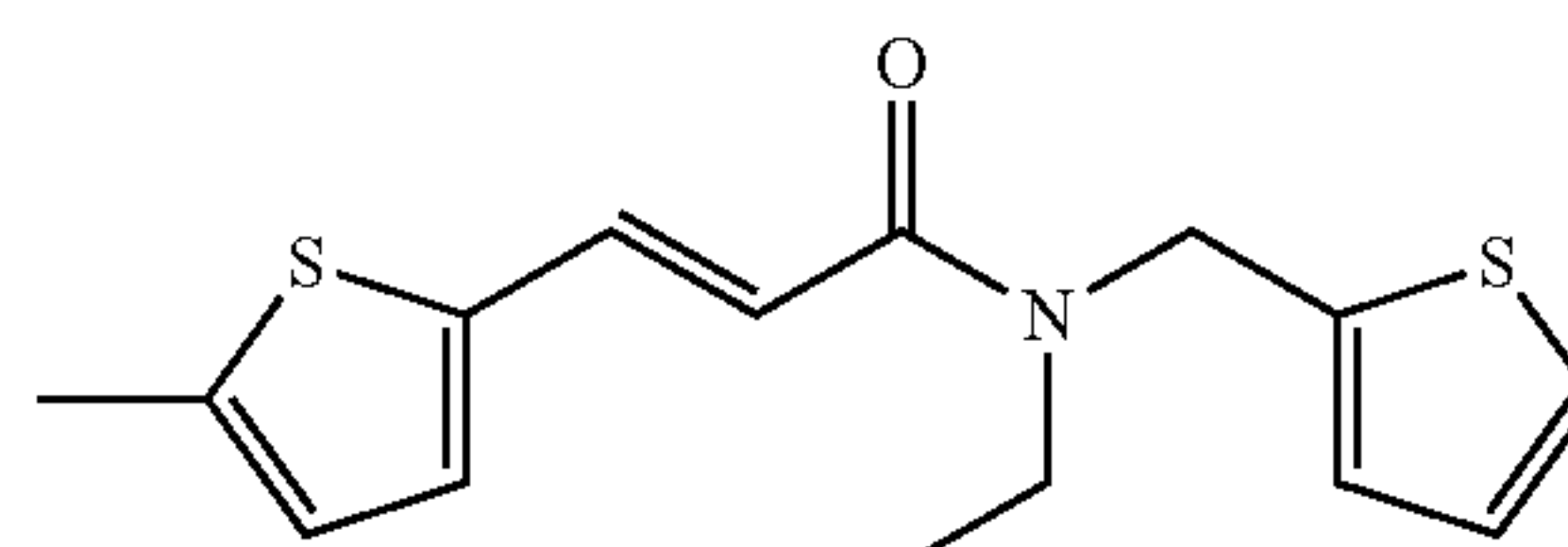
(E)-N-ethyl-3-(5-methylthiophen-2-yl)-N-(thiophen-2-ylmethyl)acrylamide; Example 209
