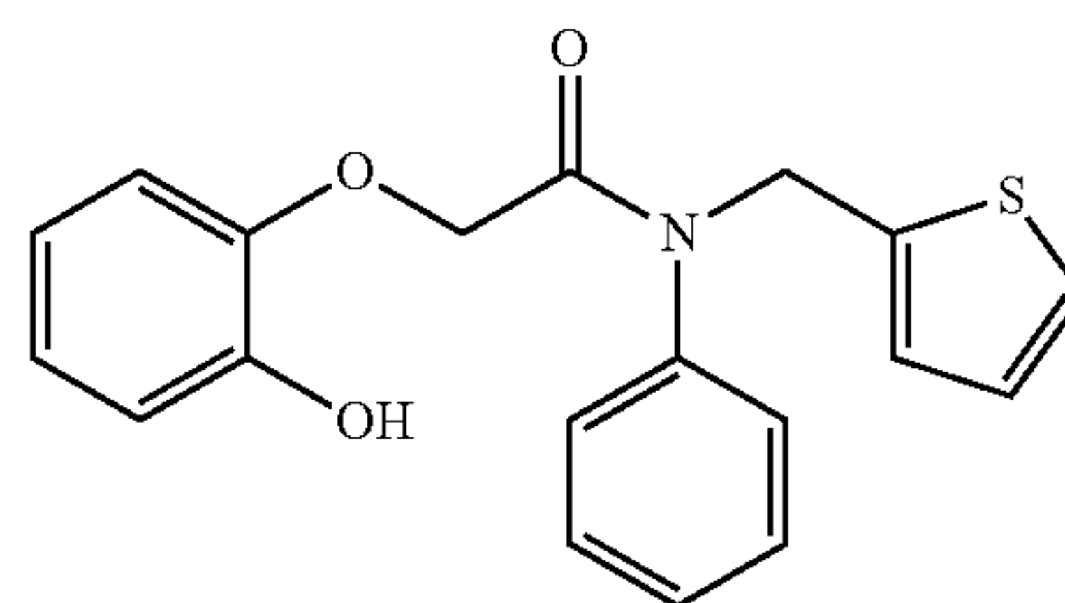
2-(2-hydroxyphenoxy)-N-phenyl-N-(thiophen-2-ylmethyl)acetamide; Example 71
