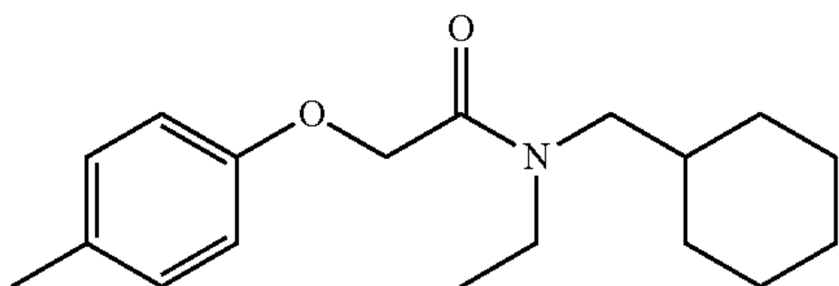
N-(cyclohexylmethyl)-N-ethyl-2-(p-tolyloxy)acetamide; Example 256
