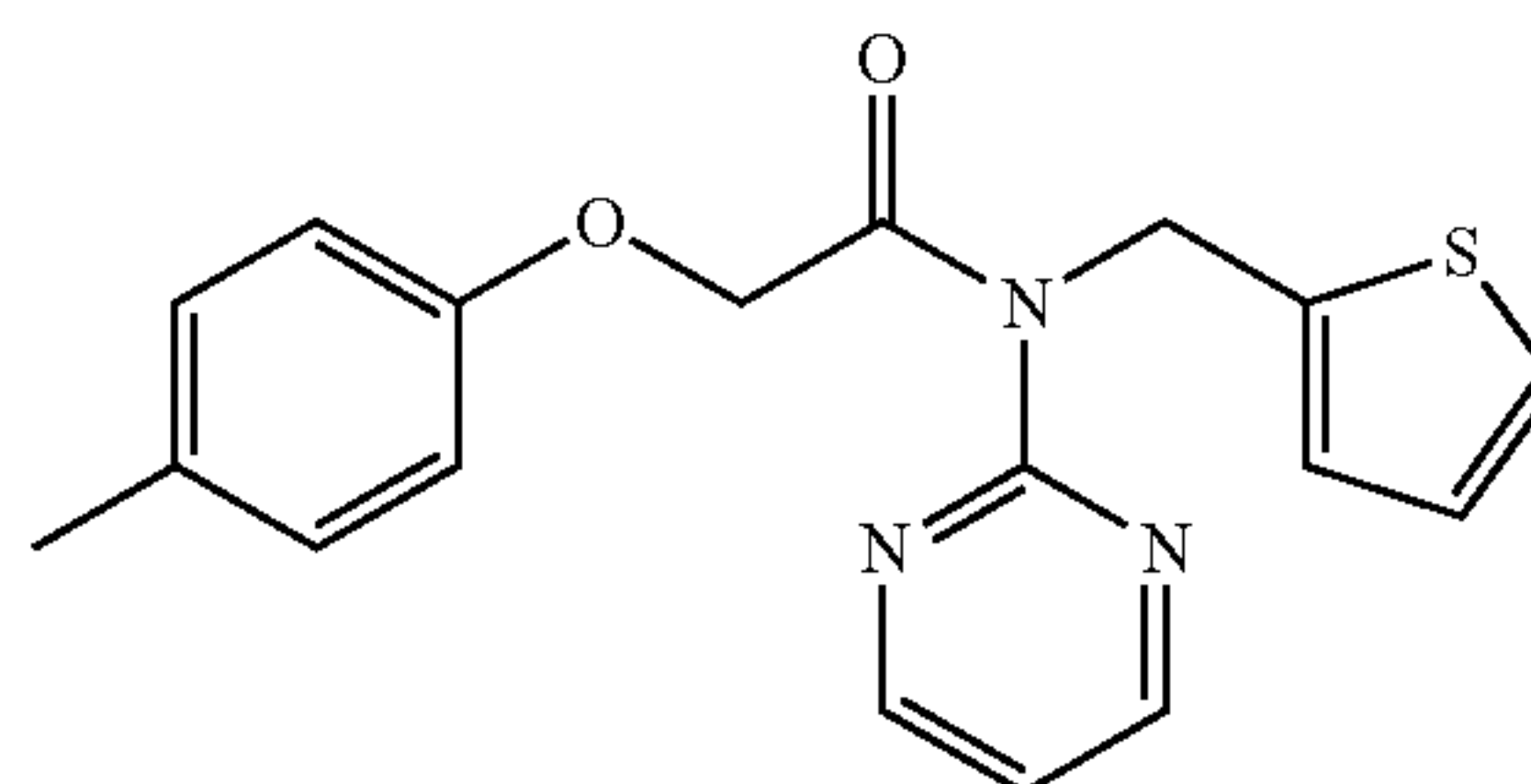
N-(pyrimidin-2-yl)-N-(thiophen-2-ylmethyl)-2-(p-tolyloxy)acetamide; Example 159
