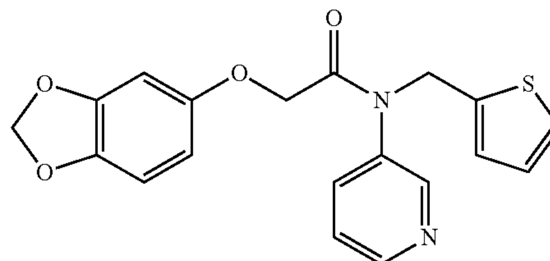
2-(benzo[d][1,3]dioxol-5-yloxy)-N-(pyridin-3-yl)-N-(thiophen-2-ylmethyl)acetamide; Example 70
