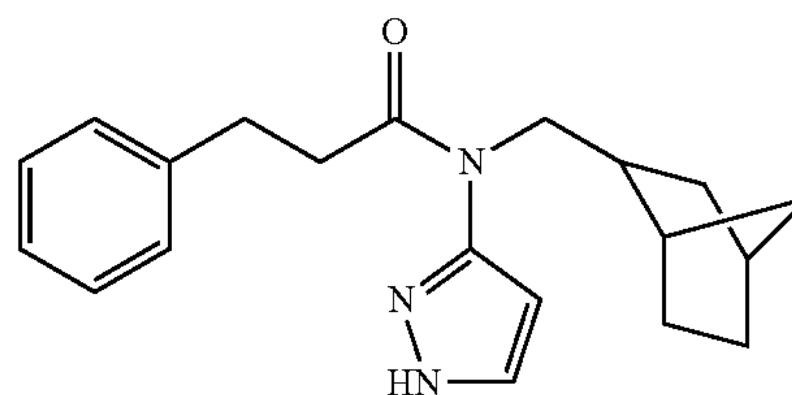
N-(bicyclo[2.2.1]heptan-2-ylmethyl)-3-phenyl-N-(1H-pyrazol-3-yl)propanamide; Example 50
