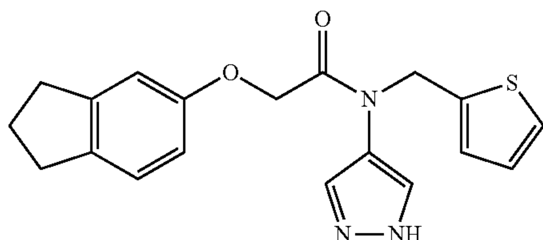
2-(2,3-dihydro-1H-inden-5-yloxy)-N-(1H-pyrazol-4-yl)-N-(thiophen-2-ylmethyl)acetamide; Example 3
