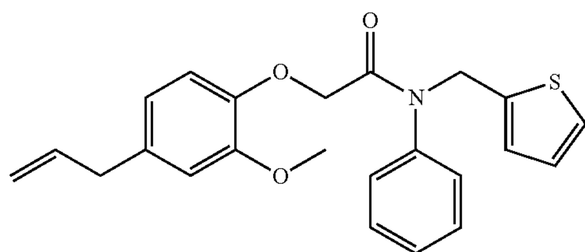
2-(4-allyl-2-methoxyphenoxy)-N-phenyl-N-(thiophen-2-ylmethyl)acetamide; Example 154
