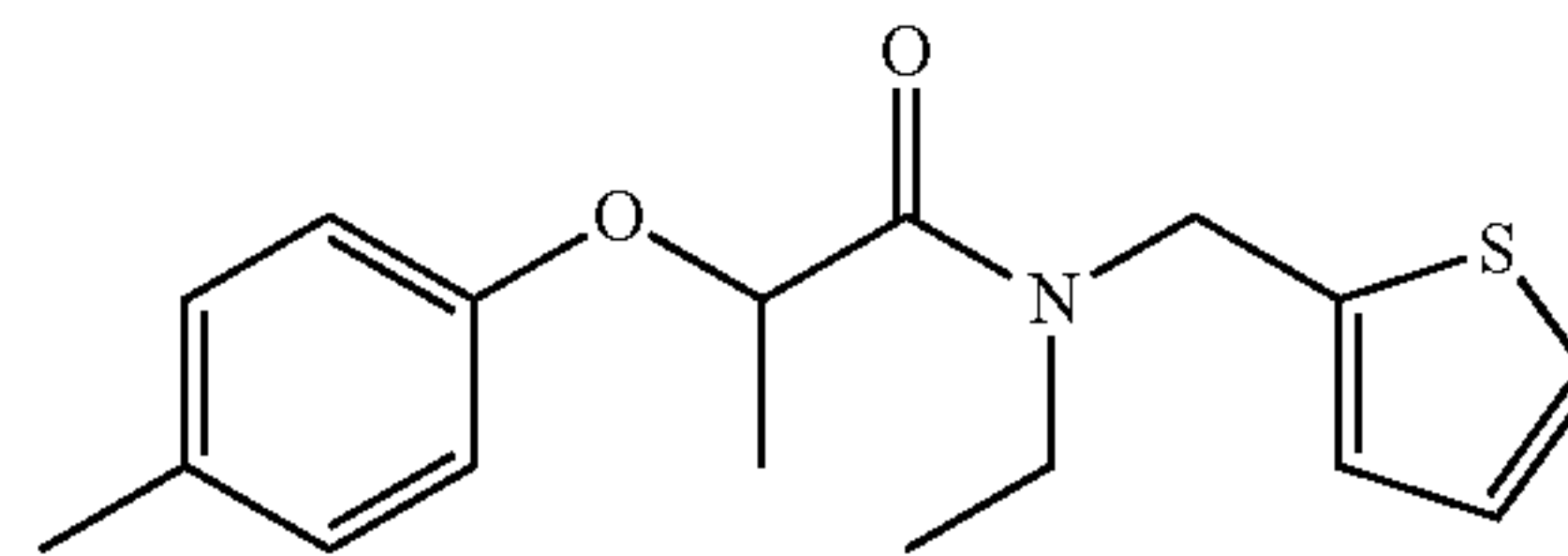
N-ethyl-N-(thiophen-2-ylmethyl)-2-(p-tolyloxy)propanamide; Example 107
