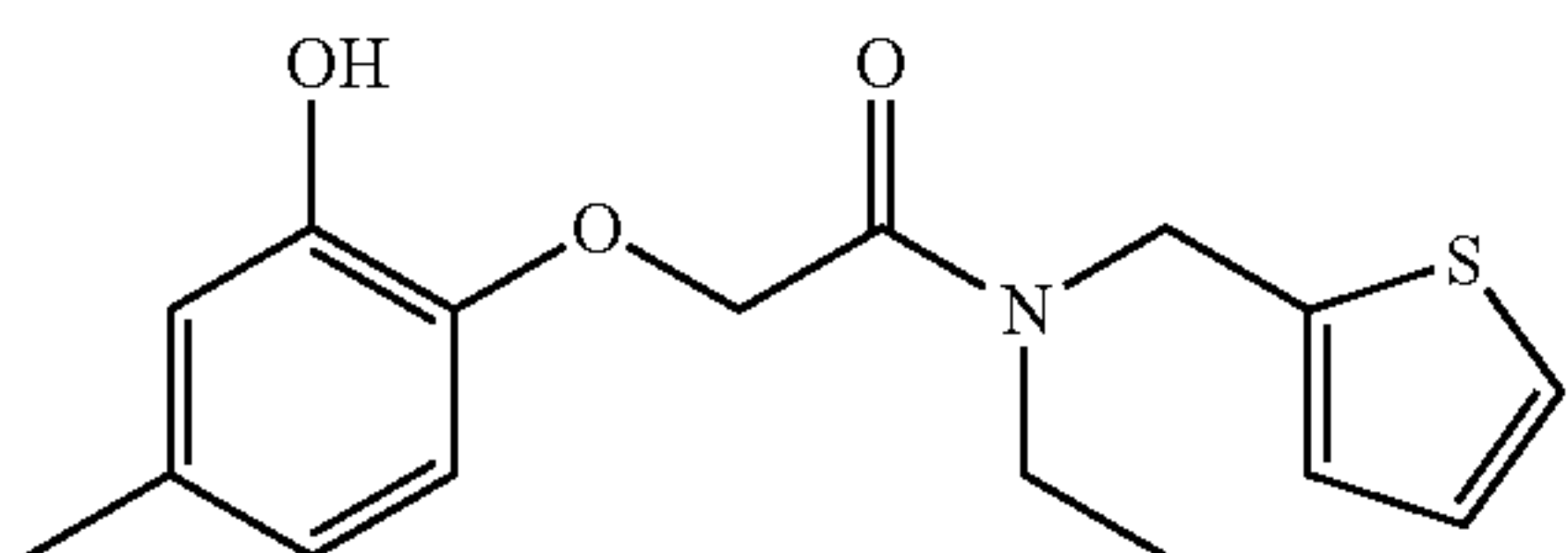
N-ethyl-2-(2-hydroxy-4-methylphenoxy)-N-(thiophen-2-ylmethyl)acetamide; Example 19
