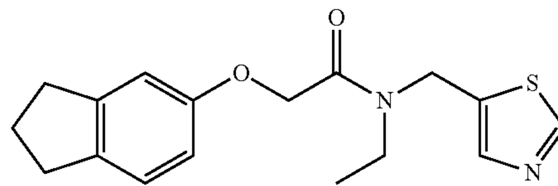
2-(2,3-dihydro-1H-inden-5-yloxy)-N-ethyl-N-(thiazol-5-ylmethyl)acetamide; Example 205
