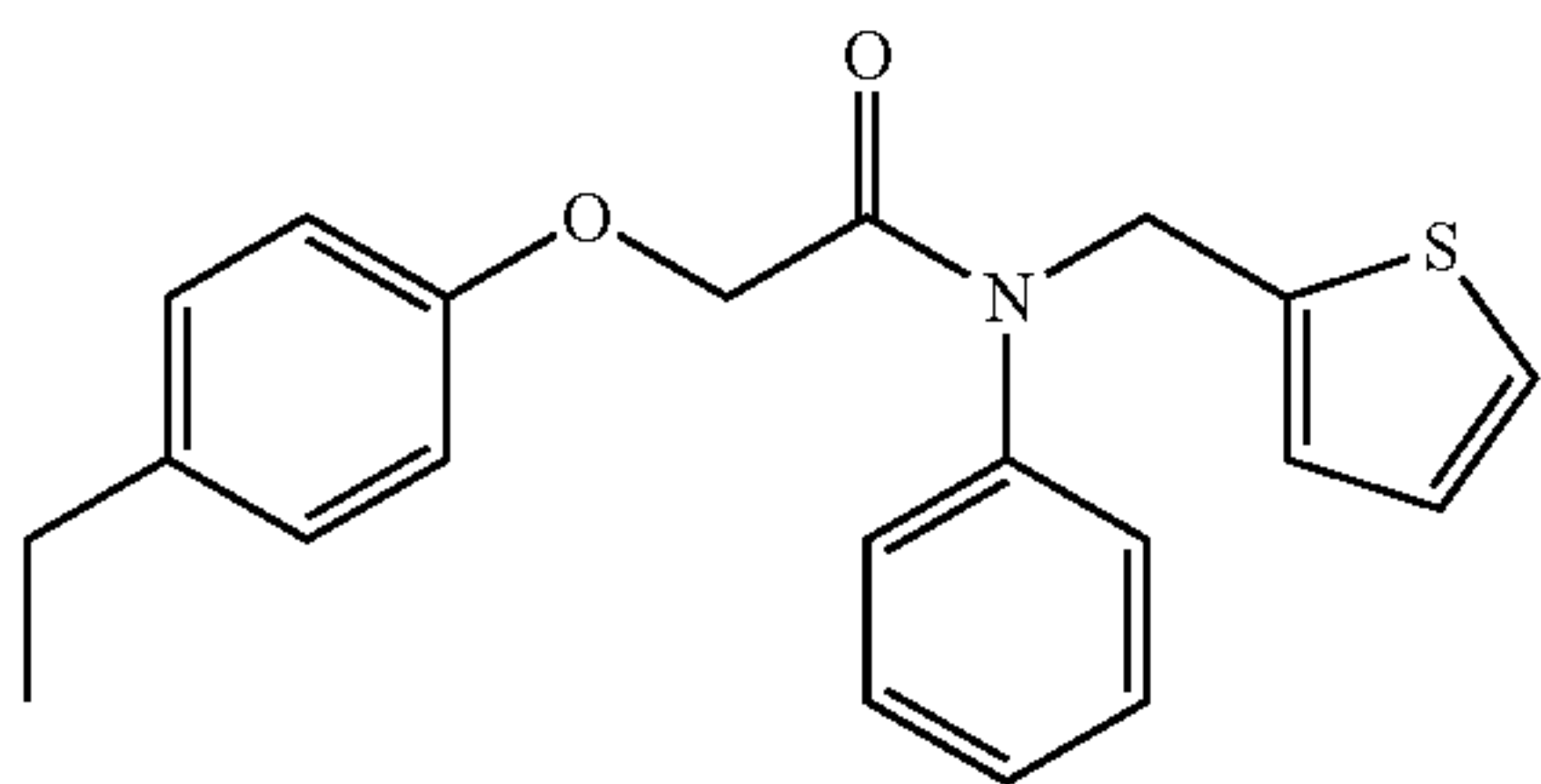
2-(4-ethylphenoxy)-N-phenyl-N-(thiophen-2-ylmethyl)acetamide; Example 63
