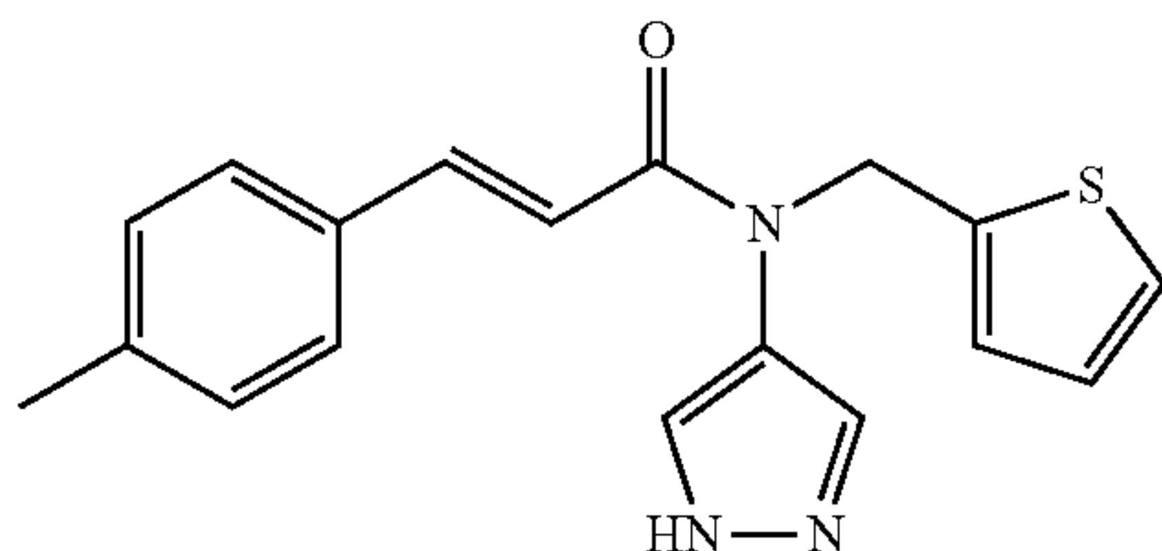
(E)-N-(1H-pyrazol-4-yl)-N-(thiophen-2-ylmethyl)-3-p-tolylacrylamide; Example 174
