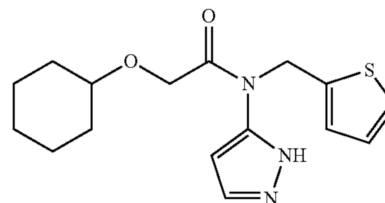
2-(cyclohexyloxy)-N-(1H-pyrazol-5-yl)-N-(thiophen-2-ylmethyl)acetamide; Example 232
