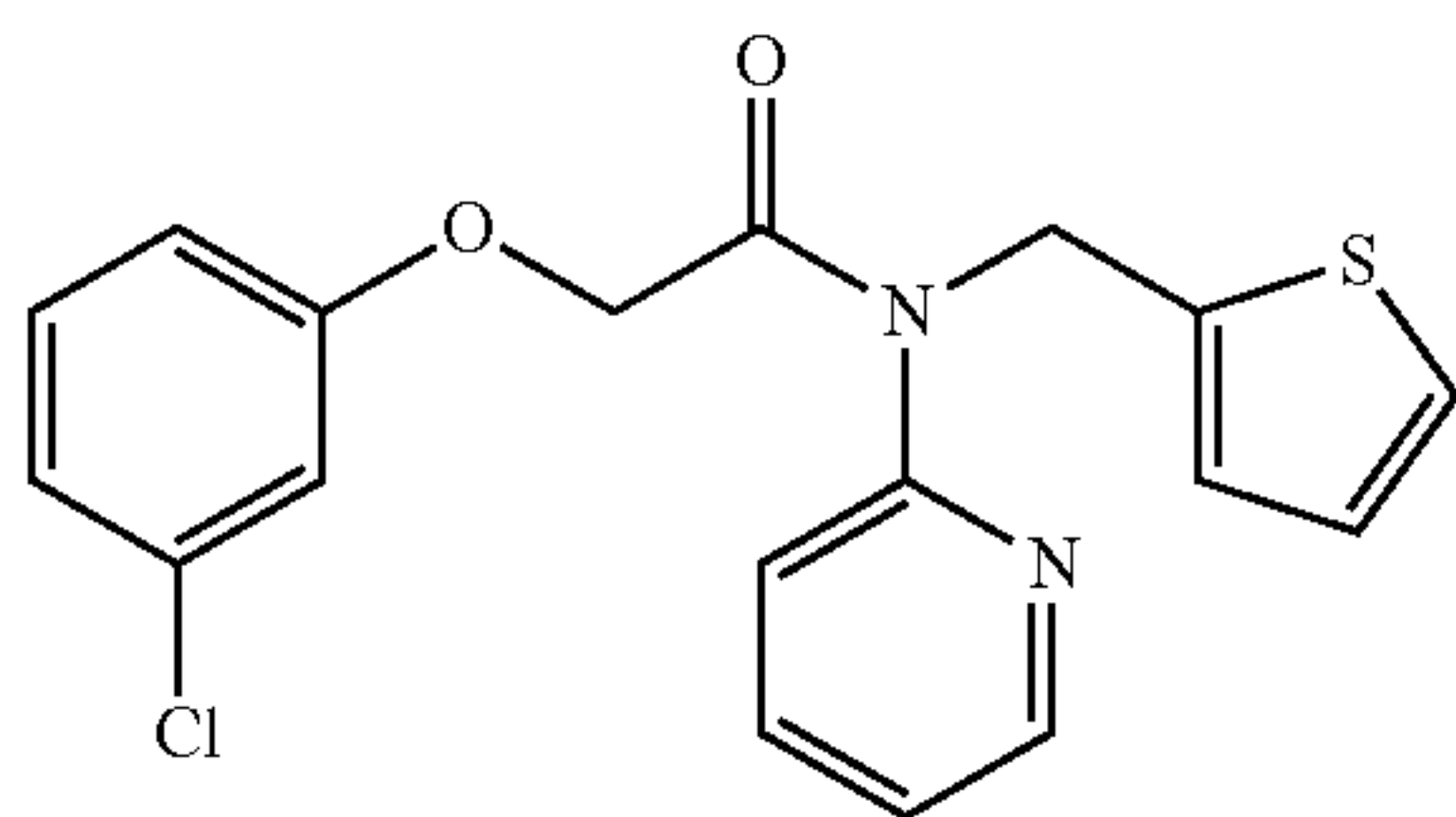
2-(3-chlorophenoxy)-N-(pyridin-2-yl)-N-(thiophen-2-ylmethyl)acetamide; Example 166
