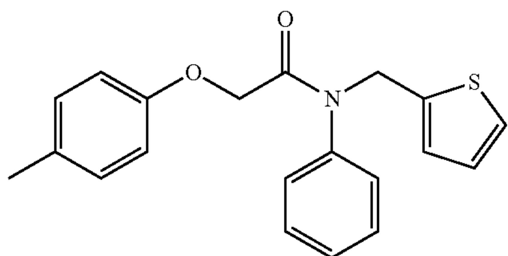
N-phenyl-N-(thiophen-2-ylmethyl)-2-(p-tolyloxy)acetamide; Example 26
