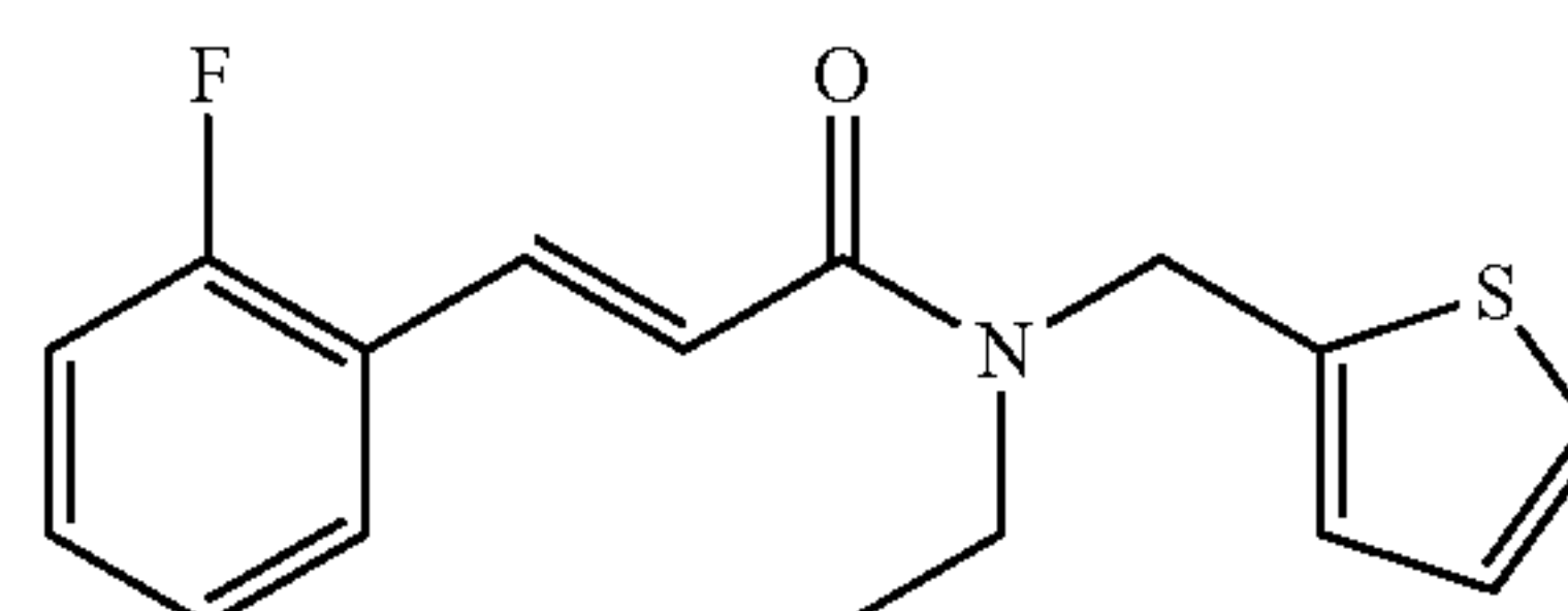
(E)-N-ethyl-3-(2-fluorophenyl)-N-(thiophen-2-ylmethyl)acrylamide; Example 216
