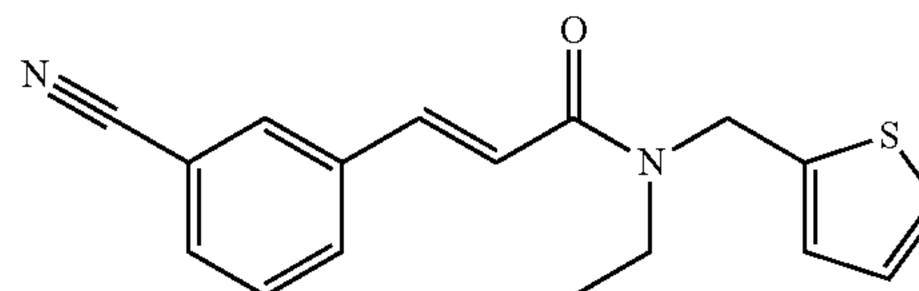
(E)-3-(3-cyanophenyl)-N-ethyl-N-(thiophen-2-ylmethyl)acrylamide; Example 246
