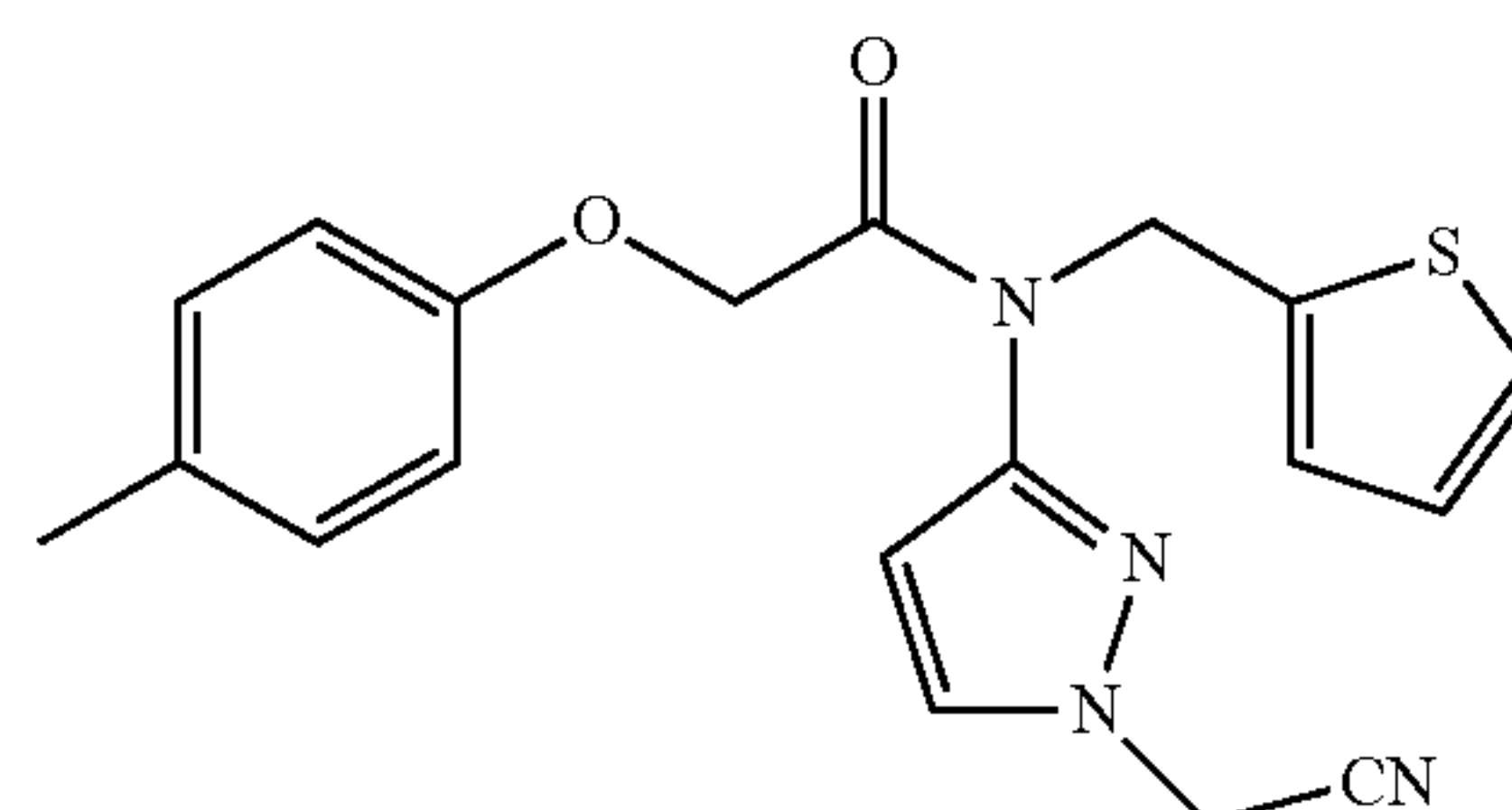
N-(1-(cyanomethyl)-1H-pyrazol-3-yl)-N-(thiophen-2-ylmethyl)-2-(p-tolyloxy)acetamide; Example 17
