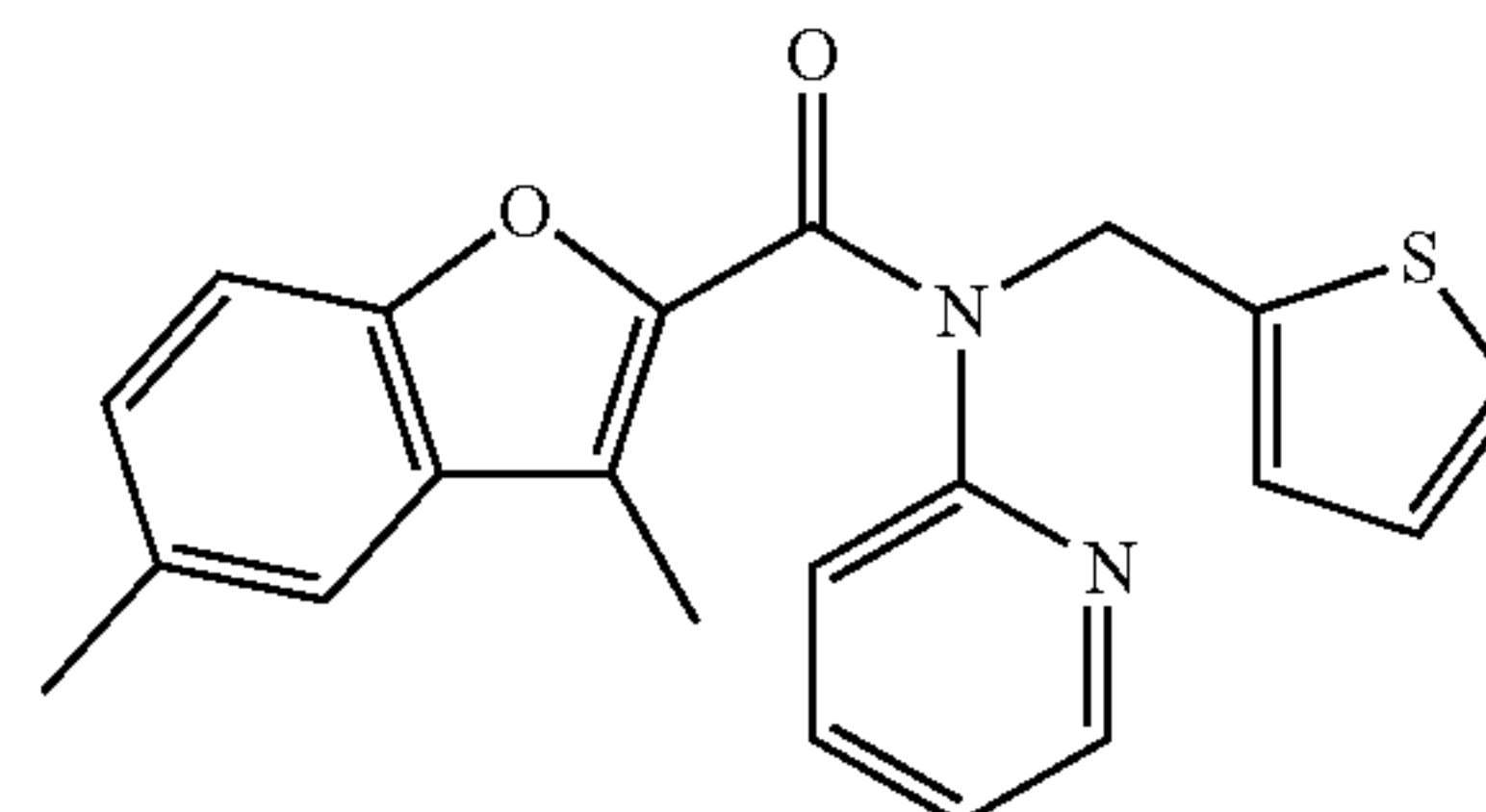
3,5-dimethyl-N-(pyridin-2-yl)-N-(thiophen-2-ylmethyl)benzofuran-2-carboxamide; Example 115
