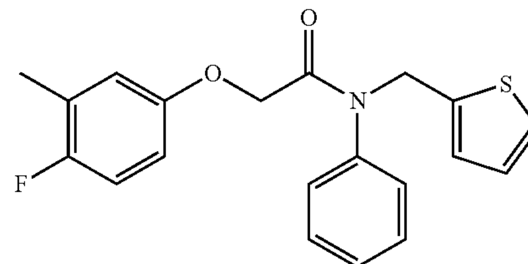
2-(4-fluoro-3-methylphenoxy)-N-phenyl-N-(thiophen-2-ylmethyl)acetamide; Example 64
