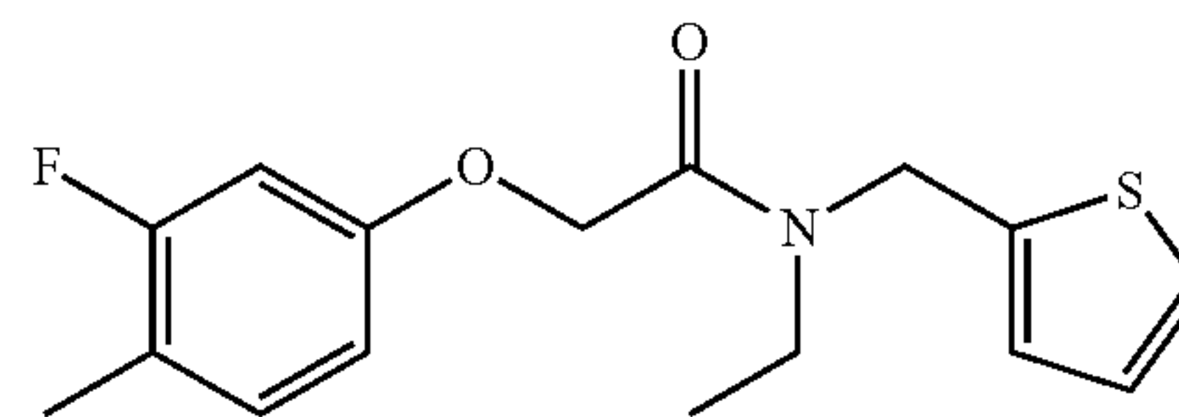
N-ethyl-2-(3-fluoro-4-methylphenoxy)-N-(thiophen-2-ylmethyl)acetamide; Example 32
