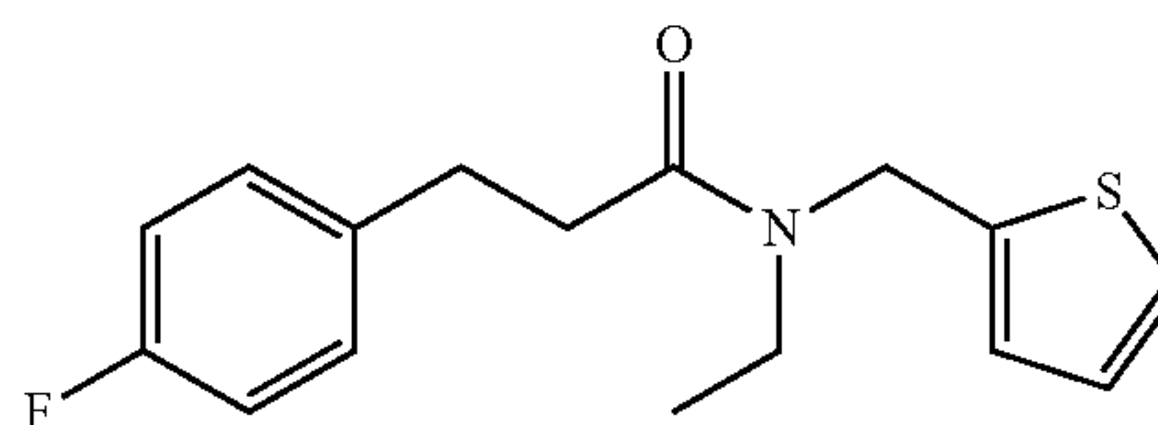
N-ethyl-3-(4-fluorophenyl)-N-(thiophen-2-ylmethyl)propanamide; Example 69
