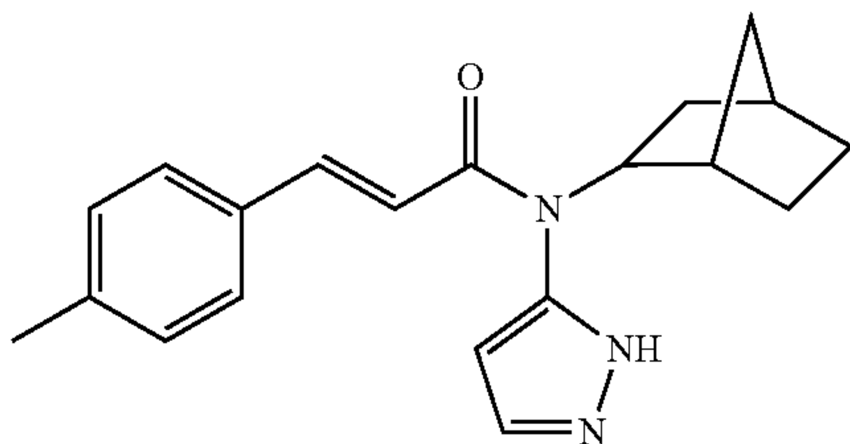
(E)-N-(bicyclo[2.2.1]heptan-2-yl)-N-(1H-pyrazol-5-yl)-3-p-tolylacrylamide; Example 223
