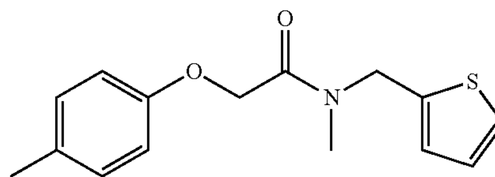
N-methyl-N-(thiophen-2-ylmethyl)-2-(p-tolyloxy)acetamide; Example 85
