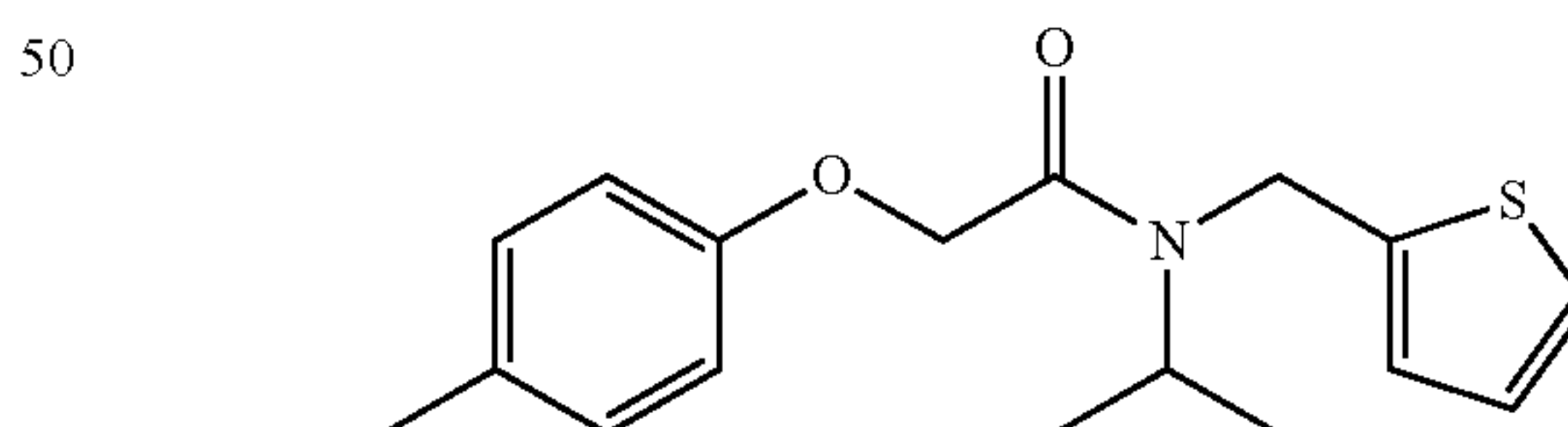
N-isopropyl-N-(thiophen-2-ylmethyl)-2-(p-tolyloxy)acetamide; Example 38
