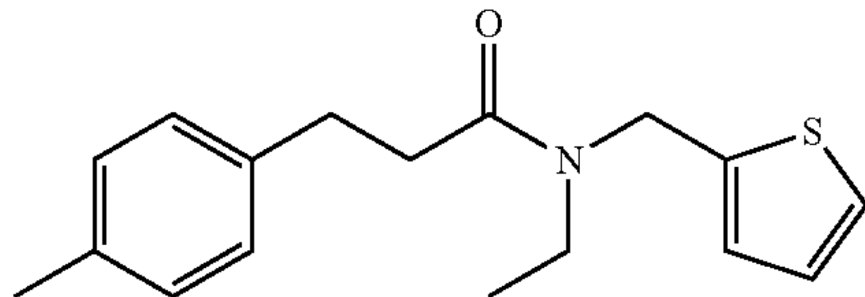
N-ethyl-N-(thiophen-2-ylmethyl)-3-p-tolylpropanamide; Example 206
