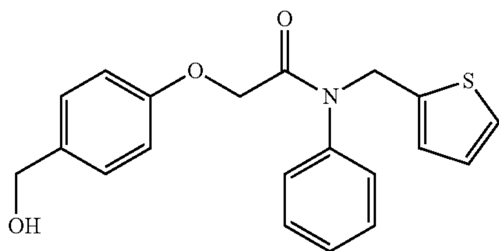
2-(4-(hydroxymethyl)phenoxy)-N-phenyl-N-(thiophen-2-ylmethyl)acetamide; Example 141
