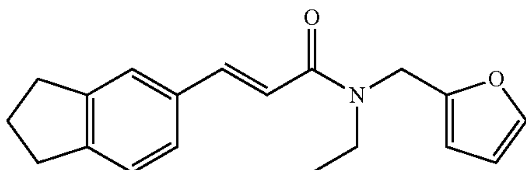
(E)-3-(2,3-dihydro-1H-inden-5-yl)-N-ethyl-N-(furan-2-ylmethyl)acrylamide; Example 231
