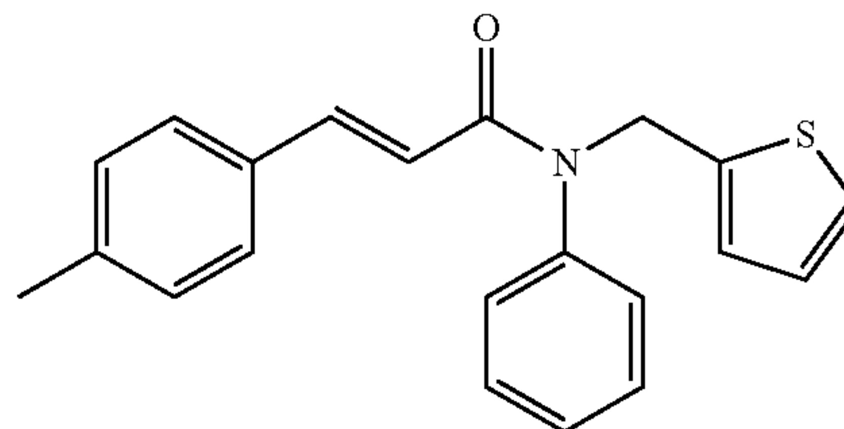
(E)-N-phenyl-N-(thiophen-2-ylmethyl)-3-p-tolylacrylamide; Example 237
