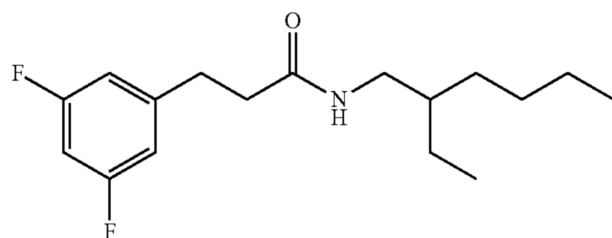
3-(3,5-difluorophenyl)-N-(2-ethylhexyl)propanamide; Example 125
