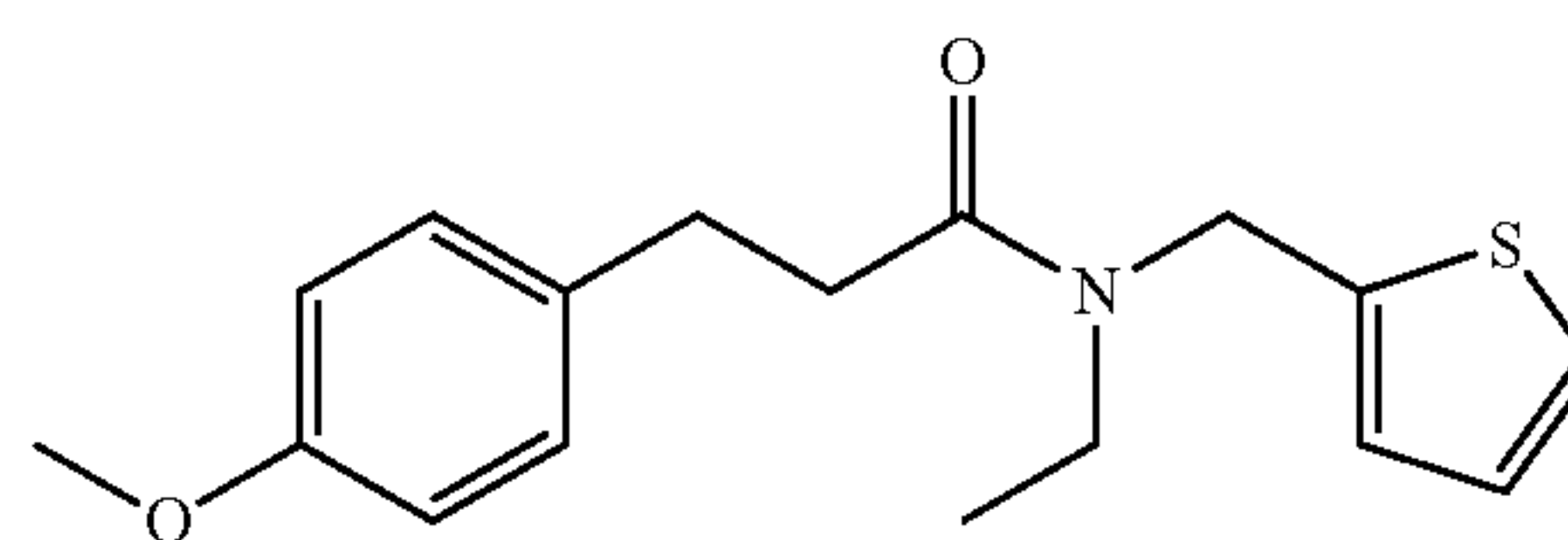
N-ethyl-3-(4-methoxyphenyl)-N-(thiophen-2-ylmethyl)propanamide; Example 126
