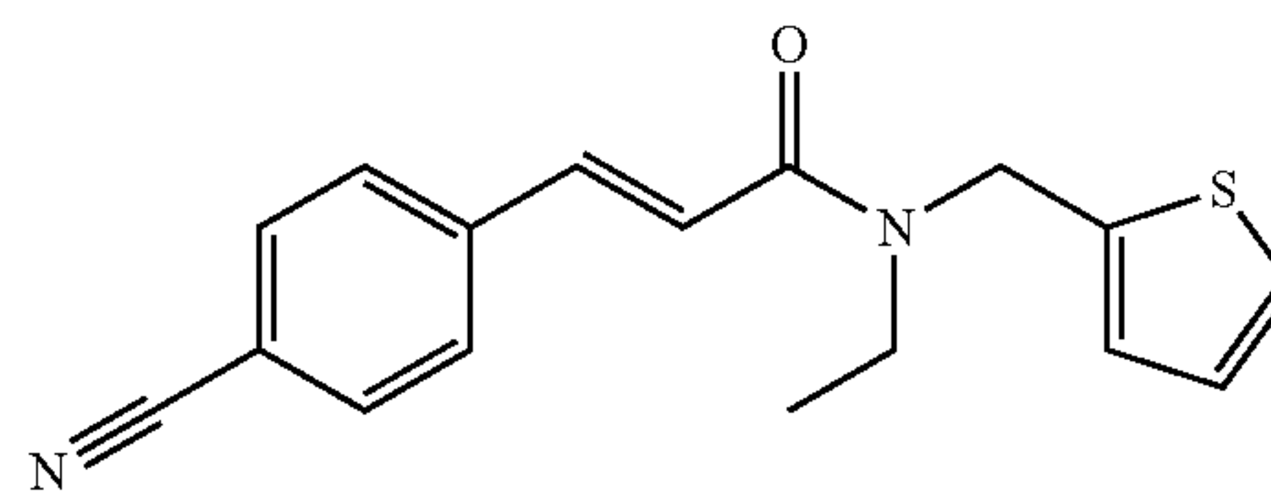
(E)-3-(4-cyanophenyl)-N-ethyl-N-(thiophen-2-ylmethyl)acrylamide; Example 226
