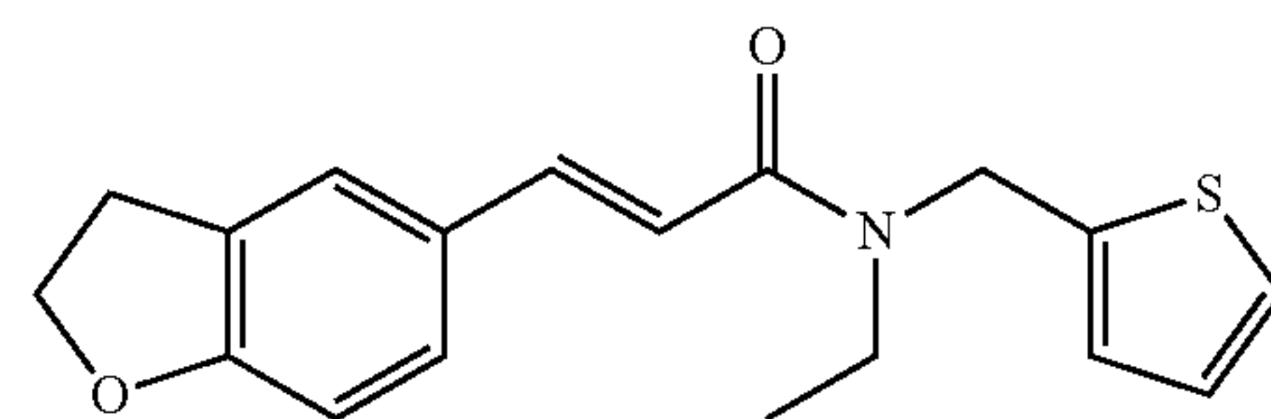
(E)-3-(2,3-dihydrobenzofuran-5-yl)-N-ethyl-N-(thiophen-2-ylmethyl)acrylamide; Example 194
