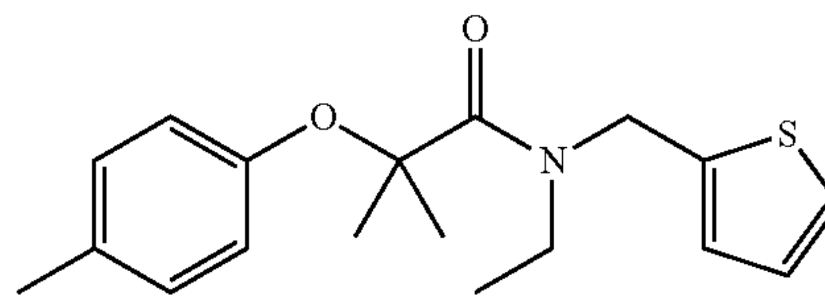
N-ethyl-2-methyl-N-(thiophen-2-ylmethyl)-2-(p-tolyloxy)propanamide; Example 170
