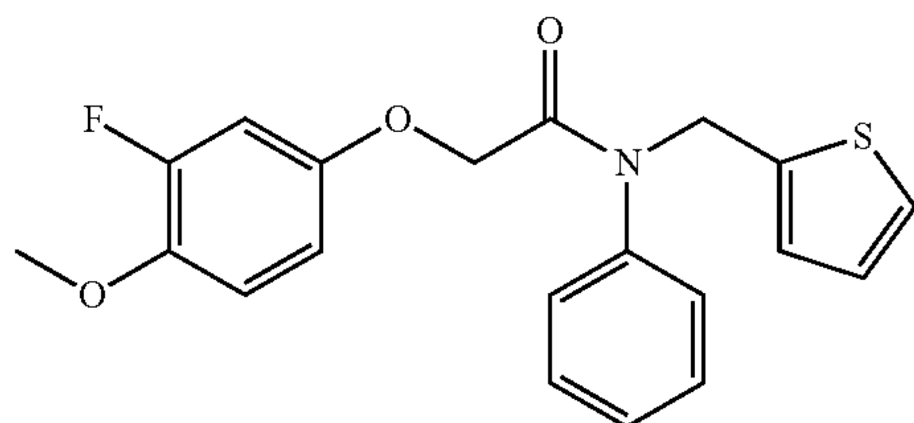
2-(3-fluoro-4-methoxyphenoxy)-N-phenyl-N-(thiophen-2-ylmethyl)acetamide; Example 76
