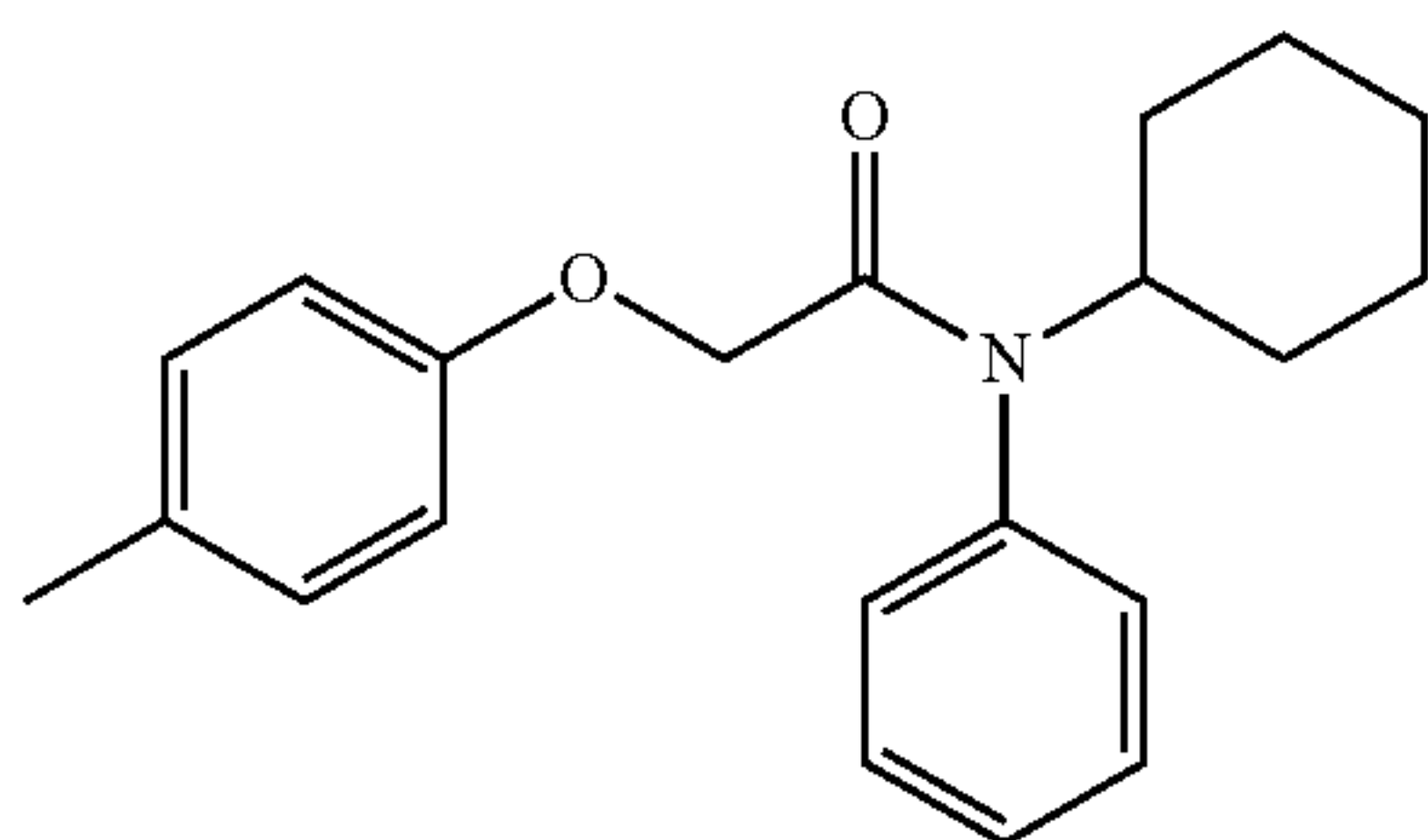
N-cyclohexyl-N-phenyl-2-(p-tolyloxy)acetamide; Example 146
