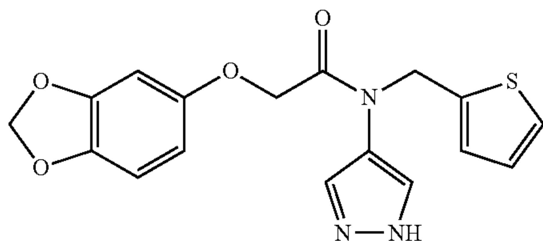
2-(benzo[d][1,3]dioxol-5-yloxy)-N-(1H-pyrazol-4-yl)-N-(thiophen-2-ylmethyl)acetamide; Example 20
