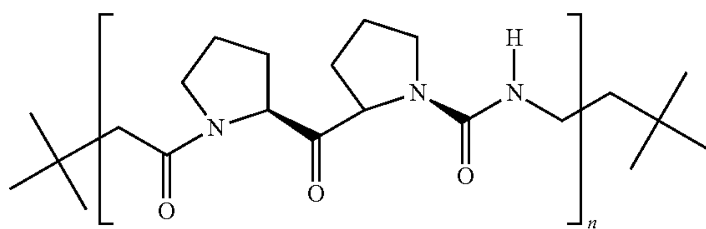
polyproline linker
