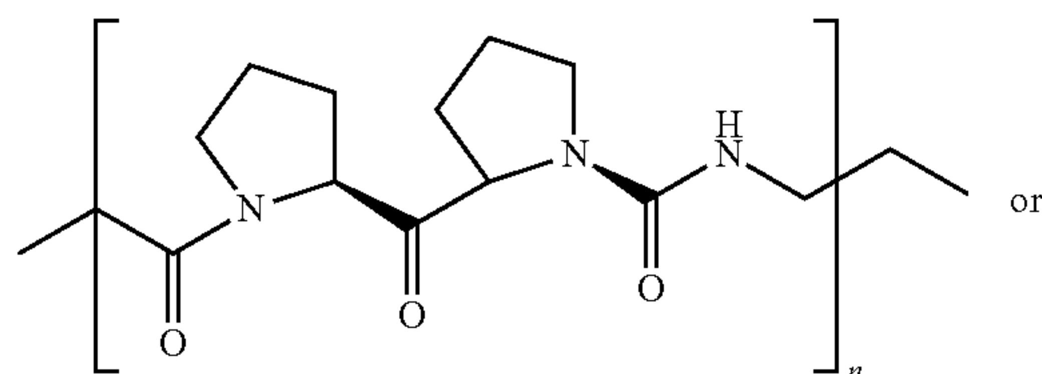
POLYPROLINE LINKER
