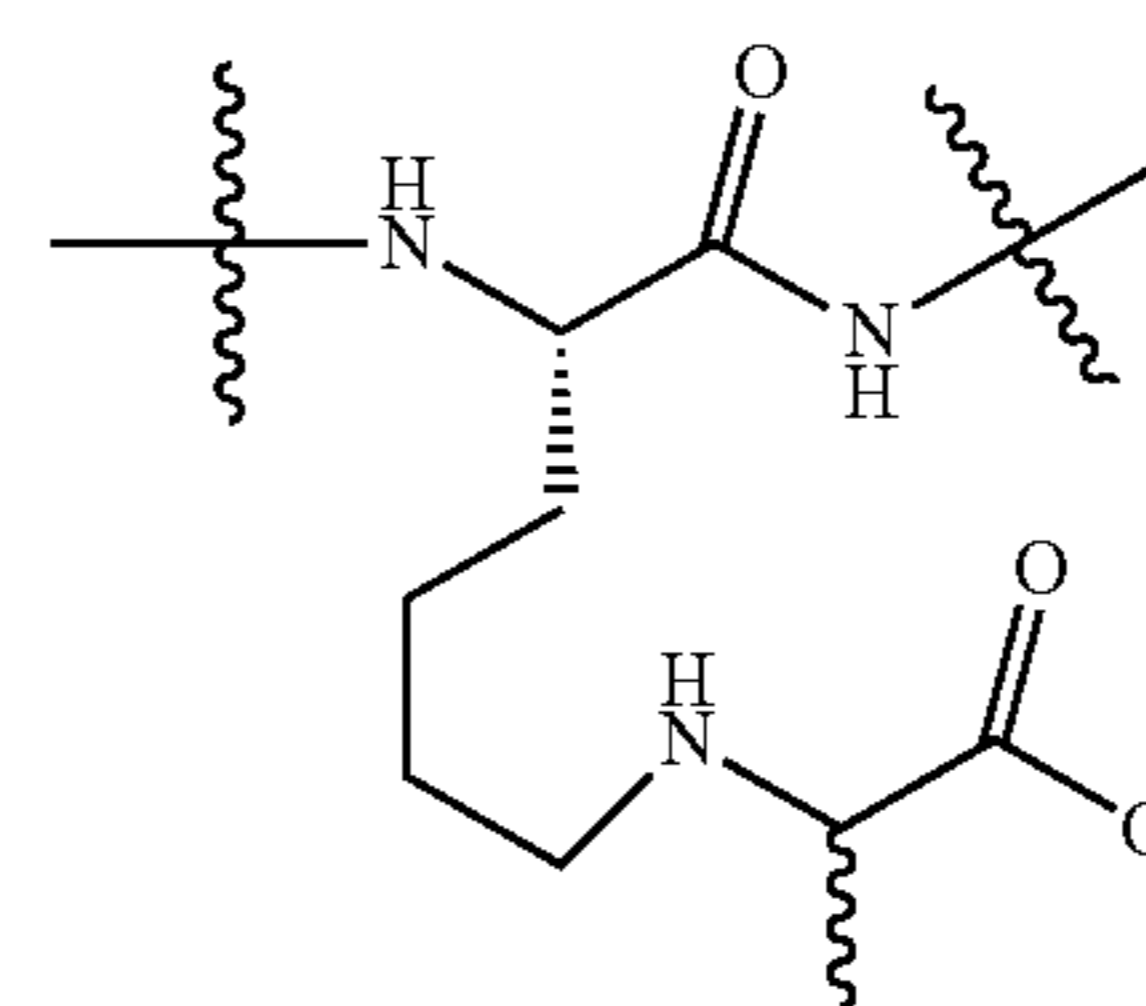
Carboxyethyl Lysine (CEL)
