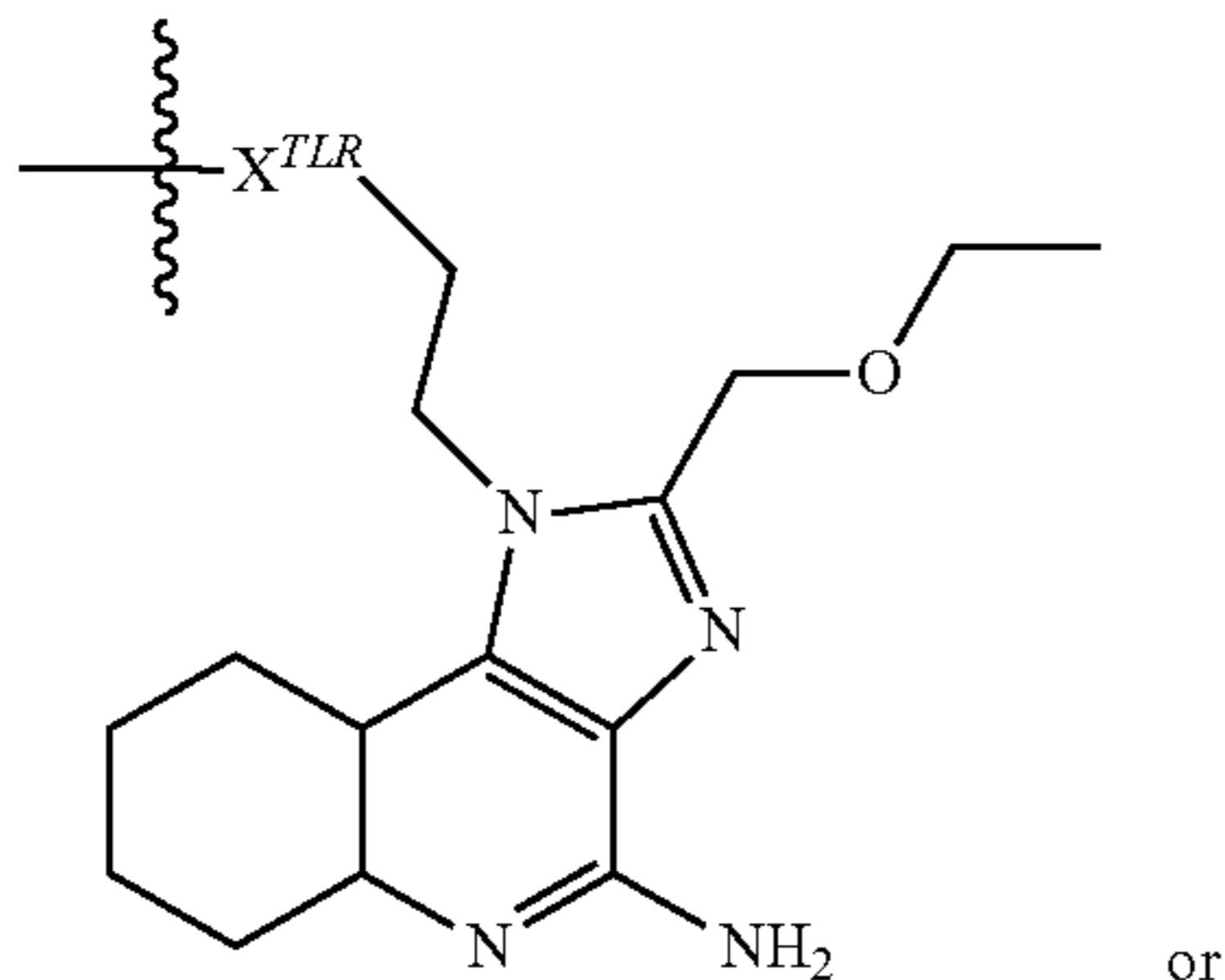
4-amino-2-(ethoxymethyl)- alpha, alpha-dimethyl-6,7,8,9- tetrahydro-1H-imidazo[4,5-c] quinoline-1-ethanol
