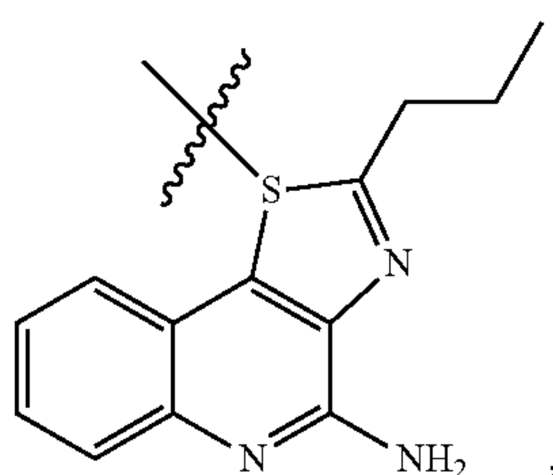
2-propylthiazolo [4,5-c]quinolin-4-amine
