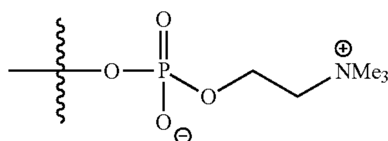
Phosphoryl Choline
