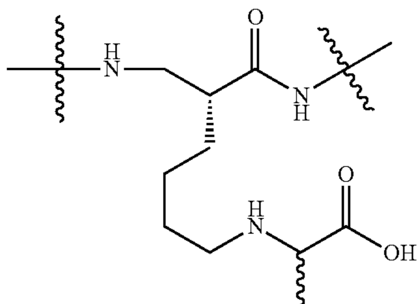
Carboxyethyl Lysine (CEL)
