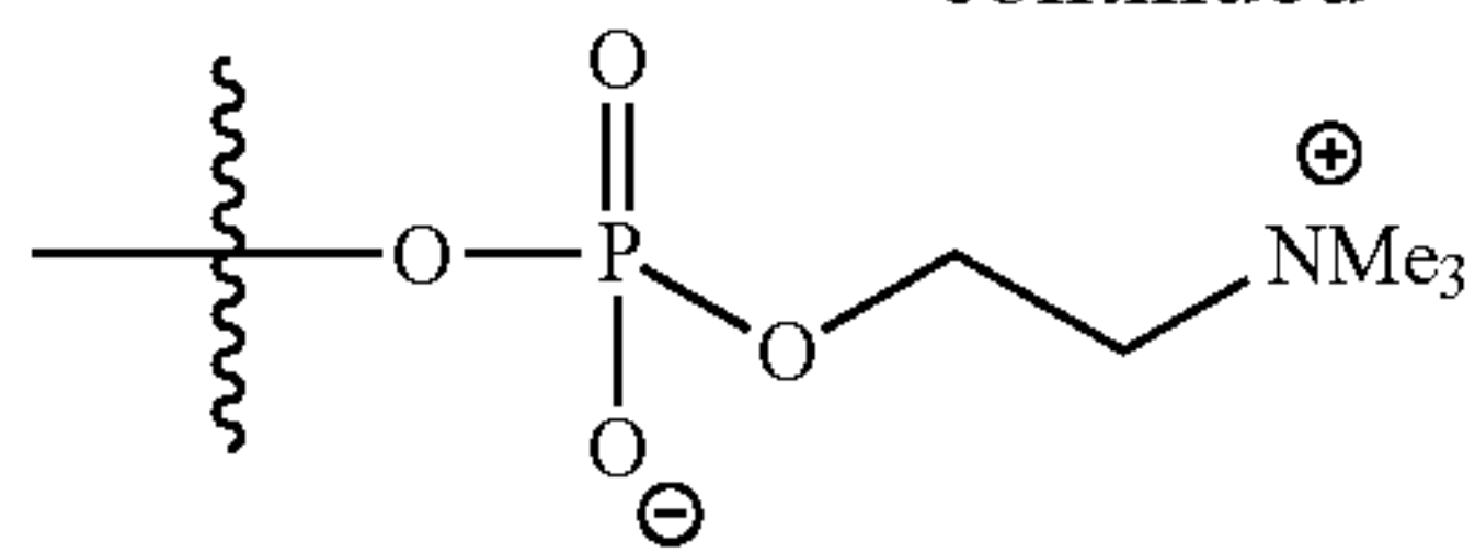
Phosphoryl Choline
