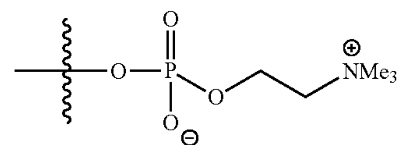
Phosphoryl Choline
