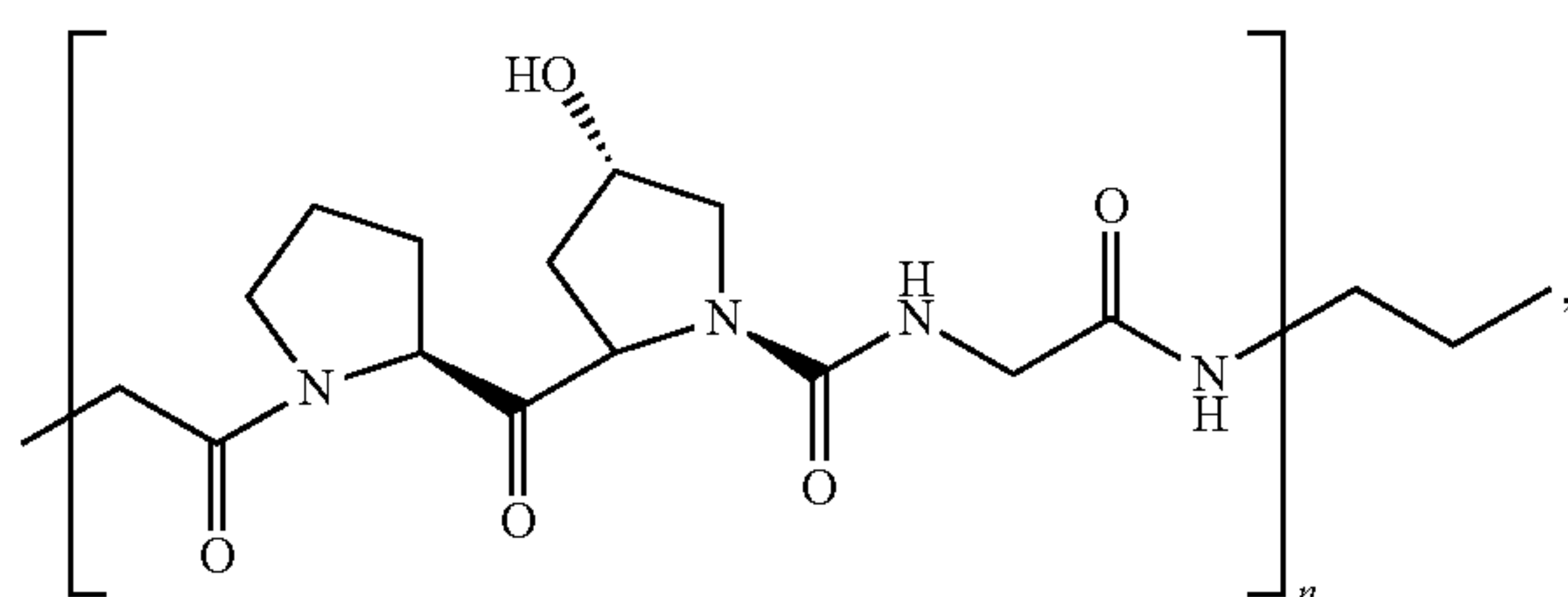
COLLAGEN LINKER
