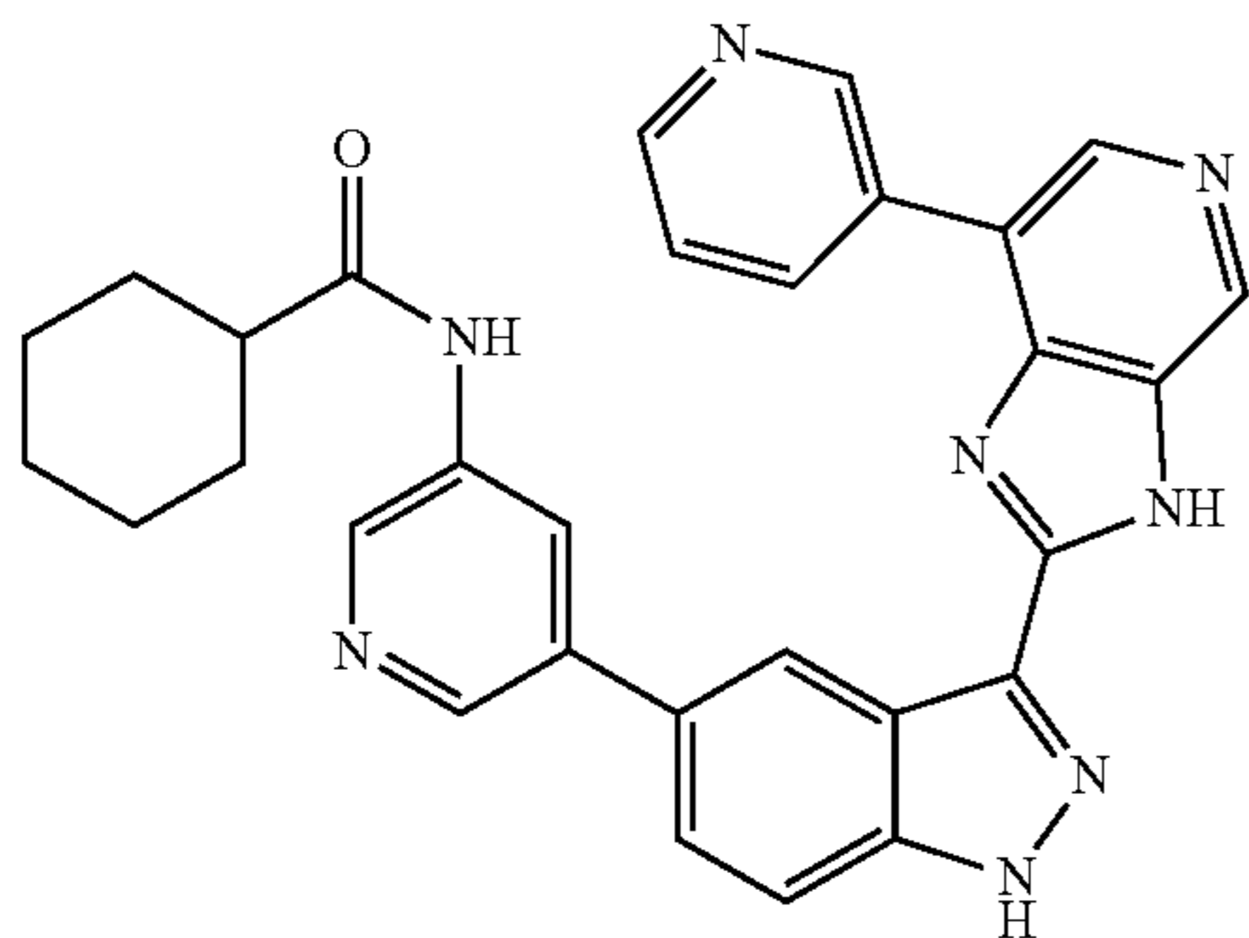
N-(5-(3-(7-(pyridin-3-yl)-3H-imidazo[4,5-c]pyridin-2-yl)-1H-indazol-5-yl)pyridin-3-yl)cyclohexanecarboxamide 19
