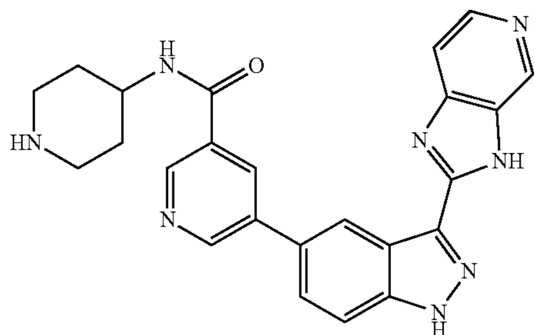
5-(3-(3H-imidazo[4,5-c]pyridin-2-yl)-1H-indazol-5-yl)-N-(piperidin-4-yl)nicotinamide 1
