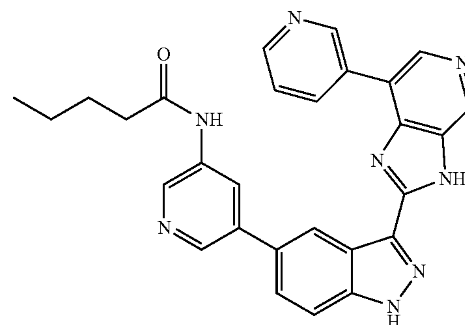
N-(5-(3-(7-(pyridin-3-yl)-3H-imidazo[4,5-c]pyridin-2-yl)-1H-indazol-5-yl)pyridin-3-yl)pentanamide 23
