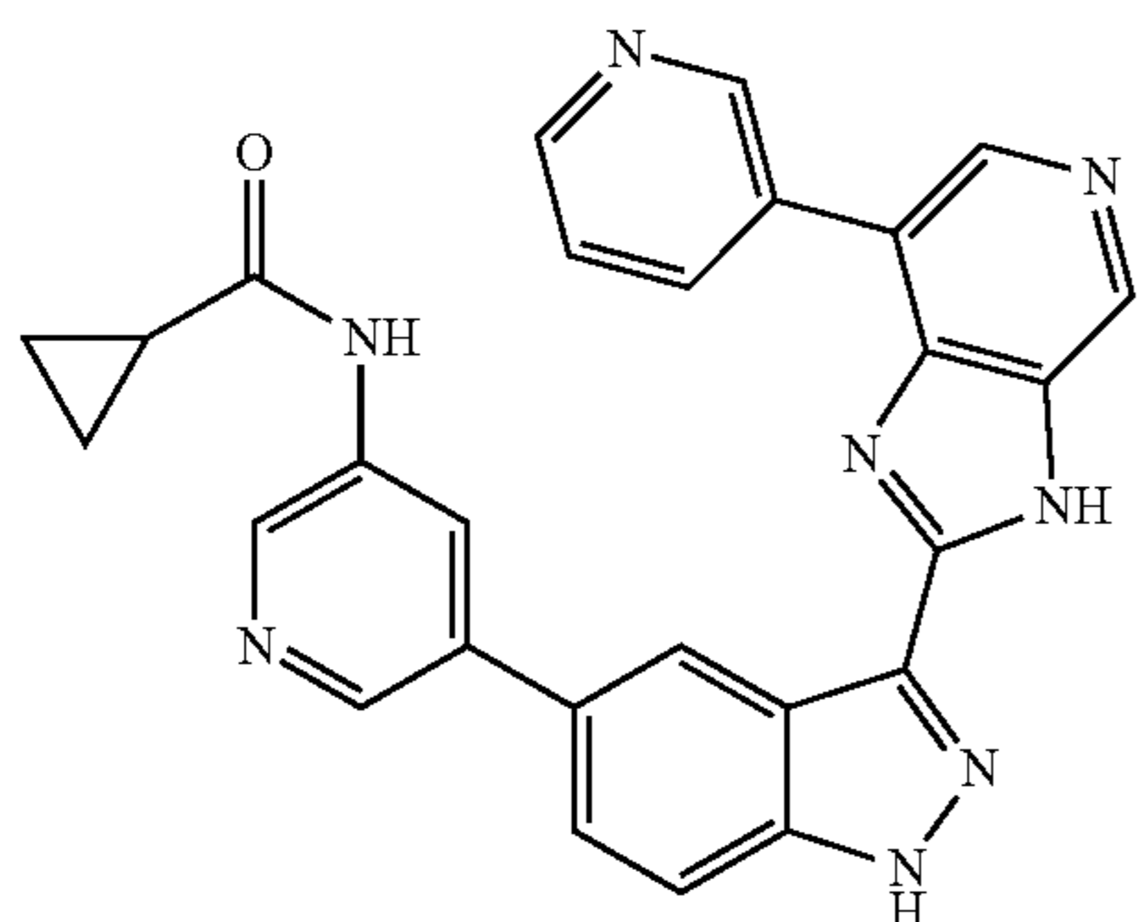
N-(5-(3-(7-(pyridin-3-yl)-3H-imidazo[4,5-c]pyridin-2-yl)-1H-indazol-5-yl)pyridin-3-yl)cyclopropanecarboxamide 12
