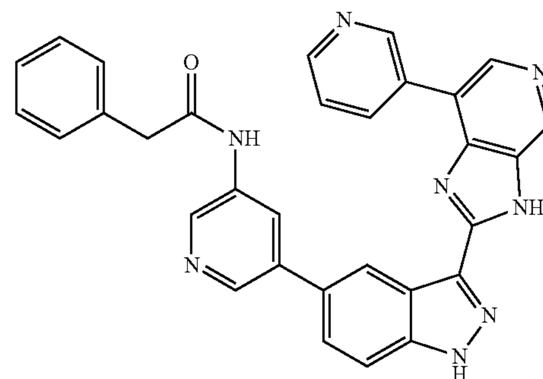
2-phenyl-N-(5-(3-(7-(pyridin-3-yl)-3H-imidazo[4,5-c]pyridin-2-yl)-1H-indazol-5-yl)pyridin-3-yl)acetamide 22
