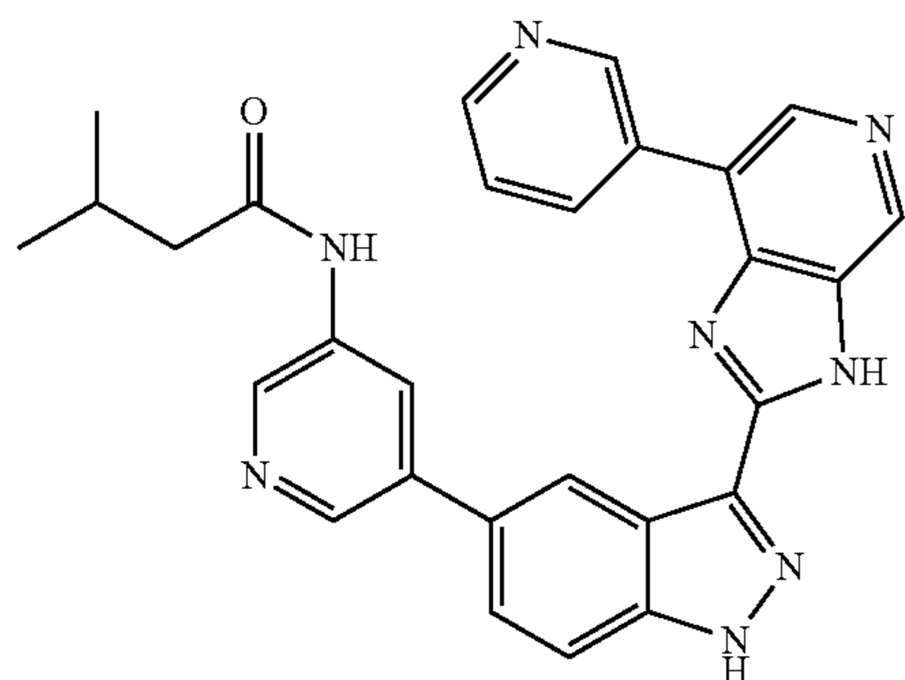
3-methyl-N-(5-(3-(7-(pyridin-3-yl)-3H-imidazo[4,5-c]pyridin-2-yl)-1H-indazol-5-yl)pyridin-3-yl)butanamide 15
