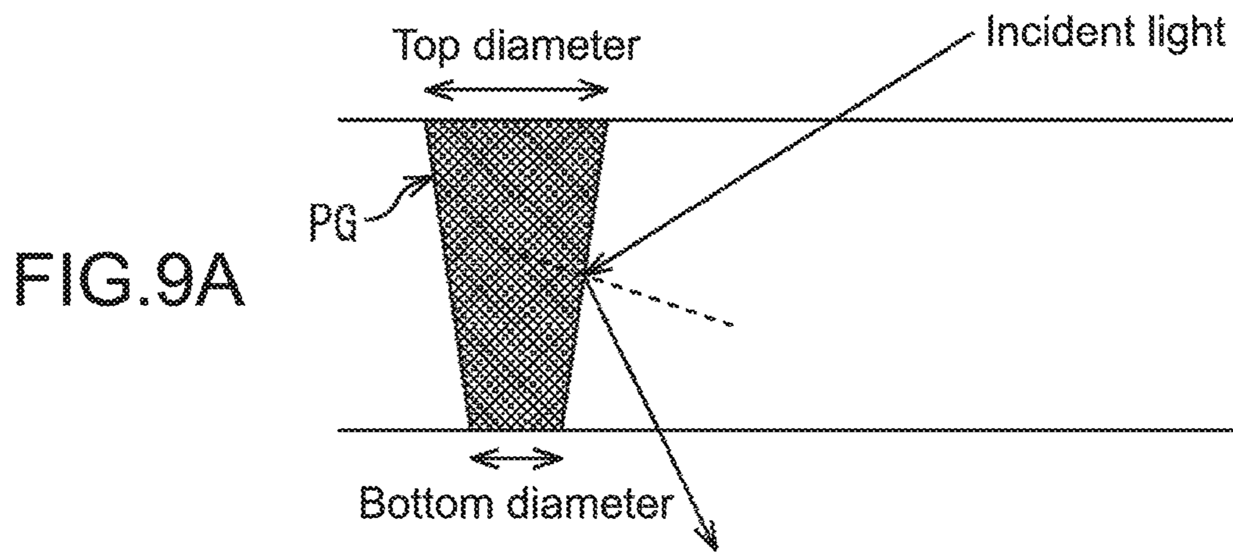
Forward taper (top diameter > bottom diameter)
