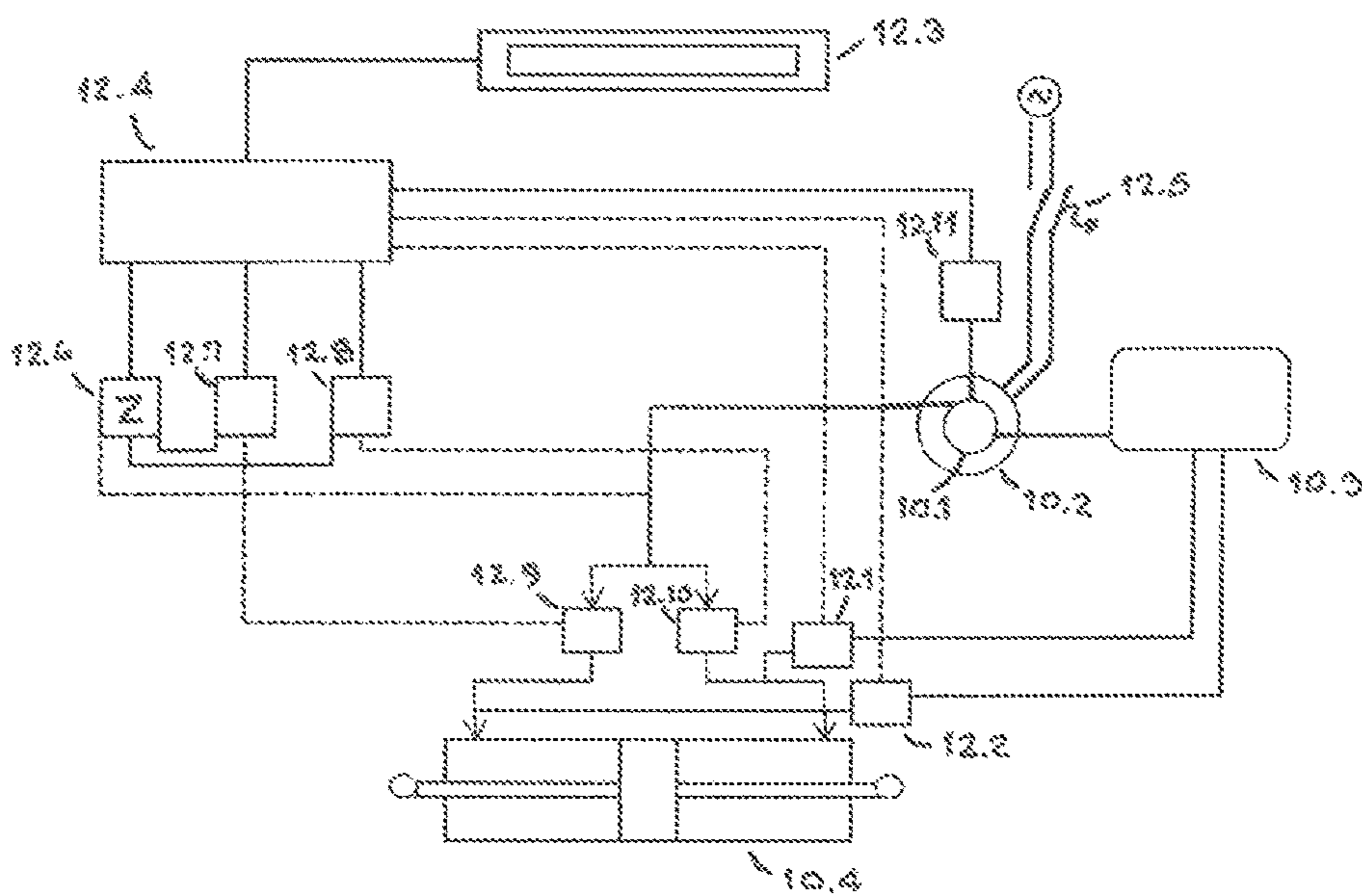
FIG 12. DIAGRAM OF CONNECTION OF THE CONTROL ELEMENTS FOR THE HYDRAULIC OPTION
