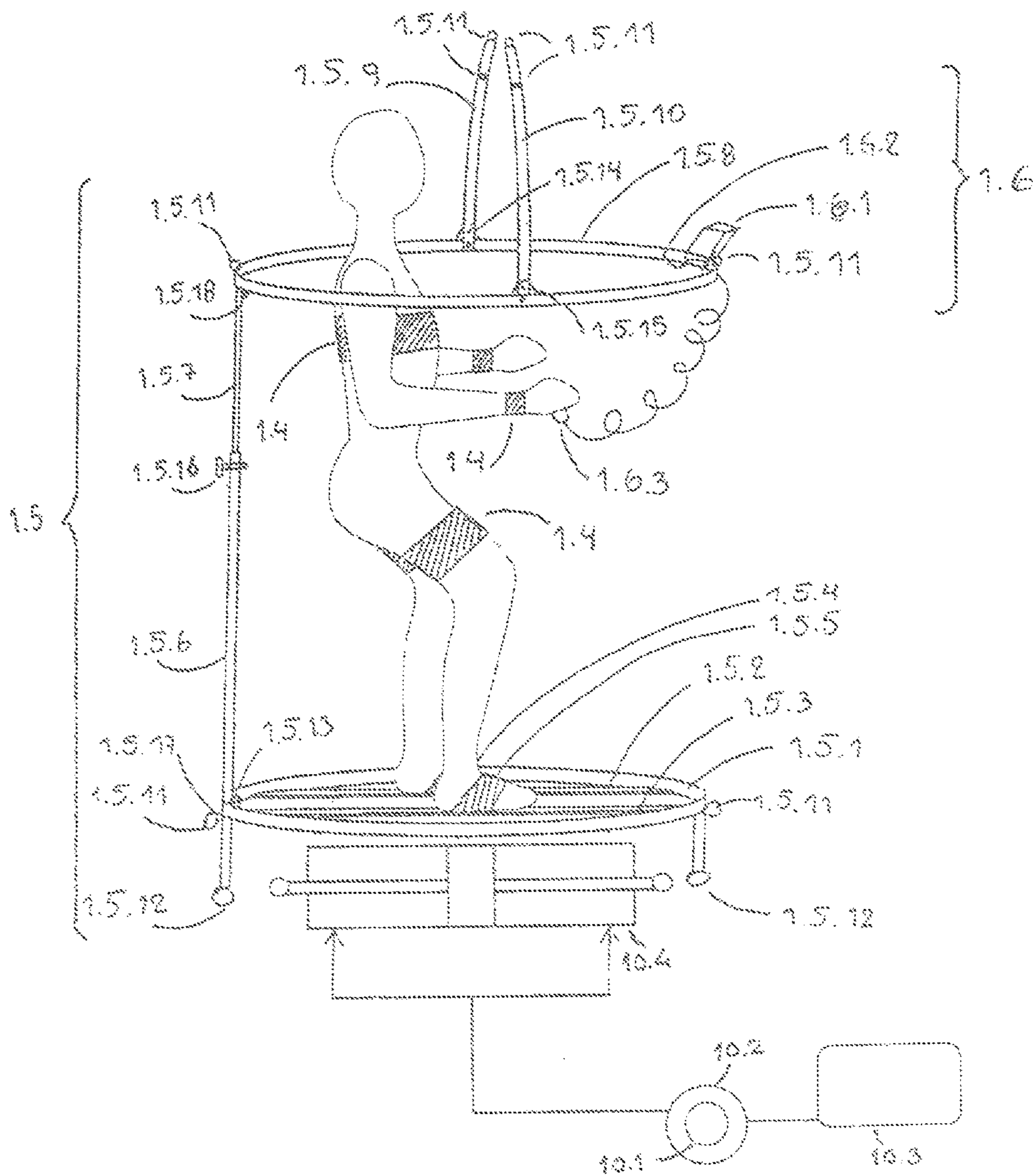
FIG 10. THE MIDSYR ACTUATED BY A HYDRAULIC PUMP
