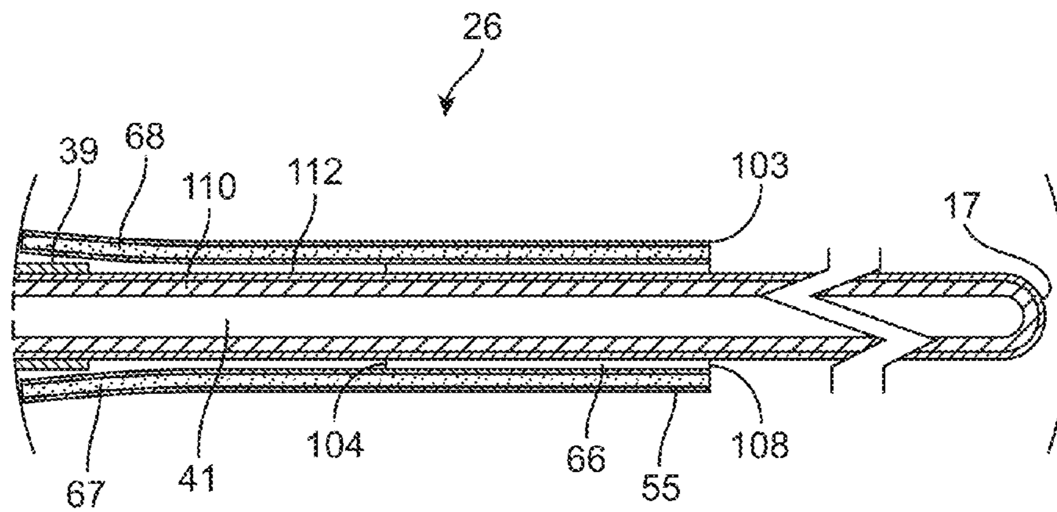
SECTION B-B ROTATED 90°
