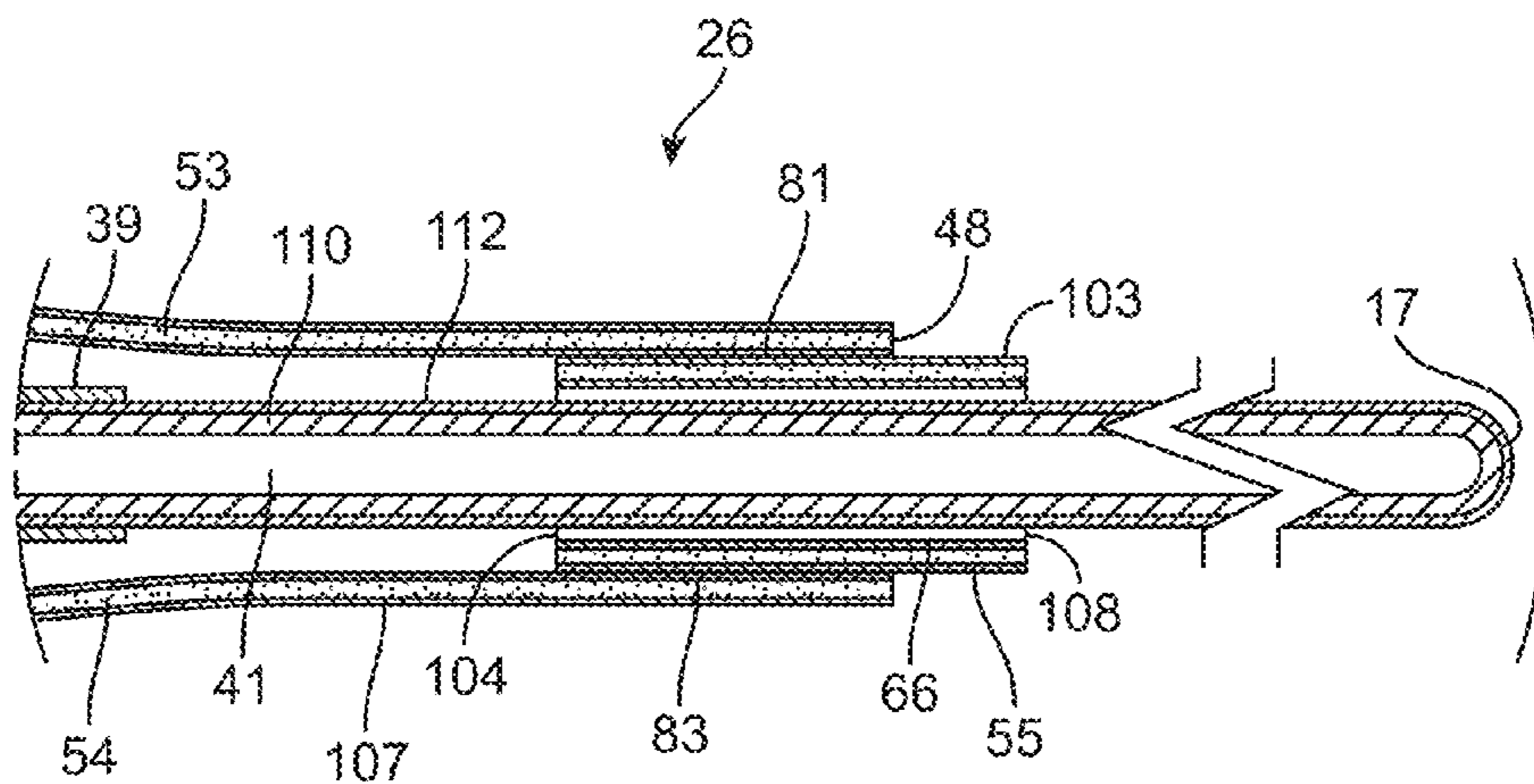
SECTION B-B
