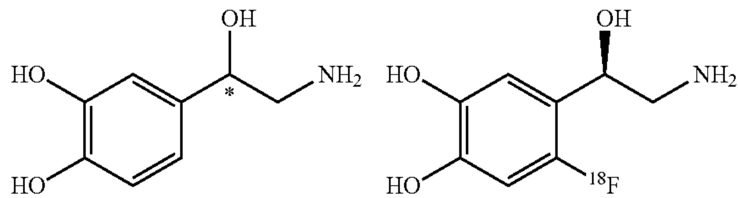
[ 11 C]Norepinephrine (NE)
