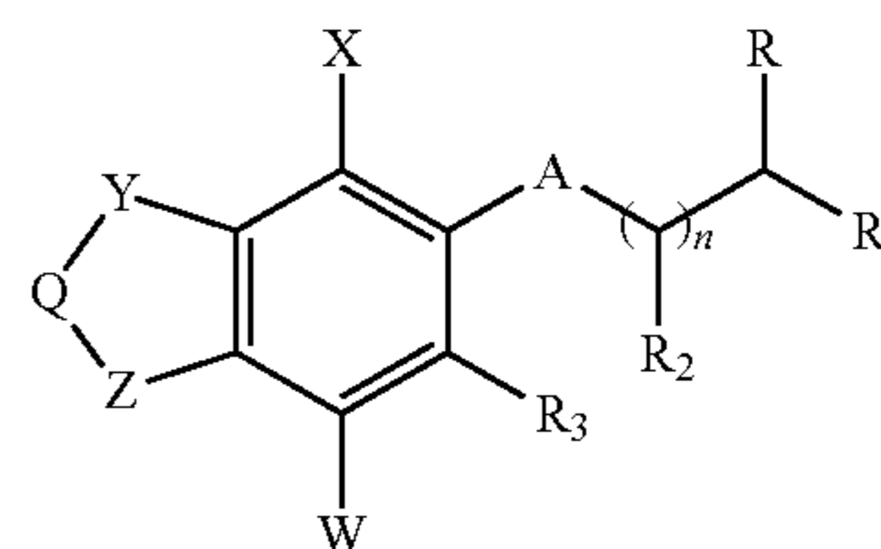
Structure Beta
