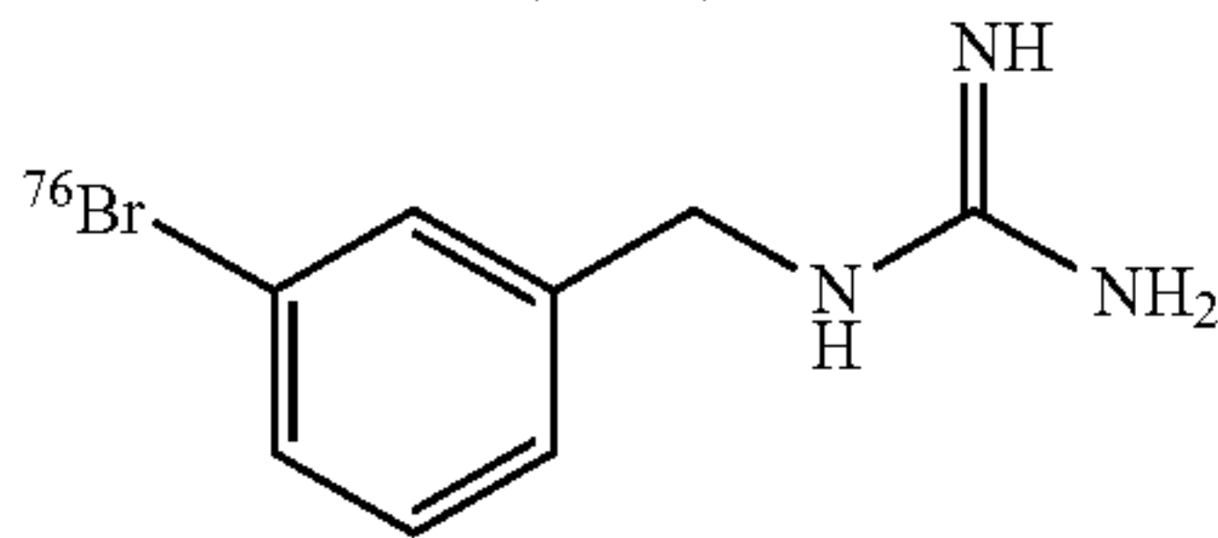
[ ^{76}\text{Br} ]-m-Bromobenzylguanidine (MBBG)
