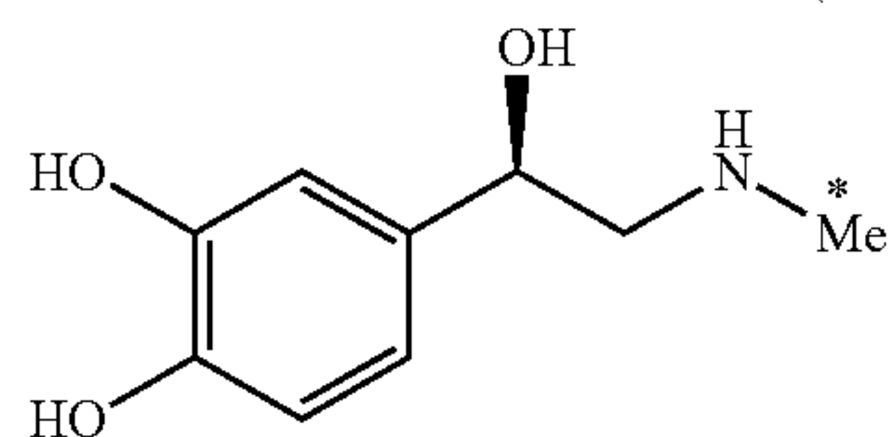
[ 11 C]Epinephrine (EPI)
