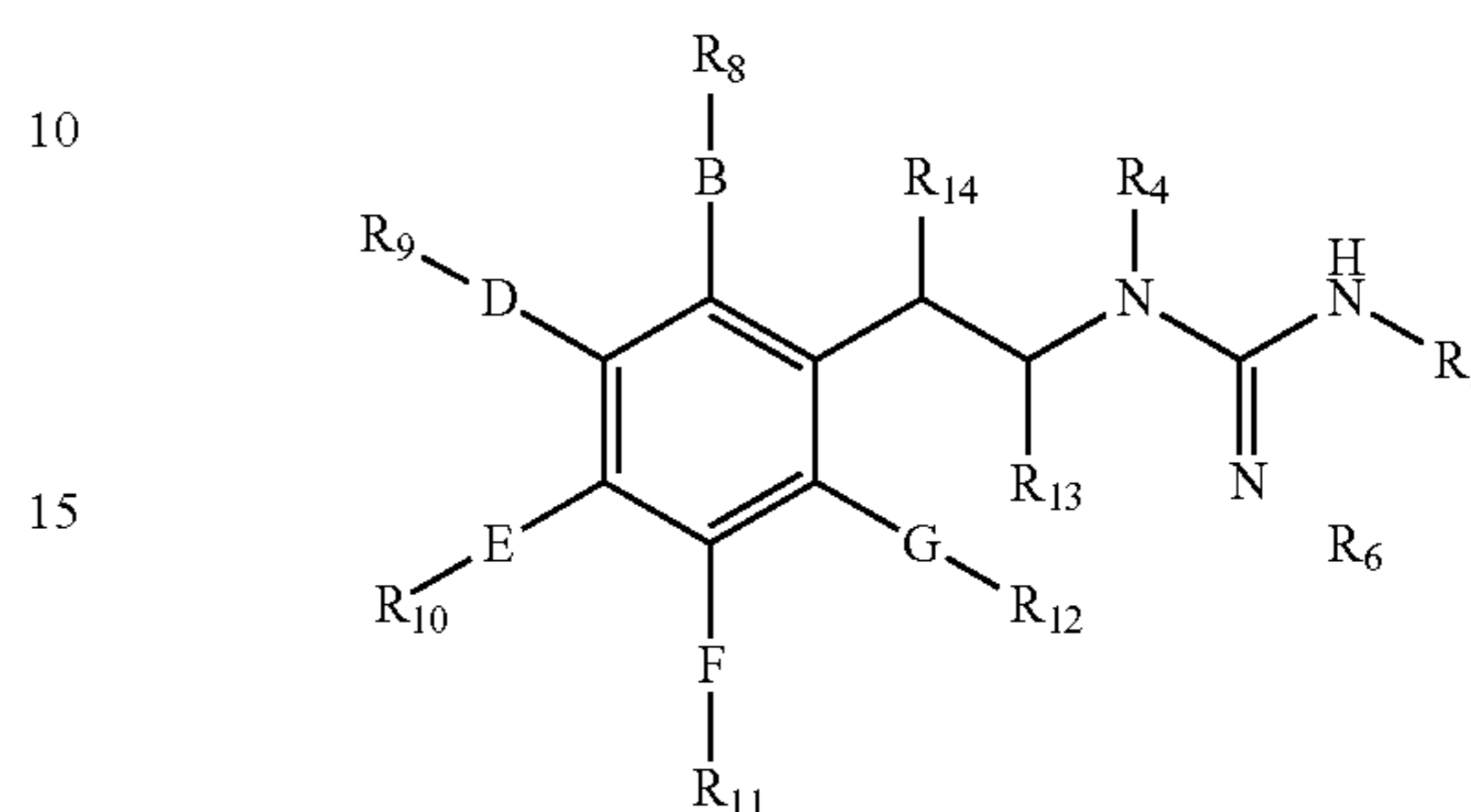
Structure Delta
