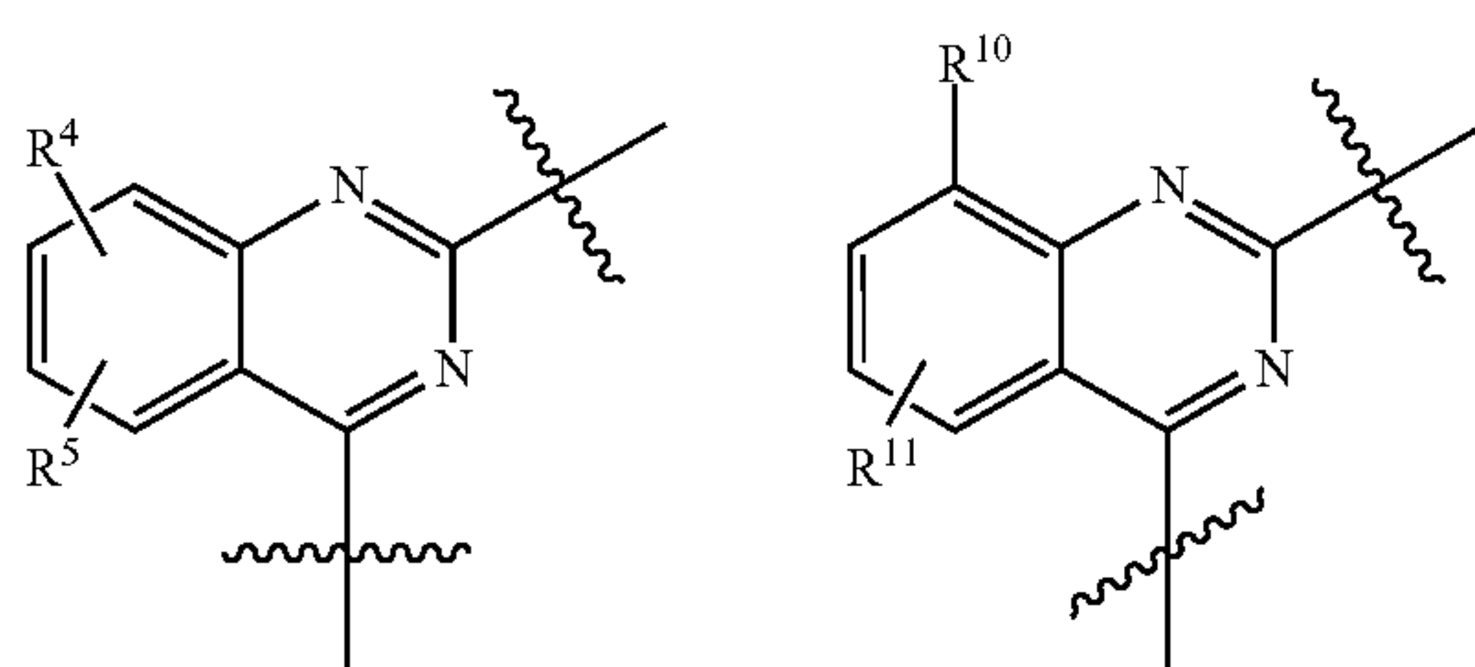
Quinazoline Scaffolds
