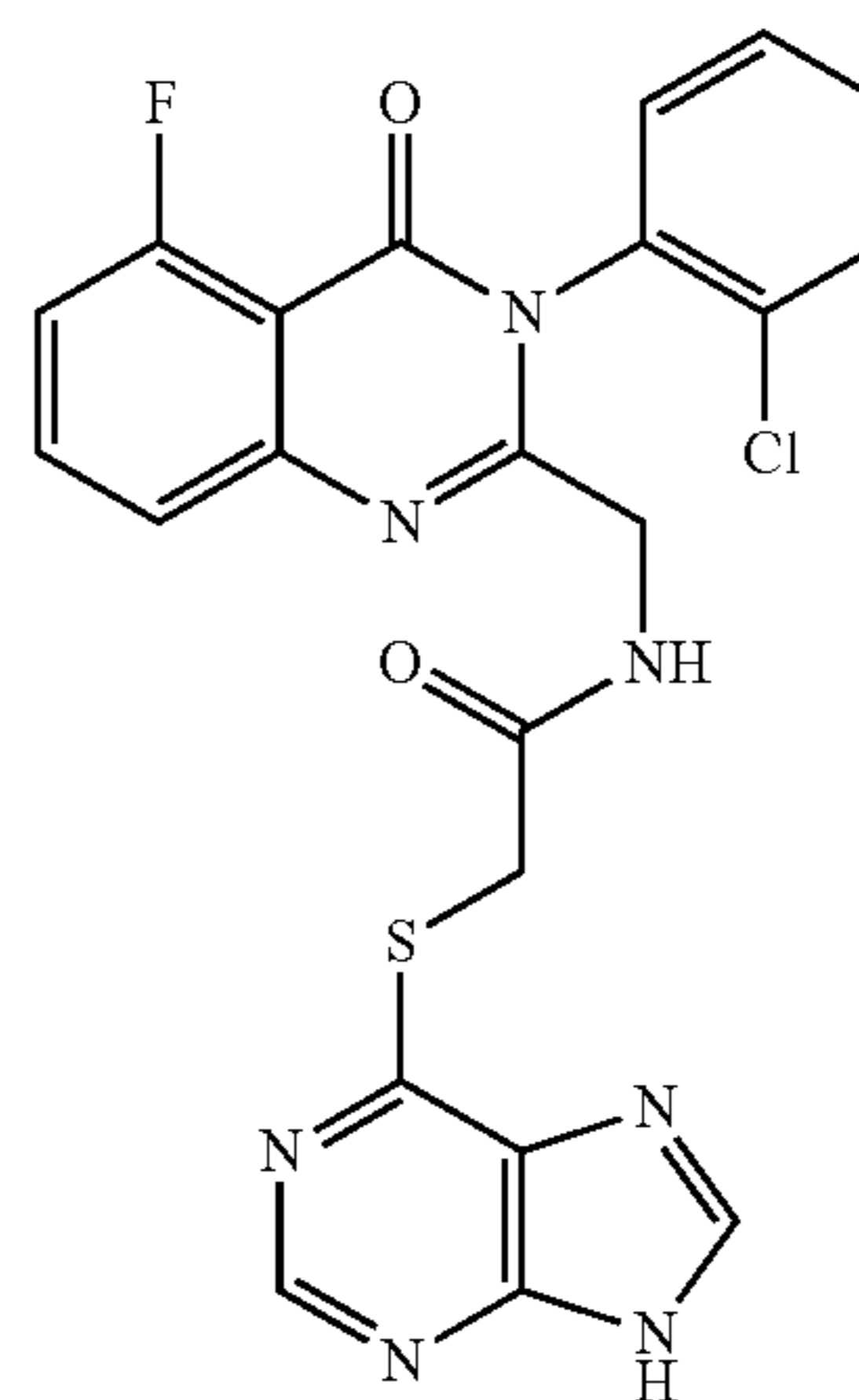
N-[3-(2-Chlorophenyl)-5-fluoro-4-oxo-3,4-dihydro-quinazolin-2-ylmethyl]-2-(9H-purin-6-ylsulfanyl)-acetamide (D-077)
