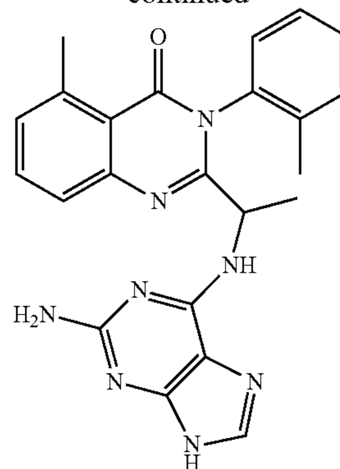
2-(1-(2-Amino-9H-purin-6-ylamino)ethyl)-5-methyl-3-o-tolyl-3H-quinazolin-4-one (D-081a)
