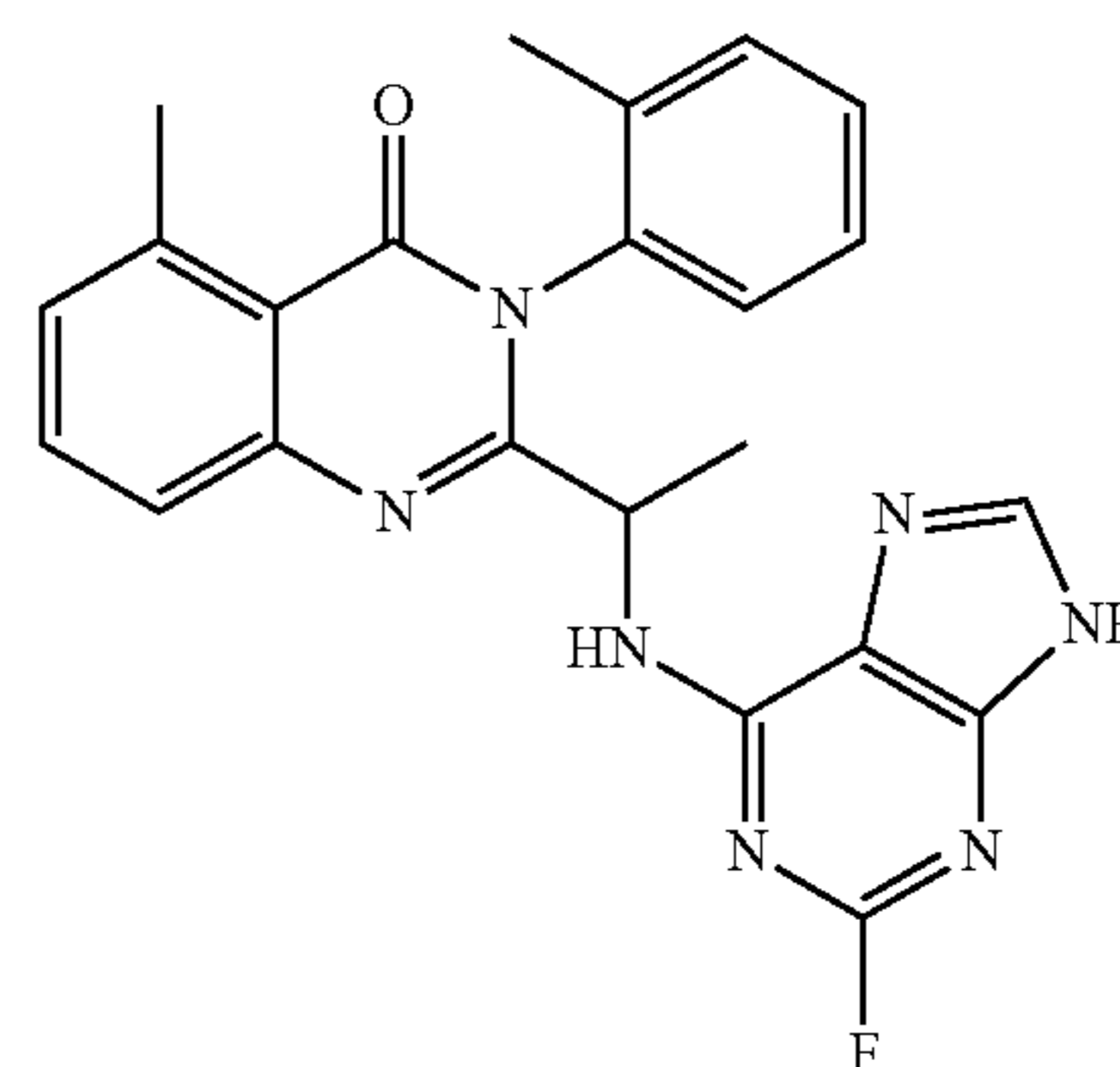
2-[1-(2-Fluoro-9H-purin-6-ylamino)ethyl]-5-methyl-3-o-tolyl-3H-quinazolin-4-one (D-080)
