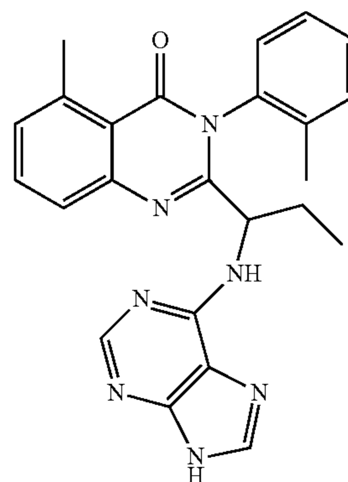
5-Methyl-2-(1-(9H-purin-6-ylamino)propyl)-3-o-tolyl-3H-quinazolin-4-one (D-081b)
