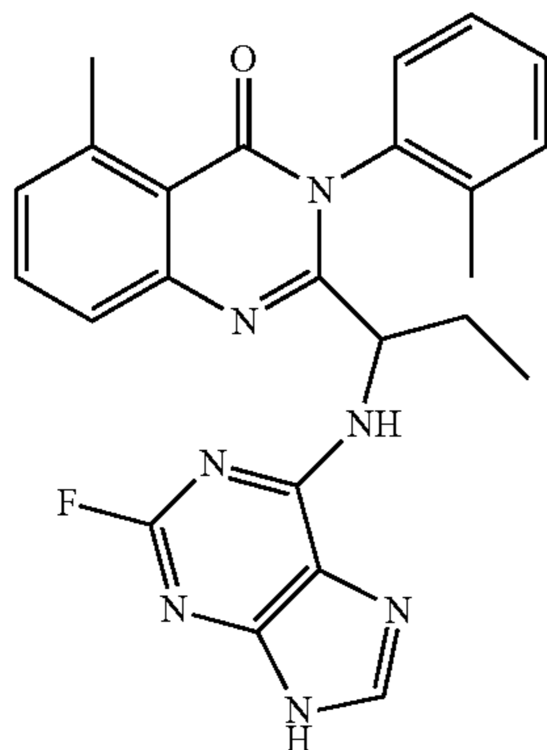
2-(1-(2-Fluoro-9H-purin-6-ylamino)propyl)-5-methyl-3-o-tolyl-3H-quinazolin-4-one (D-081c)
