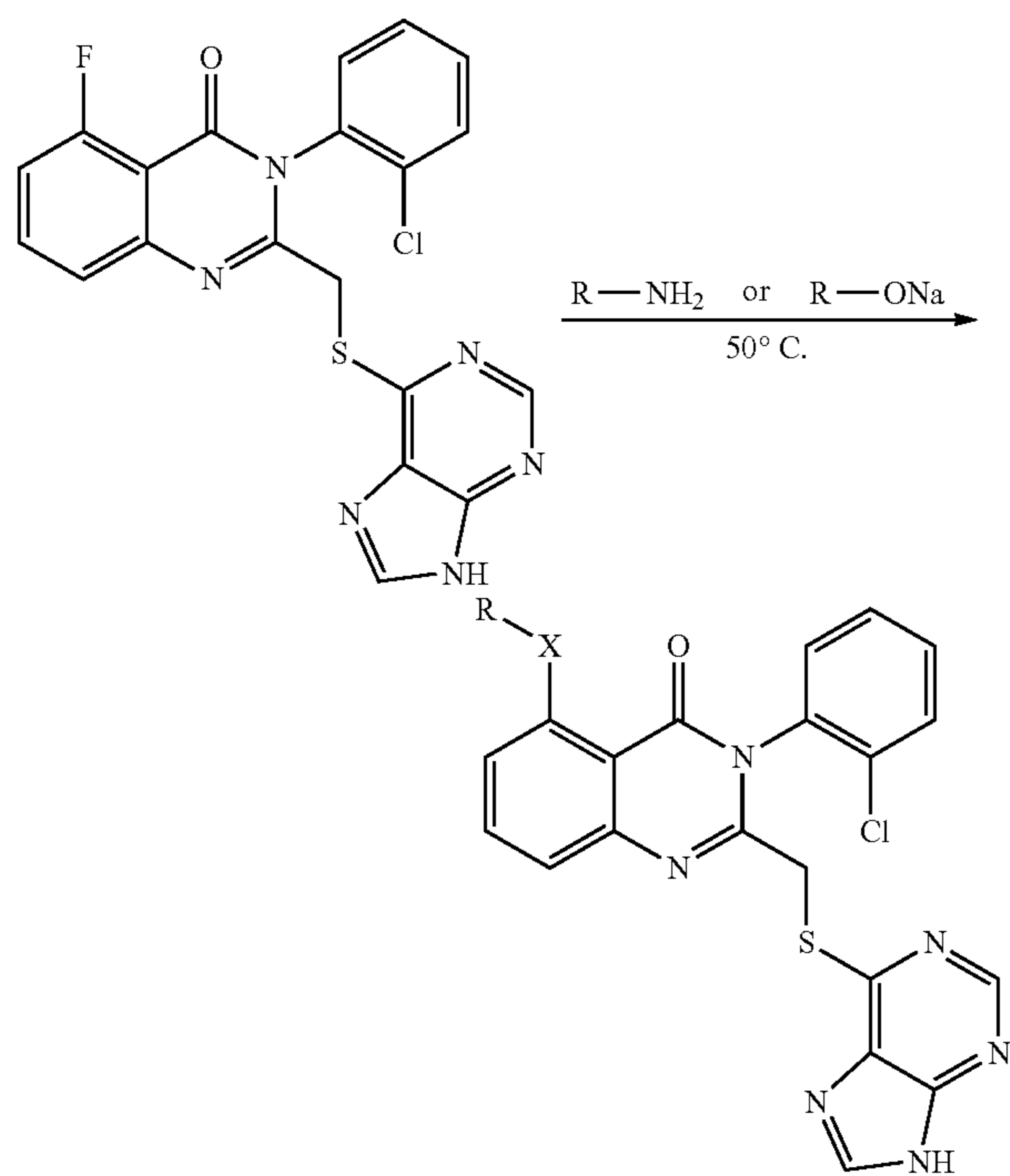
3-(2-Chlorophenyl)-5-methoxy-2-(9H-purin-6-ylsulfanylmethyl)-3H-quinazolin-4-one (D-116)
