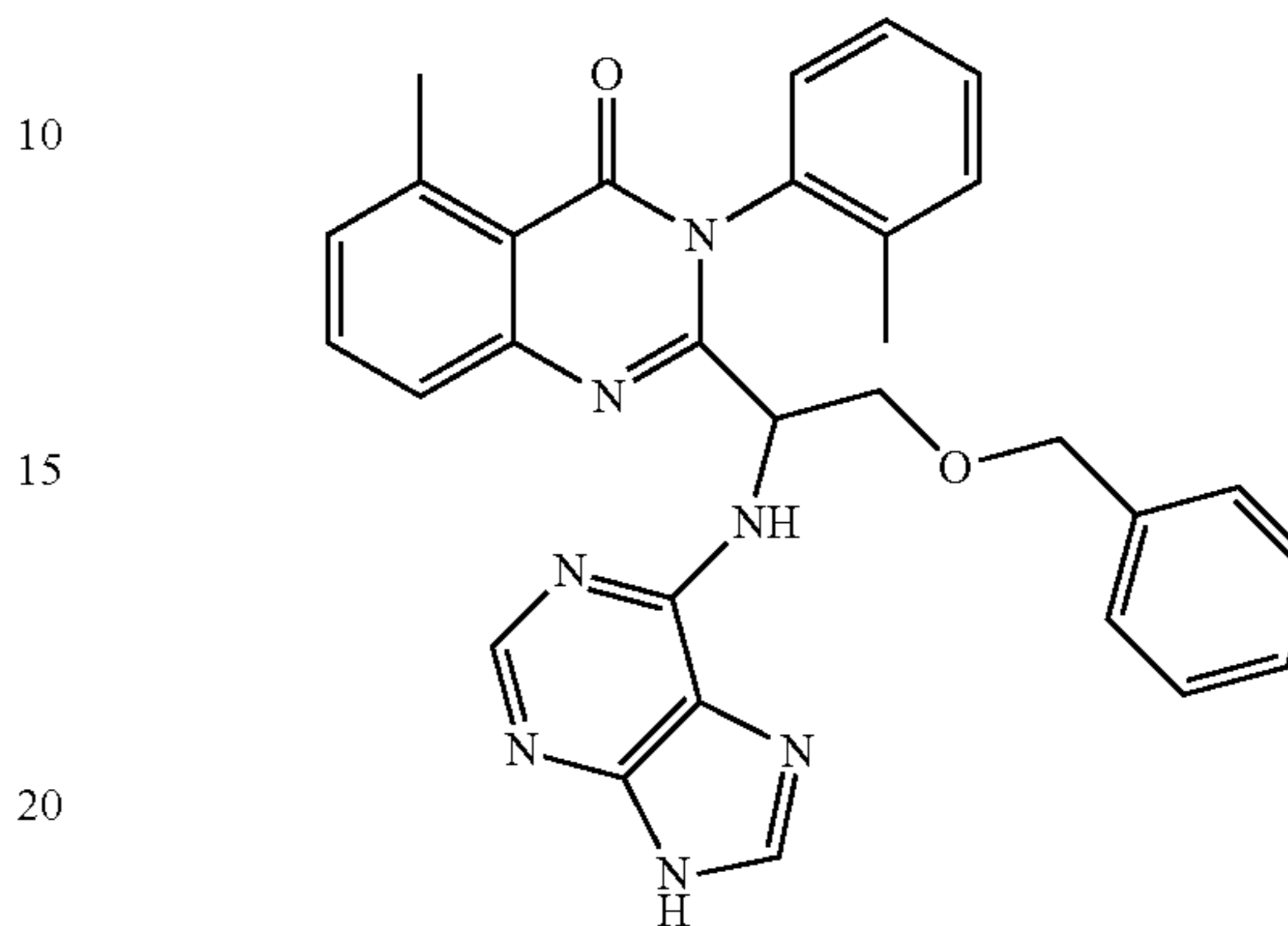
2-[2-Benzyloxy-1-(9H-purin-6-ylamino)ethyl]-5-methyl-3-o-tolyl-3H-quinazolin-4-one (D-081e)
