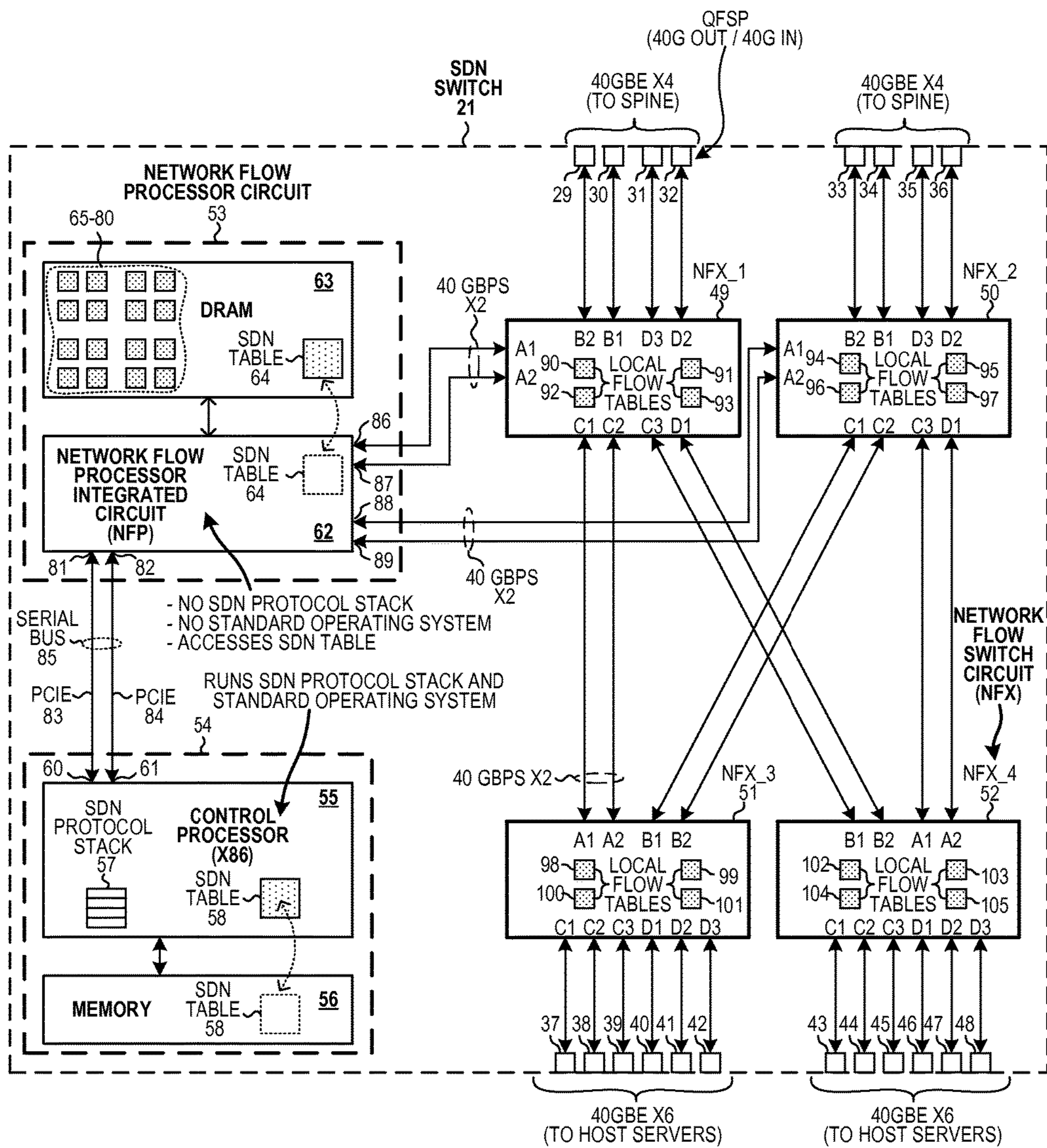
SDN SWITCH (TOP-OF-RACK) FIG. 5
