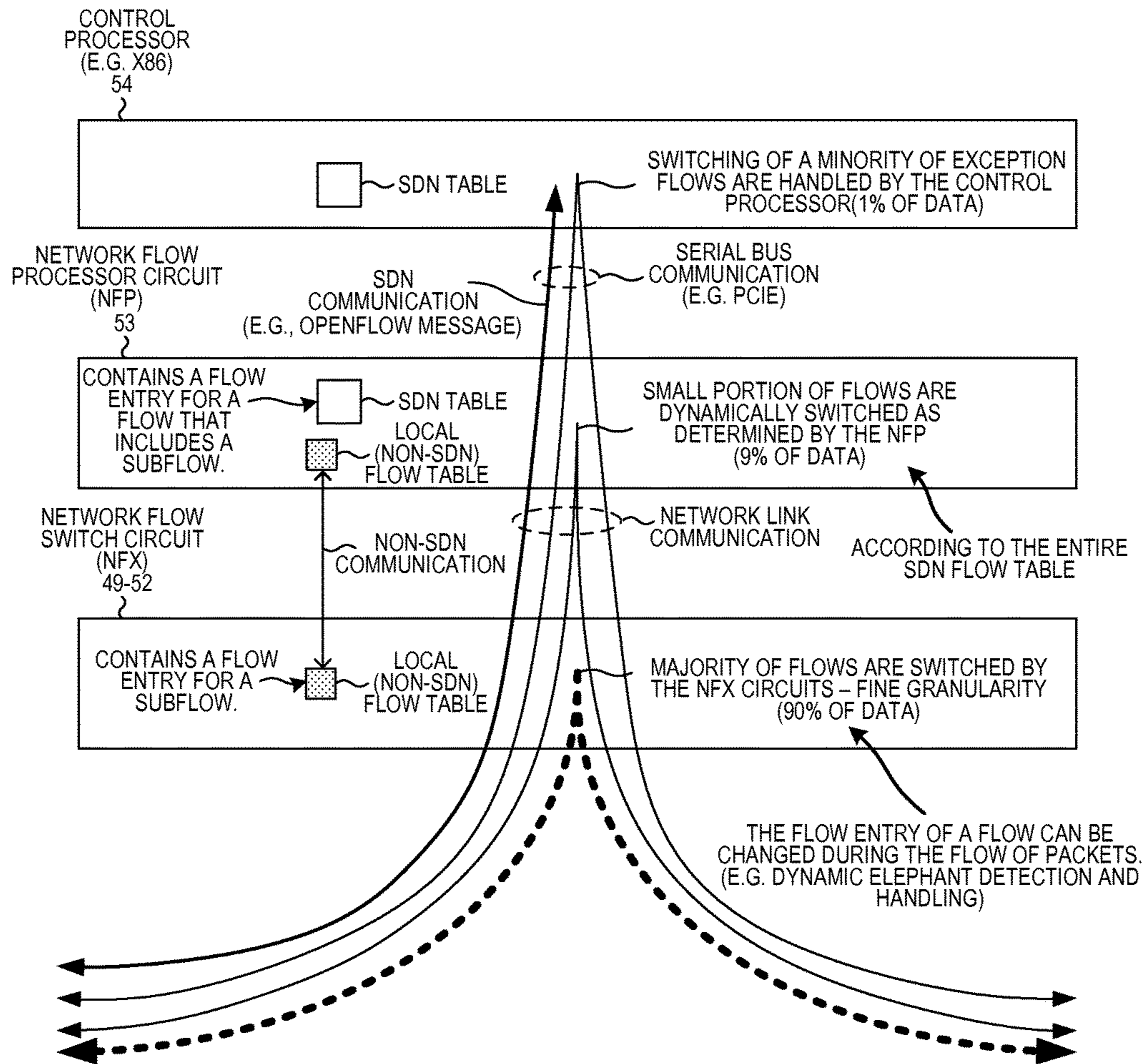
IMPROVED OPERATION WITH NFX ARCHITECTURE FIG. 16
