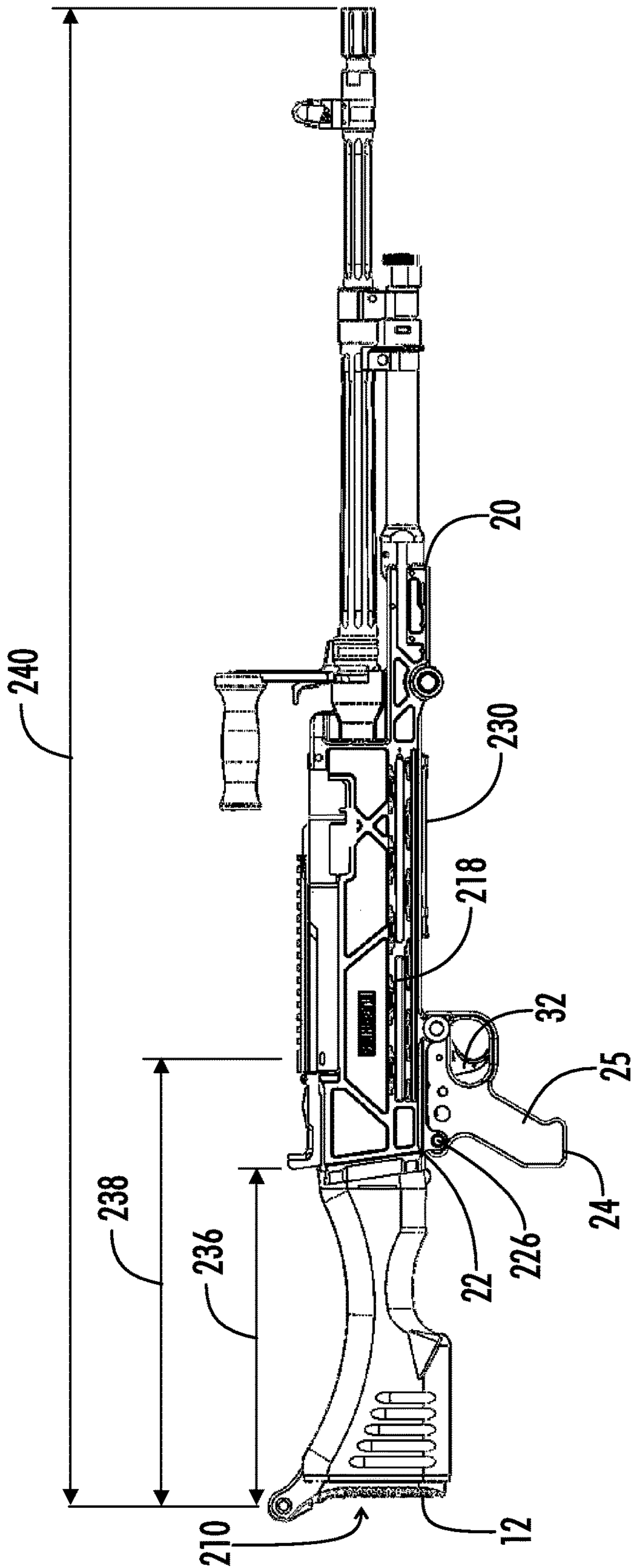
FIG. 8 (PRIOR ART)
