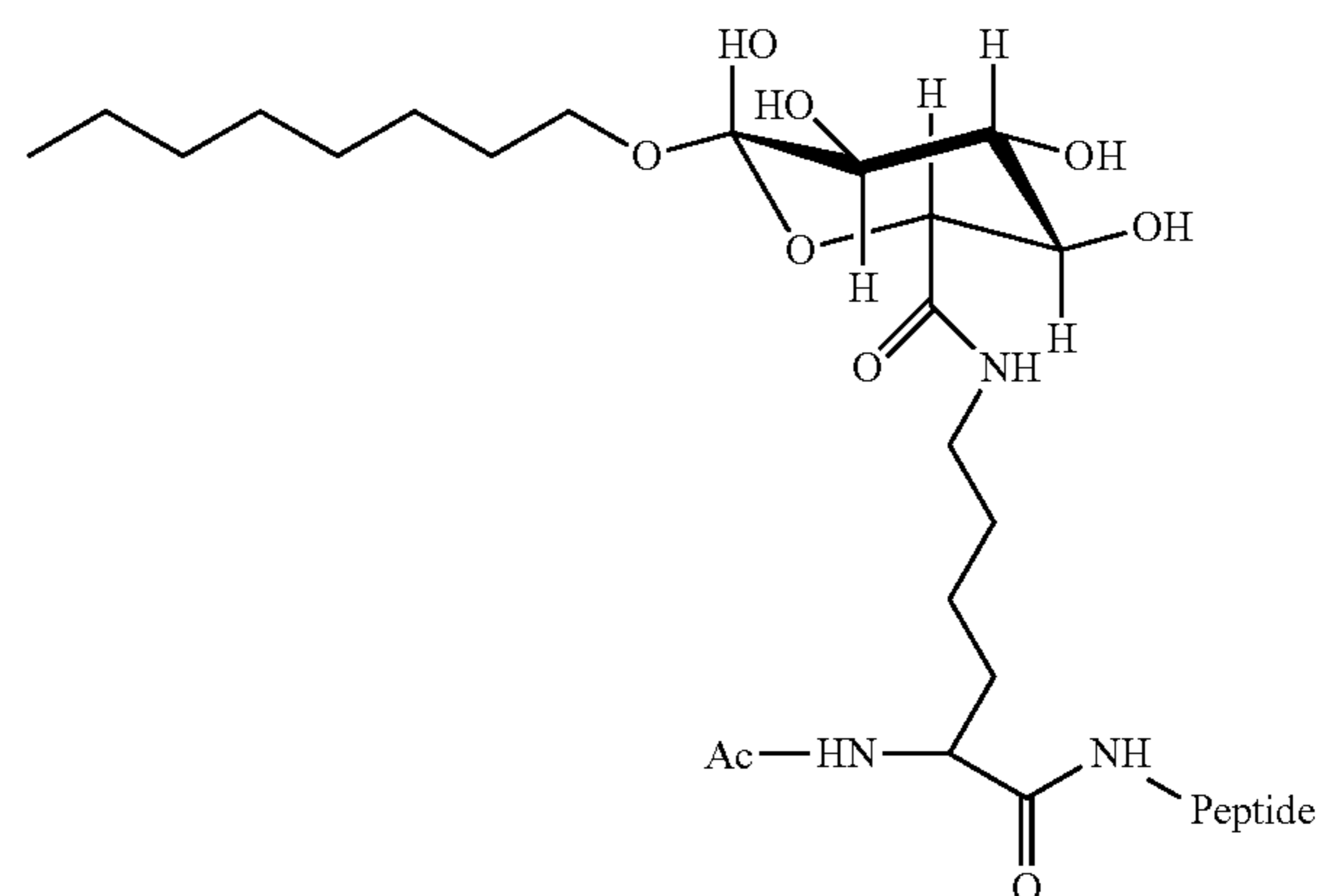
Scheme 5. Illustrative example of a peptide intermediate.
