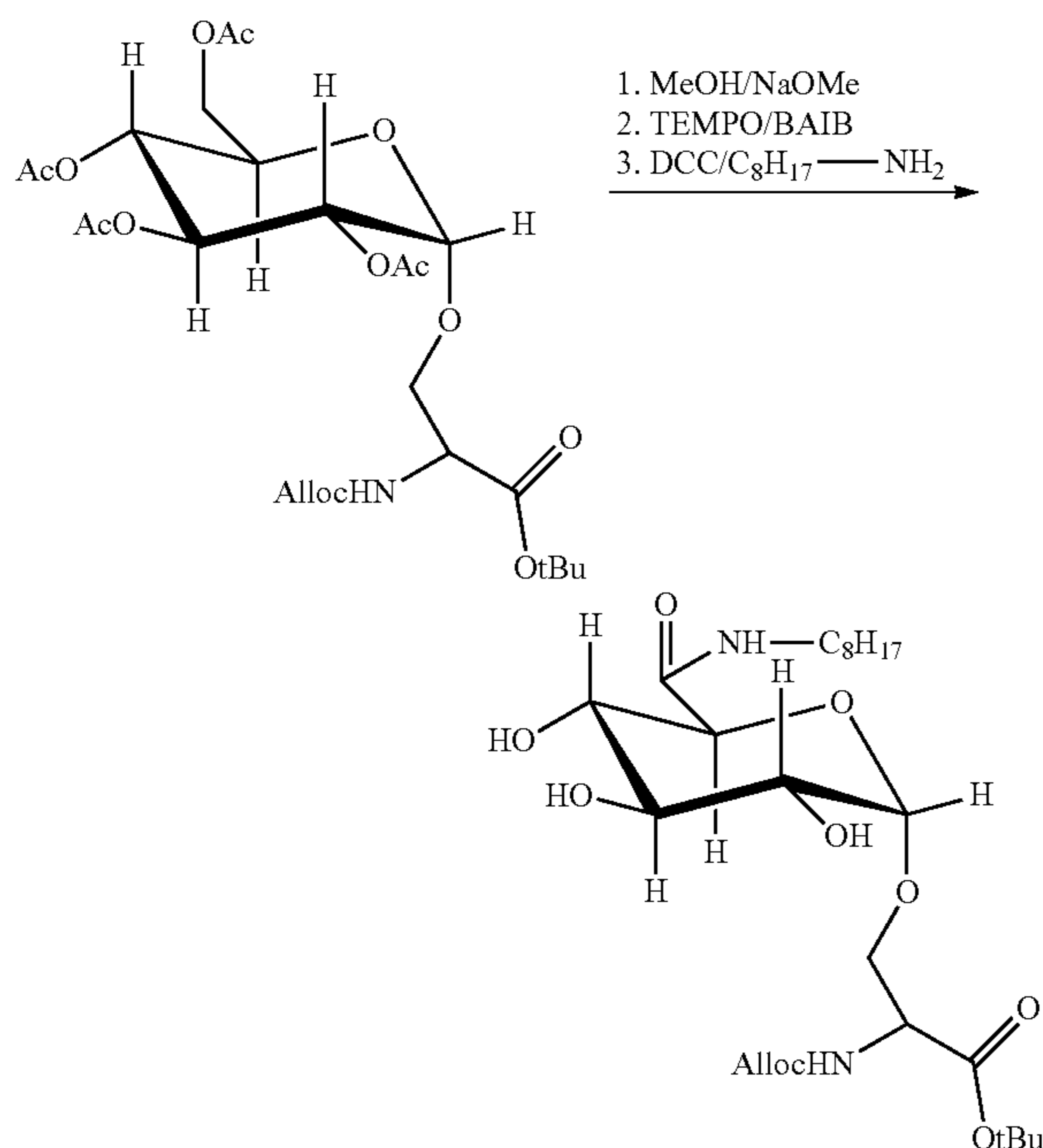
Scheme 7. Alternative example of nonionic surfactant reagent.
