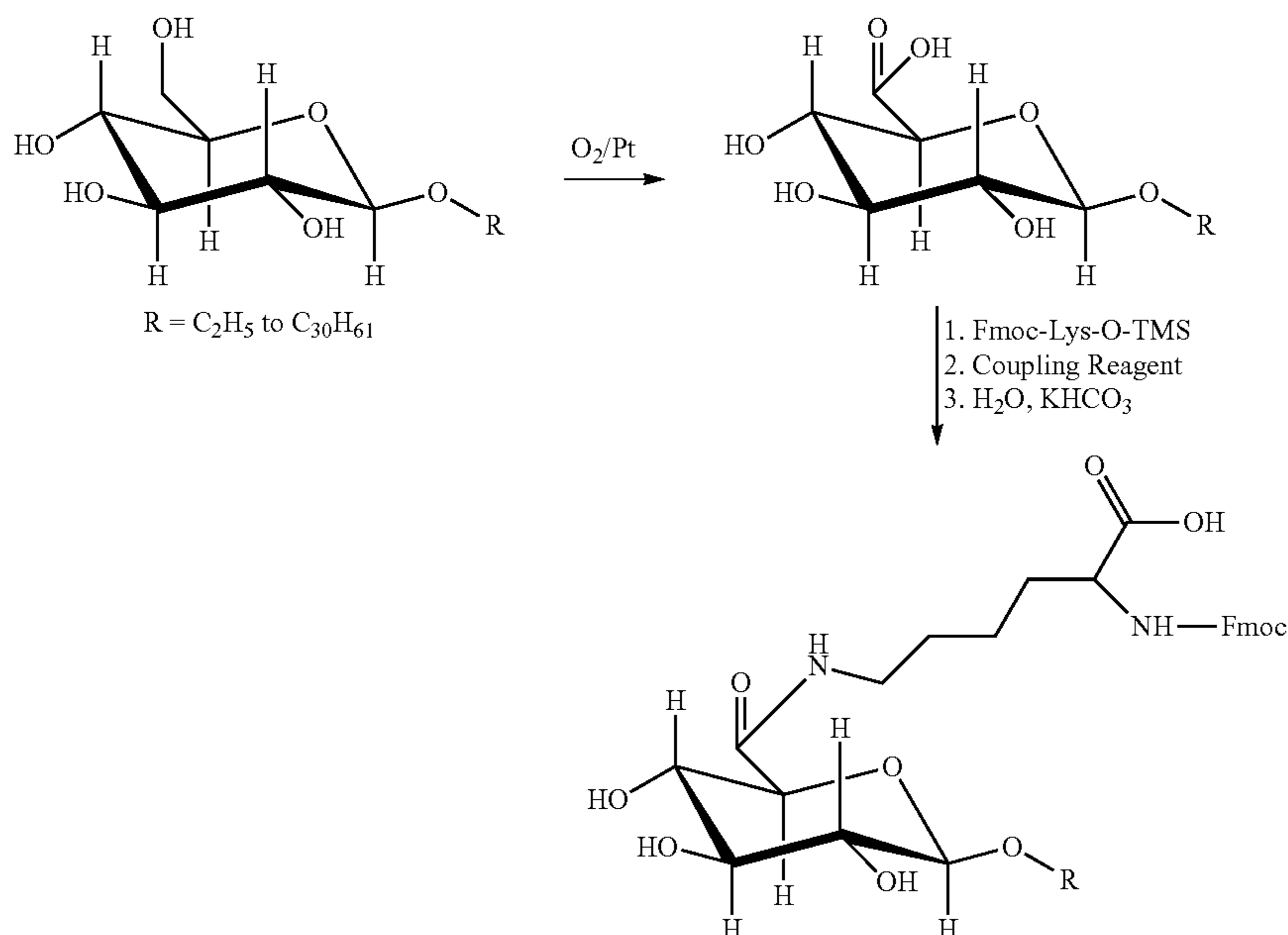
Scheme 4. Example of a preparation of a reagent
