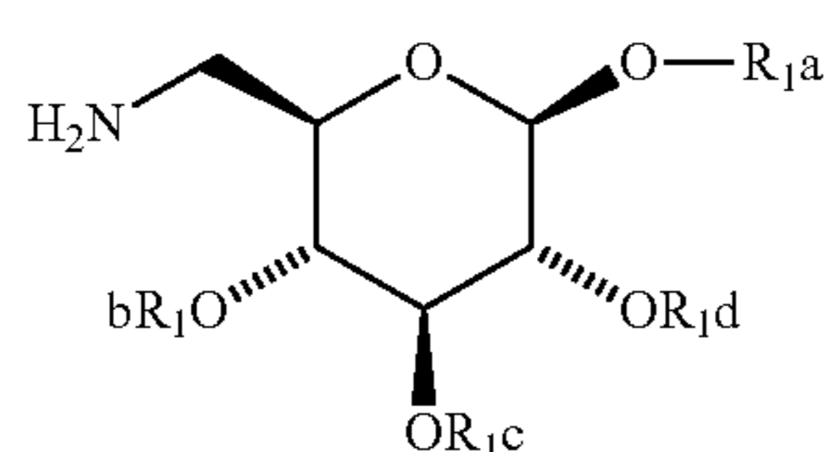
Scheme 6. Additional reagent examples.
