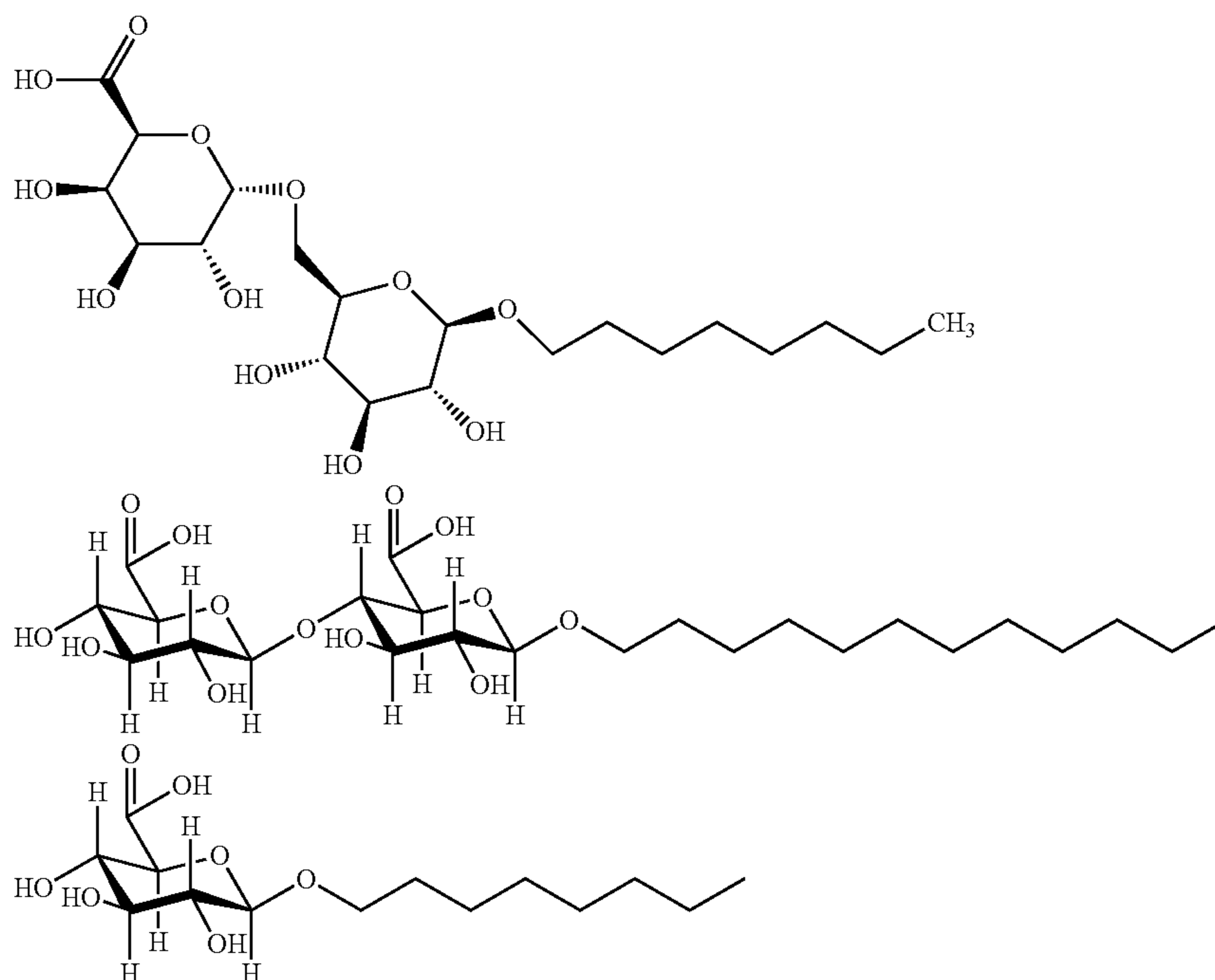
Scheme 2. Examples of alkyl melibiouronic, diglucuronic and glucuronic acid class reagents.
