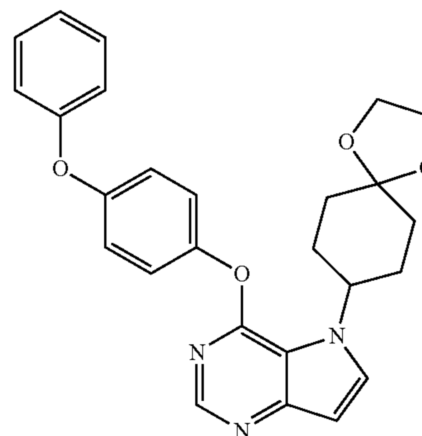
5-[1,4-dioxaspiro[4.5]decan-8-yl]-4-(4-phenoxyphenoxy)-5H-pyrrolo[3,2-d]pyrimidine
