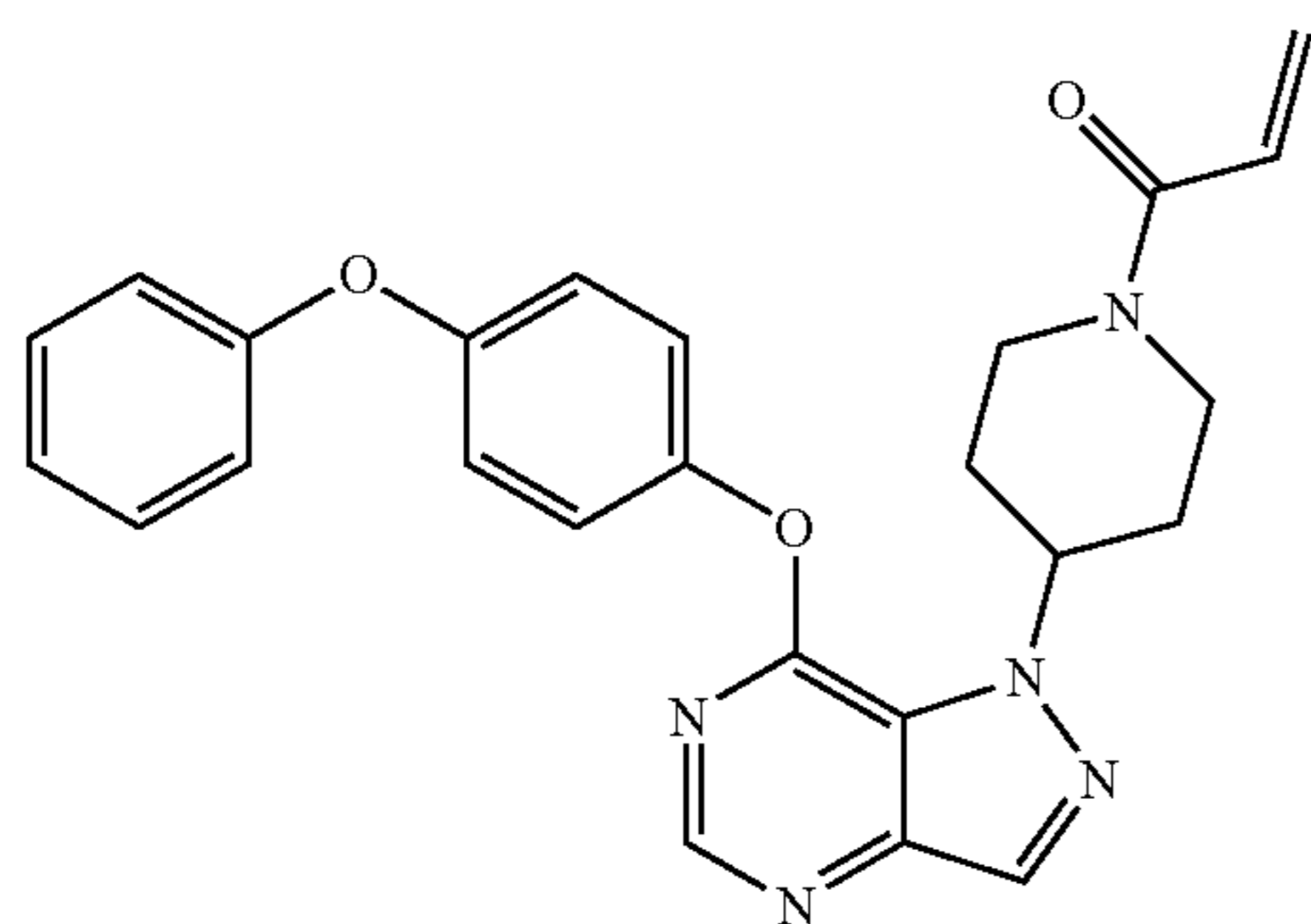
1-(4-(7-(4-phenoxyphenoxy)-1H-pyrazolo[4,3-d]pyrimidin-1-yl)piperidin-1-yl)prop-2-en-1-one (12) (Method M)
