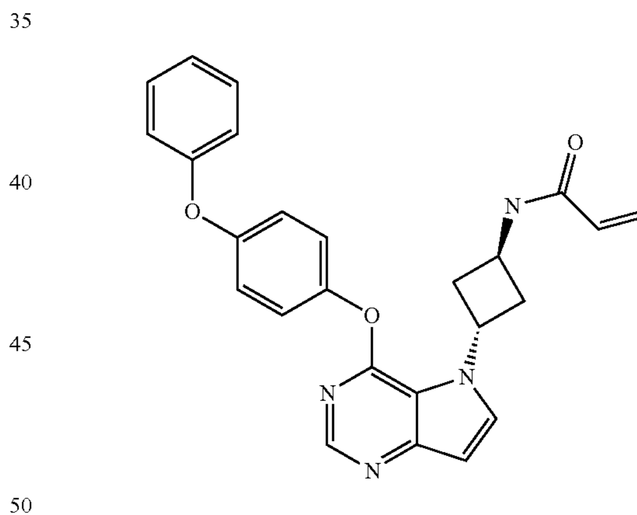
N-(trans-3-(4-(4-phenoxyphenoxy)-5H-pyrrolo[3,2-d]pyrimidin-5-yl)cyclobutyl)acrylamide (8)
