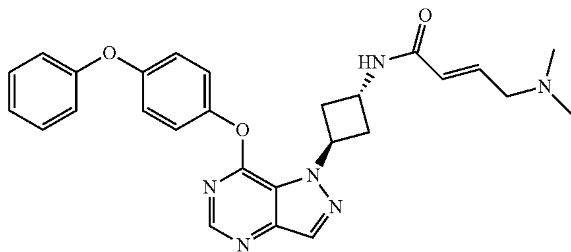
(E)-4-(dimethylamino)-N-((1r,3r)-3-(7-(4-phenoxyphenoxy)-1H-pyrazolo[4,3-d]pyrimidin-1-yl)cyclobutyl)but-2-enamide (41)
