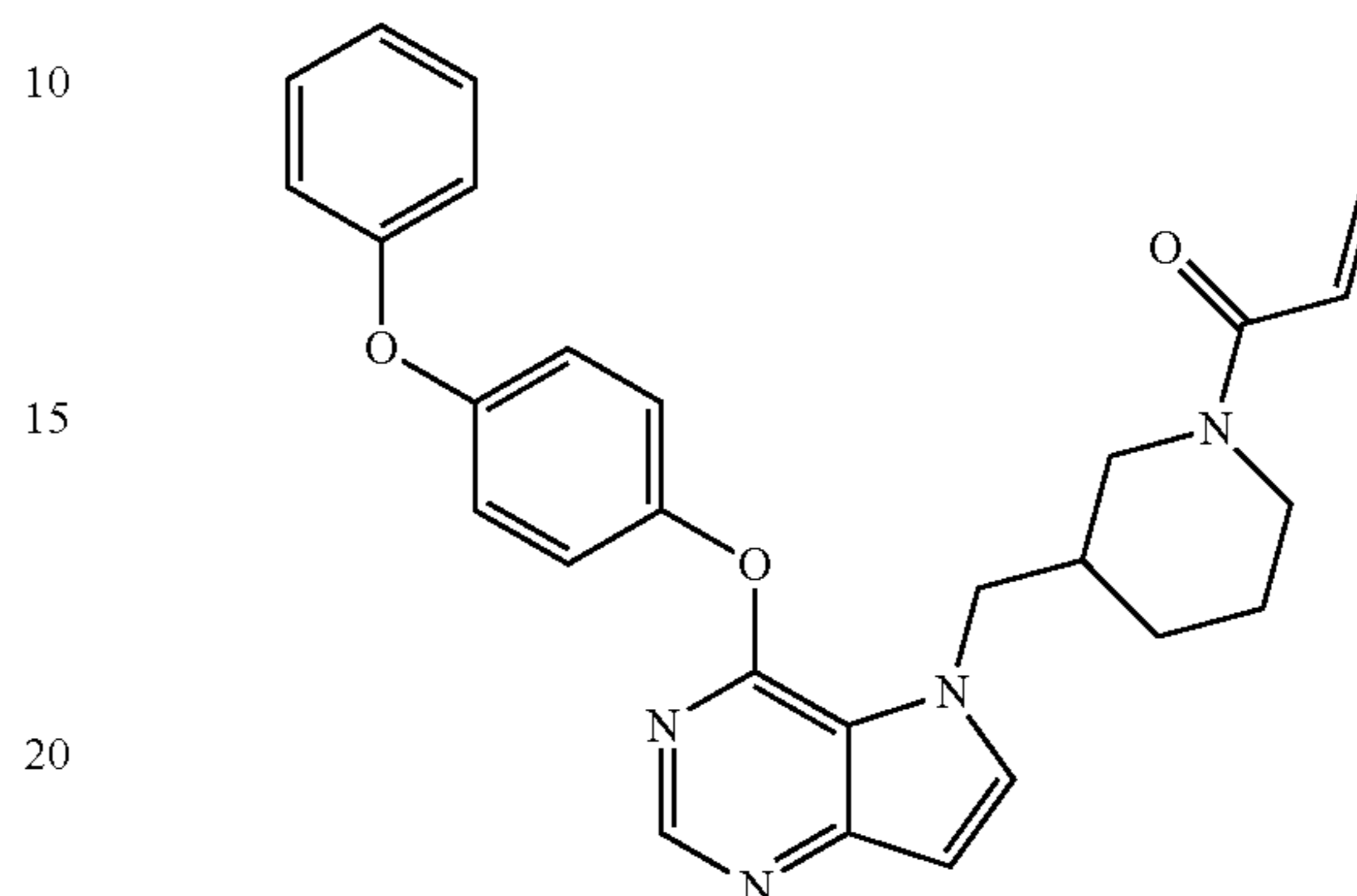
1-(3-((4-(4-phenoxyphenoxy)-5H-pyrrolo[3,2-d]pyrimidin-5-yl)methyl)piperidin-1-yl)prop-2-en-1-one (15)
