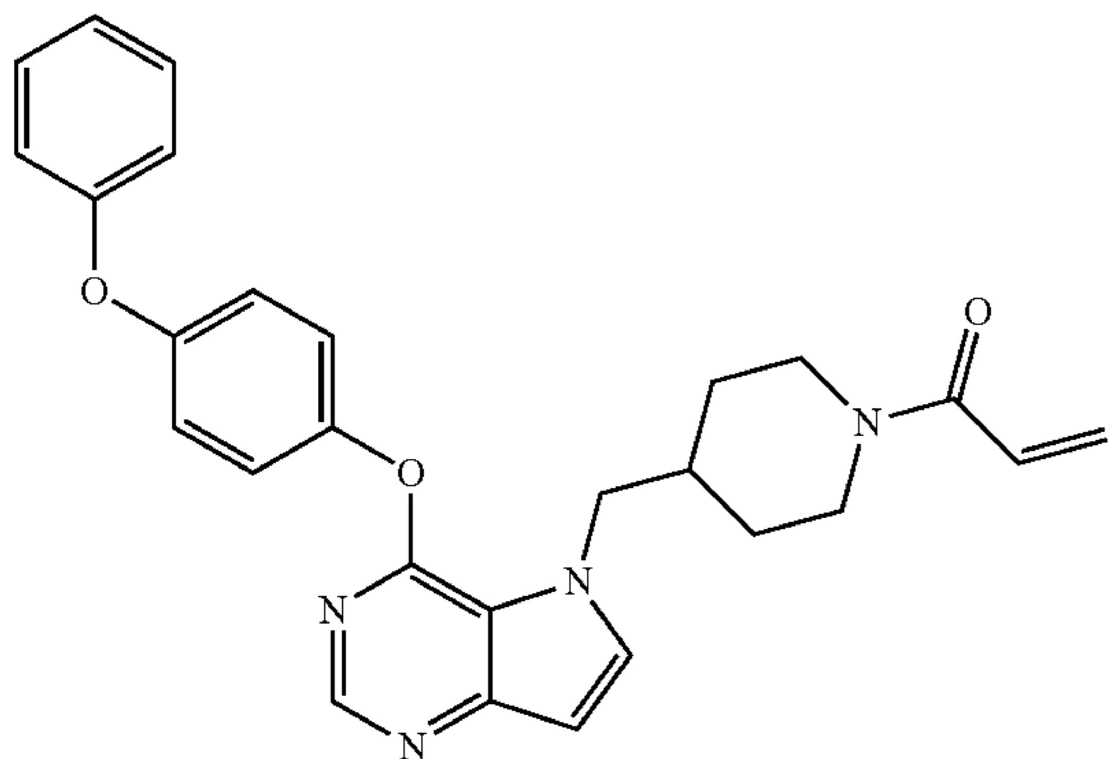
1-(4-((4-(4-phenoxyphenoxy)-5H-pyrrolo[3,2-d]pyrimidin-5-yl)methyl)piperidin-1-yl)prop-2-en-1-one (37)
