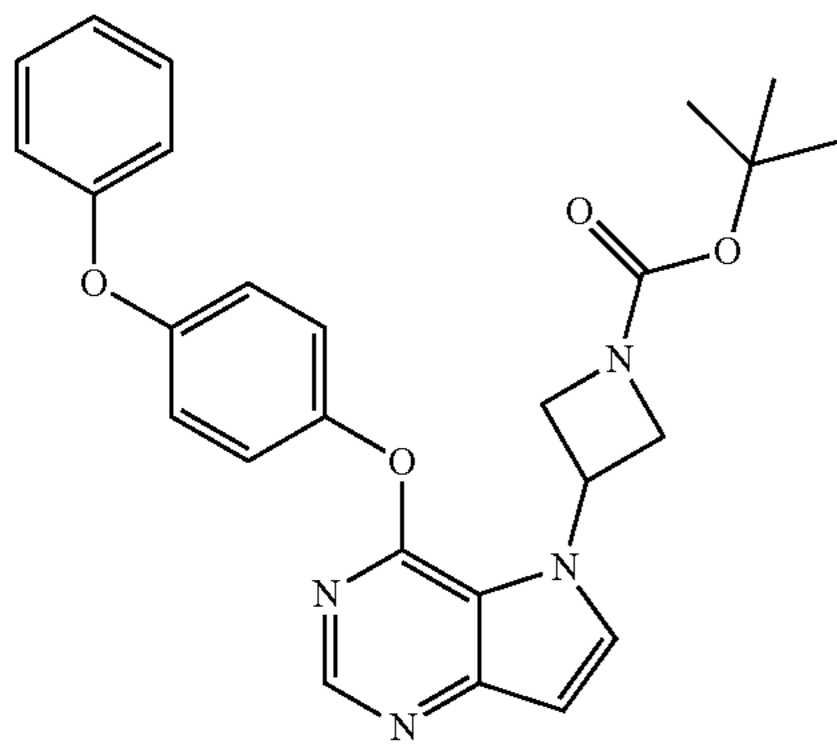
tert-butyl 3-(4-(4-phenoxyphenoxy)-5H-pyrrolo[3,2-d]pyrimidin-5-yl)azetidine-1-carboxylate (Method C)
