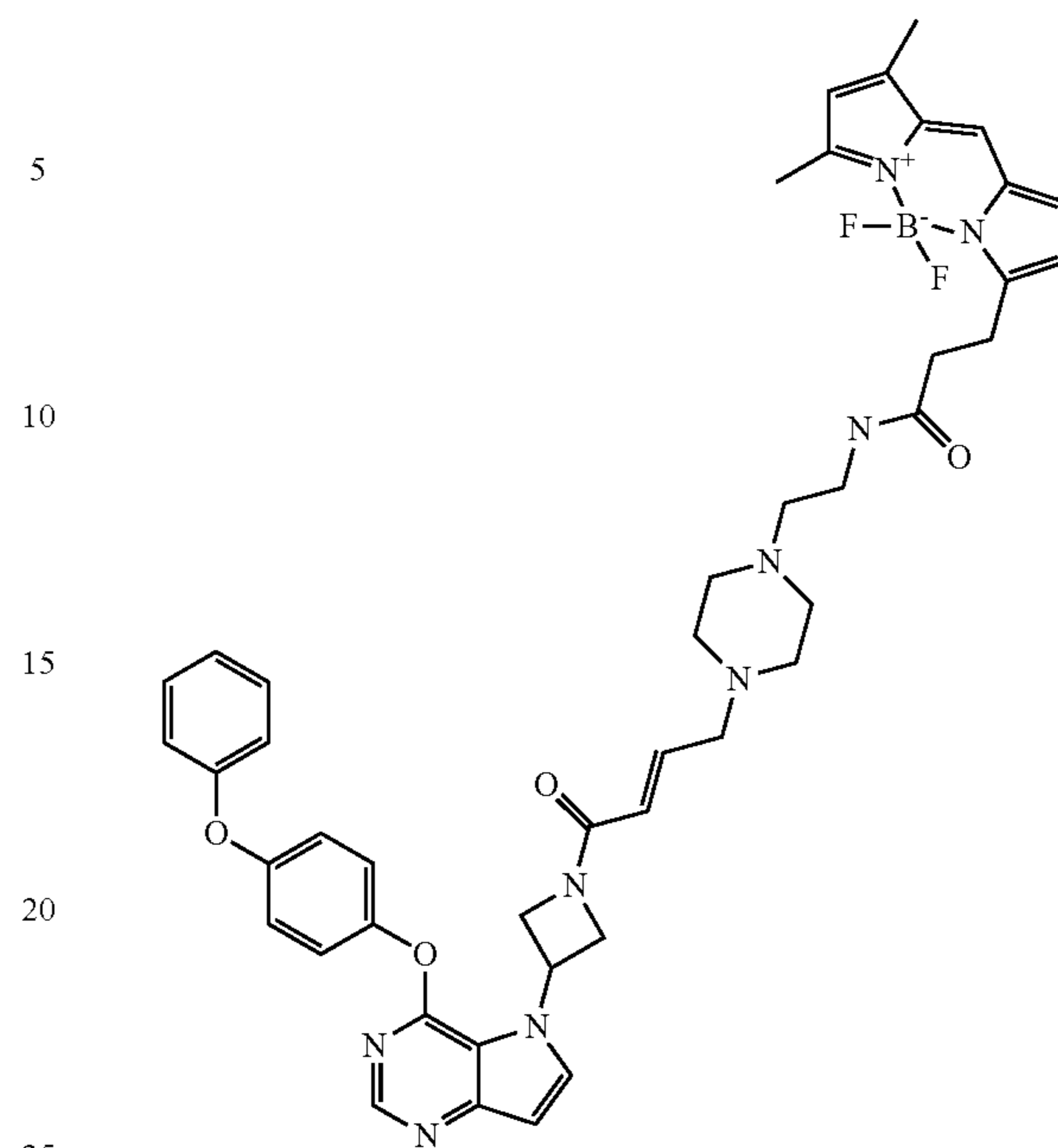
(E)-5,5-difluoro-1,3-dimethyl-7-(3-oxo-3-((2-(4-(4-oxo-4-(3-(4-(4-phenoxyphenoxy)-5H-pyrrolo[3,2-d]pyrimidin-5-yl)azetid-1-yl)but-2-en-1-yl)piperazin-1-yl)ethyl)amino)propyl)-5H-dipyrrolo[1,2-c:2',1'-f][1,3,2]diazaborinin-4-ium-5-uide (32)
