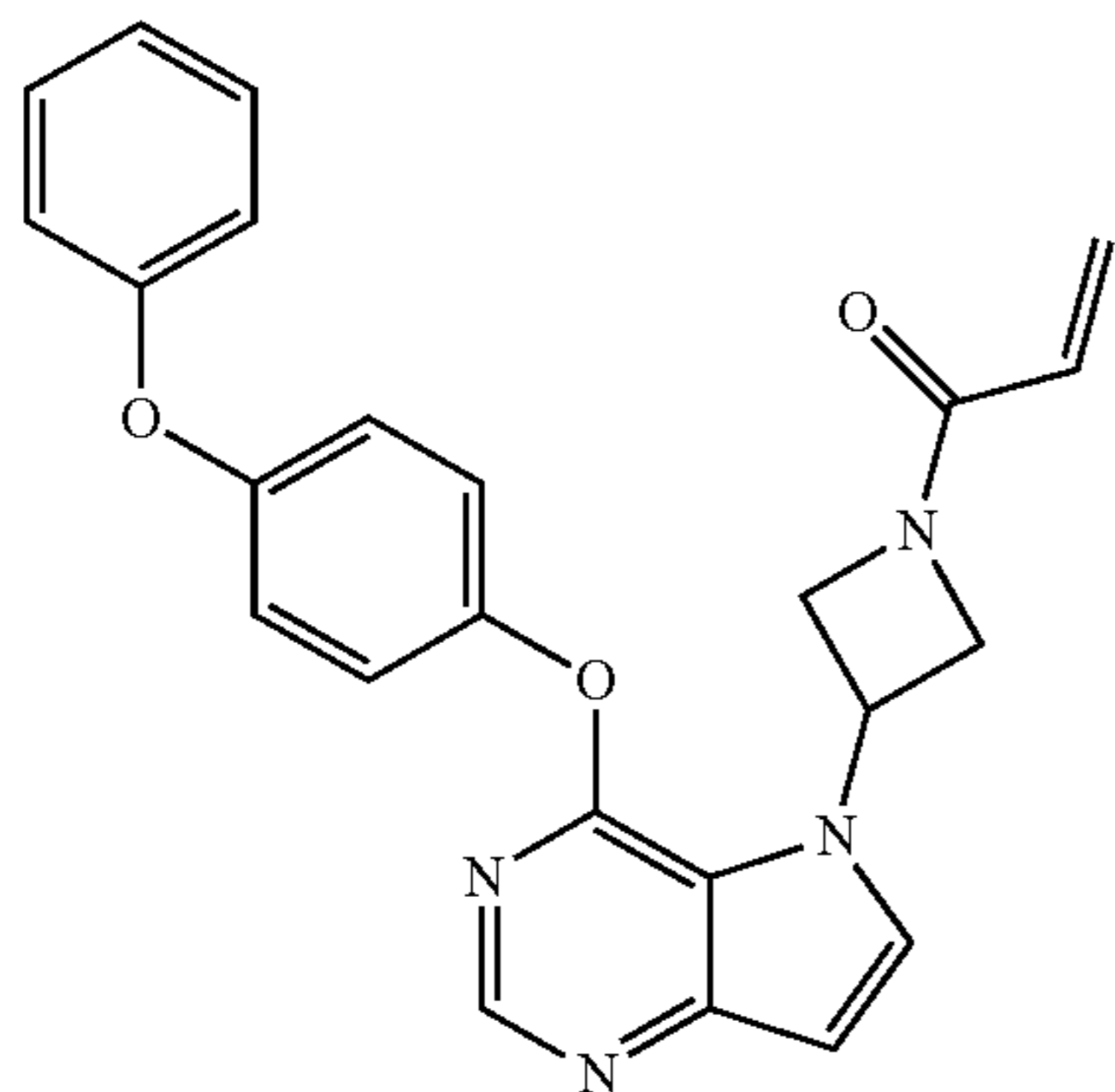
1-(3-(4-(4-phenoxyphenoxy)-5H-pyrrolo[3,2-d]pyrimidin-5-yl)azetidin-1-yl)prop-2-en-1-one (3) (Method F)
