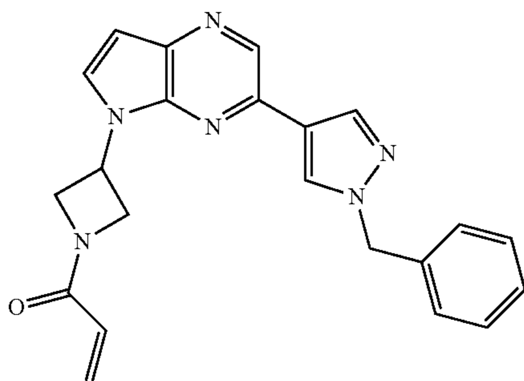
1-(3-(3-(1-benzyl-1H-pyrazol-4-yl)-5H-pyrrolo[2,3-b]pyrazin-5-yl)azetid-1-yl)prop-2-en-1-one (52)
