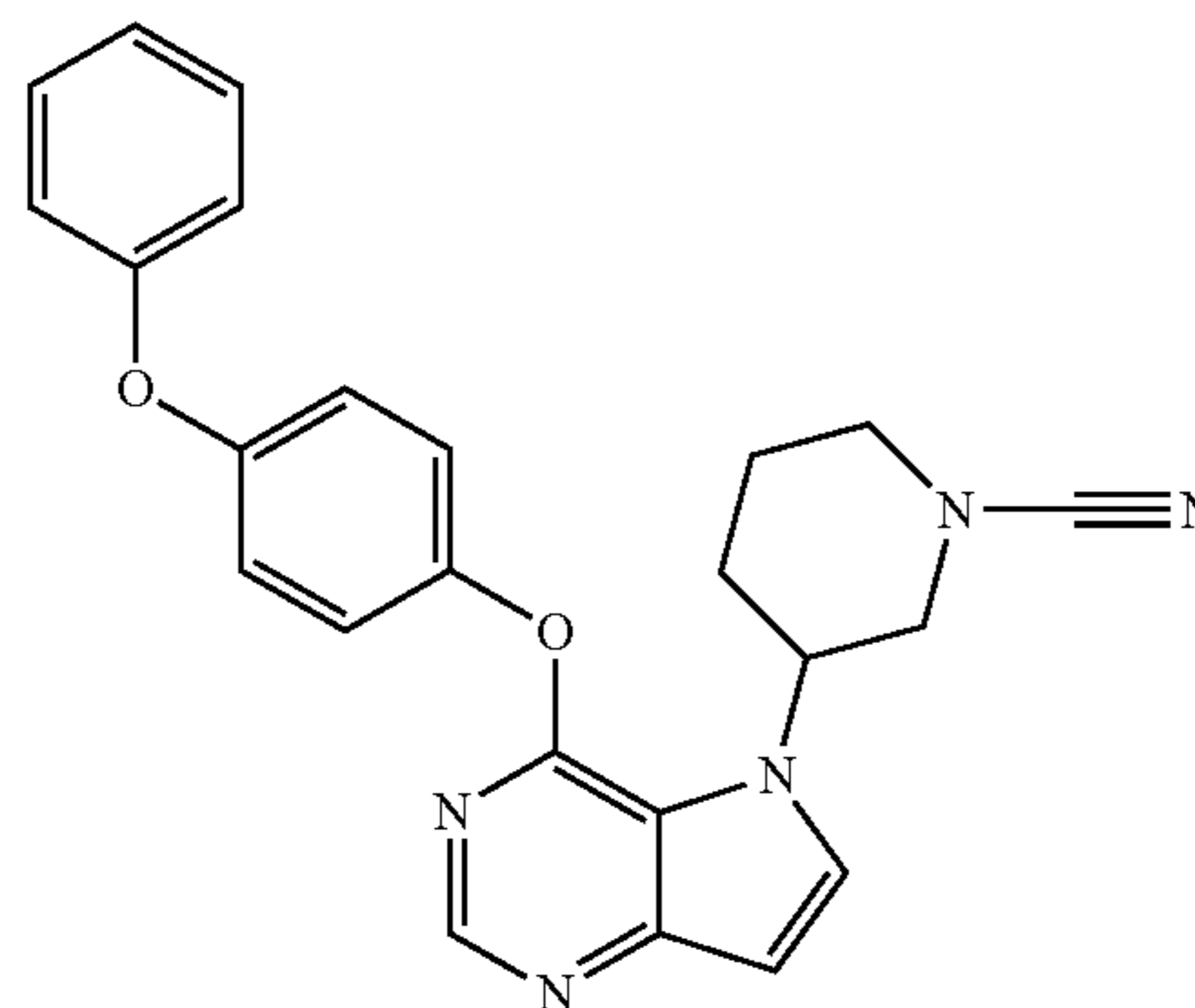
3-[4-(4-phenoxyphenoxy)-5H-pyrrolo[3,2-d]pyrimidin-5-yl]piperidine-1-carbonitrile (64)
