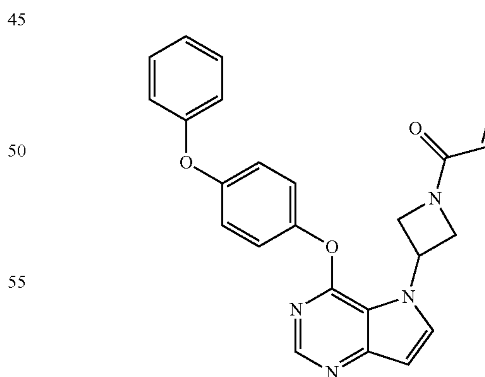
1-(3-(4-((4-phenoxyphenyl)amino)-5H-pyrrolo[3,2-d]pyrimidin-5-yl)azetidin-1-yl)prop-2-en-1-one (6)
