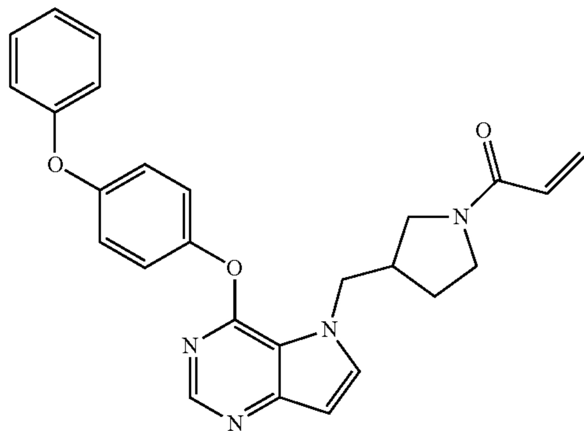
1-(3-((4-(4-phenoxyphenoxy)-5H-pyrrolo[3,2-d]pyrimidin-5-yl)methyl)pyrrolidin-1-yl)prop-2-en-1-one (29)
