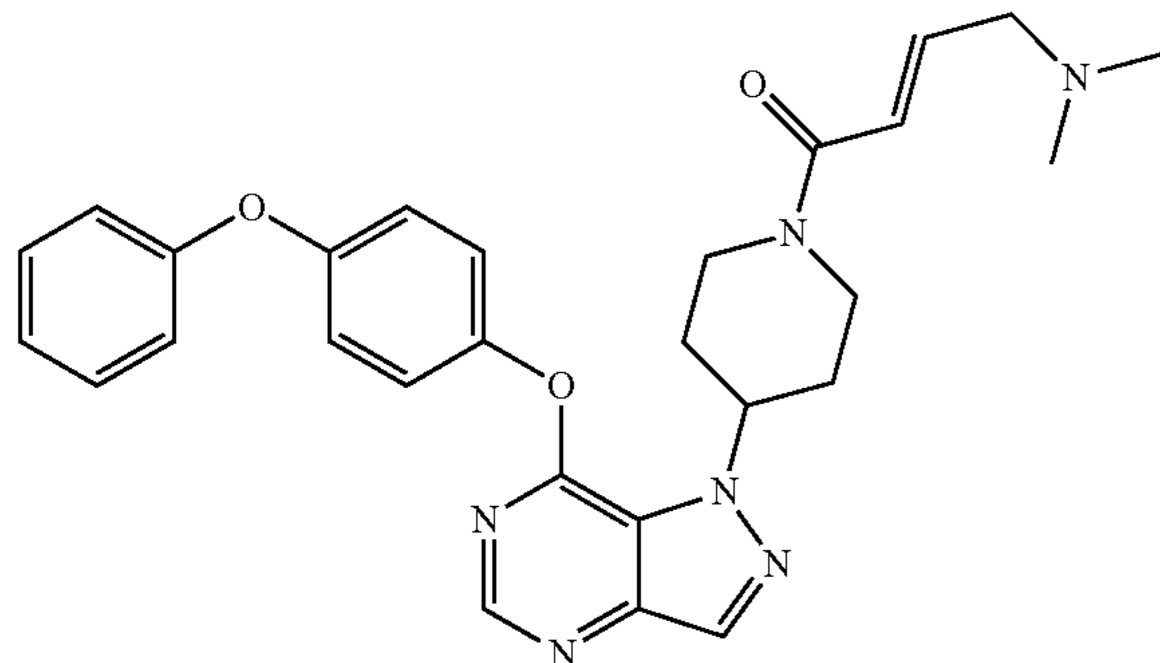
(E)-4-(dimethylamino)-1-(4-(7-(4-phenoxyphenoxy)-1H-pyrazolo[4,3-d]pyrimidin-1-yl)piperidin-1-yl)but-2-en-1-one (14)
