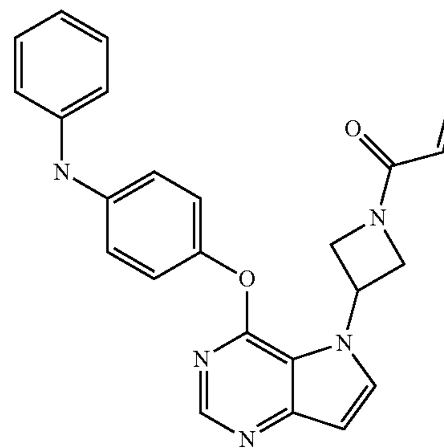
1-(3-(4-(4-(phenylamino)phenoxy)-5H-pyrrolo[3,2-d]pyrimidin-5-yl)azetidin-1-yl)prop-2-en-1-one (22)
