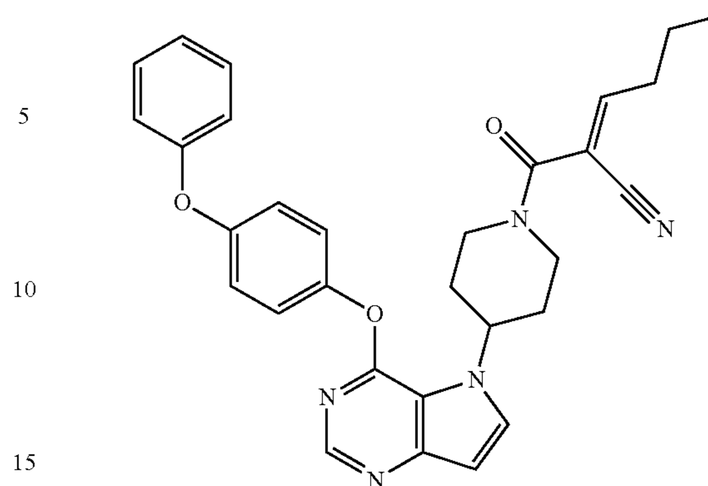
(E)-4-(4-(4-(4-phenoxyphenoxy)-5H-pyrrolo[3,2-d]pyrimidin-5-yl)piperidine-1-carbonyl)hex-2-enitrile (55)
