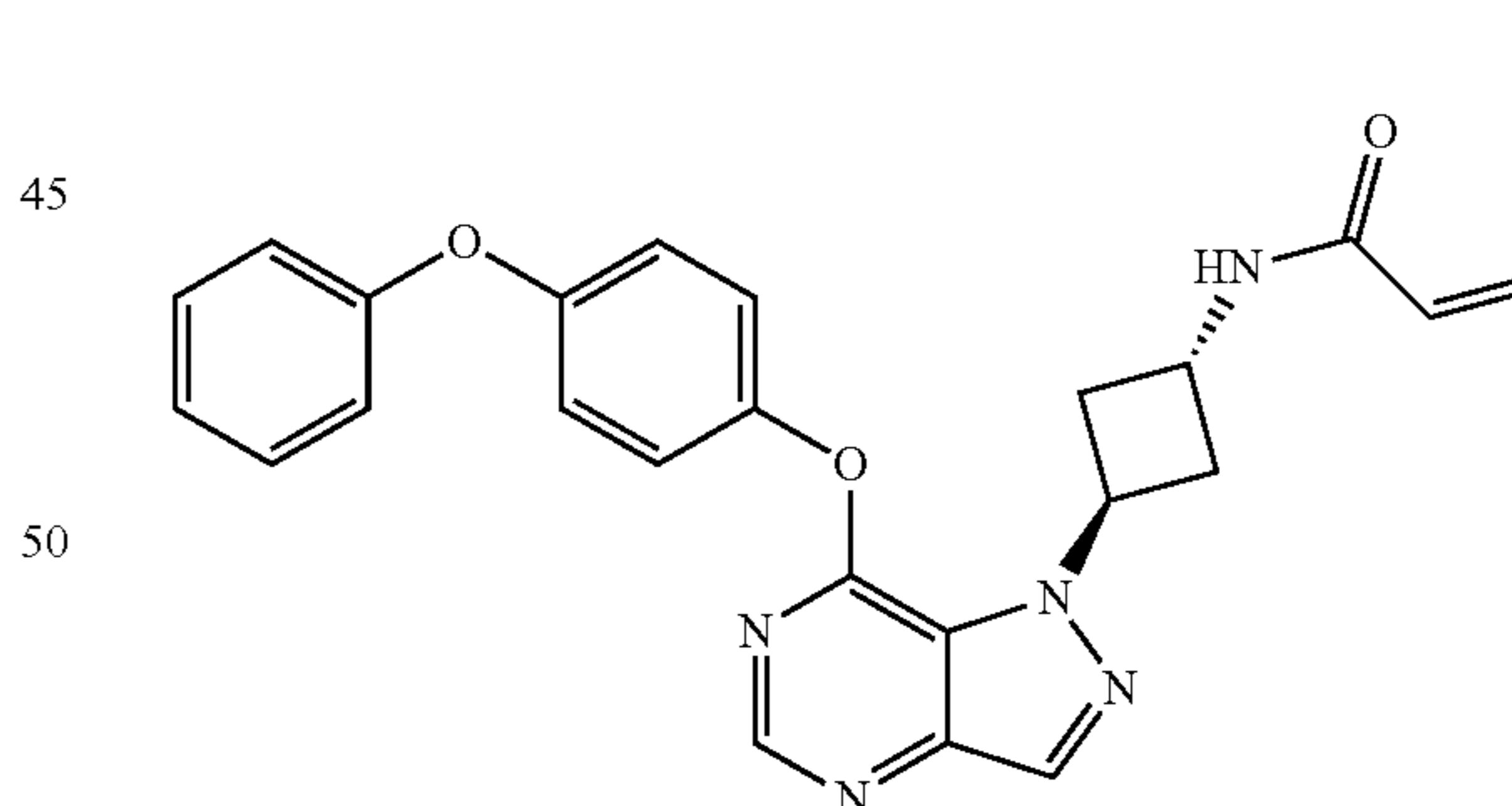
N-((1r,3r)-3-(7-(4-phenoxyphenoxy)-1H-pyrazolo[4,3-d]pyrimidin-1-yl)cyclobutyl)acrylamide (21)
