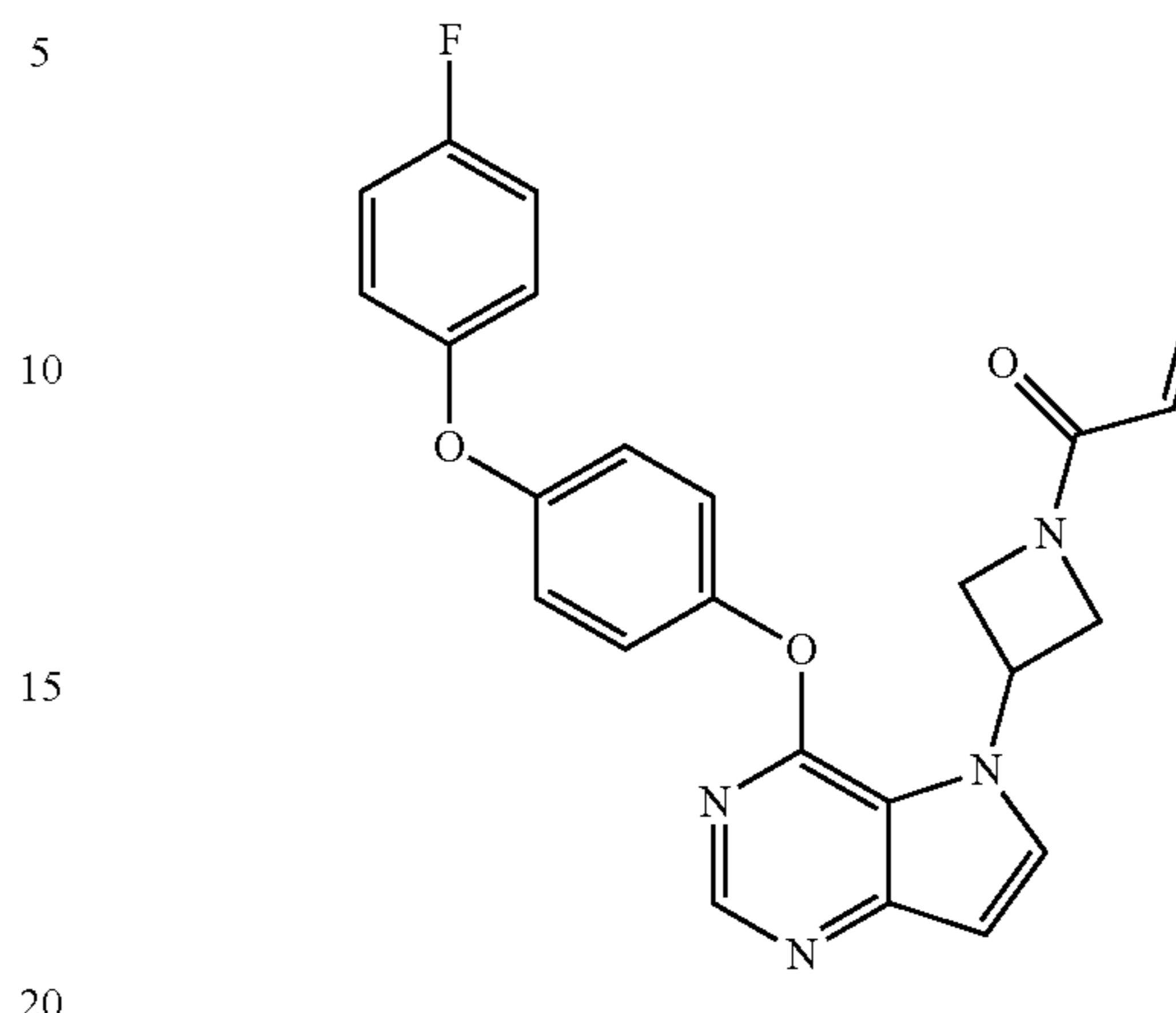
1-(3-(4-(4-(4-fluorophenoxy)phenoxy)-5H-pyrrolo[3,2-d]pyrimidin-5-yl)azetidin-1-yl)prop-2-en-1-one (27)
