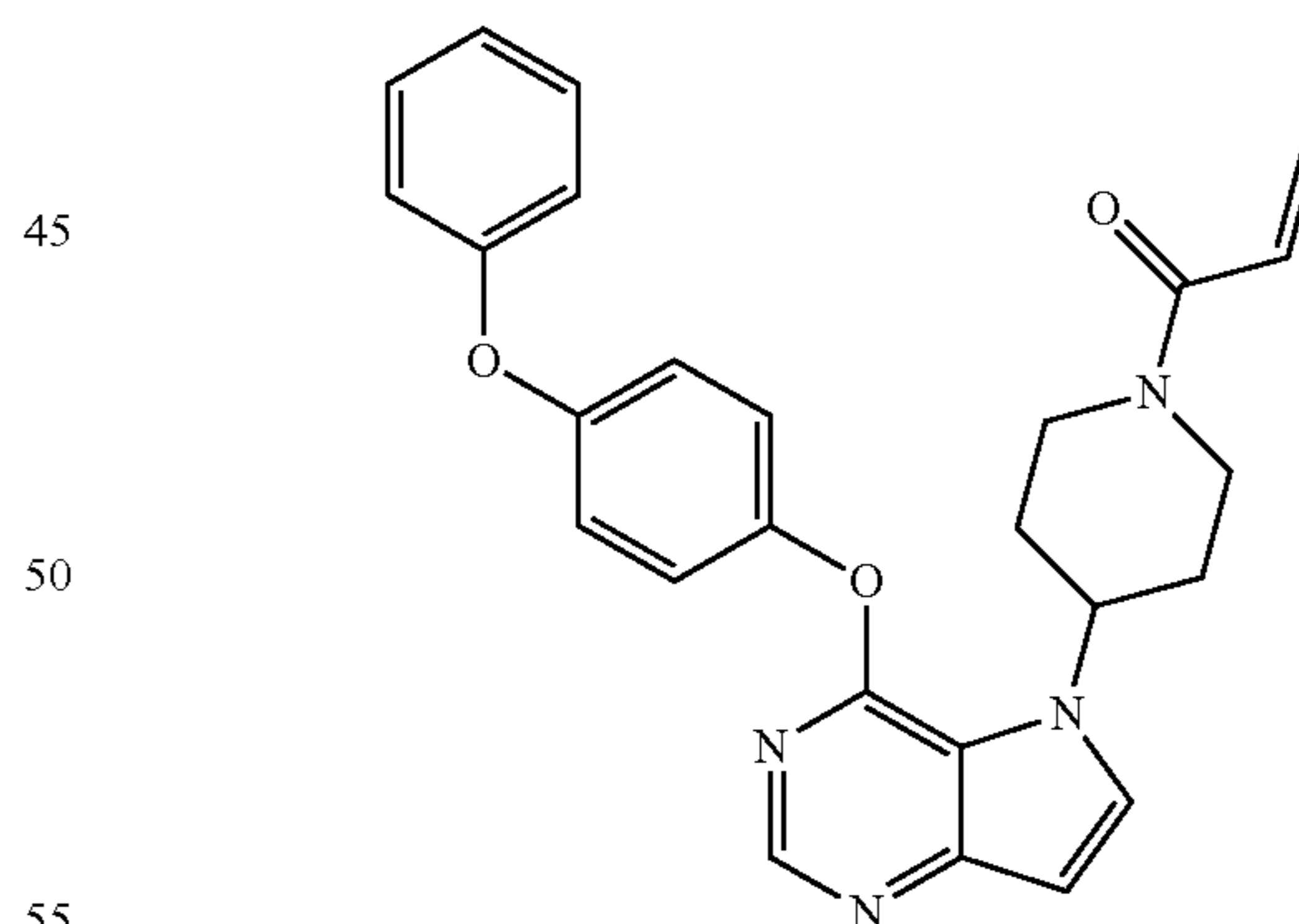
1-(4-(4-(4-phenoxyphenoxy)-5H-pyrrolo[3,2-d]pyrimidin-5-yl)piperidin-1-yl)prop-2-en-1-one (2)
