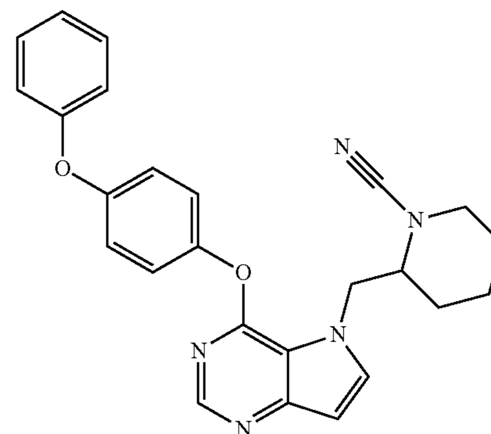
2-[[4-(4-phenoxyphenoxy)-5H-pyrrolo[3,2-d]pyrimidin-5-yl]methyl]piperidine-1-carbonitrile (62)
