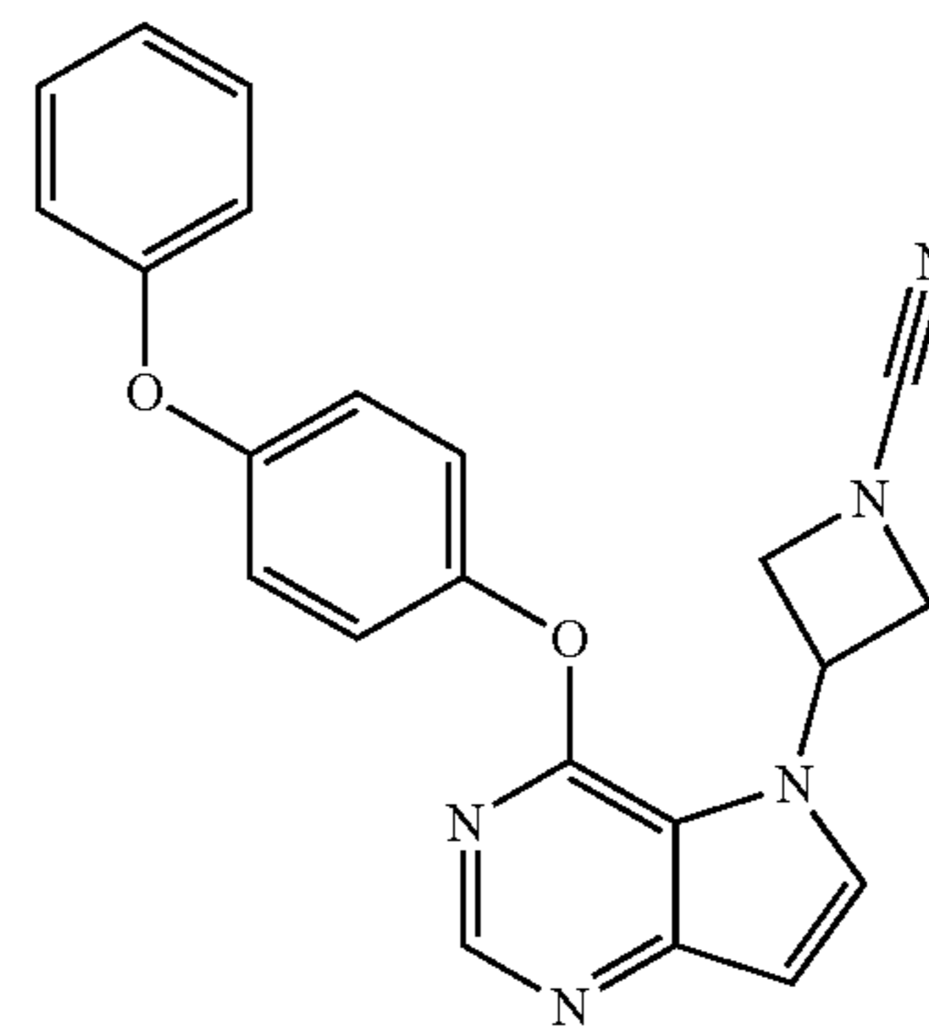
3-[4-(4-phenoxyphenoxy)-5H-pyrrolo[3,2-d]pyrimidin-5-yl]azetidine-1-carbonitrile (68)
