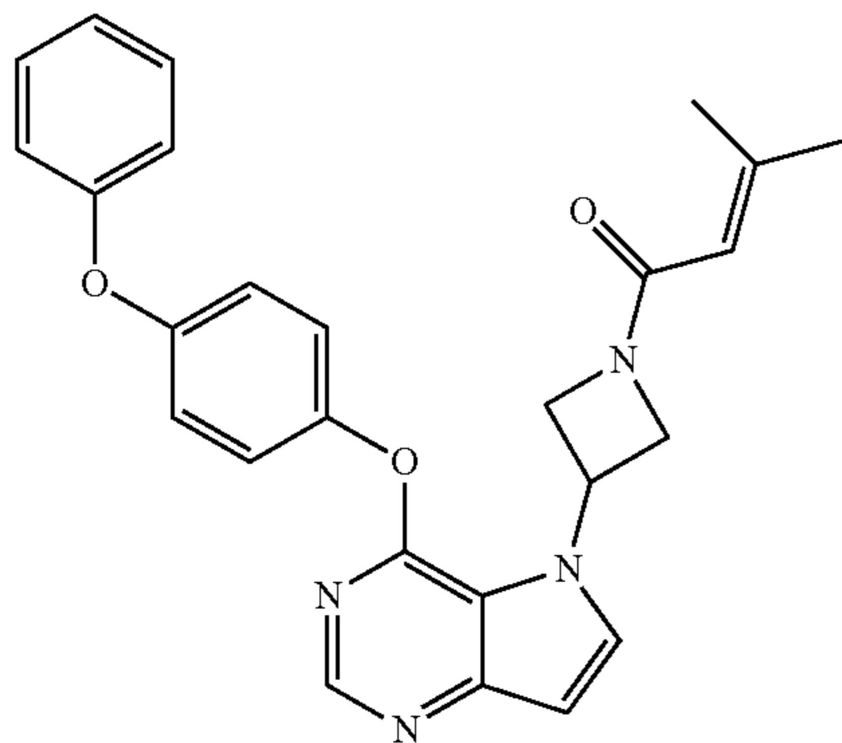
3-methyl-1-(3-(4-(4-phenoxyphenyl)-5H-pyrrolo[3,2-d]pyrimidin-5-yl)azetidin-1-yl)but-2-en-1-one (49)
