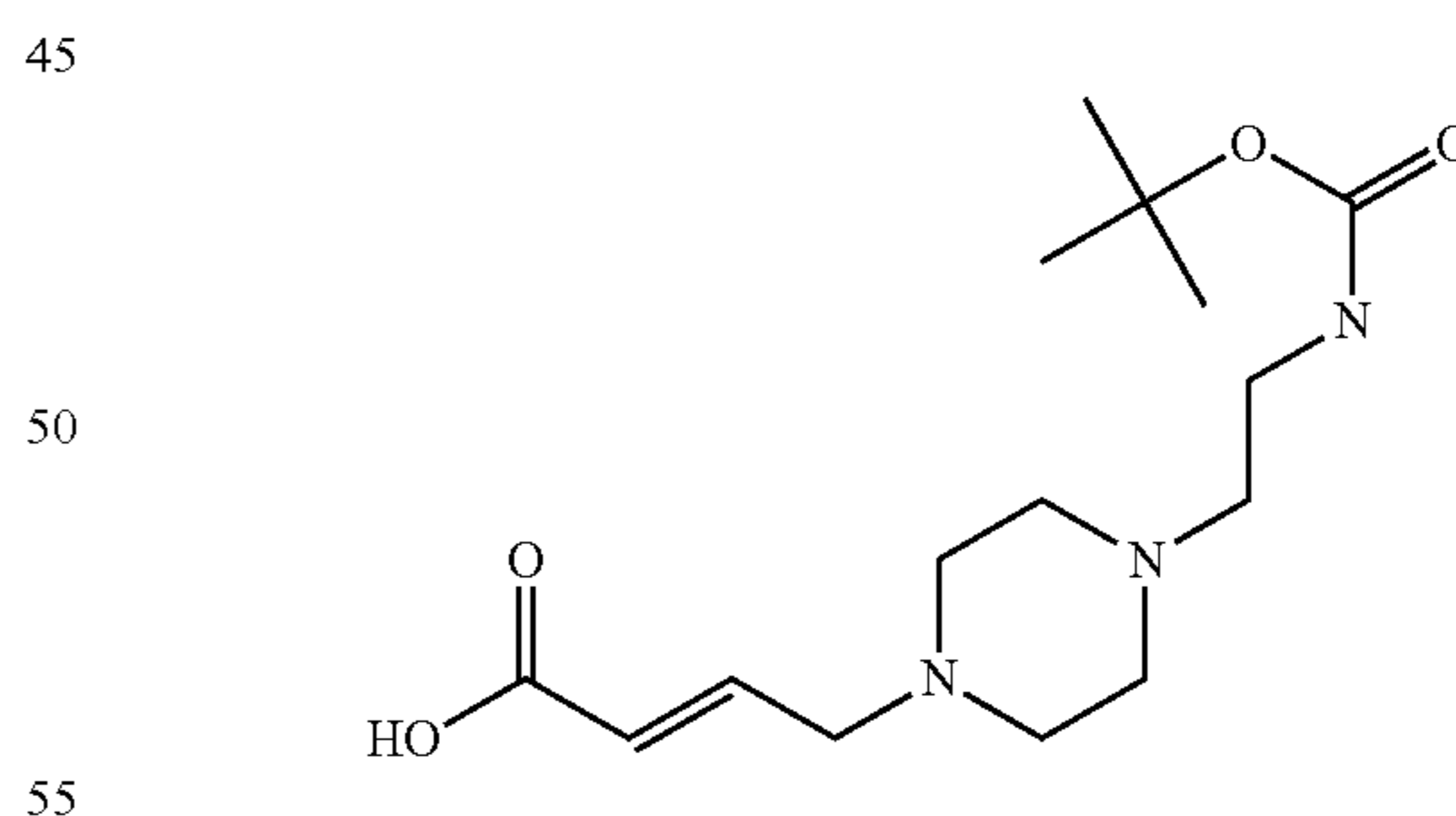
(E)-4-(4-(2-((tert-butoxycarbonyl)amino)ethyl)piperazin-1-yl)but-2-enoic acid
