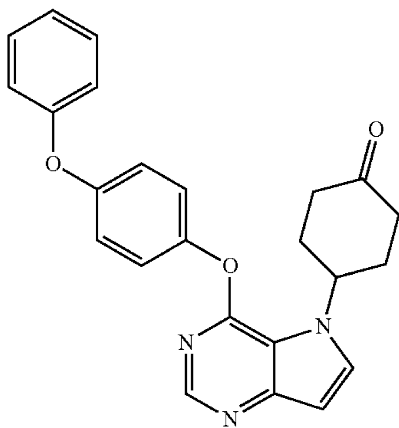
4-[4-(4-phenoxyphenoxy)-5H-pyrrolo[3,2-d]pyrimidin-5-yl]cyclohexan-1-one
