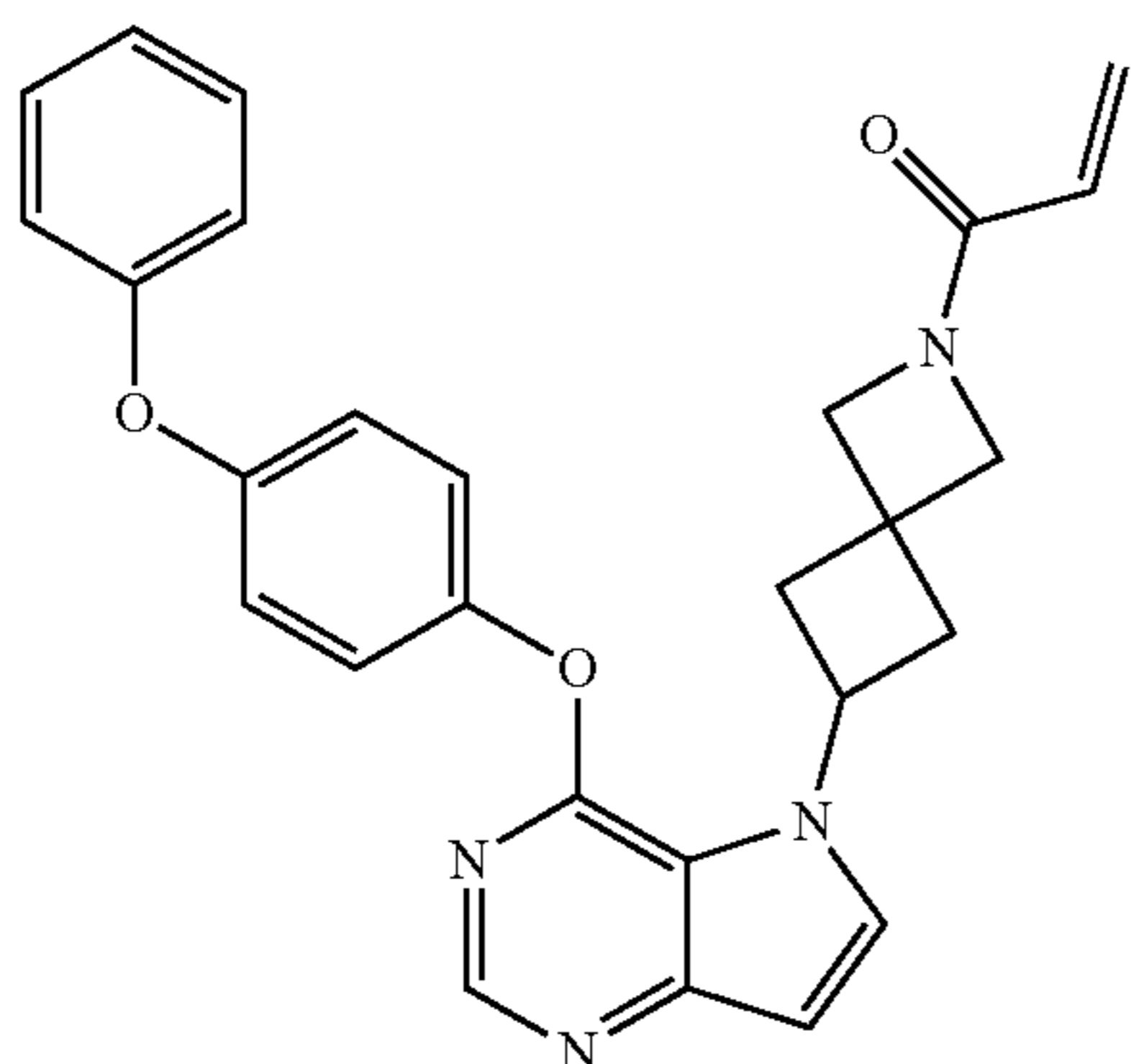
1-(6-(4-(4-phenoxyphenoxy))-5H-pyrrolo[3,2-d]pyrimidin-5-yl)azaspiro[3.3]heptan-2-ylprop-2-en-1-one (28)
