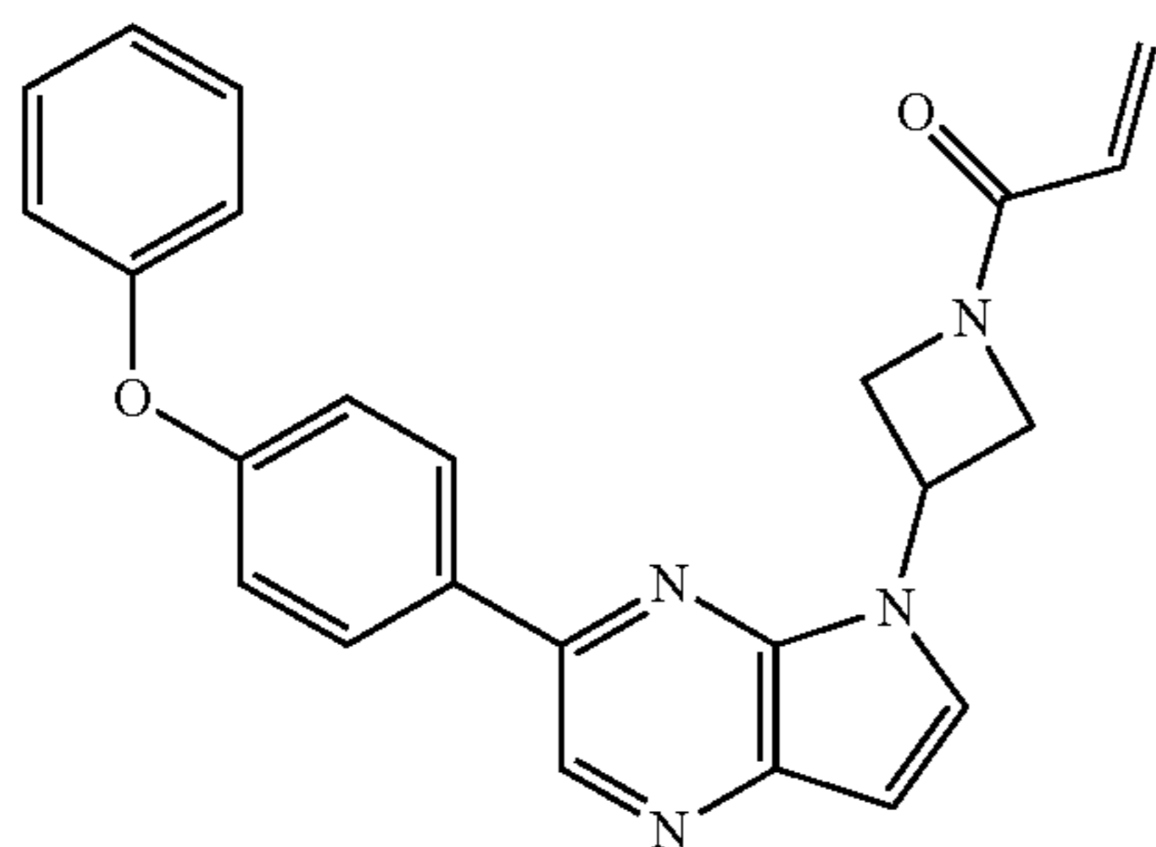
1-(3-(3-(4-phenoxyphenyl)-5H-pyrrolo[2,3-b]pyrazin-5-yl)azetidin-1-yl)prop-2-en-1-one (7)
