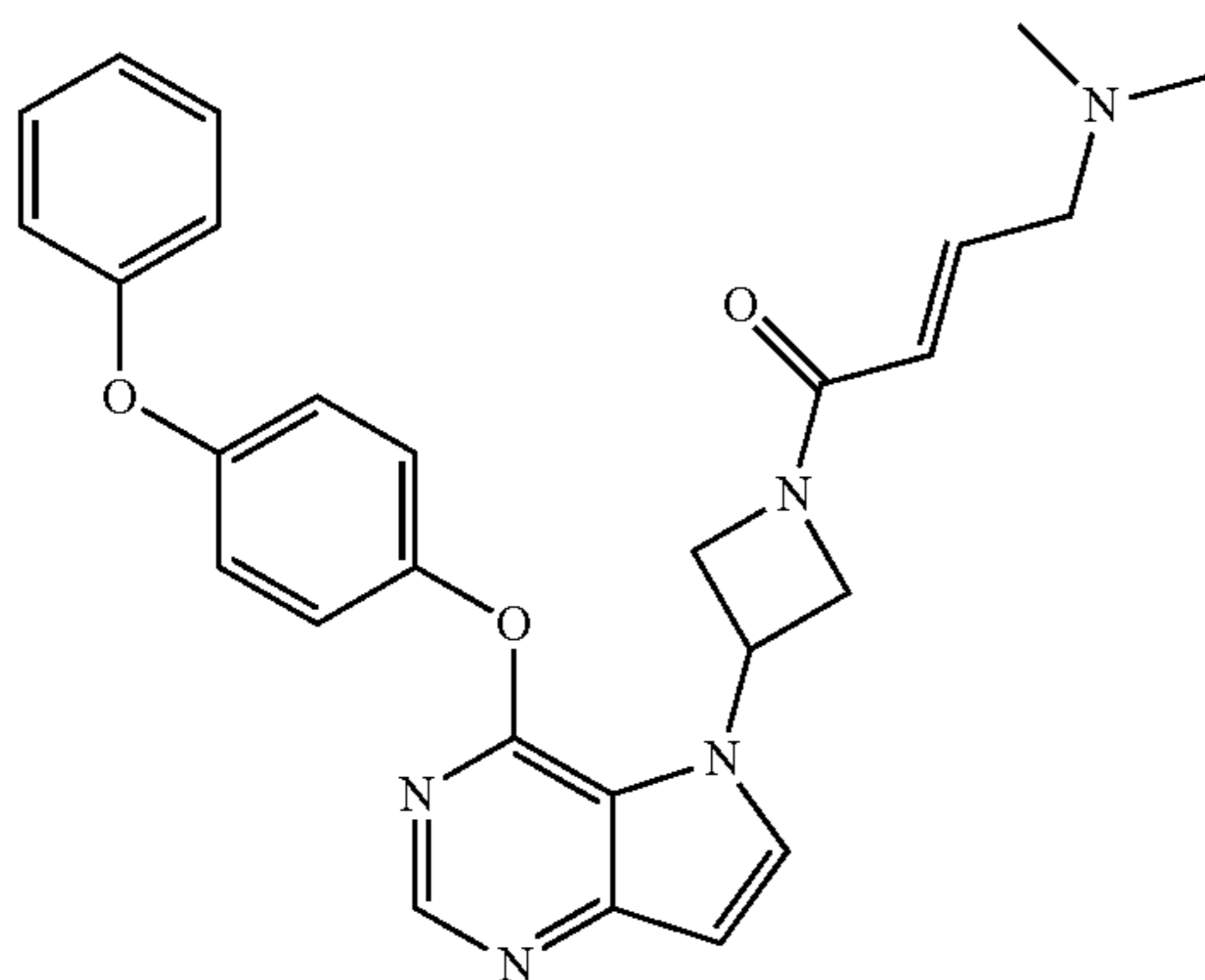
(E)-4-(dimethylamino)-1-(3-(4-(4-phenoxyphenoxy)-5H-pyrrolo[3,2-d]pyrimidin-5-yl)azetidin-1-yl)but-2-en-1-one (19) (Method G)
