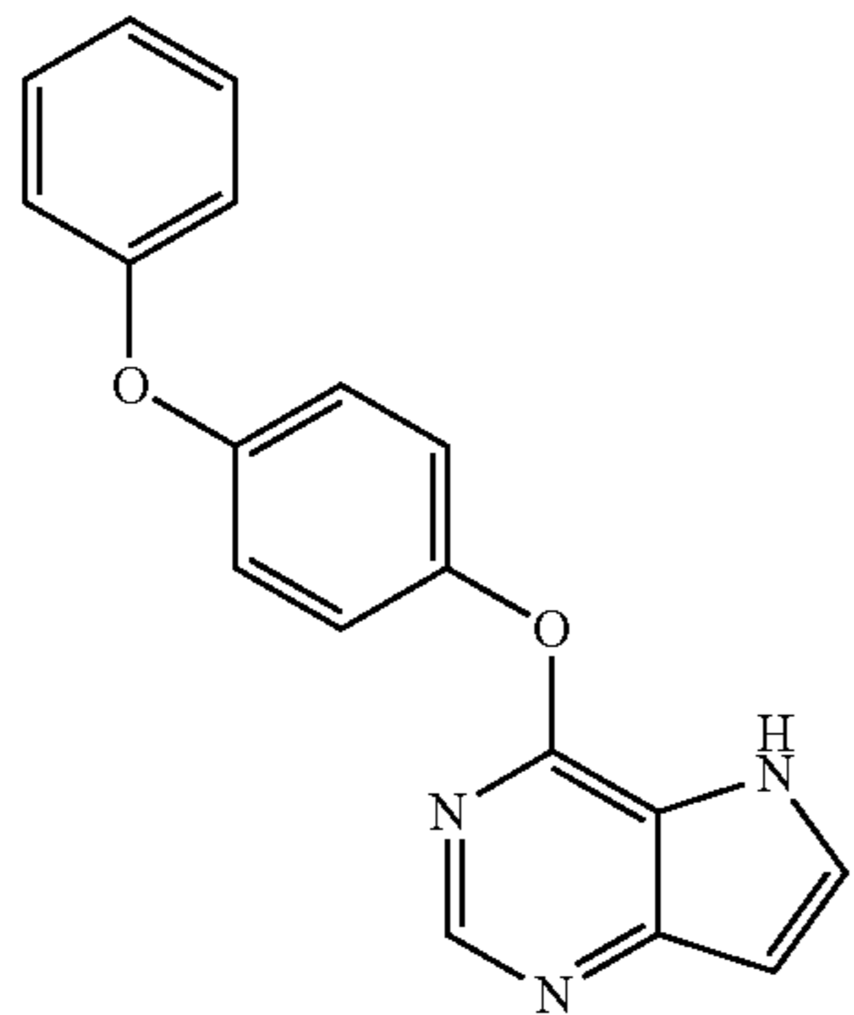
4-(4-phenoxyphenoxy)-5H-pyrrolo[3,2-d]pyrimidine (Method B)
