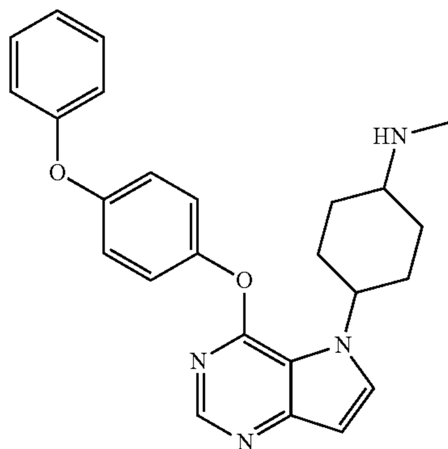
N-methyl-4-[4-(4-phenoxyphenoxy)-5H-pyrrolo[3,2-d]pyrimidin-5-yl]cyclohexan-1-amine
