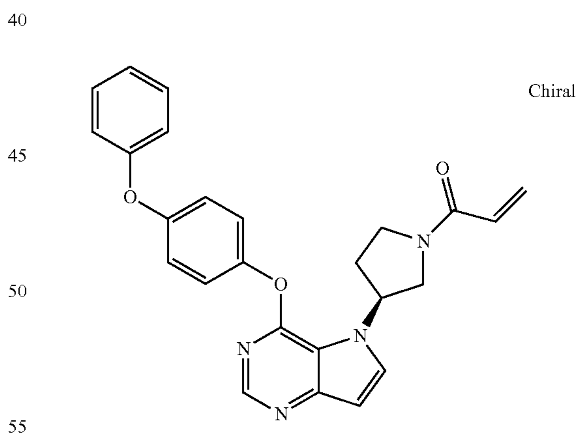
(S)-1-(3-(4-(4-phenoxyphenoxy)-5H-pyrrolo[3,2-d]pyrimidin-5-yl)pyrrolidin-1-yl)prop-2-en-1-one (5)
