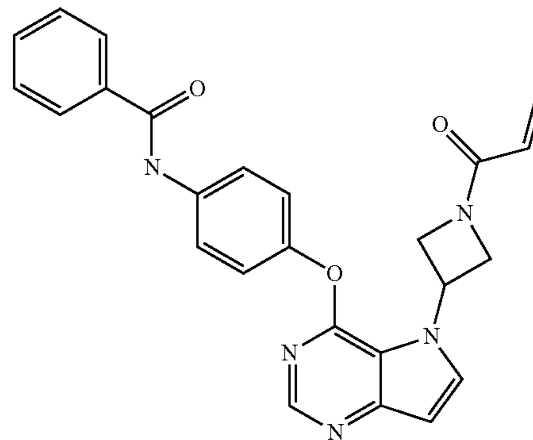
N-(4-((5-(1-acryloylazetidin-3-yl)-5H-pyrrolo[3,2-d]pyrimidin-4-yl)oxy)phenyl)benzamide (35)
