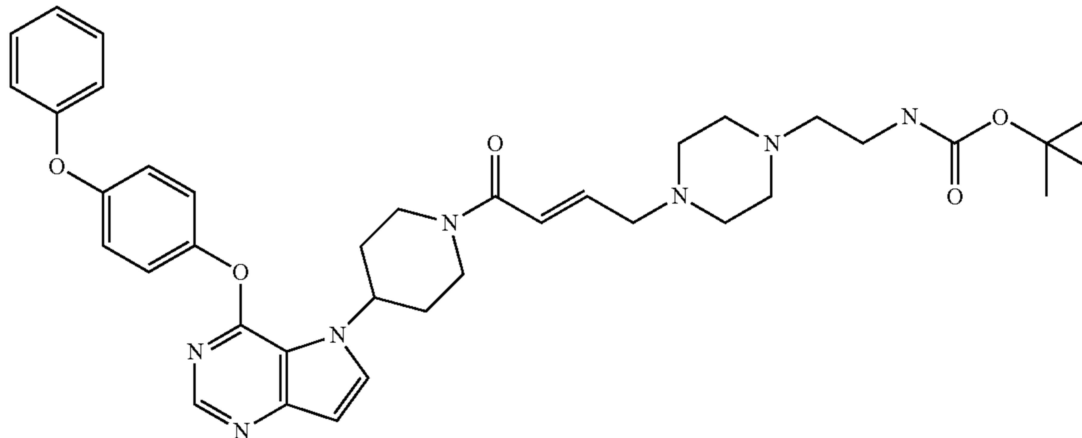
20 tert-butyl (E)-(2-(4-(4-oxo-4-(4-(4-(4-phenoxyphenoxy)-5H-pyrrolo[3,2-d]pyrimidin-5-yl)piperidin-1-yl)but-2-en-1-yl)piperazin-1-yl)ethyl)carbamate
