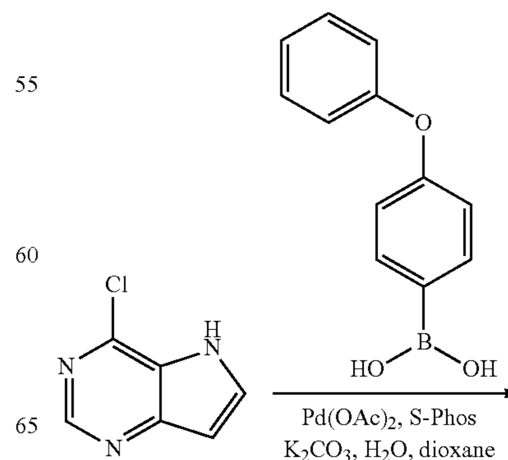
Scheme 1
