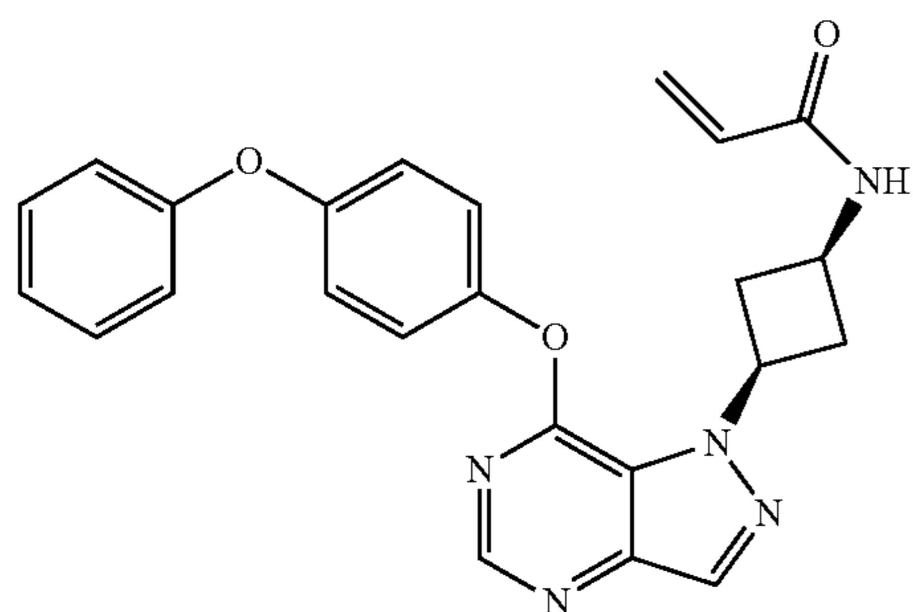
N-((1s,3s)-3-(7-(4-phenoxyphenoxy)-1H-pyrazolo[4,3-d]pyrimidin-1-yl)cyclobutyl)acrylamide (11) (relative configuration)
