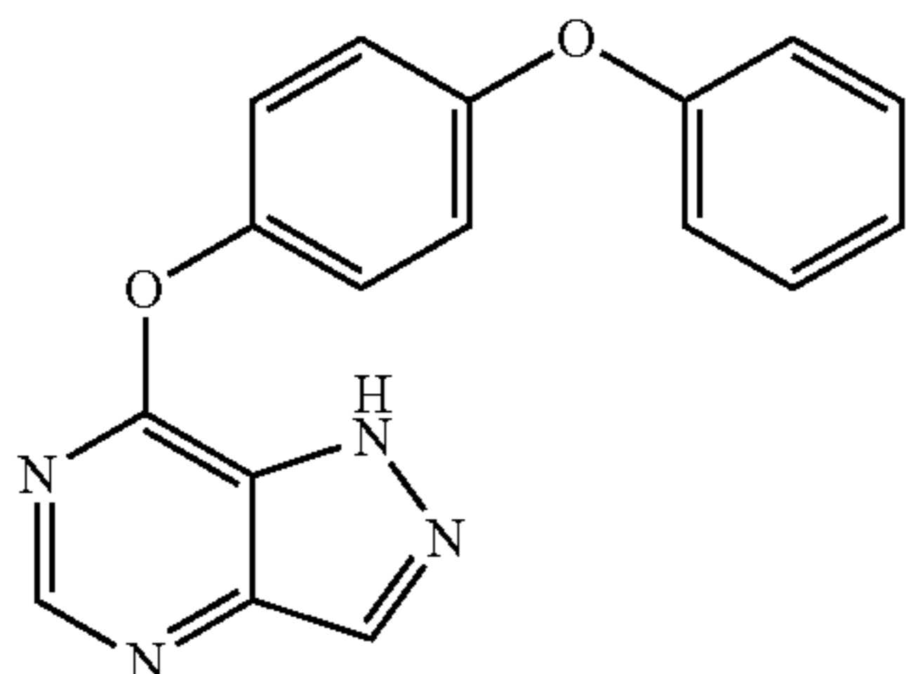
7-(4-phenoxyphenoxy)-1H-pyrazolo[4,3-d]pyrimidine (Method J)
