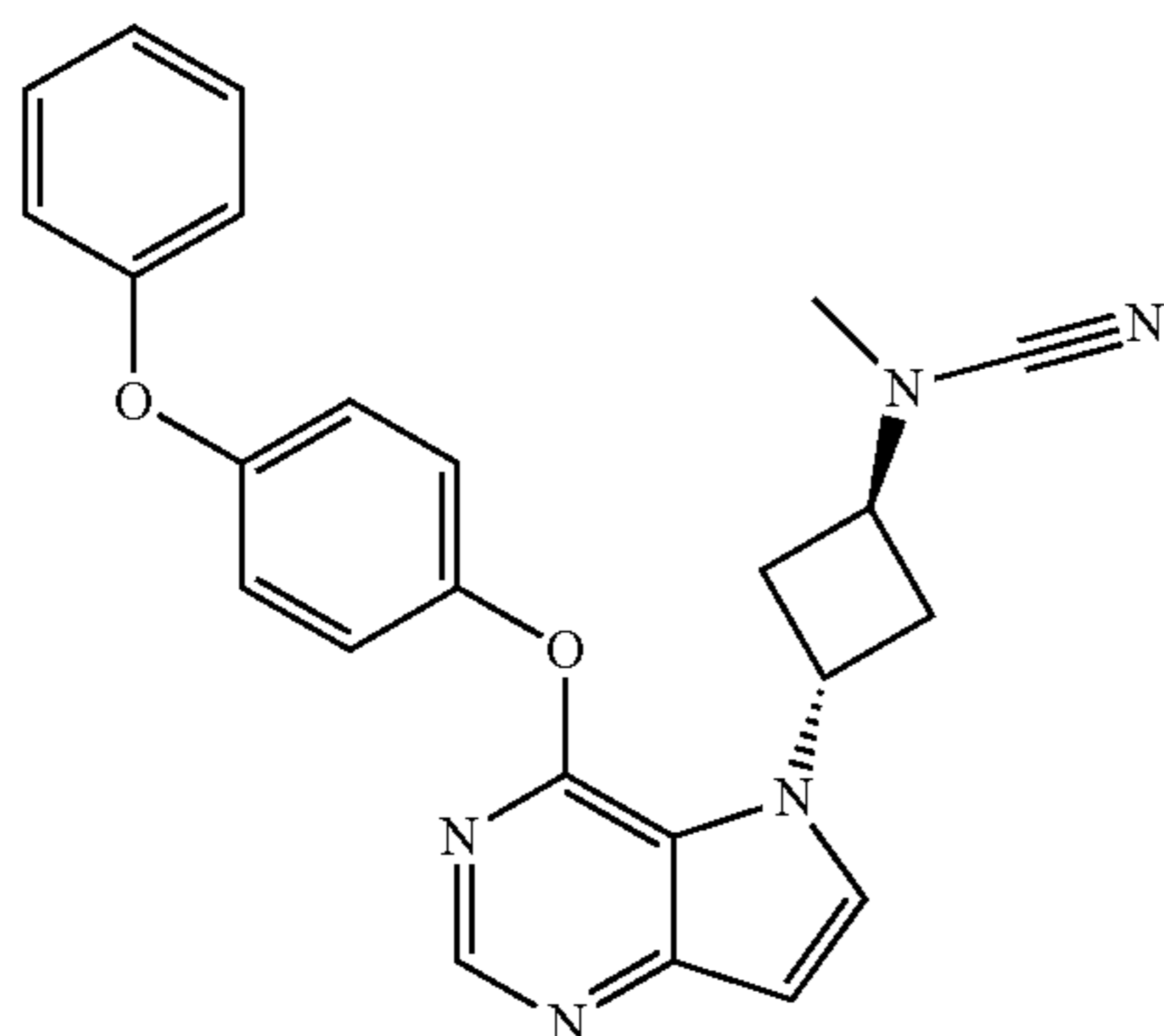
(1R,3R)—N-cyano-N-methyl-3-[4-(4-phenoxyphenoxy)-5H-pyrrolo[3,2-d]pyrimidin-5-yl]cyclobutan-1-amine (67)
