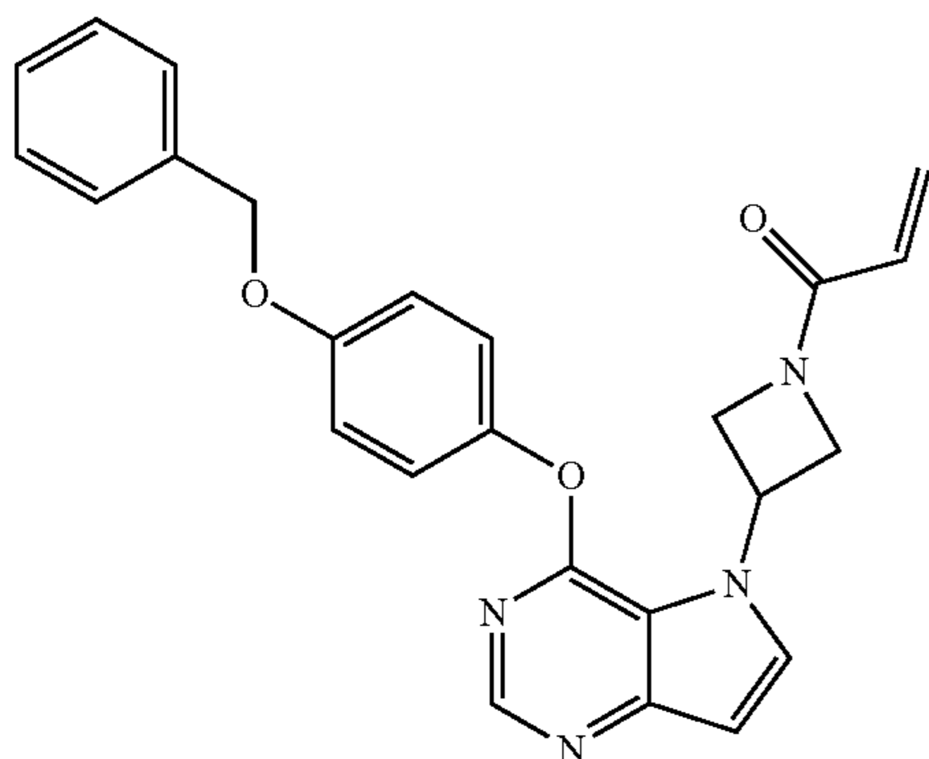
1-(3-(4-(4-(benzyloxy)phenoxy)-5H-pyrrolo[3,2-d]pyrimidin-5-yl)azetidin-1-yl)prop-2-en-1-one (16)
