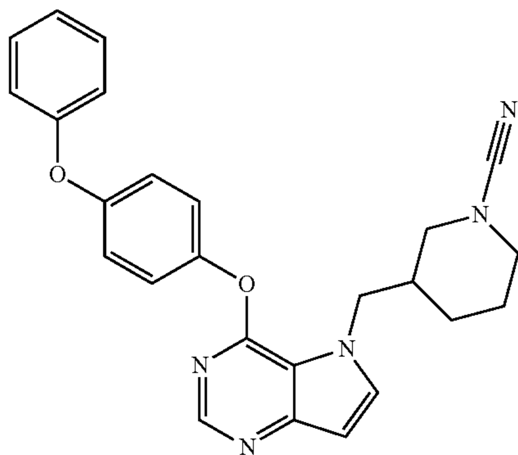
3-[[4-(4-phenoxyphenoxy)-5H-pyrrolo[3,2-d]pyrimidin-5-yl]methyl]piperidine-1-carbonitrile (63)
