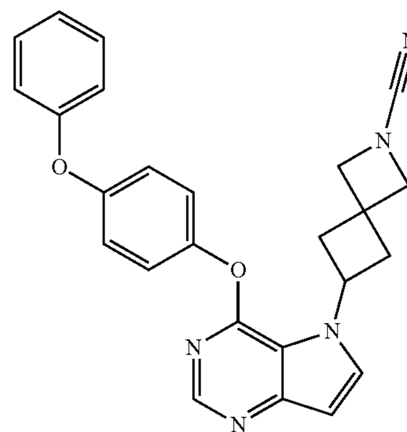
6-[4-(4-phenoxyphenoxy)-5H-pyrrolo[3,2-d]pyrimidin-5-yl]-2-azaspiro[3.3]heptane-2-carbonitrile (69)
