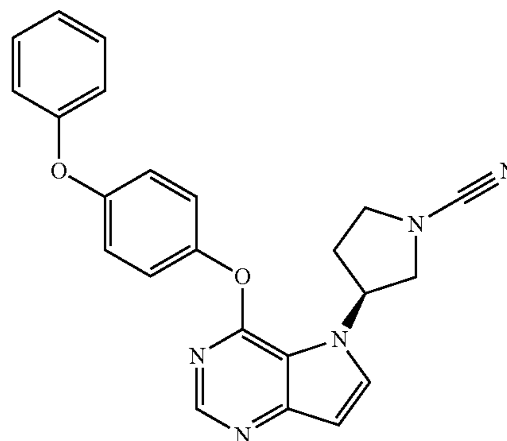
(3S)-3-[4-(4-phenoxyphenoxy)-5H-pyrrolo[3,2-d]pyrimidin-5-yl]pyrrolidine-1-carbonitrile (72)
