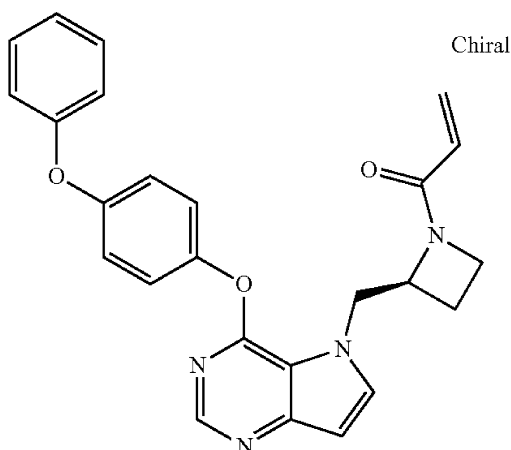
(S)-1-(2-((4-(4-phenoxyphenoxy))-5H-pyrrolo[3,2-d]pyrimidin-5-yl)methyl)azetidin-1-yl)prop-2-en-1-one (25)
