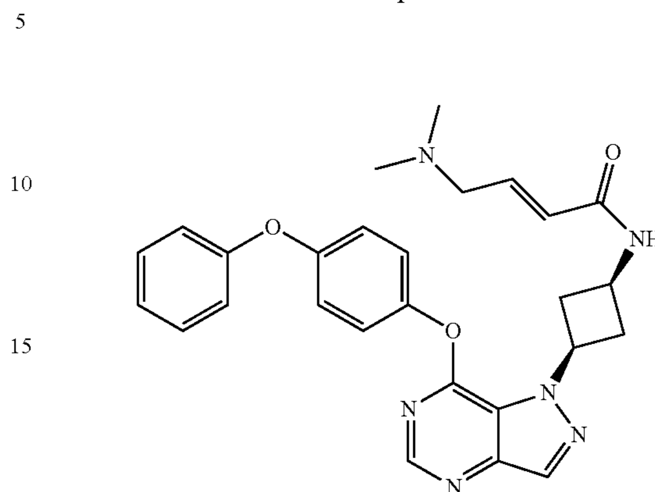
(E)-4-(dimethylamino)-N-((1s,3s)-3-(7-(4-phenoxyphenoxy)-1H-pyrazolo[4,3-d]pyrimidin-1-yl)cyclobutyl)but-2-enamide (36)
