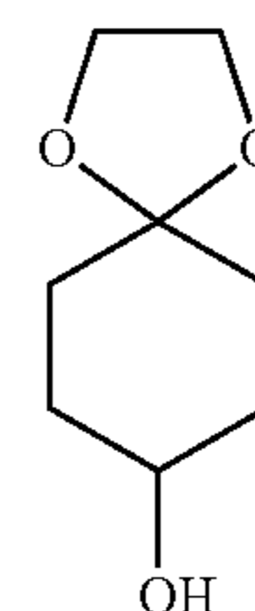
1,4-dioxaspiro[4.5]decan-8-ol
