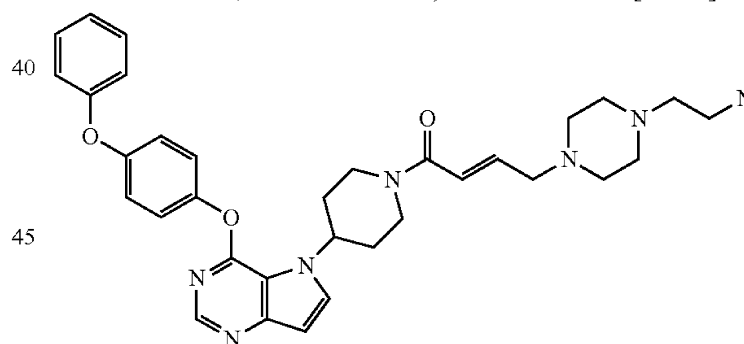
40 (E)-4-(4-(2-aminoethyl)piperazin-1-yl)-1-(4-(4-(4-phenoxyphenoxy)-5H-pyrrolo[3,2-d]pyrimidin-5-yl)piperidin-1-yl)but-2-en-1-one
