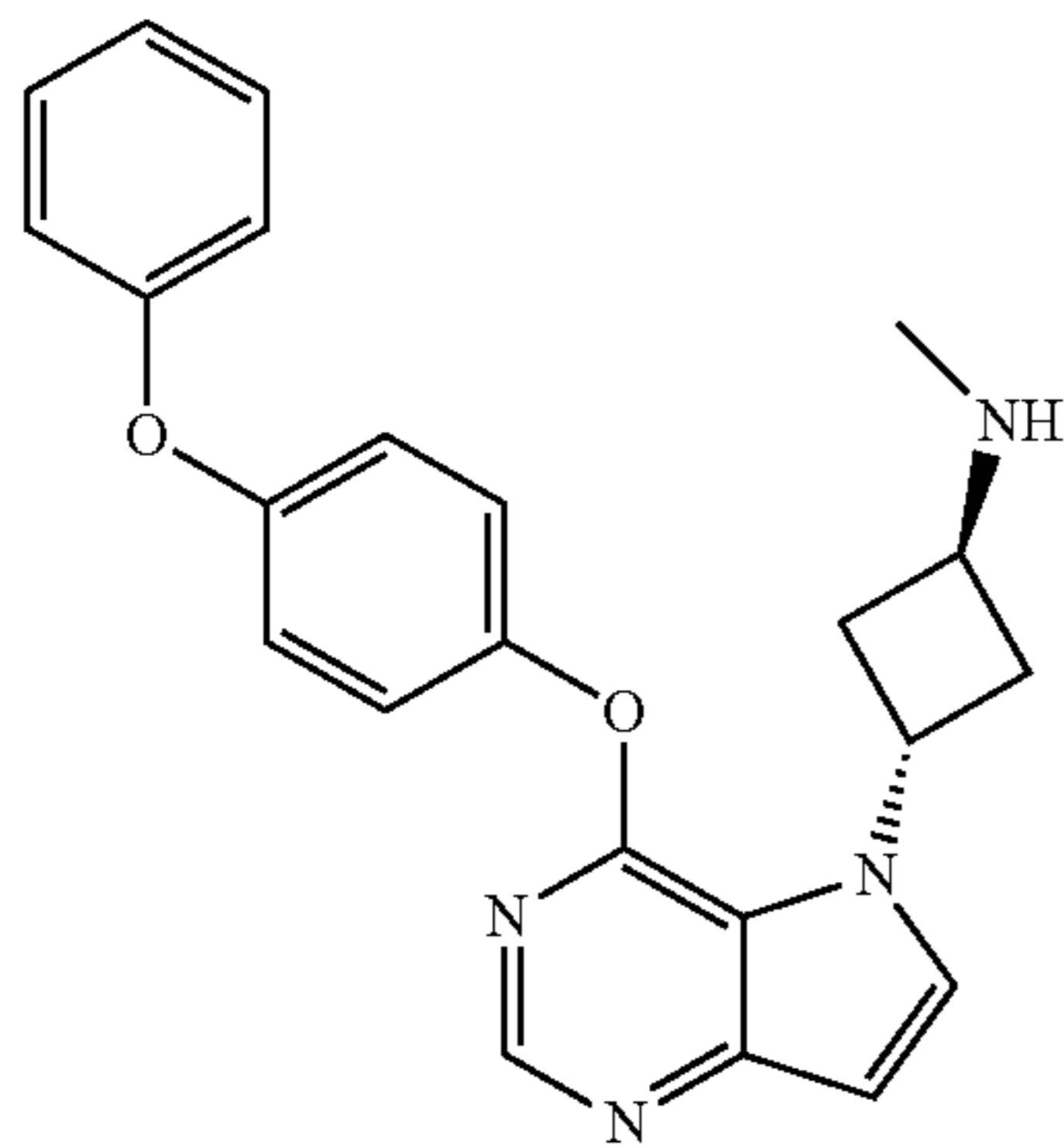
(1R,3R)—N-methyl-3-[4-(4-phenoxyphenoxy)-5H-pyrrolo[3,2-d]pyrimidin-5-yl]cyclobutan-1-amine
