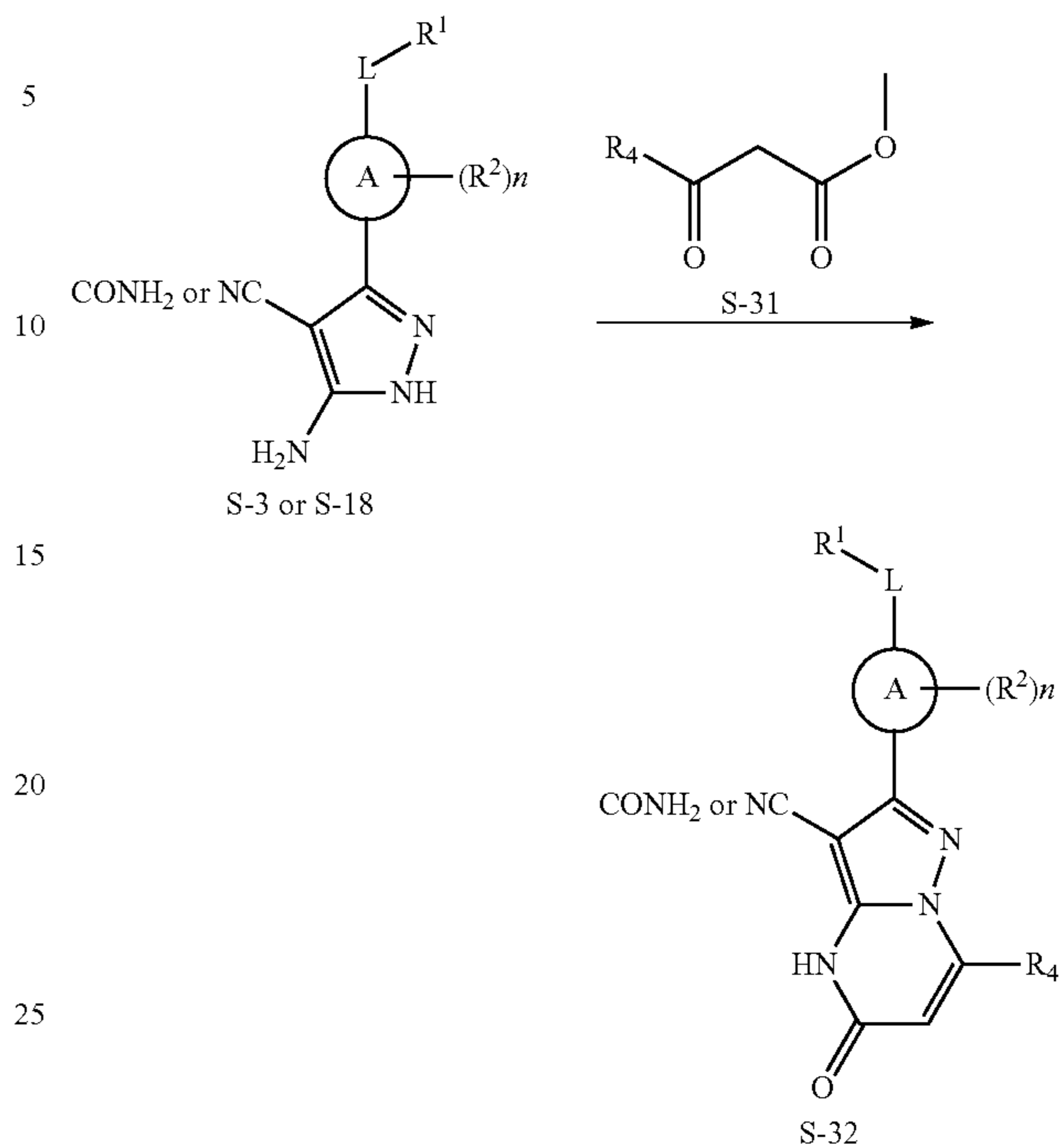
Scheme VII
