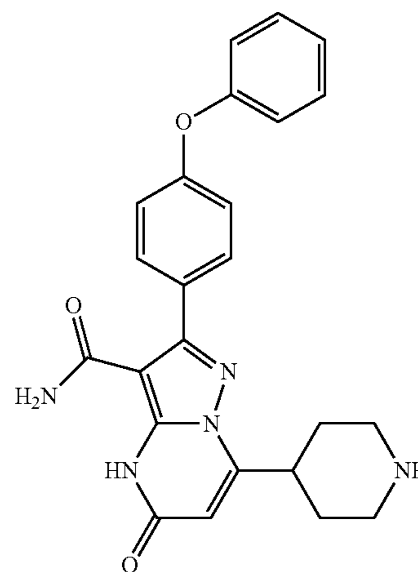
Compound 80: 5-Oxo-2-(4-phenoxyphenyl)-7-(piperidin-4-yl)-4,5-dihydropyrazolo[1,5-a]pyrimidine-3-carboxamide
