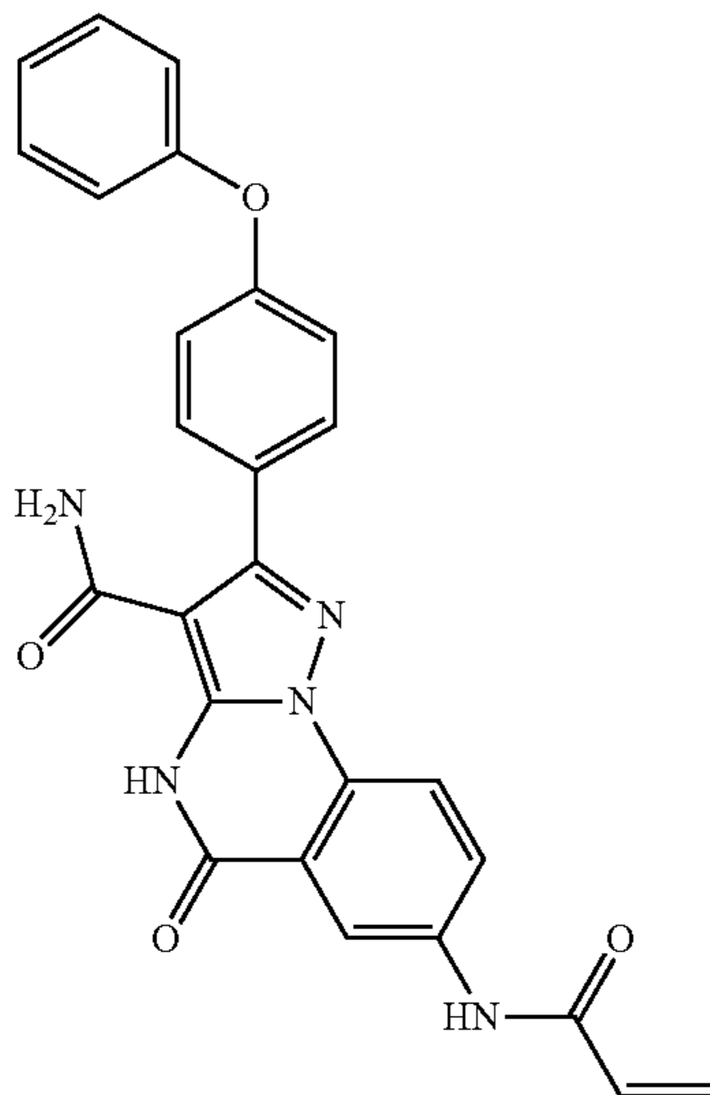
Compound 78: 7-Acrylamido-5-oxo-2-(4-phenoxyphenyl)-4,5-dihydropyrazolo[1,5-a]quinazoline-3-carboxamide
