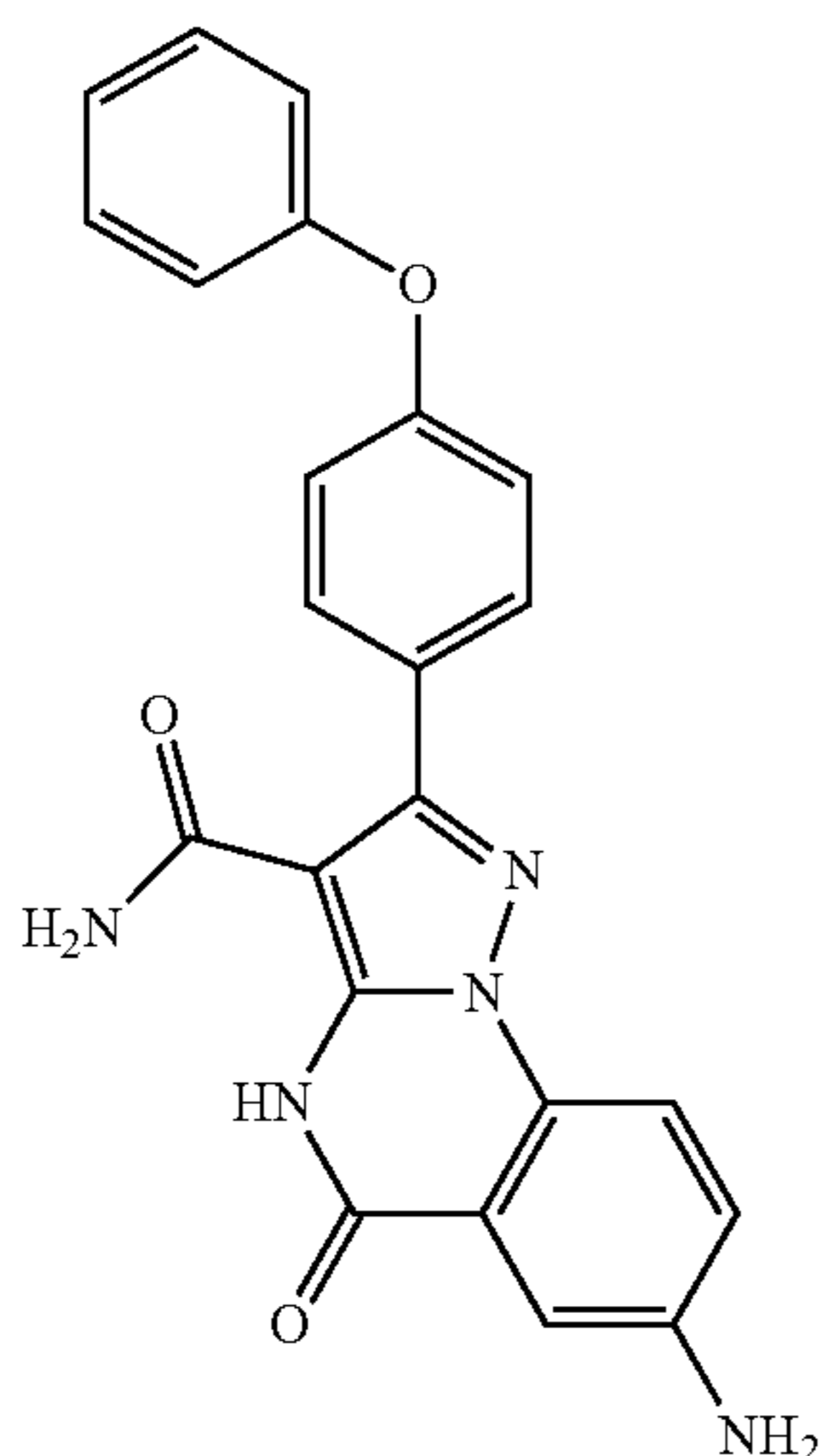
Compound 77: 7-Amino-5-oxo-2-(4-phenoxyphenyl)-4,5-dihydropyrazolo[1,5-a]quinazoline-3-carboxamide
