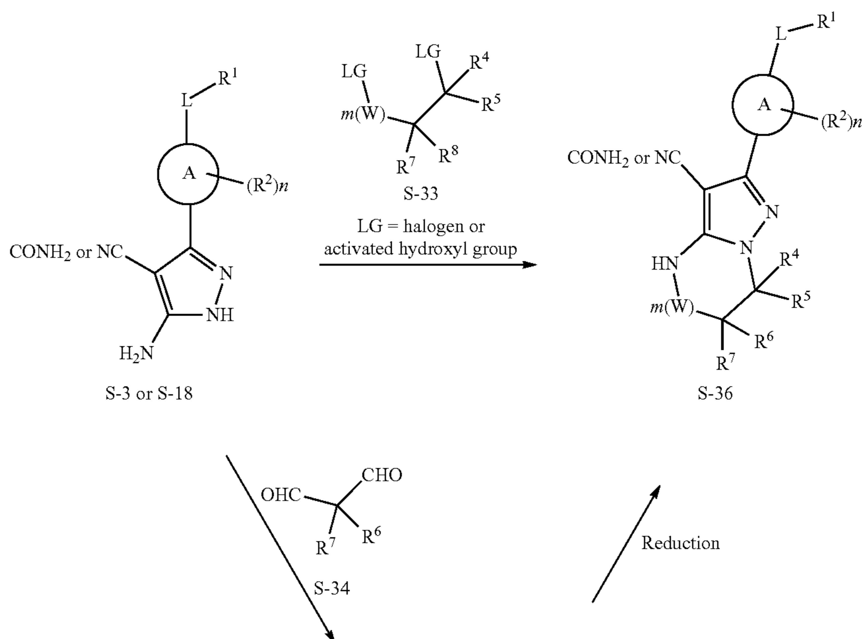
Scheme VIII
