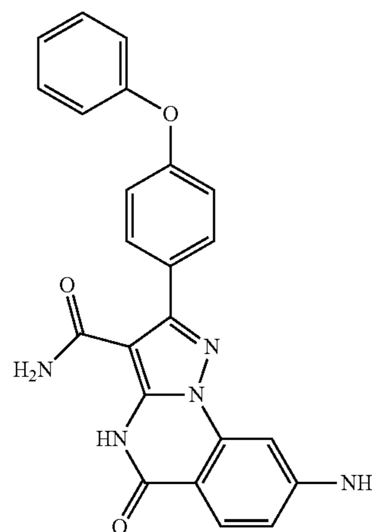
Compound 79: 8-Amino-5-oxo-2-(4-phenoxyphenyl)-4,5-dihydropyrazolo[1,5-a]quinazoline-3-carboxamide
