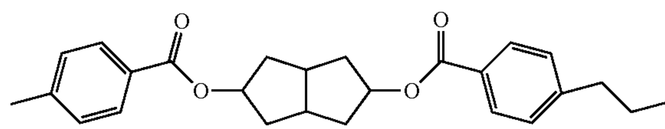
4-(7-(4-propylphenylcarbonyloxy)bicyclo[3.3.0]oct-2-yl)oxycarbonyl)phenyl
