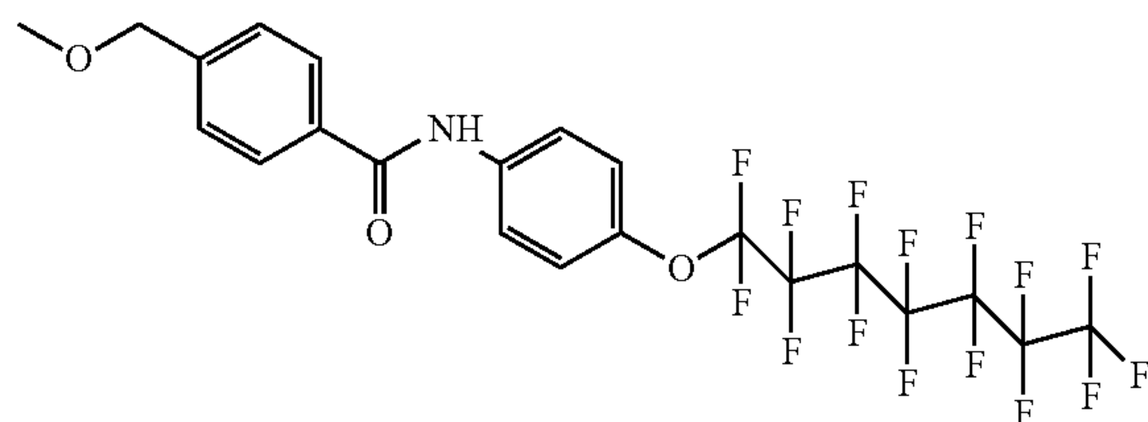
4-(4-(pentadecafluoroheptyloxy-phenylcarbamoyl)-benzyloxy)
