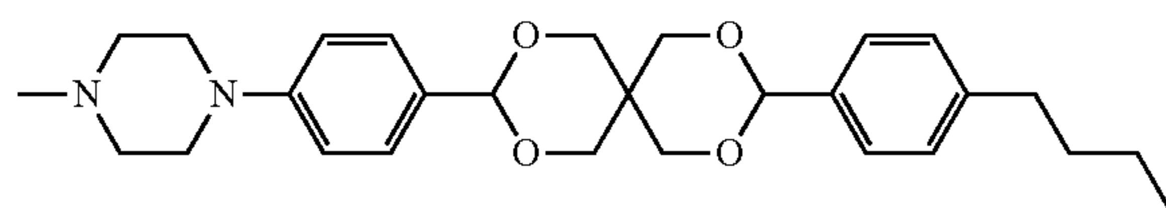
4-(4-(9-(4-butylphenyl)-2,4,8,10-tetraoxaspiro[5.5]undec-3-yl)phenyl)piperazin-1-yl
