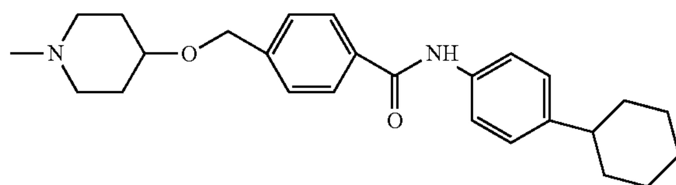
4-[4-(4-cyclohexyl-phenylcarbamoyl)-benzyloxy]-piperidin-1-yl
