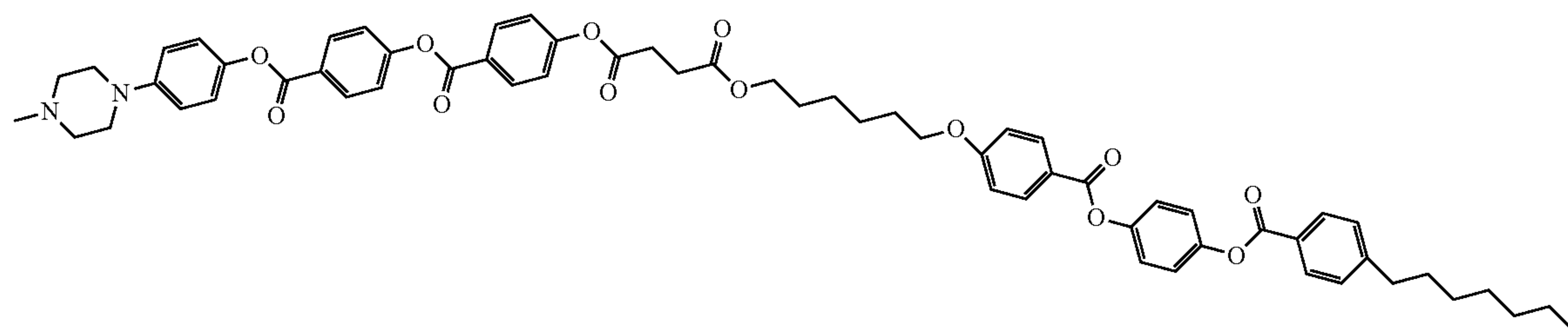
4-[4-(4-{4-[3-(6-{4-[4-(4-nonyl-benzoyloxy)-phenoxy]-hexyloxy]-propionyloxy]-benzoyloxy}-benzoyloxy)-phenyl]-piperazin-1-yl
