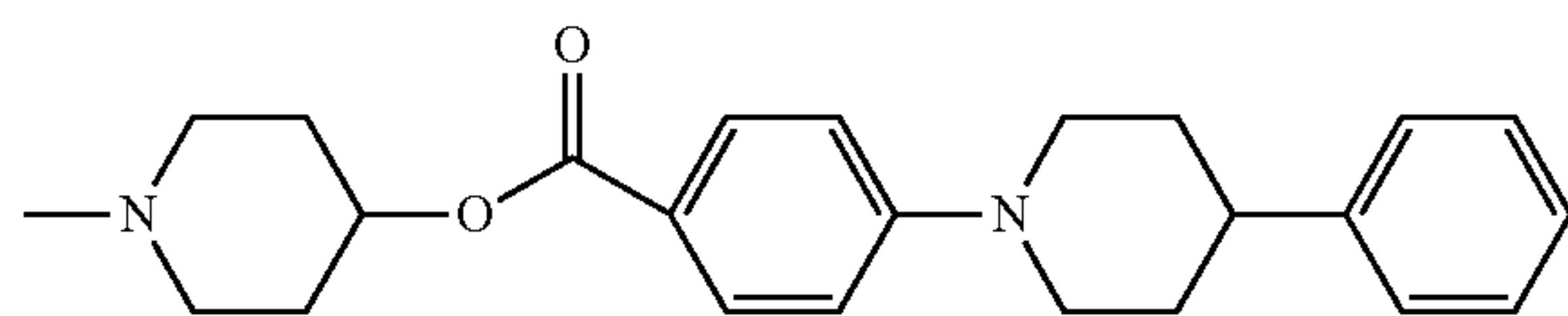
4-(4-(4-phenylpiperidin-1-yl)-benzoyloxy)-piperidin-1-yl
