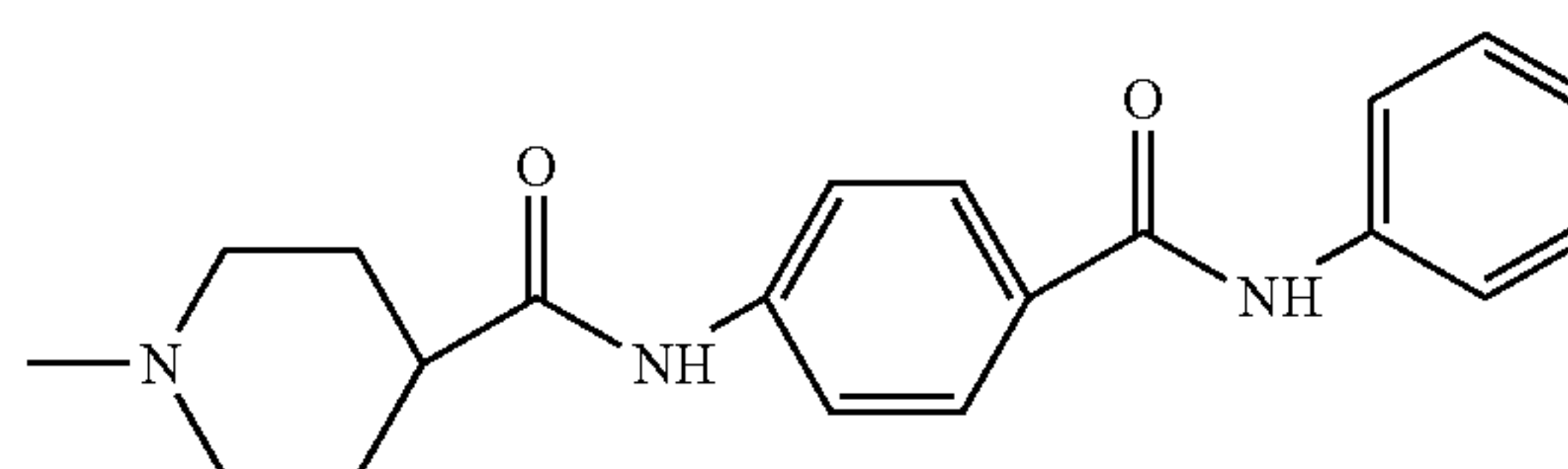
4-(4-phenyl-carbamoyl-phenyl-carbamoyl)-piperidin-1-yl
