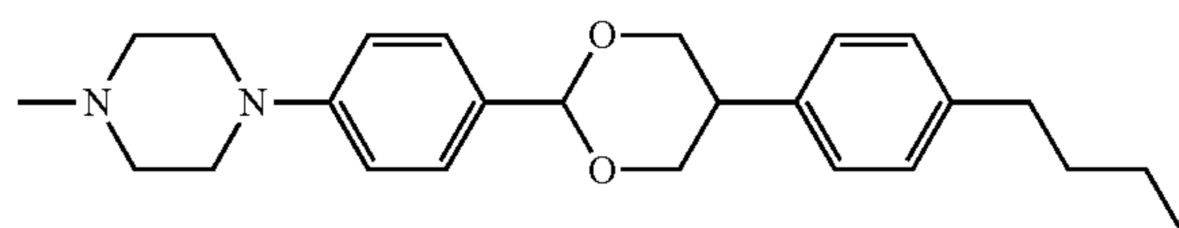
1-{4-[5-(4-butyl-phenyl)-[1,3]dioxan-2-yl]-phenyl}-4-methyl-piperazin-1-yl
