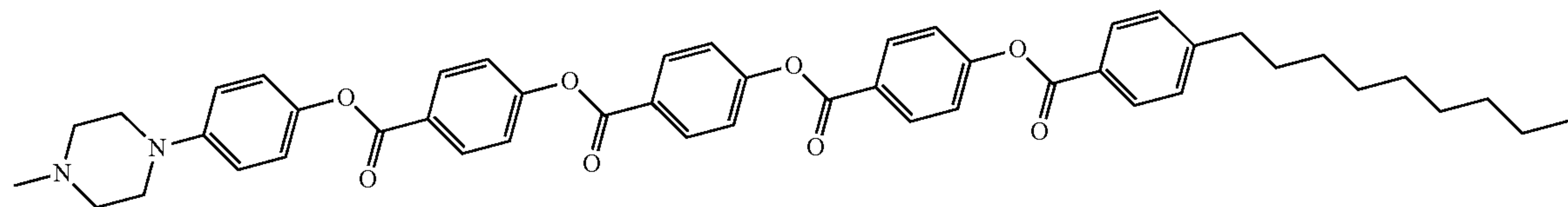
{4-[4-(4-{4-[4-(4-nonyl-benzoyloxy)-benzoyloxy]-benzoyloxy}-benzoyloxy)-phenyl]-piperazin-1-yl}
