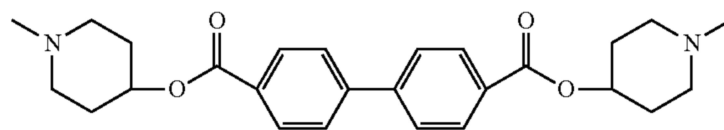
biphenyl-4,4'-dicarboxylic acid bis-[1-Name of PC Group]-piperidin-4-yl ester
