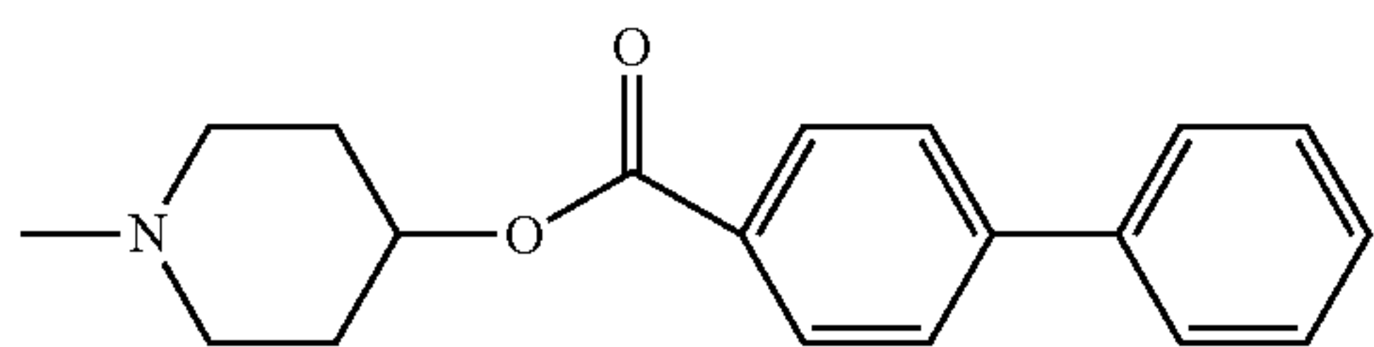
4-(biphenyl-4-carbonyloxy)-piperidin-1-yl
