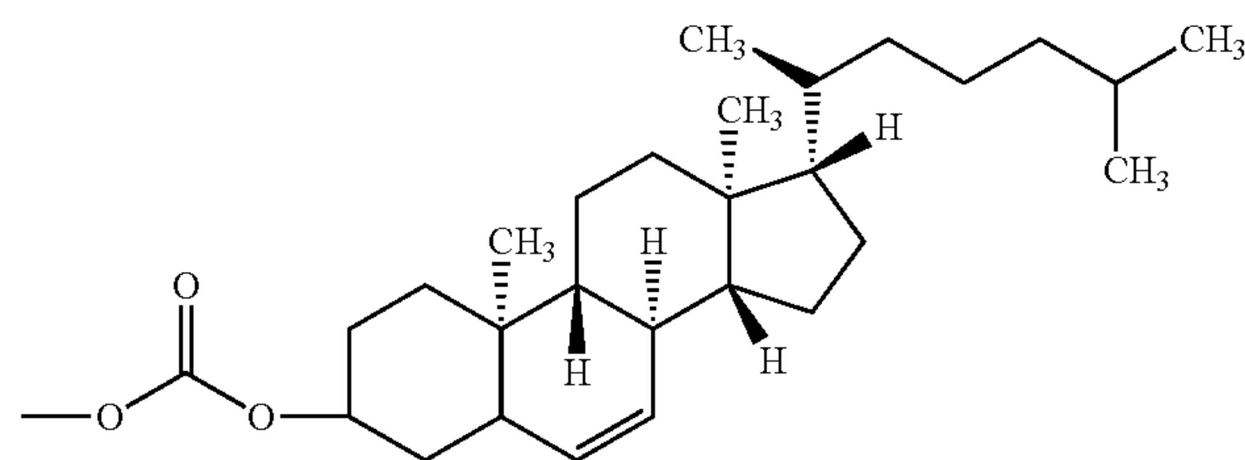
4-[17-(1,5-dimethyl-hexyl)-10,13-dimethyl-2,3,4,7,8,9,10,11,12,13,14,15,16,17-tetradecahydro-1H-cyclopenta[a]phenanthren-3-yloxy]carbonyloxy
