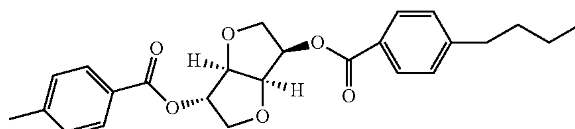
4-(6-(4-butylphenyl)carbonyloxy-(4,8-dioxabicyclo[3.3.0]oct-2-yl)oxycarbonyl)phenyl
