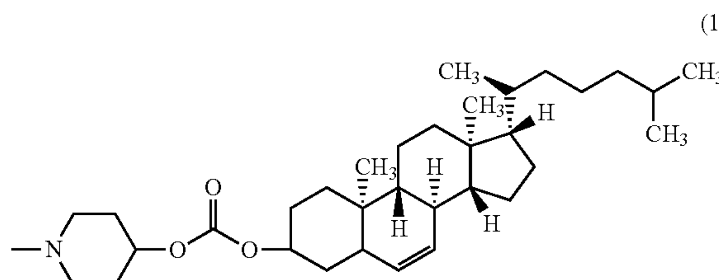
4-[17-(1,5-dimethyl-hexyl)-10,13-dimethyl-2,3,4,7,8,9,10,11,12,13,14,15,16,17-tetradecahydro-1H-cyclopenta[a]phenanthren-3-yloxy-carbonyloxy]-piperidin-1-yl
