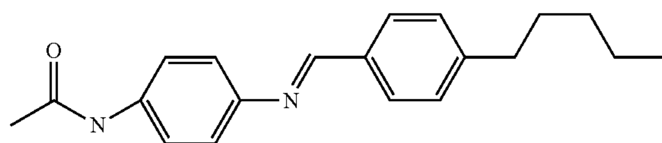
N-{4-[(4-pentyl-benzylidene)-amino]-phenyl}-acetamidyl
