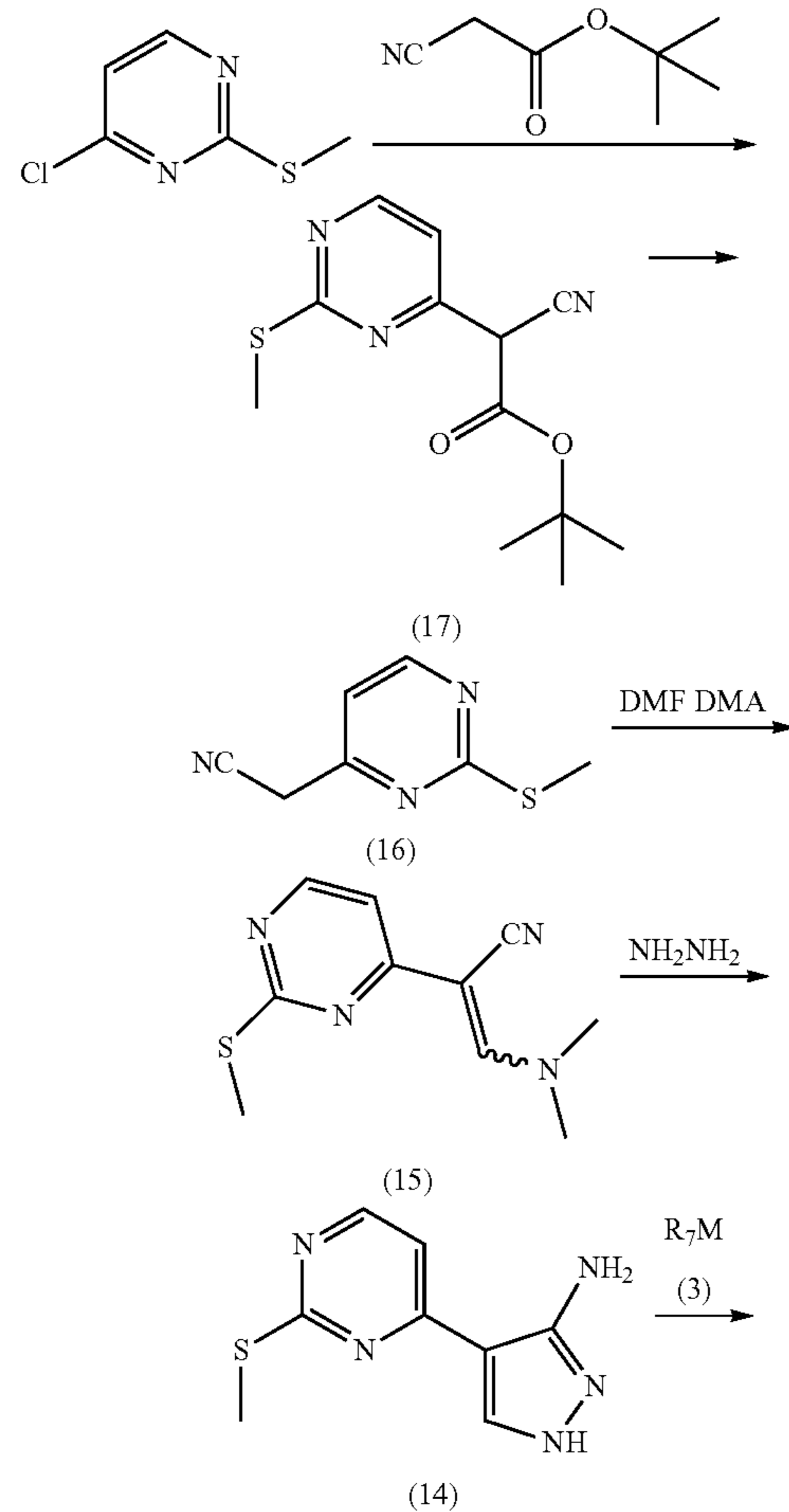
Reaction Scheme V
