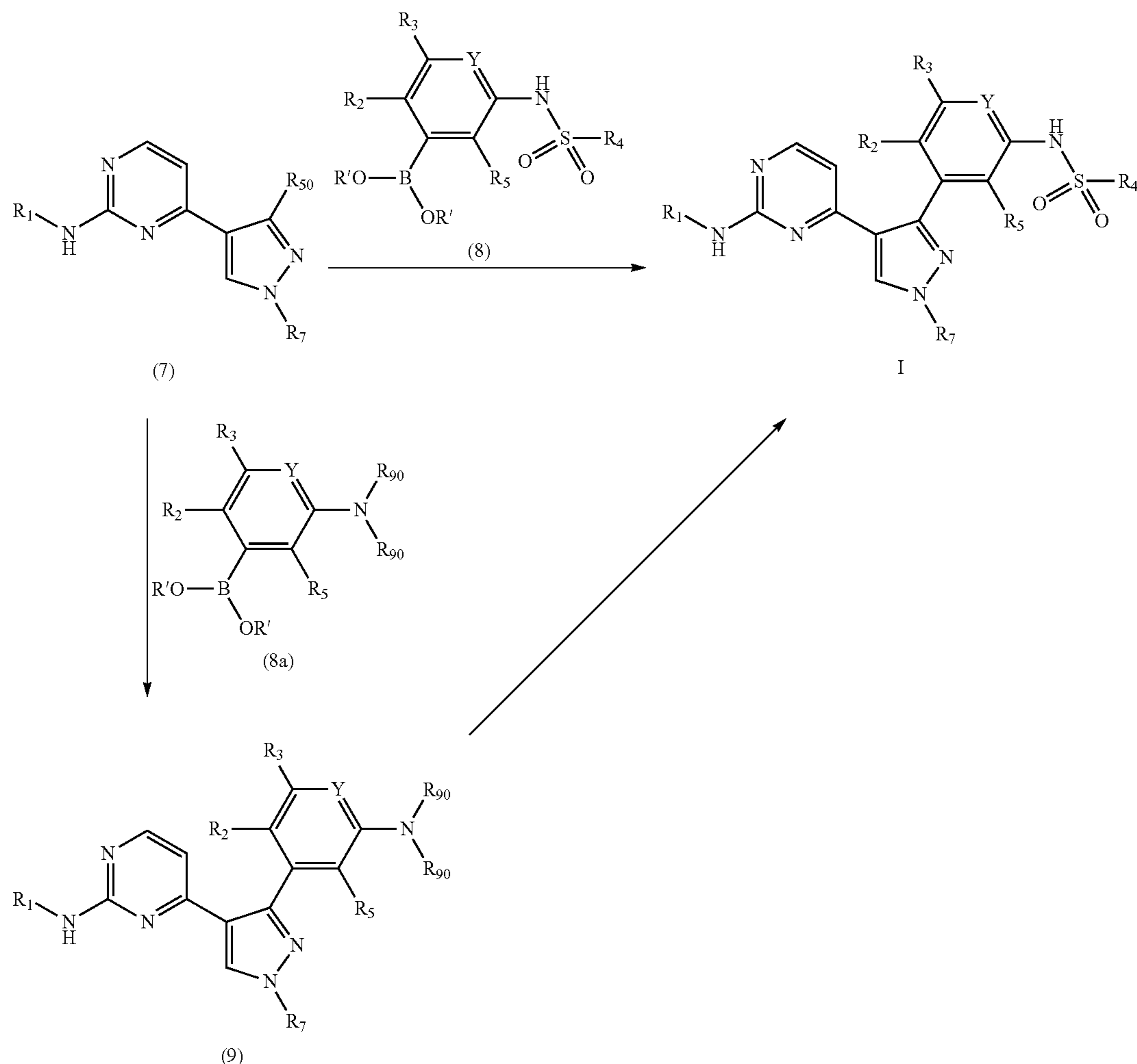
Reaction Scheme III
