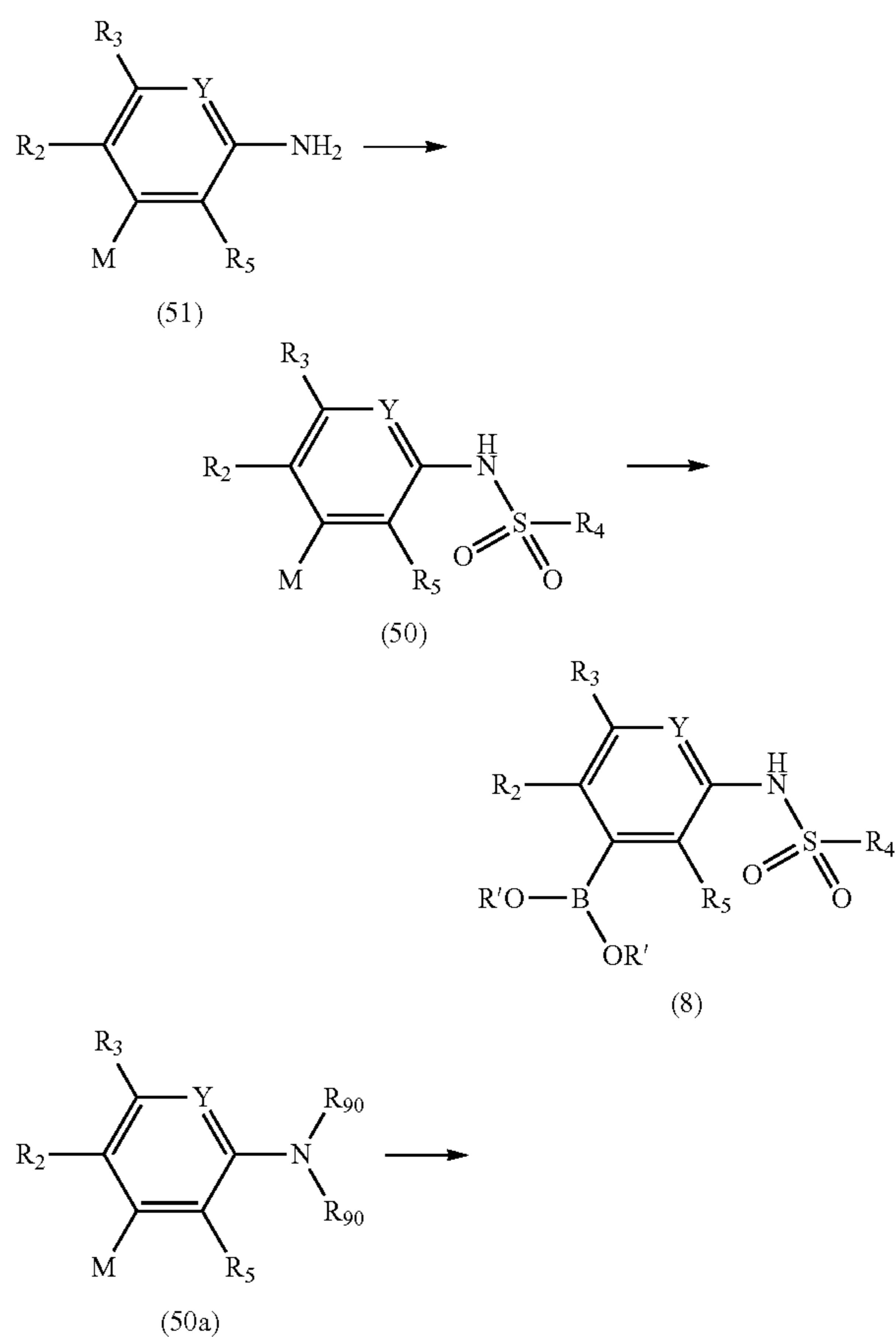
Reaction Scheme VII
