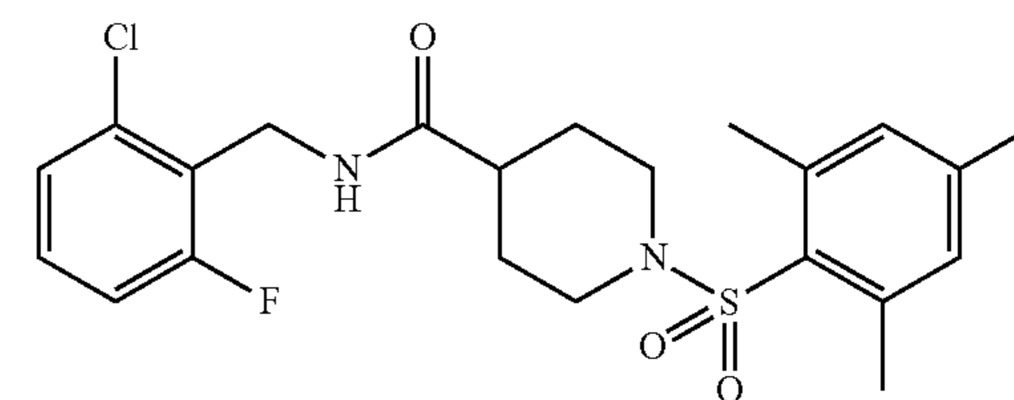
COMPOUND 8-42
