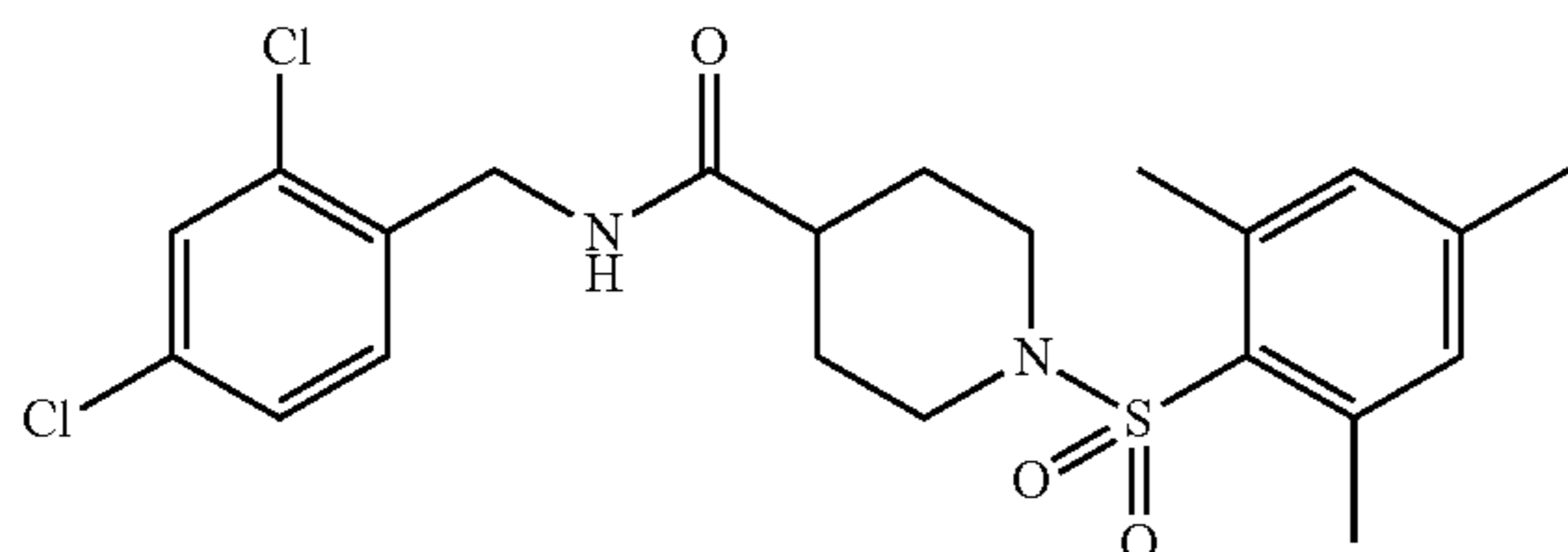
COMPOUND 1
