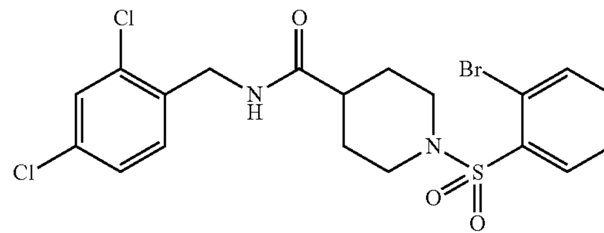
COMPOUND 8-9
