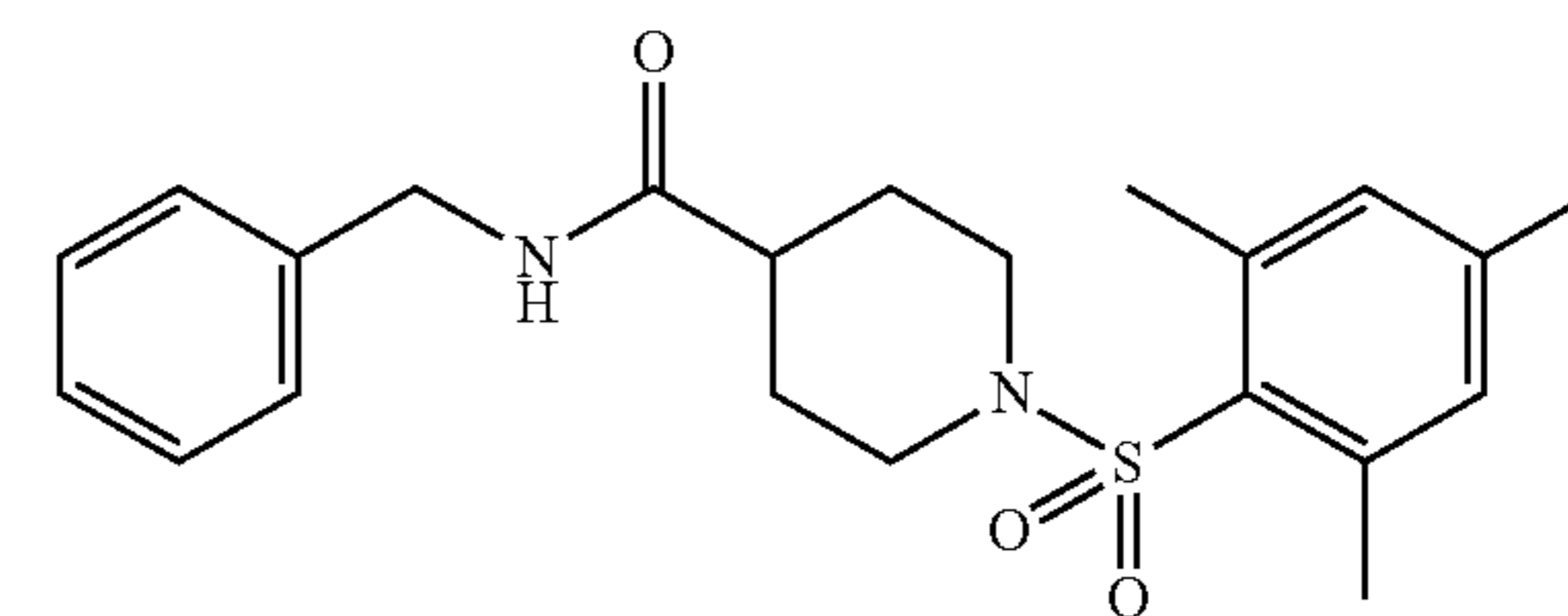
COMPOUND 8-14
