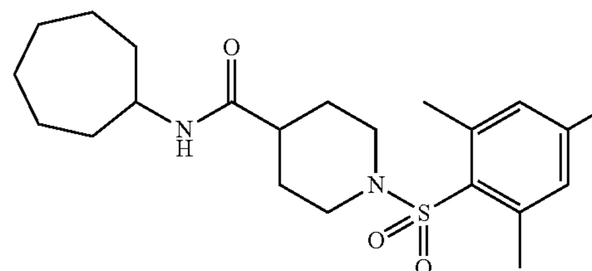
COMPOUND 8-47
