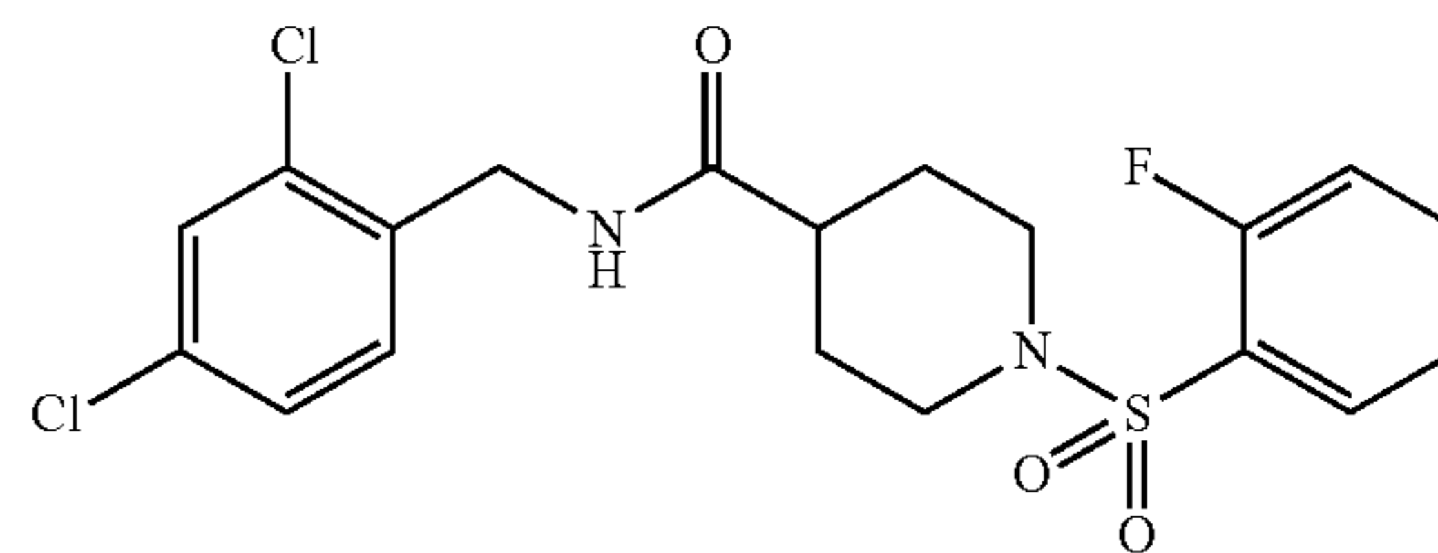
COMPOUND 6-6(b)
