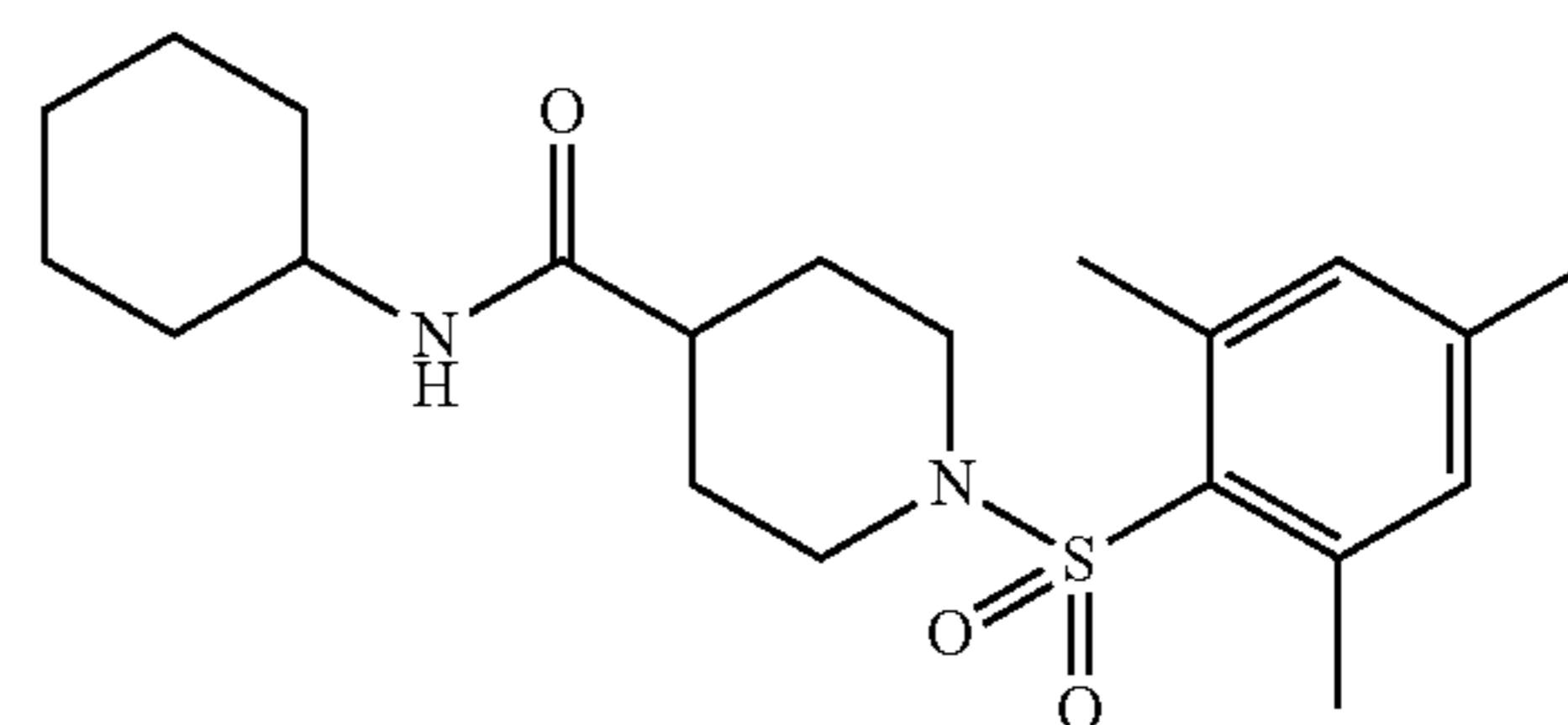
COMPOUND 8-37
