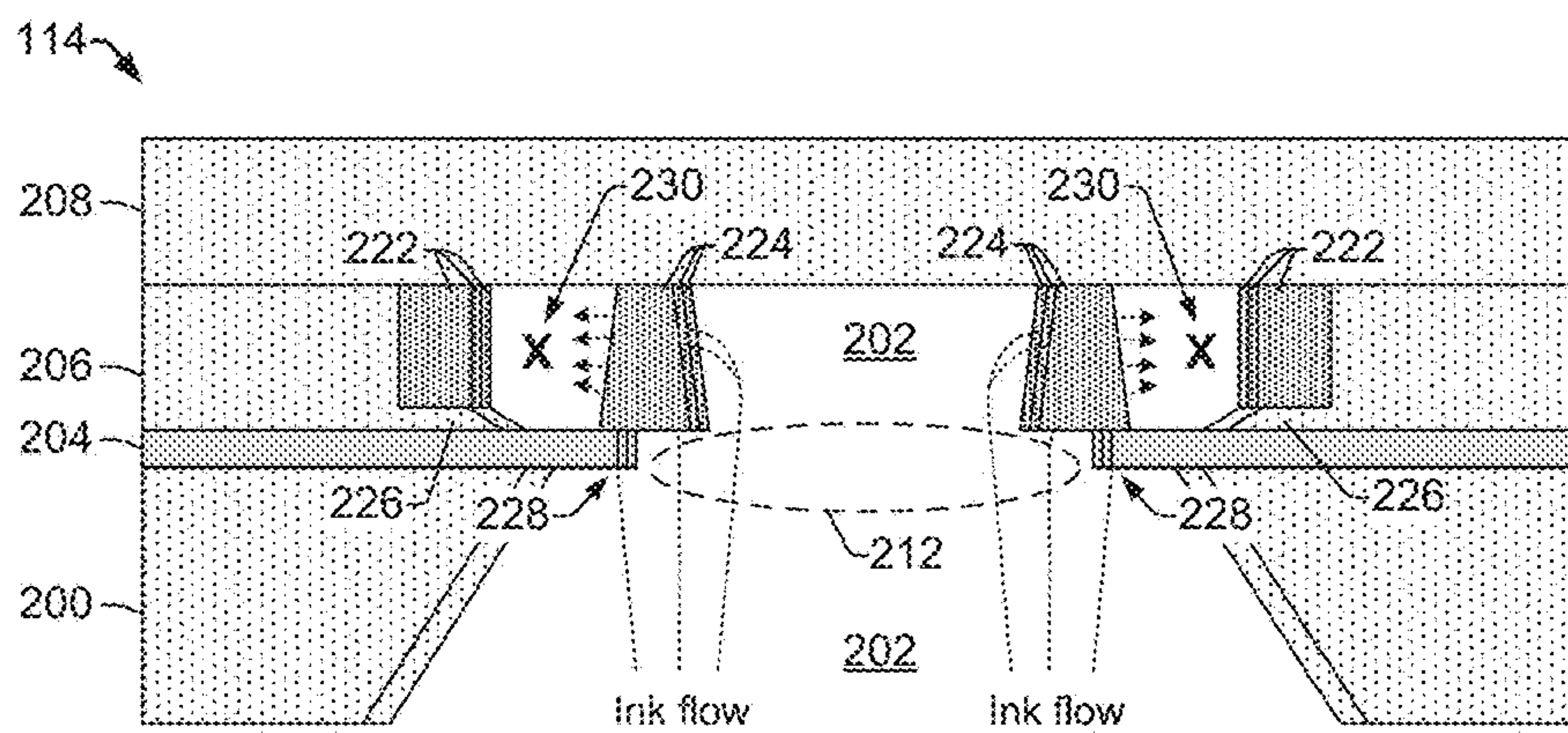
View A-A from FIG. 2
