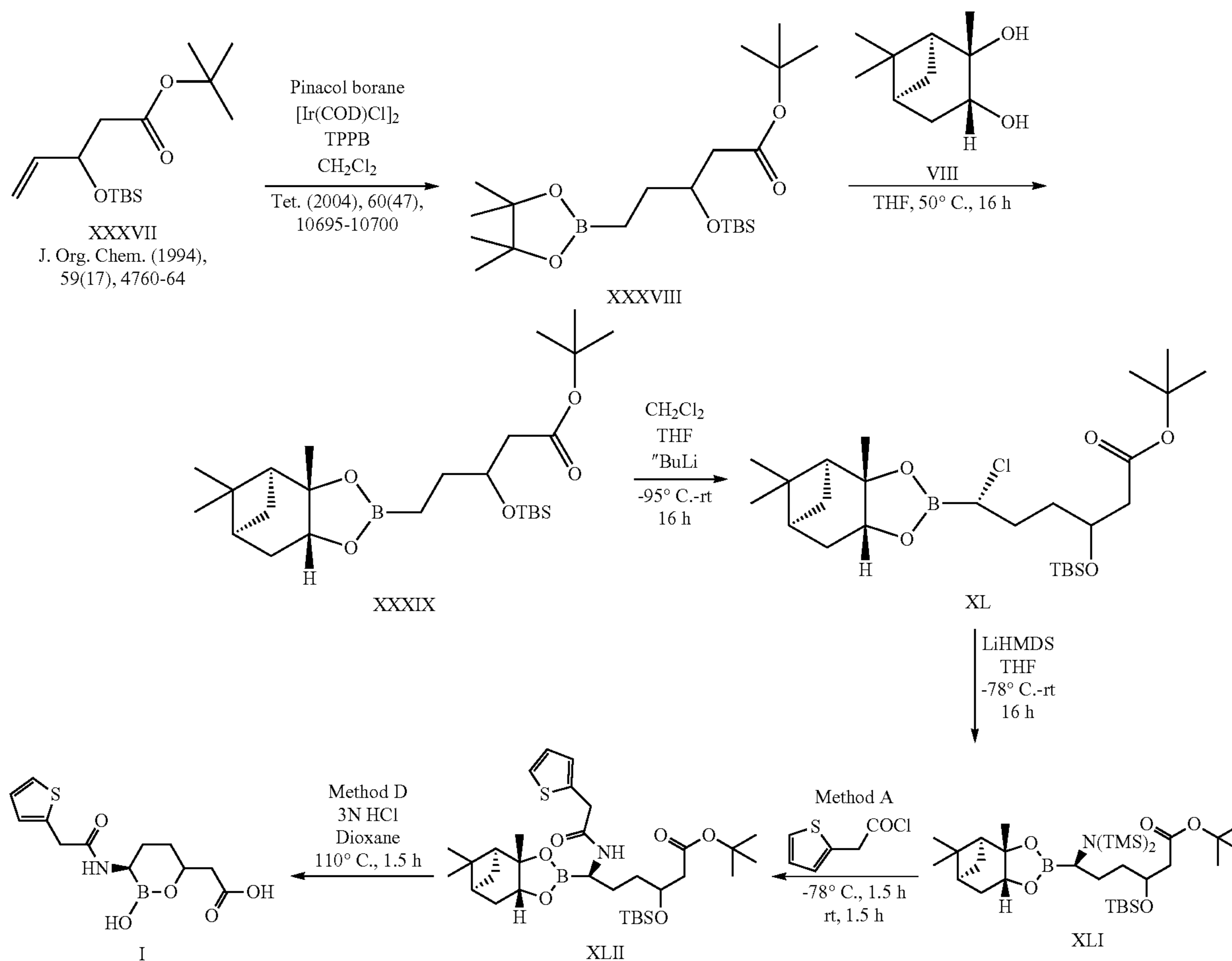
Scheme 8
