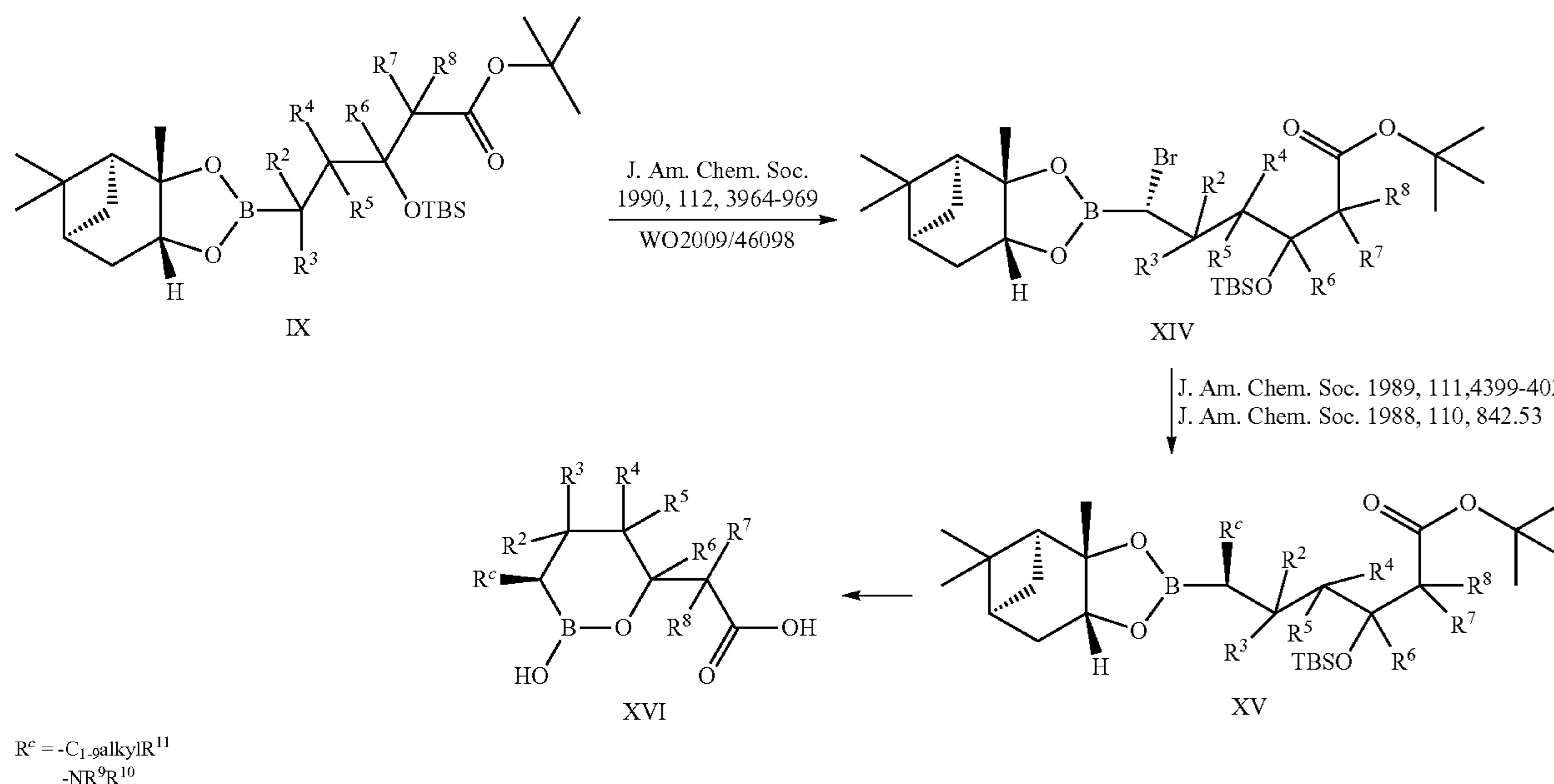
Scheme 2
