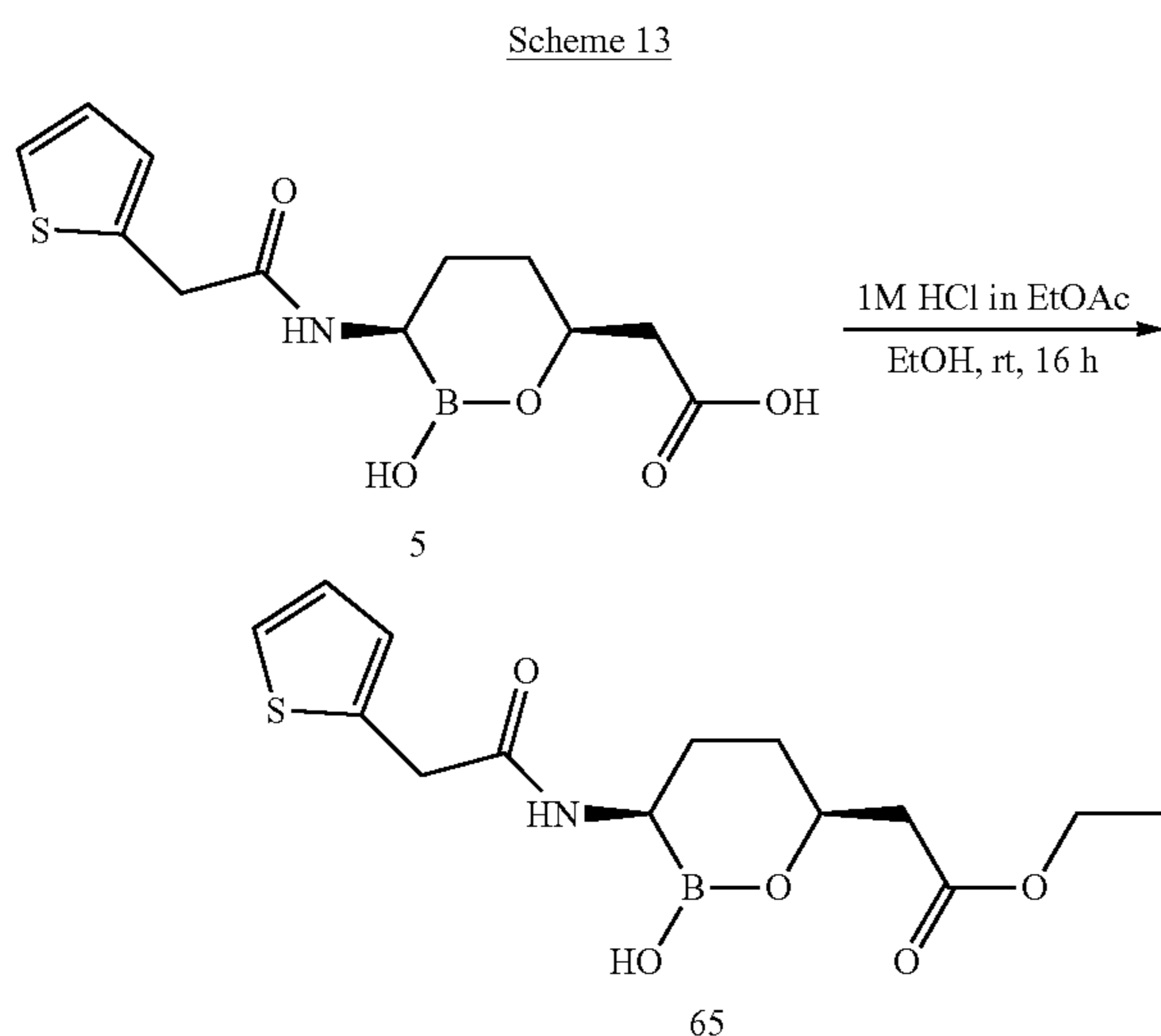
Example 5
