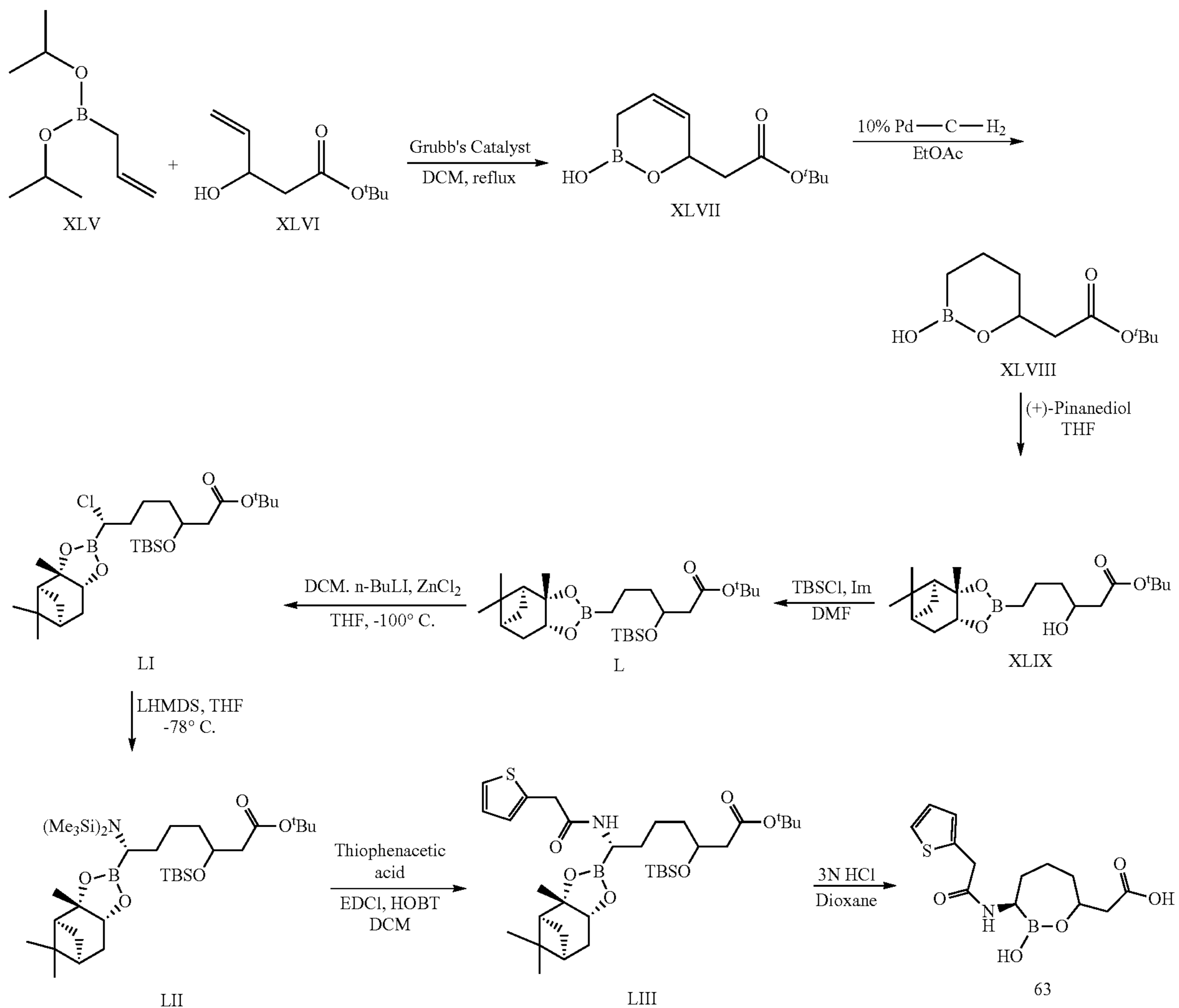
Scheme 11
