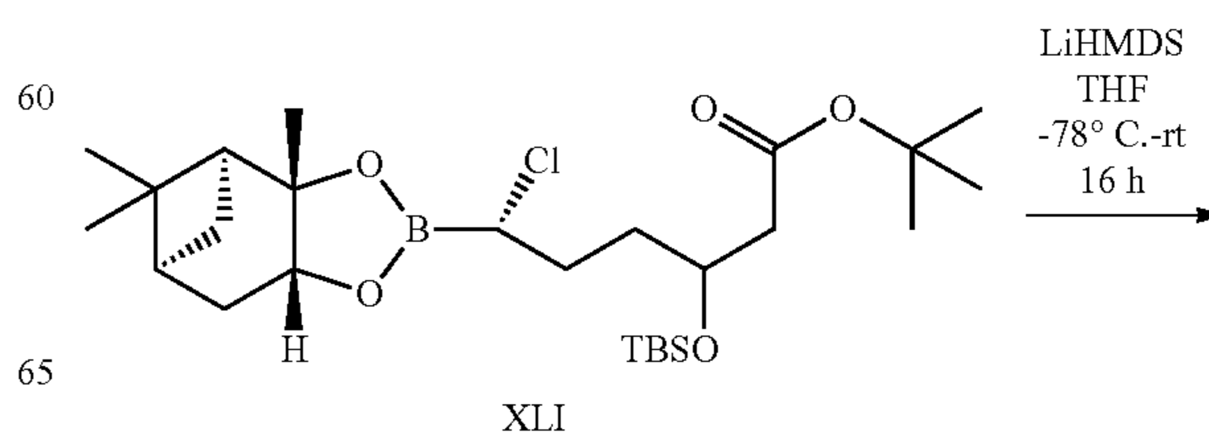
Scheme 10
