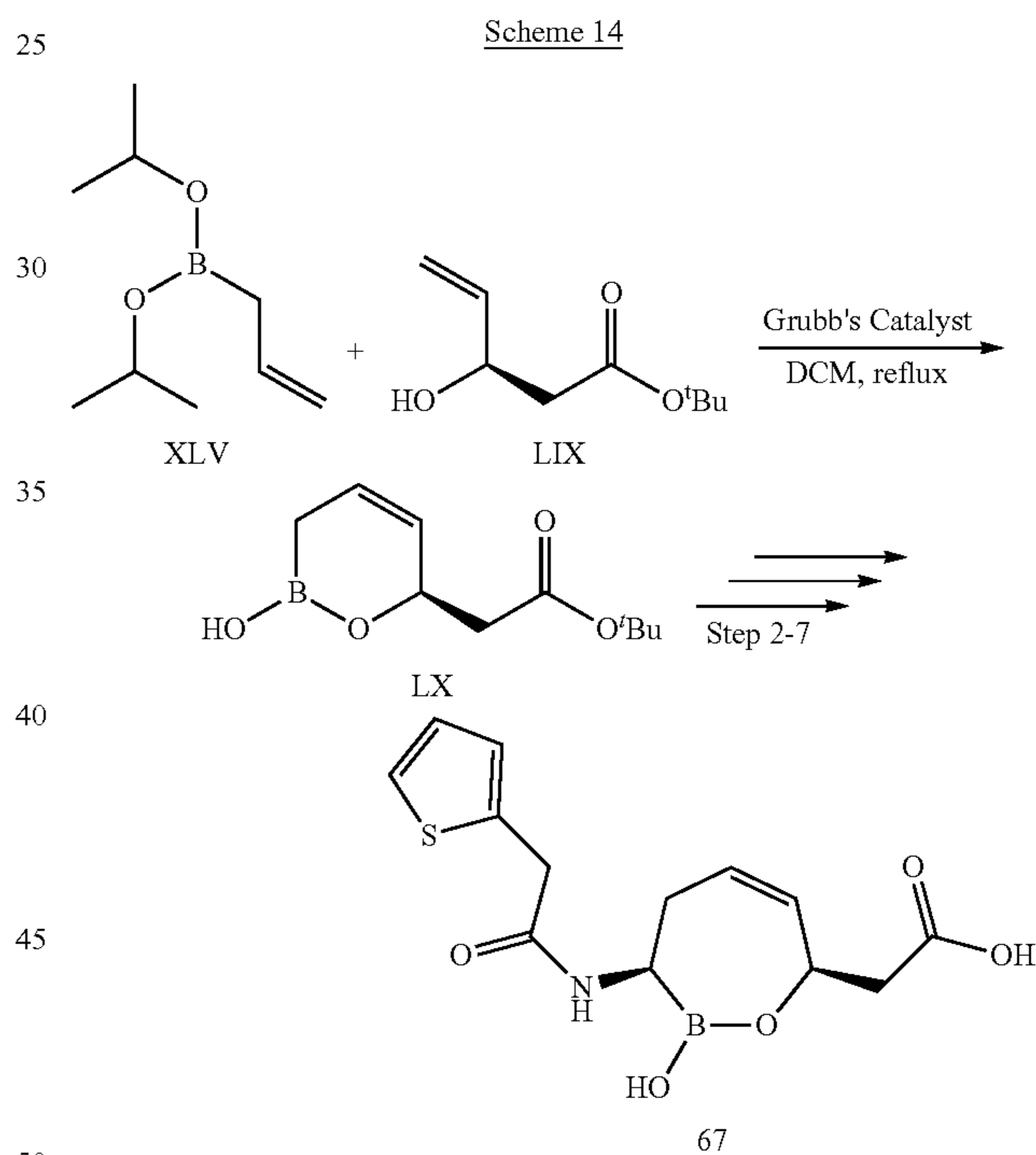
Example 6
