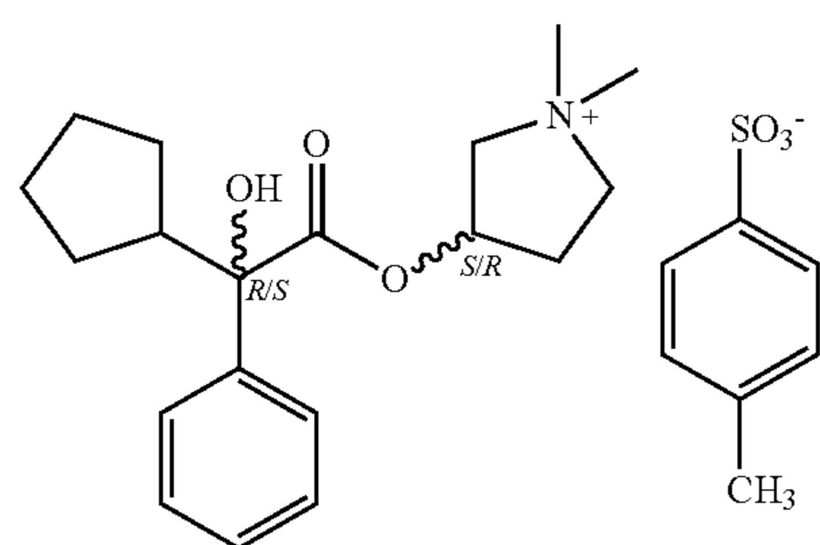
Glycopyrrolate tosylate (threo pair) FW = 489.62
