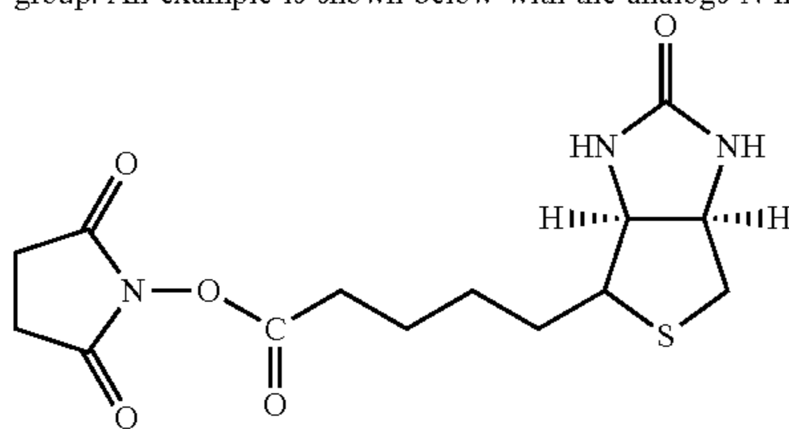
N-hydroxysuccinimide biotin
