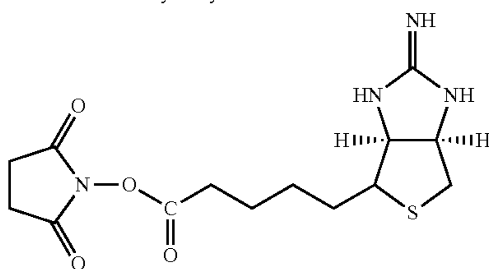
N-hydroxysuccinimide iminobiotin
