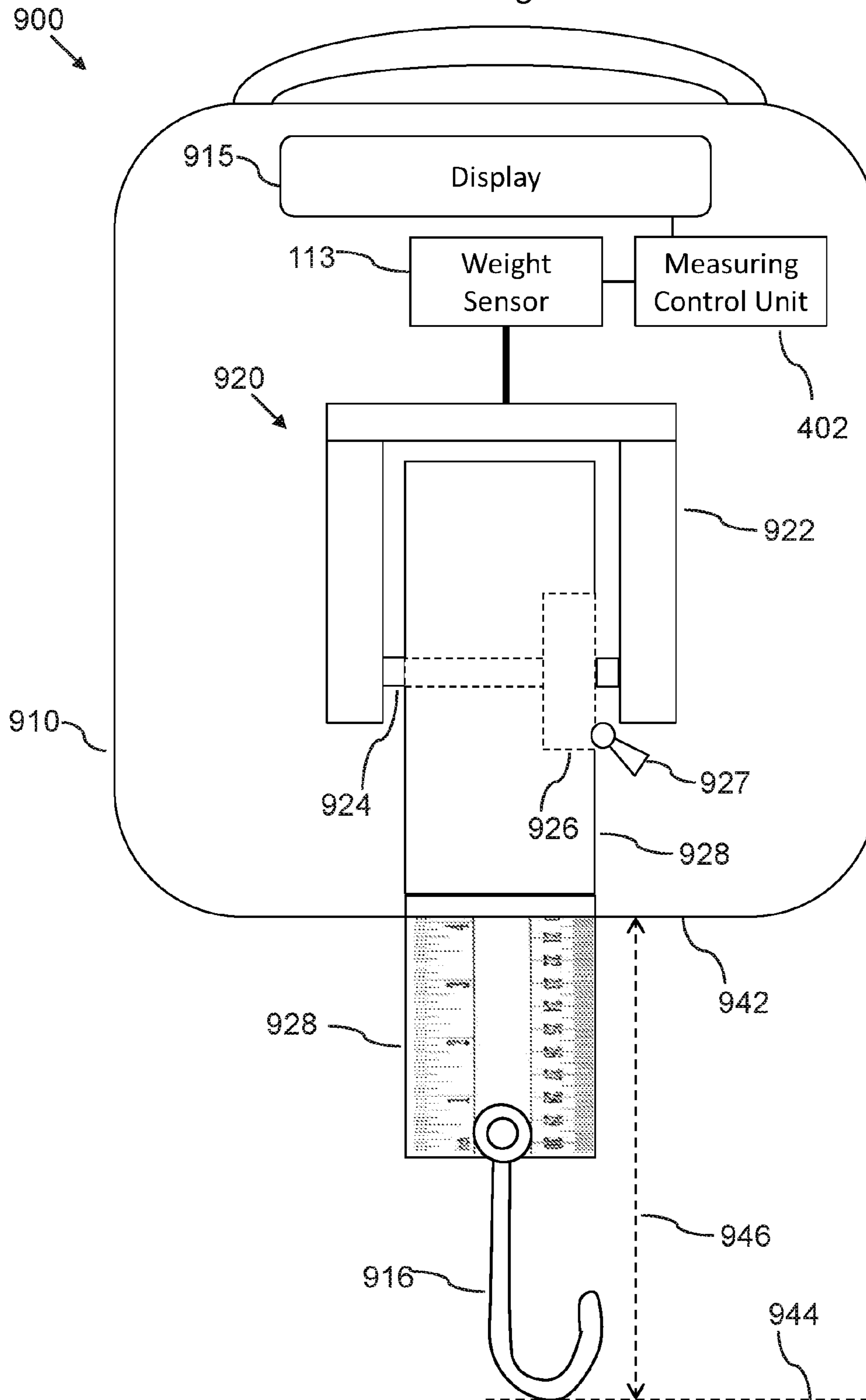
FIG. 9 Measuring Device
