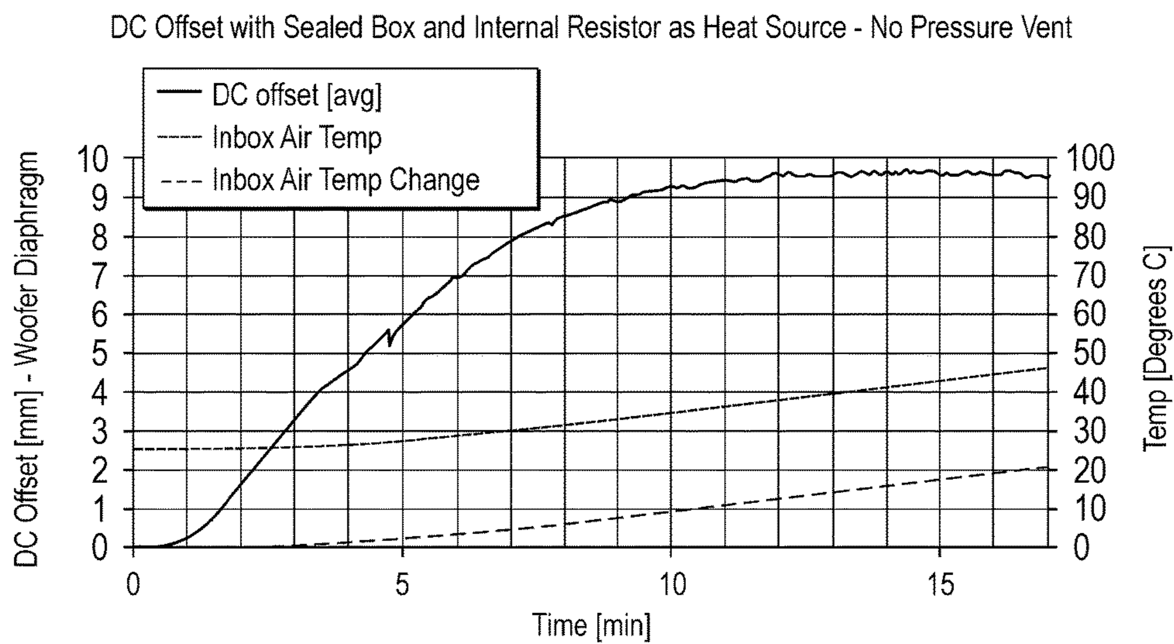
FIG. 10 (Prior Art)
