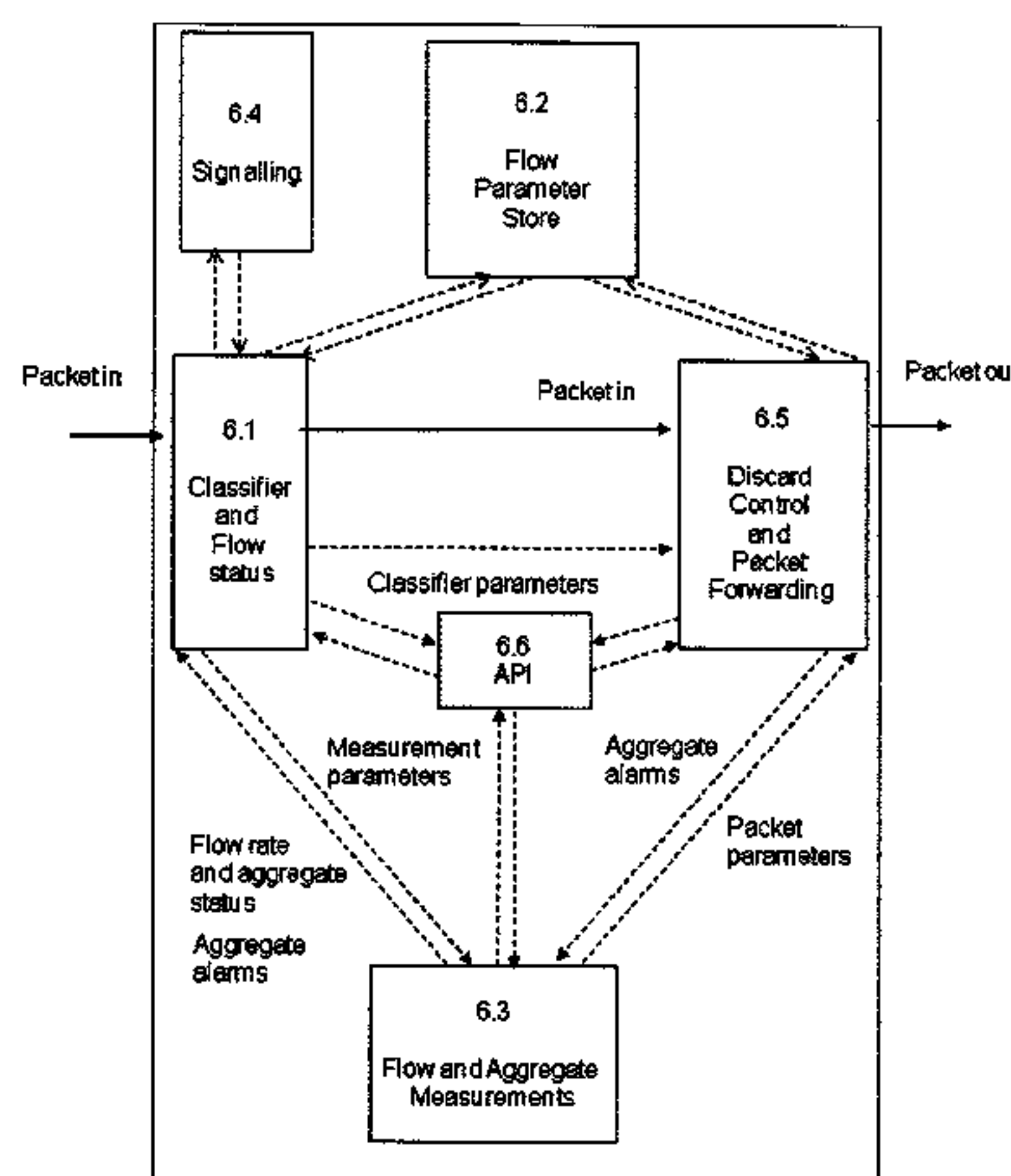
Another embodiment of function 6 with additional API function 6.6
