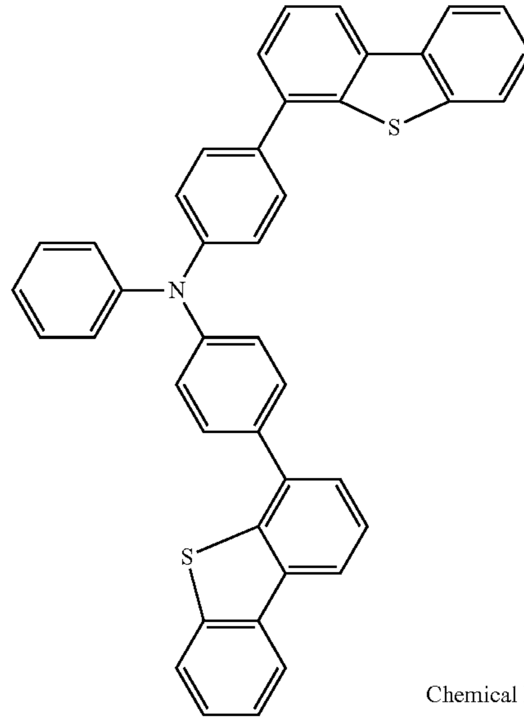
Chemical Formula 1-5
