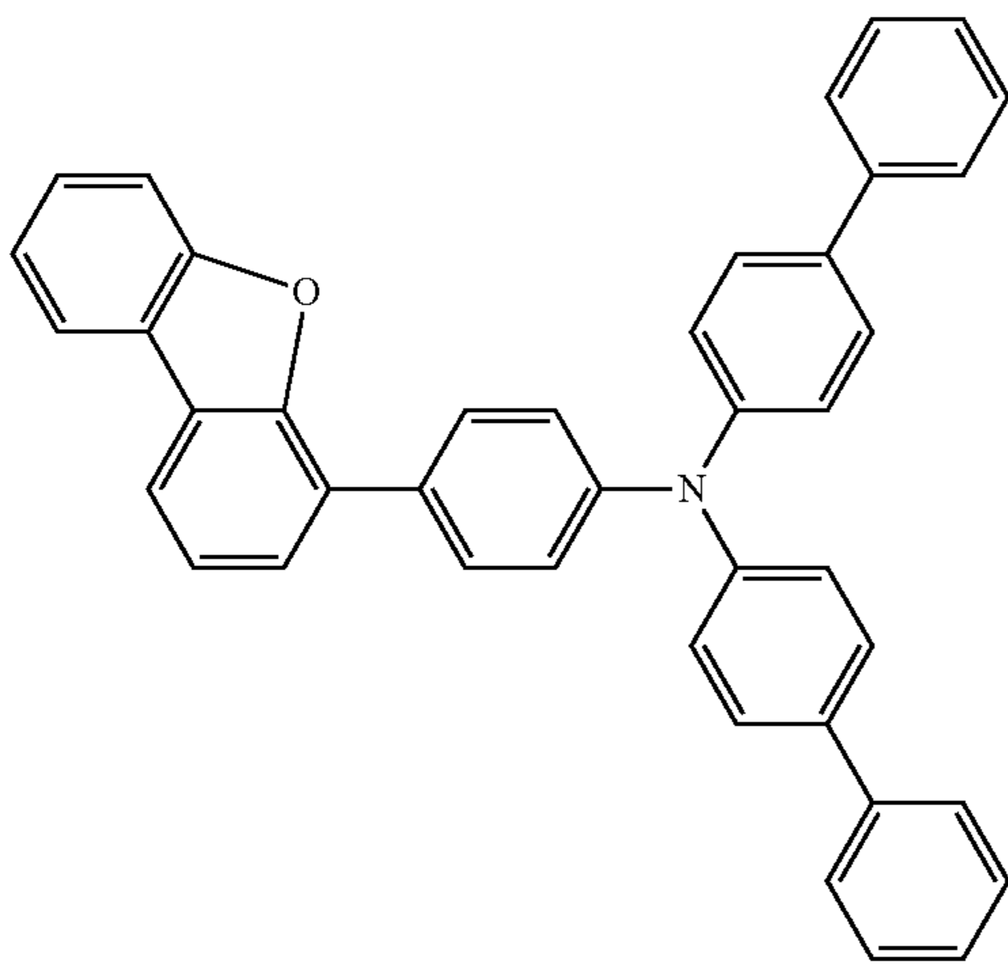
Chemical Formula 1-4
