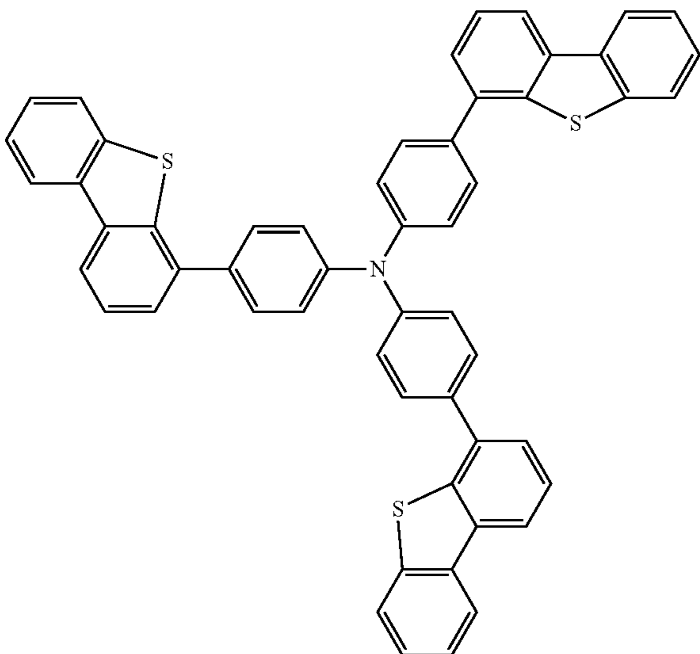
Chemical Formula 1-4
