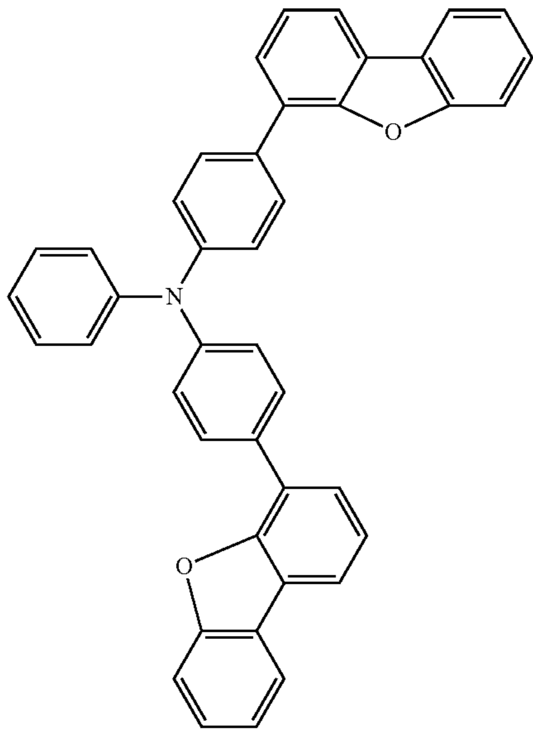
Chemical Formula 1-2
