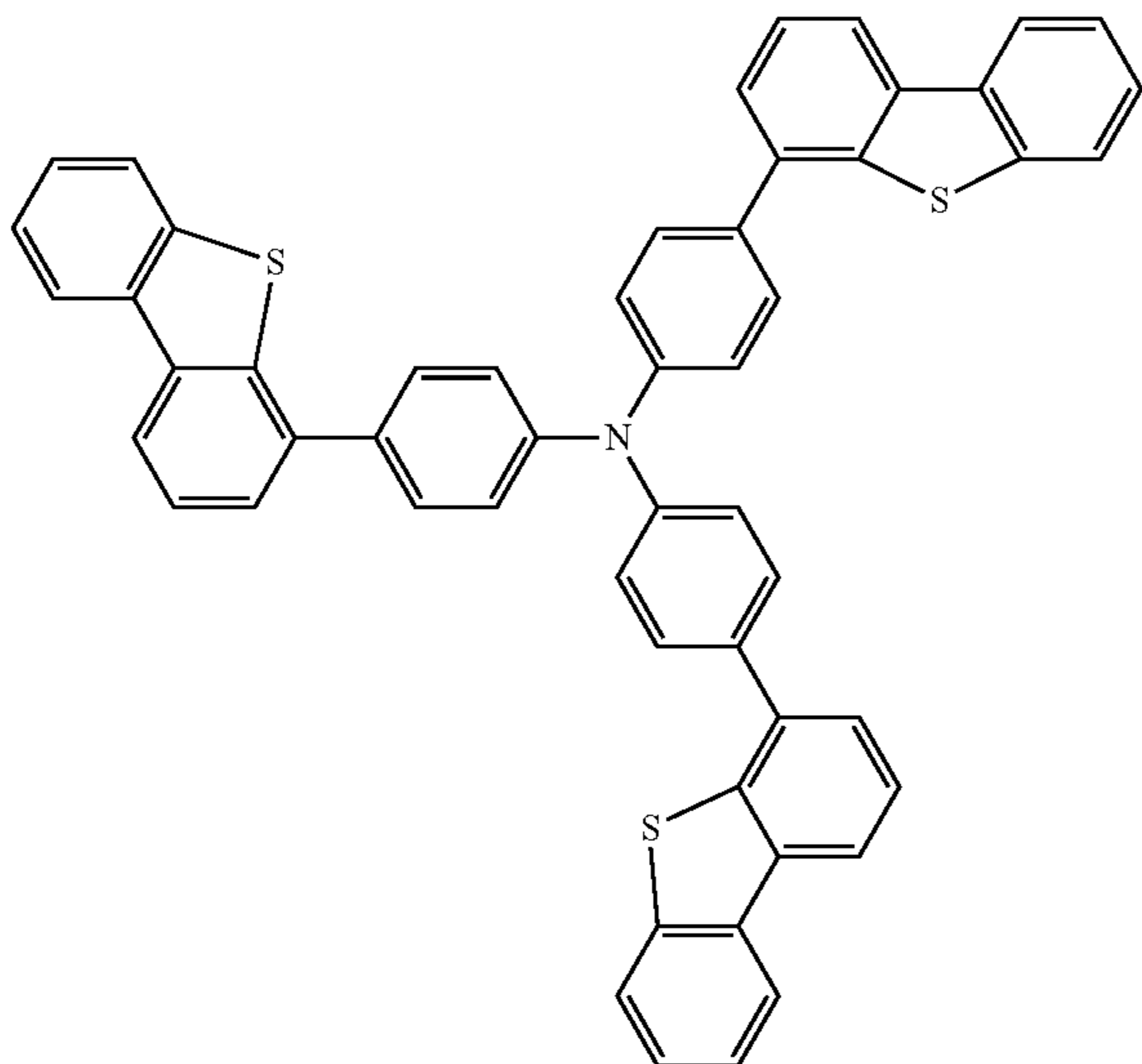
Chemical Formula 1-4
