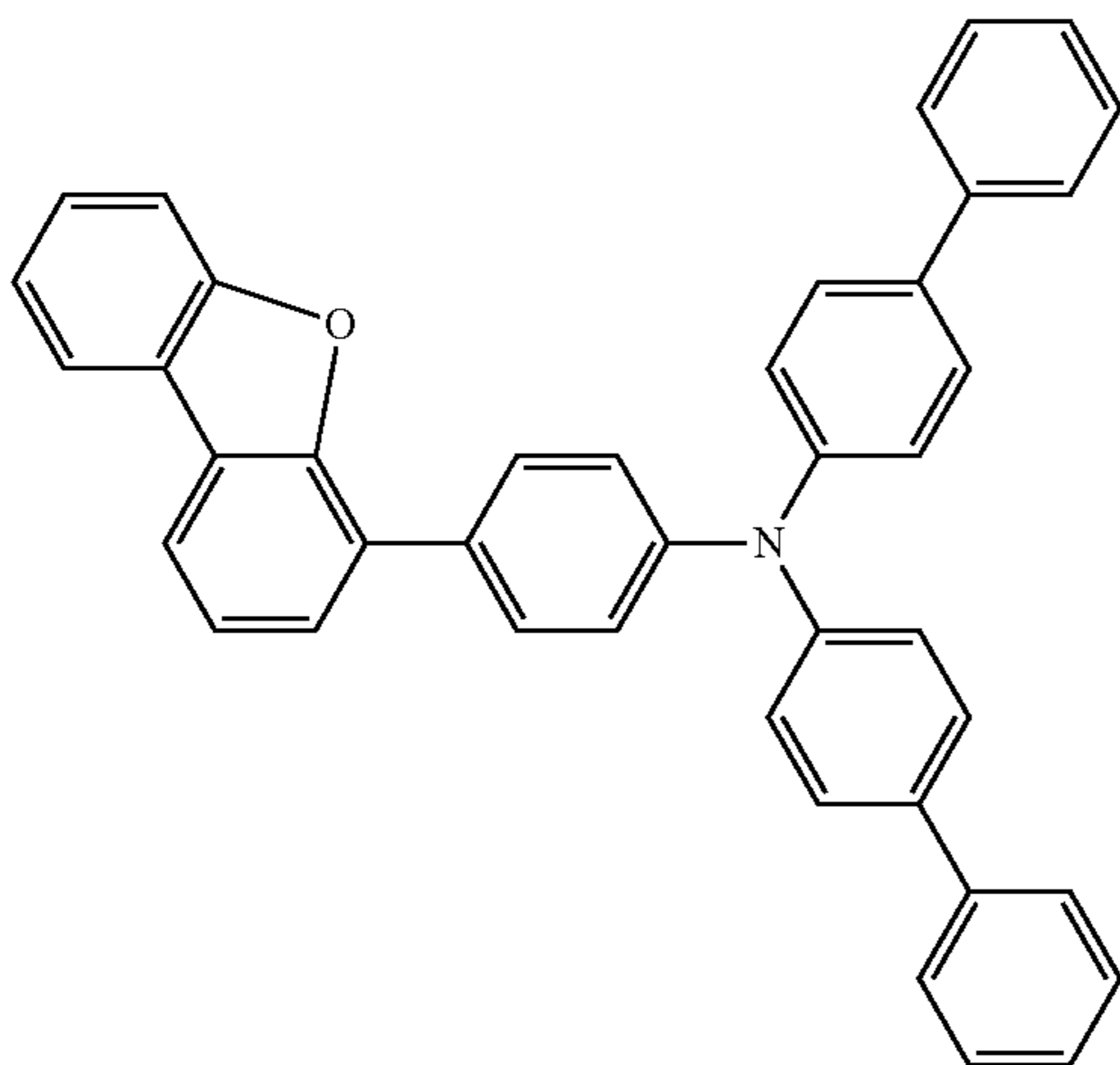
Chemical Formula 1-4
