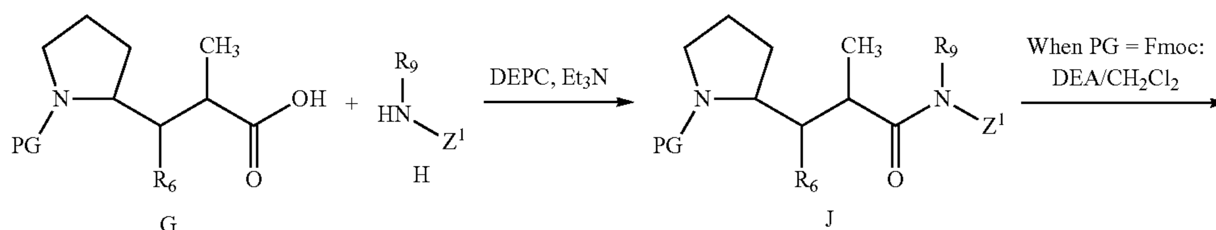
Scheme 6
