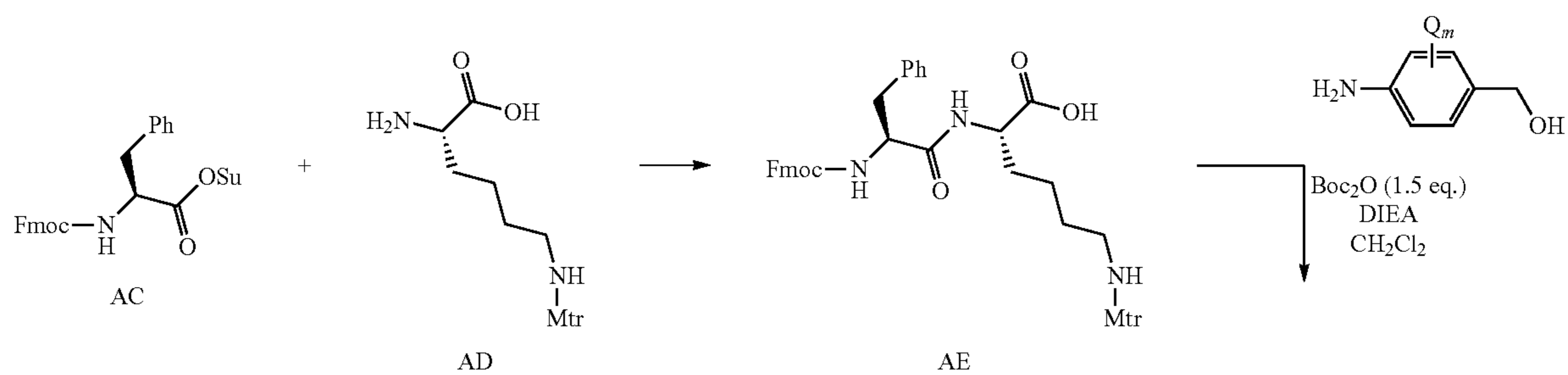
Scheme 12
