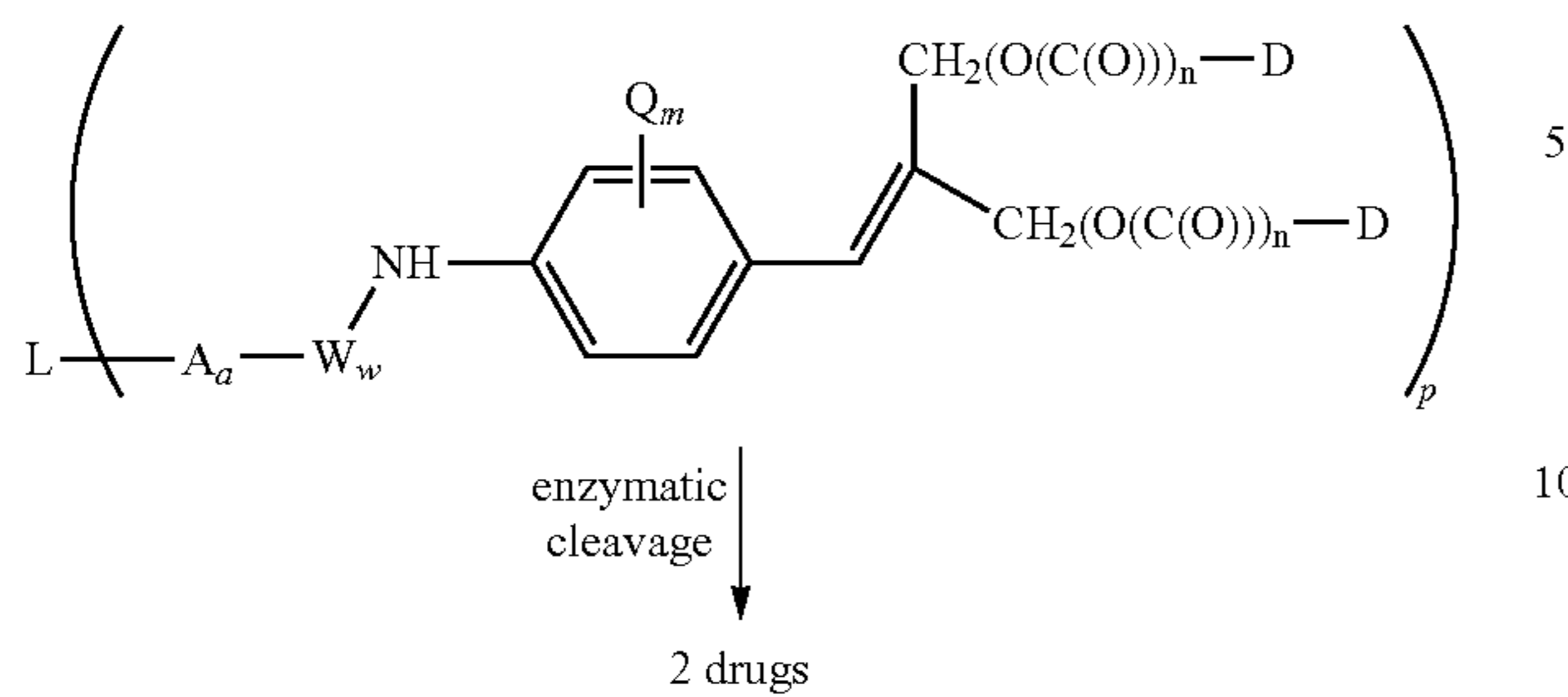
Scheme 4
