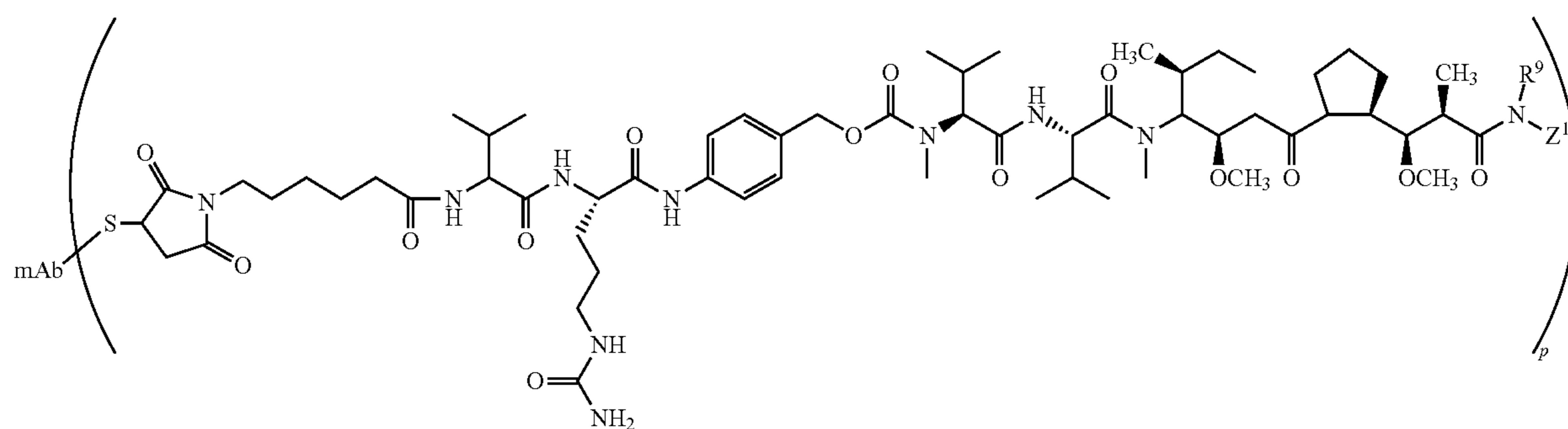
mAb-MC-vc-PAB-MMAZ
