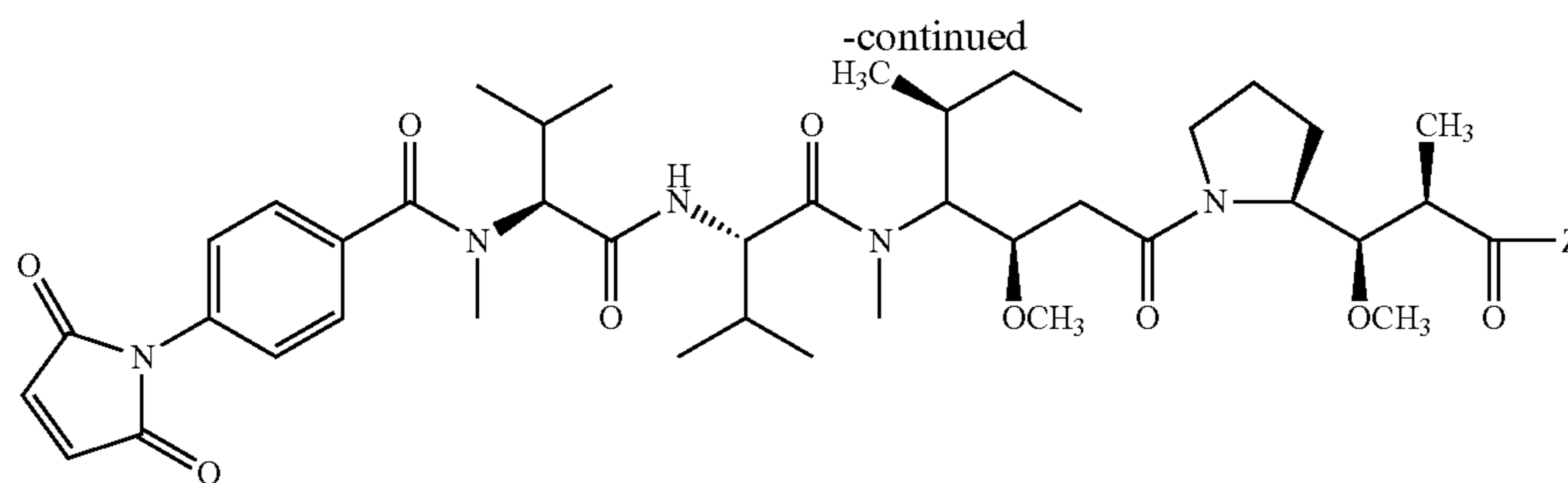
MB-MMAZ
