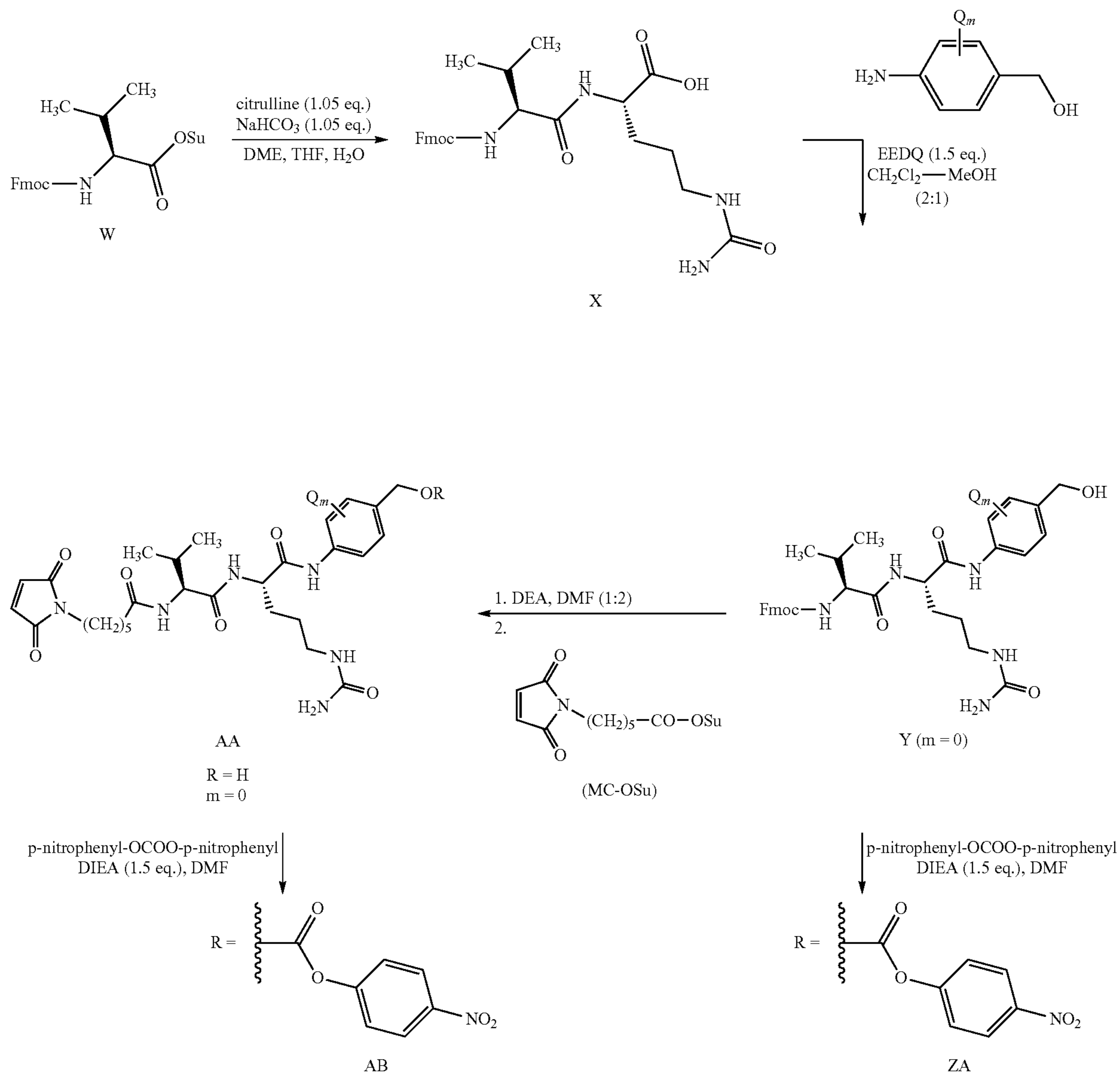
Scheme 11
