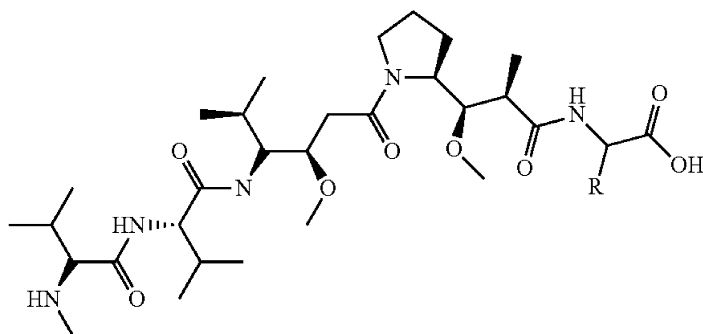
Drug Ib
