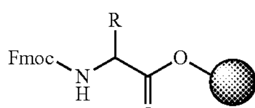
Compound SP1
