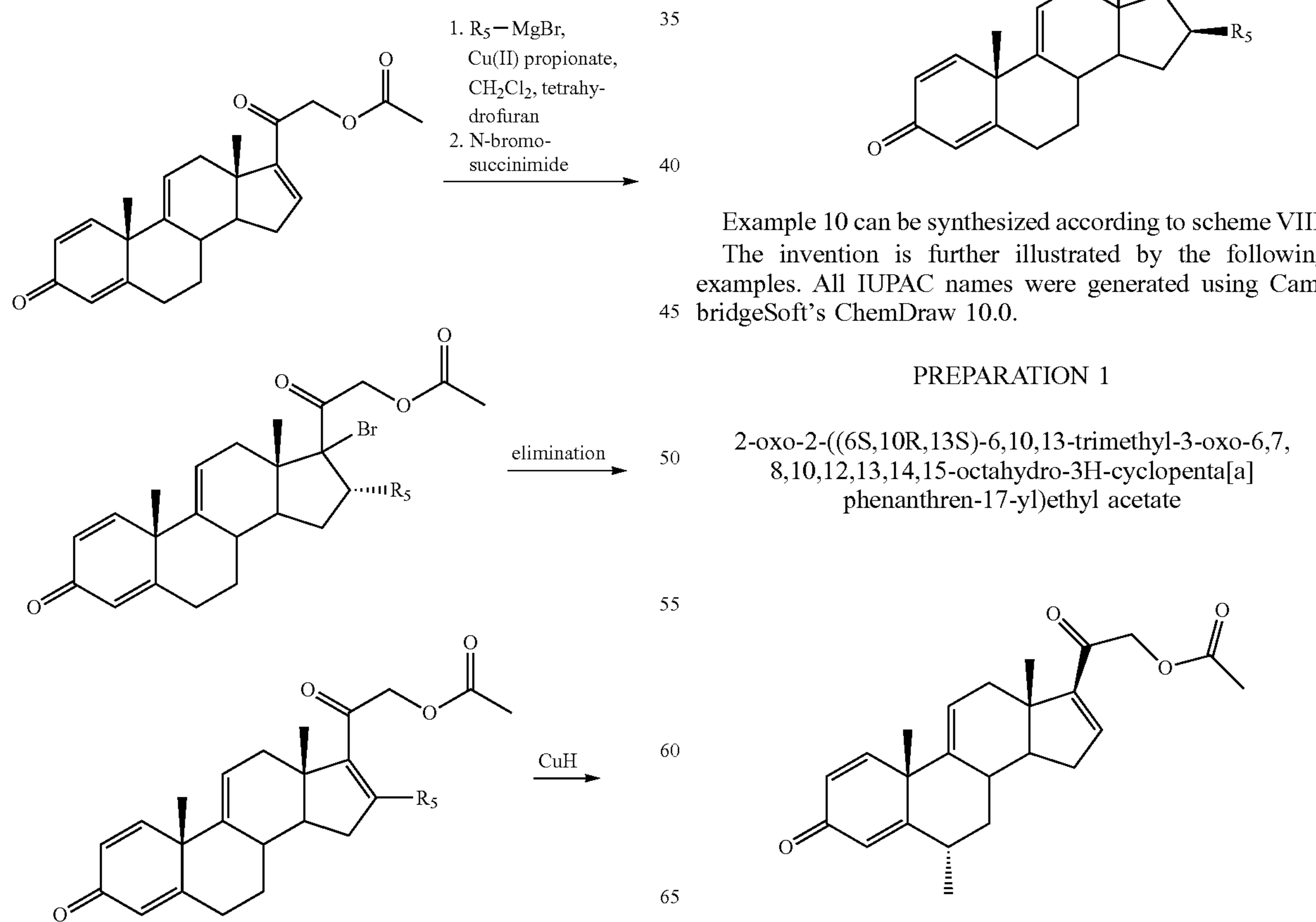
Scheme VIII
