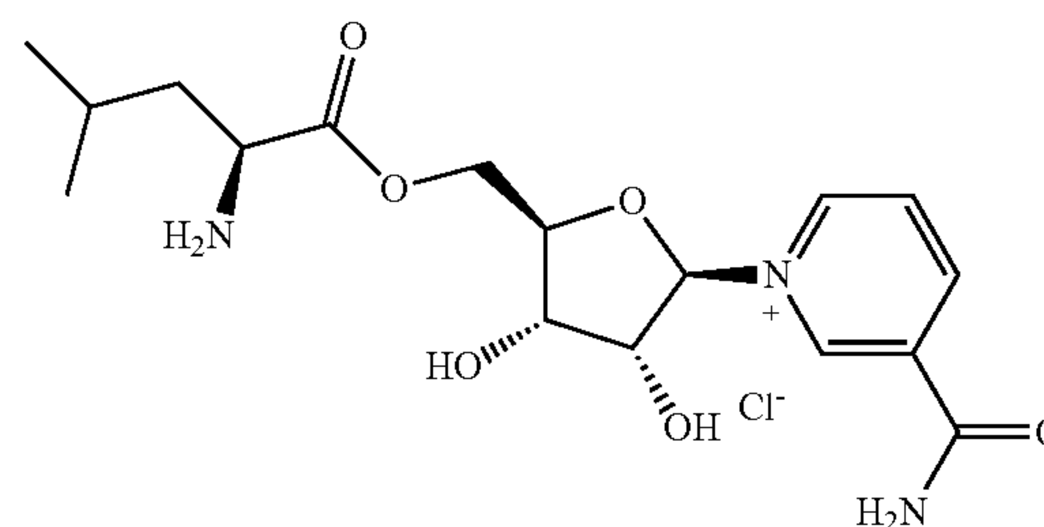
Compound 35
