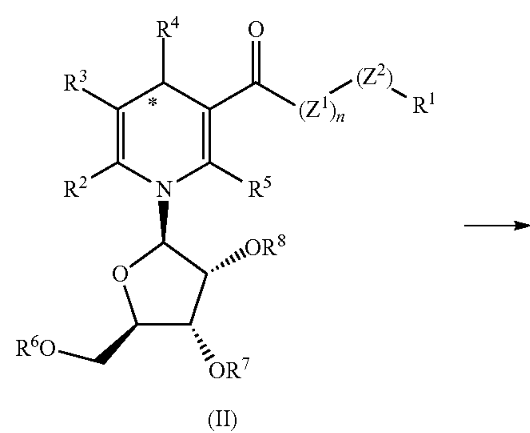
Scheme C
