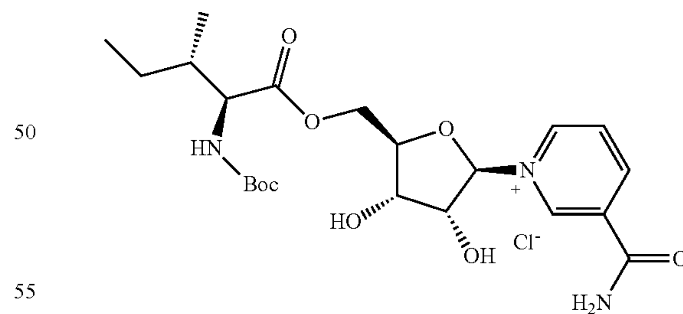
Compound 20
