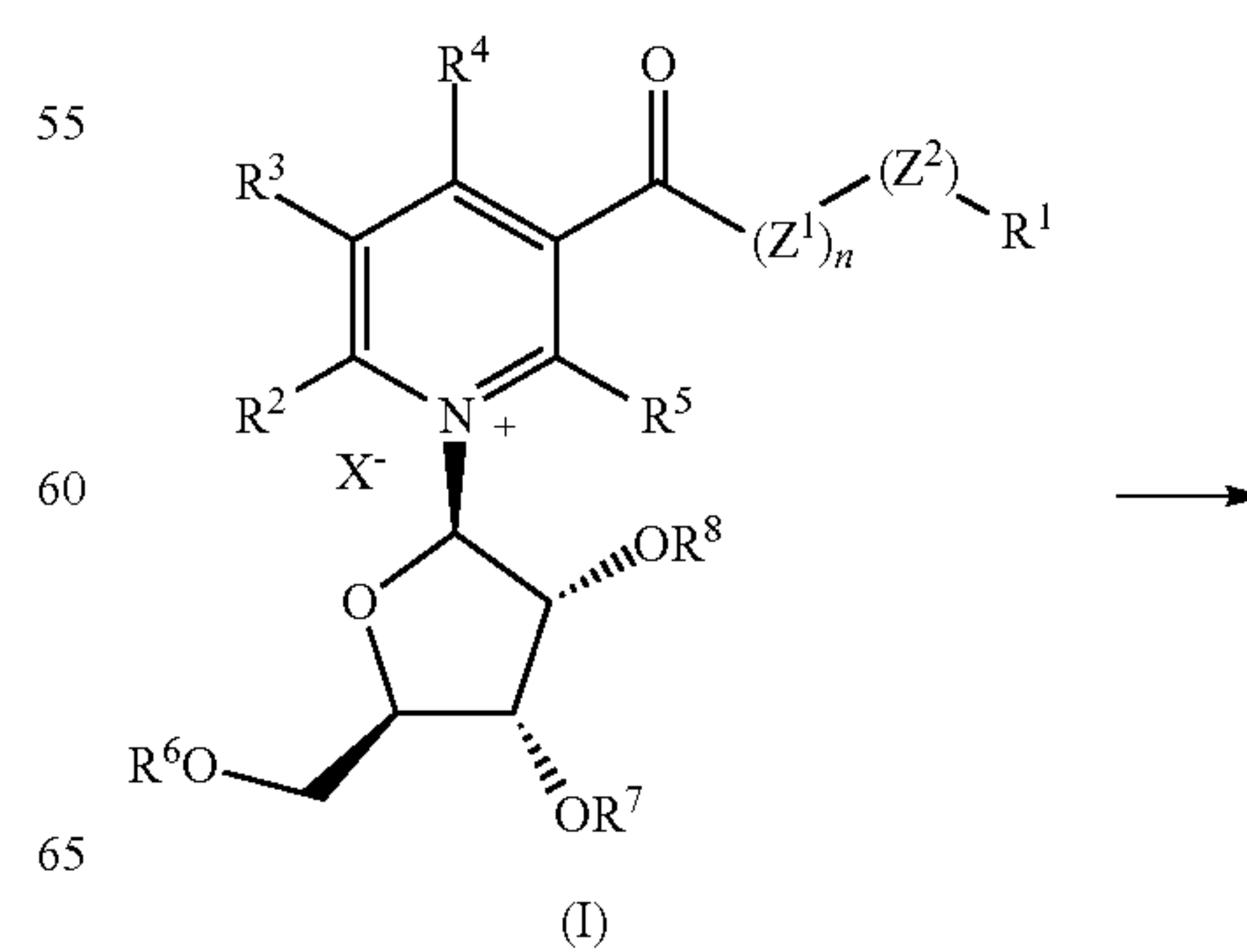
Scheme E
