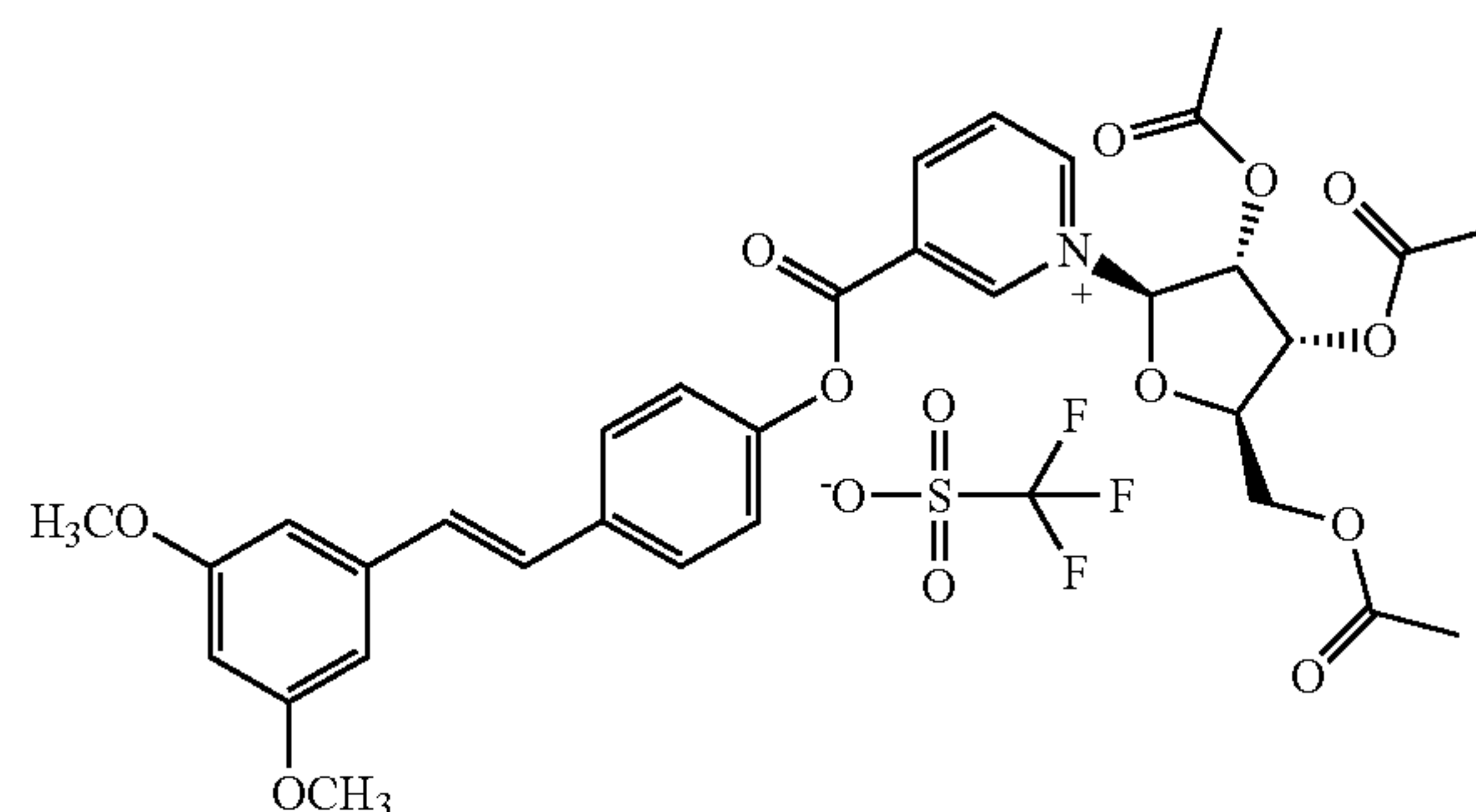
Compound 4
