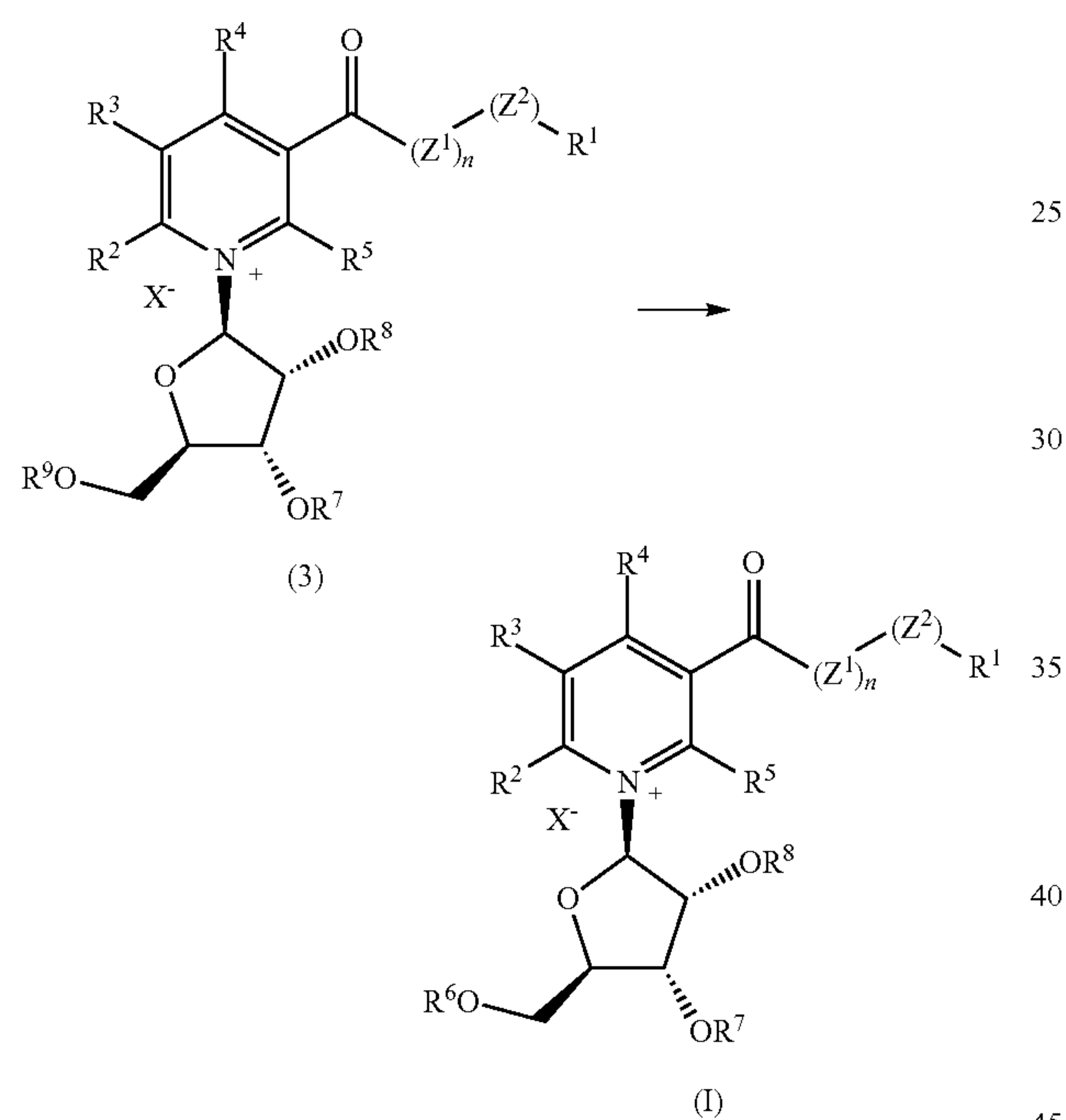
Scheme B
