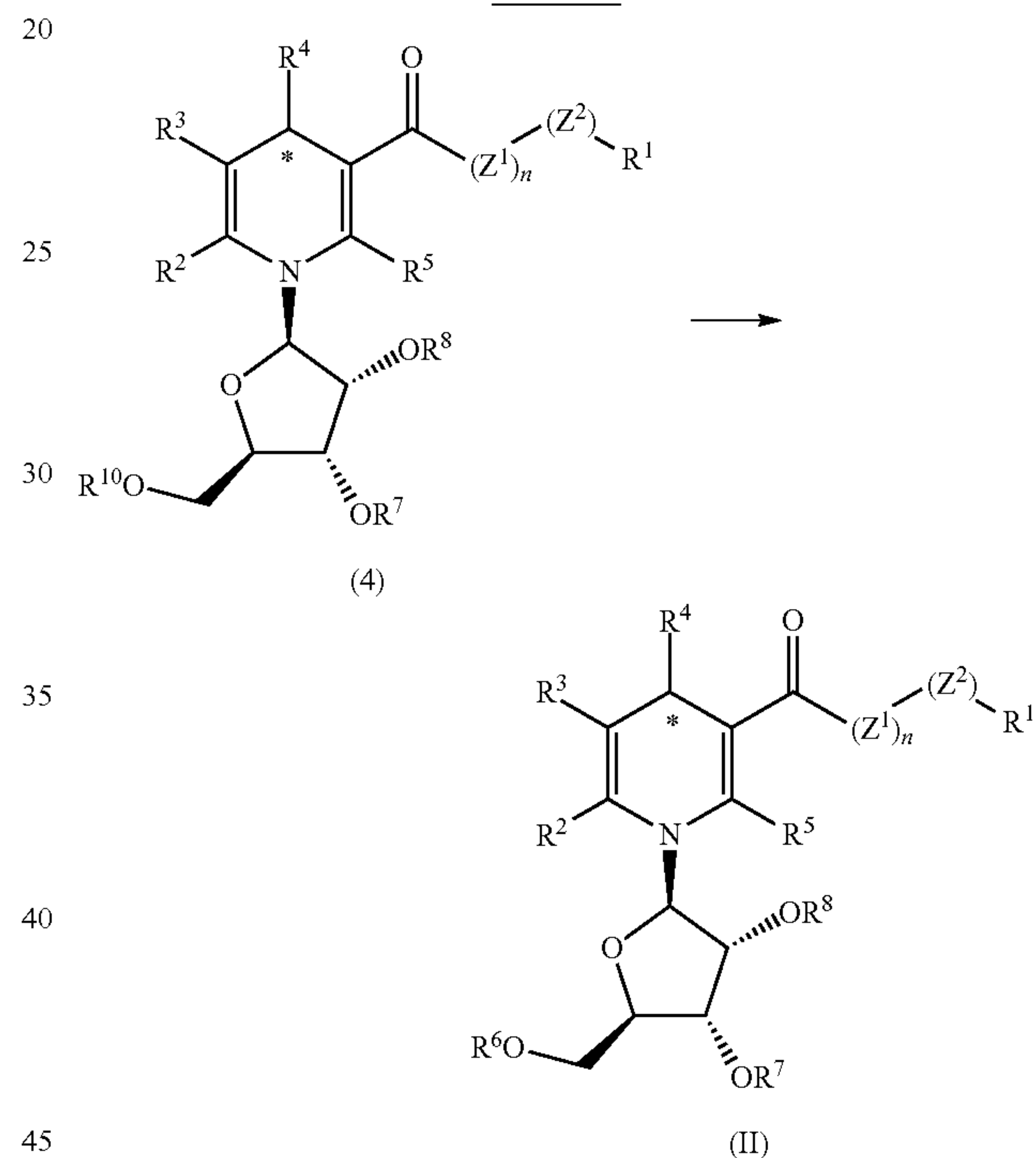
Scheme D
