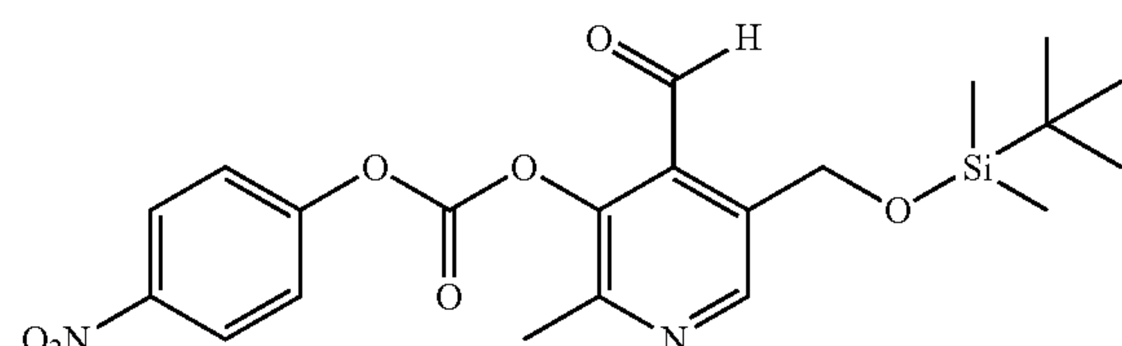
Compound 14
