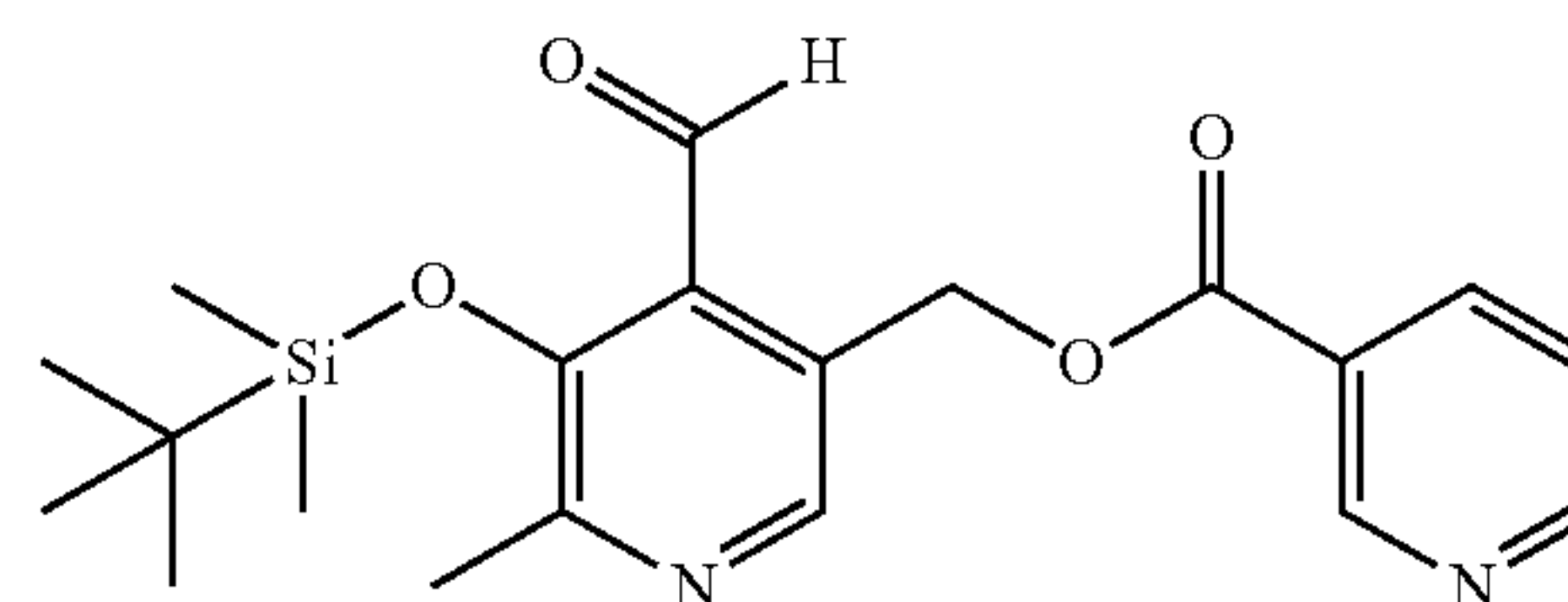
Compound 11
