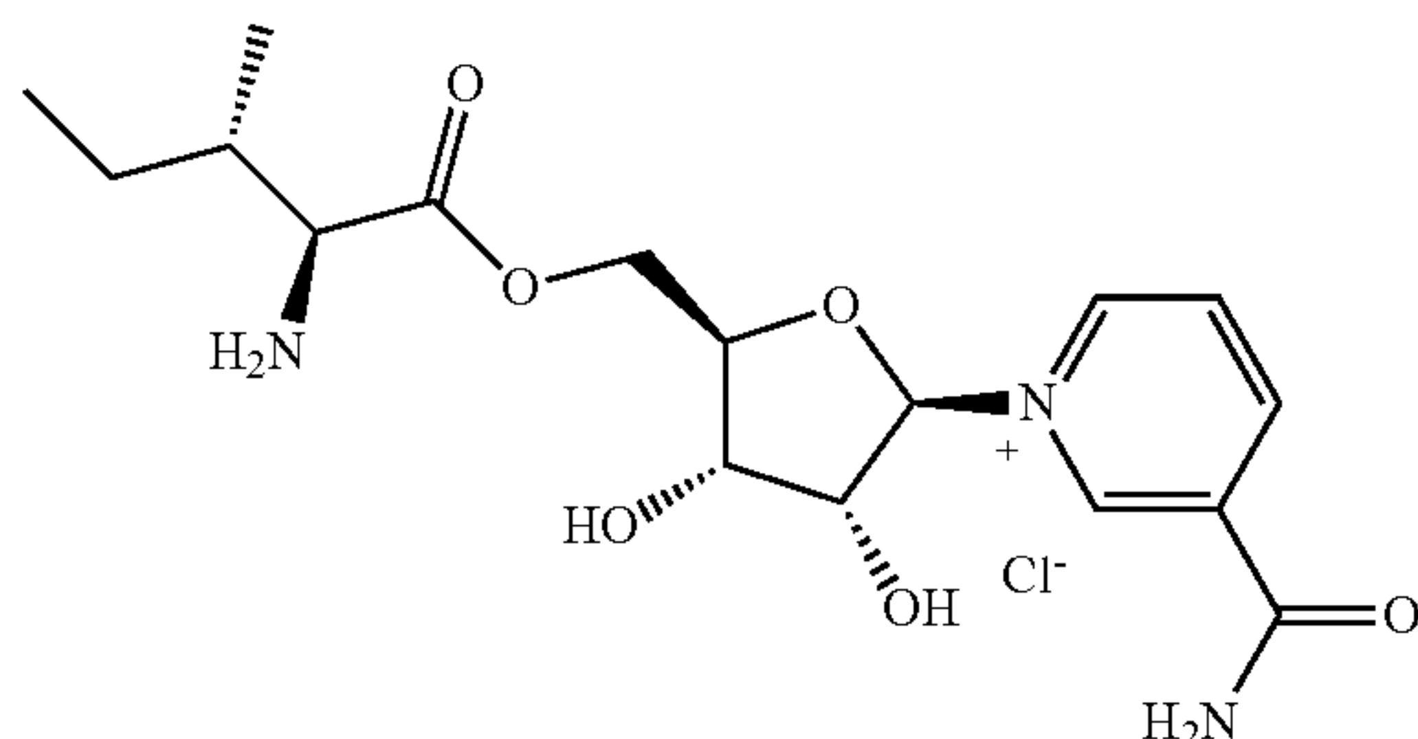
Compound 21
