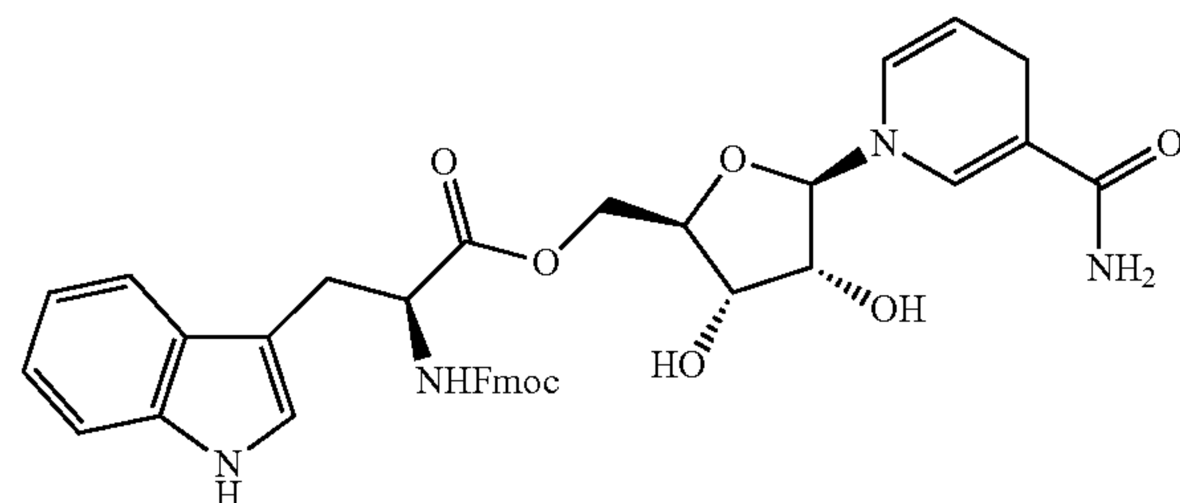
Compound 15
